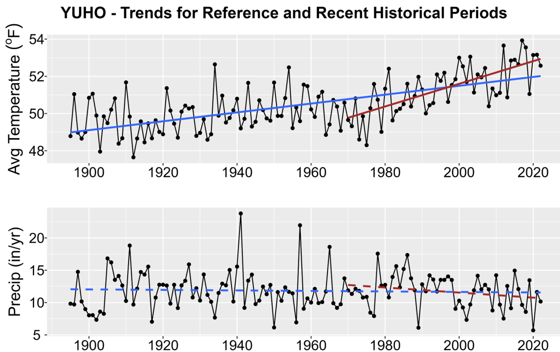
Figure 1. Historical trends in annual average temperature (upper plot) and annual total precipitation (lower plot) for YUHO from 1895-2022. Black points show yearly values while blue lines are linear regressions for the entire period record and red lines for 1970-2022 trends. Solid lines are significant trends (i.e., p < 0.05 ); dashed lines are not statistically significant.
