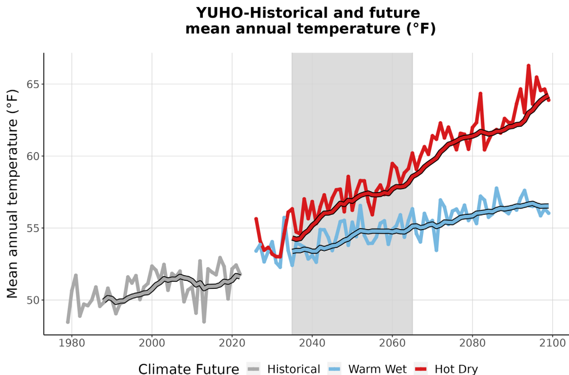
Figure 3. This graph compares observed average annual temperature at YUHO (°F) (1979-2022) with projected average annual temperature for the two climate futures over the period 2023-2099. The historically observed data
