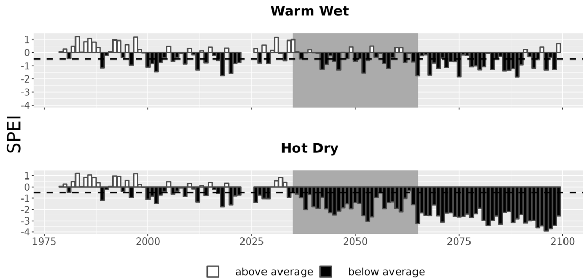
Figure 7. Drought metrics for YUHO. Drought index (SPEI; units = standard deviations from historical) timeseries for each climate future. Below-average SPEI (black bars) indicates dry conditions. The dotted line (SPEI = -0.5) indicates drought conditions.
