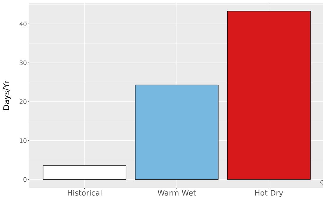
Figure 5. Metrics of extreme temperature at YUHO. The bar graph represents the average number of days annually with temperatures greater than the historical 99th percentile (95.8 °F) historically (1979-2012) and for the two climate futures (2050).
