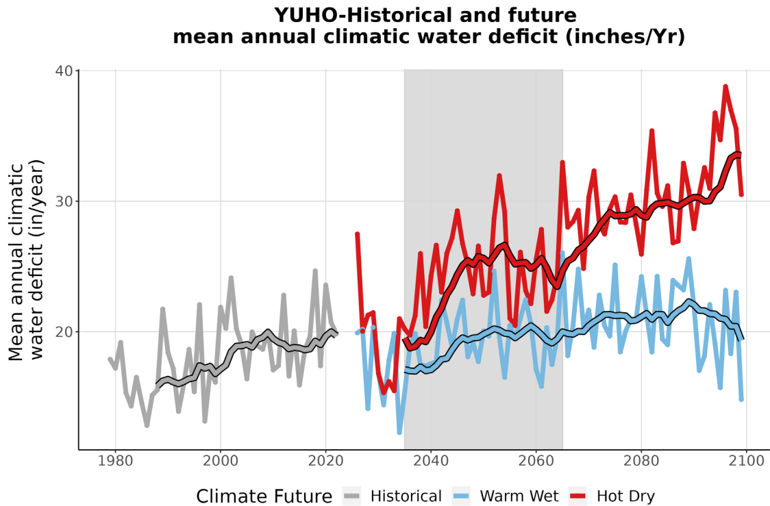
Figure 9. This line graph compares observed climatic water deficit at YUHO (inches/year) (1979-2022) with projected climatic water deficit for the two climate futures over the period 2023-2099. The historical observation data is shown in gray, the Warm Wet climate future in blue, and the Hot Dry climate future in red. The smooth line running through each projection is the 10-year running average for historical observations and future projections. Gray-shaded area represents the time period that was averaged (2035-2065) to summarize future projections for the year 2050.
