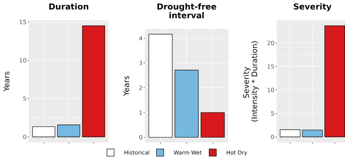
Figure 8. Drought metrics for YUHO. (Left) Average drought duration (years) historically (1979-2012) and under each climate future. (Middle) Average drought return interval (years), indicating the expected amount of time between periods of drought, historically and under each climate future. (Right) Average drought severity, a measure of drought intensity multiplied by duration, historically and under each climate future.
