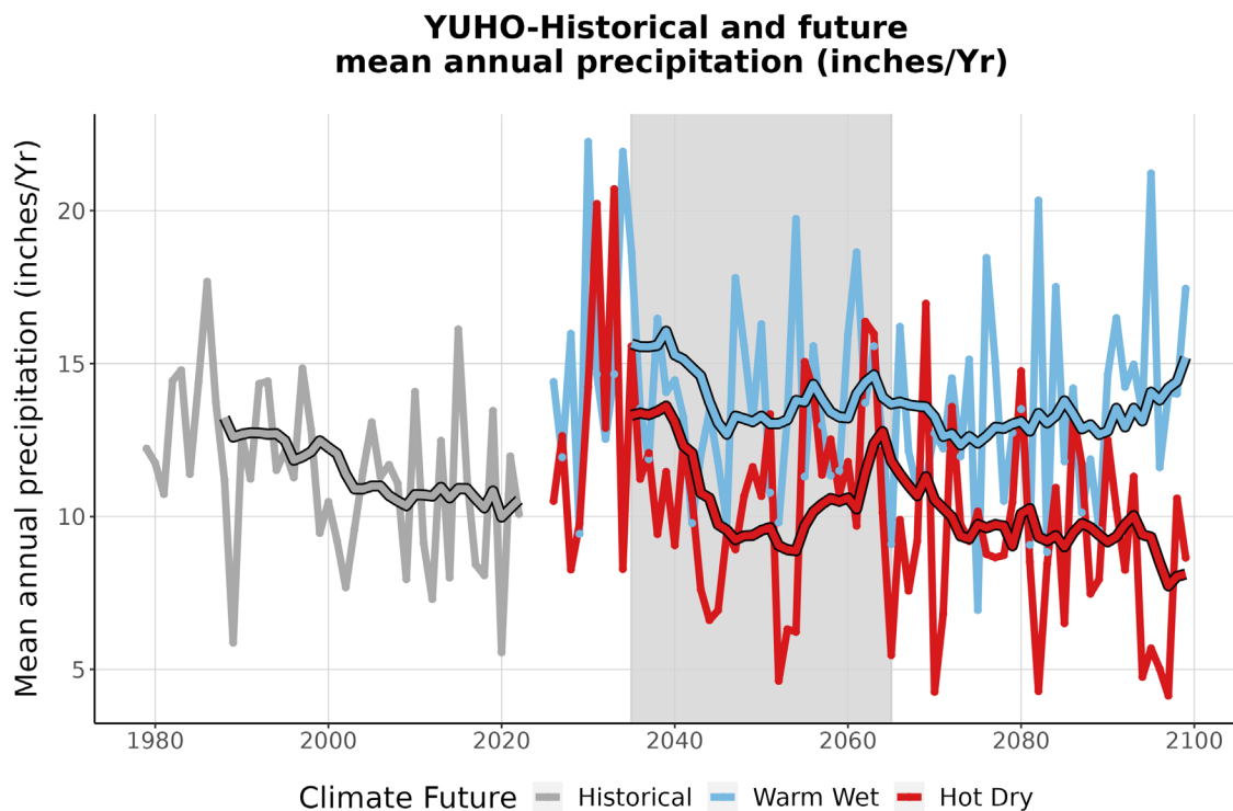
Figure 4. This graph compares observed average annual precipitation at YUHO (inches/year) (1979-2022) with projected average annual precipitation for the two climate futures over the period 2023-2099. The historically observed data is shown in gray, the Warm Wet climate future in blue, and the Hot Dry climate future in red. The smooth line running through each projection is the 10-year running average for historical observations and future projections. The gray-shaded area represents the time period that was averaged (2035-2065) to summarize future projections for the year 2050 (Appendix 1).
