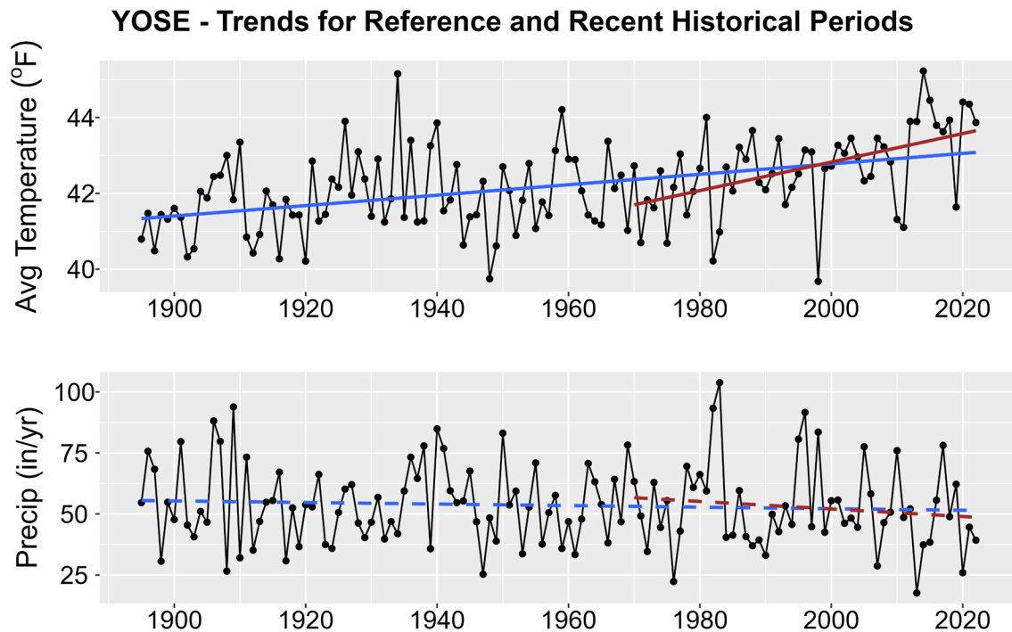
Figure 1. Historical trends in annual average temperature (upper plot) and annual total precipitation (lower plot) for YOSE from 1895-2022. Black points show yearly values while blue lines are linear regressions for the entire period record and red lines for 1970-2022 trends. Solid lines are significant trends (i.e., p < 0.05 ); dashed lines are not statistically significant.
