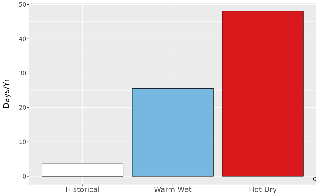
Figure 5. Metrics of extreme temperature at YOSE. The bar graph represents the average number of days annually with temperatures greater than the historical 99th percentile (77.6 °F) historically (1979-2012) and for the two climate futures (2050).
