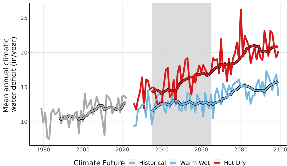
Figure 9. This line graph compares observed climatic water deficit at YOSE (inches/year) (1979-2022) with projected climatic water deficit for the two climate futures over the period 2023-2099. The historical observation data is shown in gray, the Warm Wet climate future in blue, and the Hot Dry climate future in red. The smooth line running through each projection is the 10-year running average for historical observations and future projections. Gray-shaded area represents the time period that was averaged (2035-2065) to summarize future projections for the year 2050.
