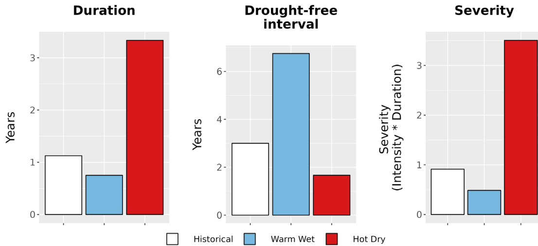
Figure 8. Drought metrics for YOSE. (Left) Average drought duration (years) historically (1979-2012) and under each climate future. (Middle) Average drought return interval (years), indicating the expected amount of time between periods of drought, historically and under each climate future. (Right) Average drought severity, a measure of drought intensity multiplied by duration, historically and under each climate future.
