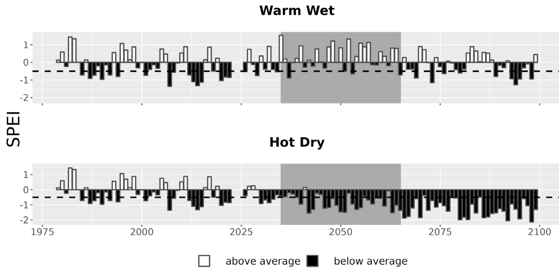
Figure 7. Drought metrics for YOSE. Drought index (SPEI; units = standard deviations from historical) timeseries for each climate future. Below-average SPEI (black bars) indicates dry conditions. The dotted line (SPEI = -0.5) indicates drought conditions.
