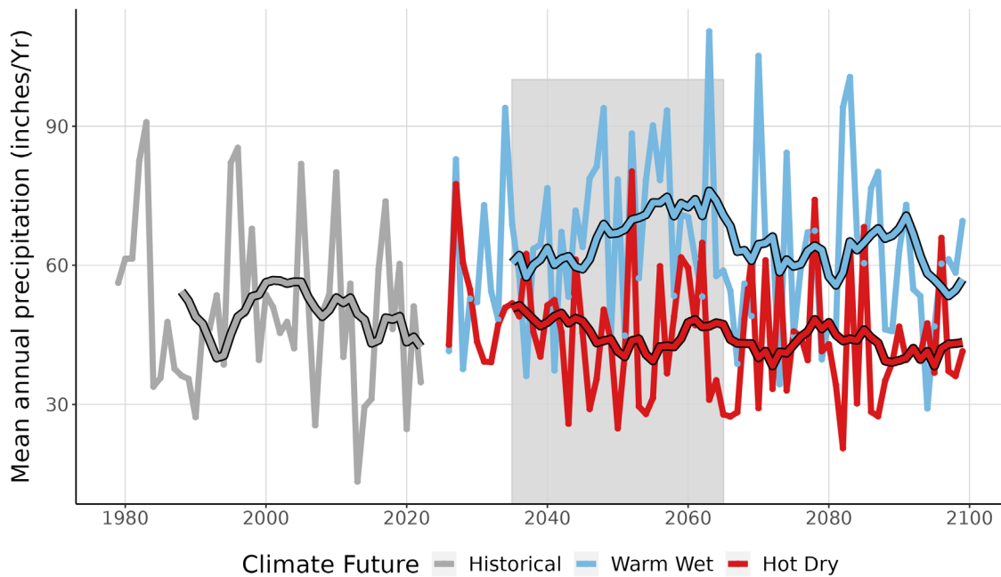
Figure 4. This graph compares observed average annual precipitation at YOSE (inches/year) (1979-2022) with projected average annual precipitation for the two climate futures over the period 2023-2099. The historically observed data is shown in gray, the Warm Wet climate future in blue, and the Hot Dry climate future in red. The smooth line running through each projection is the 10-year running average for historical observations and future projections. The gray-shaded area represents the time period that was averaged (2035-2065) to summarize future projections for the year 2050 (Appendix 1).
