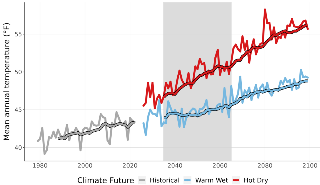
Figure 3. This graph compares observed average annual temperature at YOSE (°F) (1979-2022) with projected average annual temperature for the two climate futures over the period 2023-2099. The historically observed data is shown in gray, the Warm Wet climate future in blue, and the Hot Dry climate future in red. The smooth line running through each projection is the 10-year running average for historical observations and future projections. Gray-shaded area represents the time period that was averaged (2035-2065) to summarize future projections for the year 2050 (Appendix 1).
