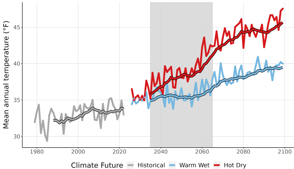
Figure 3. This graph compares observed average annual temperature at YELL (°F) (1979-2022) with projected average annual temperature for the two climate futures over the period 2023-2099. The historically observed data is shown in gray, the Warm Wet climate future in blue, and the Hot Dry climate future in red. The smooth line running through each projection is the 10-year running average for historical observations and future projections. Gray-shaded area represents the time period that was averaged (2035-2065) to summarize future projections for the year 2050 (Appendix 1).
