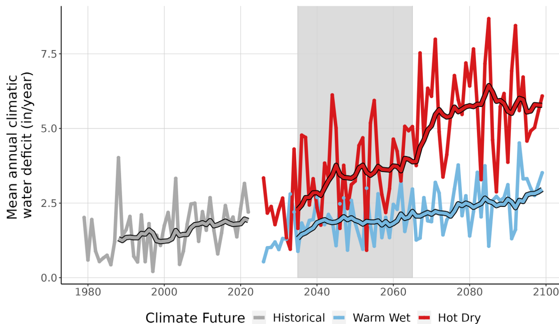
Figure 9. This line graph compares observed climatic water deficit at YELL (inches/year) (1979-2022) with projected climatic water deficit for the two climate futures over the period 2023-2099. The historical observation data is shown in gray, the Warm Wet climate future in blue, and the Hot Dry climate future in red. The smooth line running through each projection is the 10-year running average for historical observations and future projections. Gray-shaded area represents the time period that was averaged (2035-2065) to summarize future projections for the year 2050.
