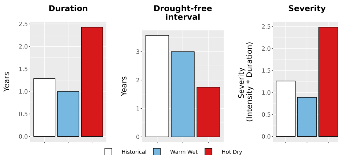
Figure 8. Drought metrics for YELL. (Left) Average drought duration (years) historically (1979-2012) and under each climate future. (Middle) Average drought return interval (years), indicating the expected amount of time between periods of drought, historically and under each climate future. (Right) Average drought severity, a measure of drought intensity multiplied by duration, historically and under each climate future.
