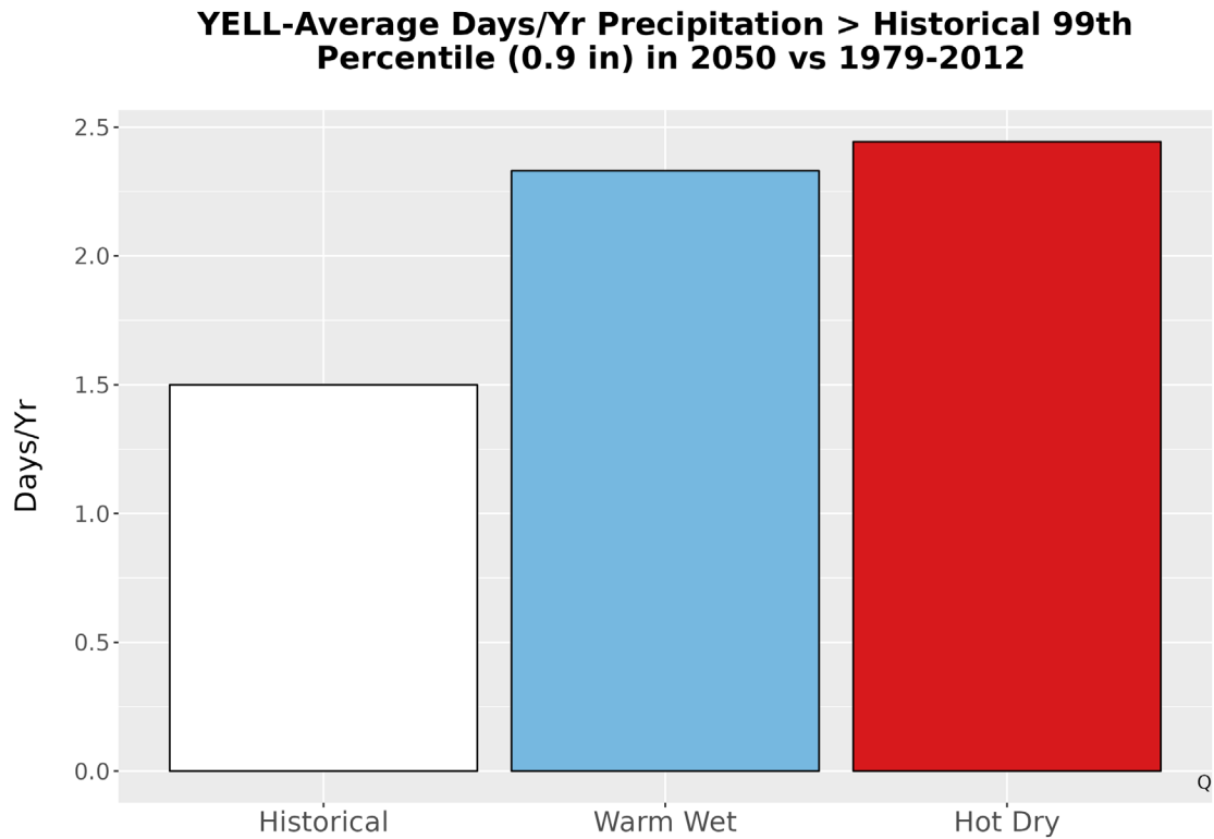
Figure 6. Average number of days annually with precipitation exceeding the 99th percentile (0.9 in.) of precipitation from the historical period 1979-2012 and for each climate future.
