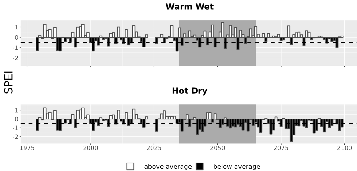
Figure 7. Drought metrics for YELL. Drought index (SPEI; units = standard deviations from historical) timeseries for each climate future. Below-average SPEI (black bars) indicates dry conditions. The dotted line (SPEI = -0.5) indicates drought conditions.
