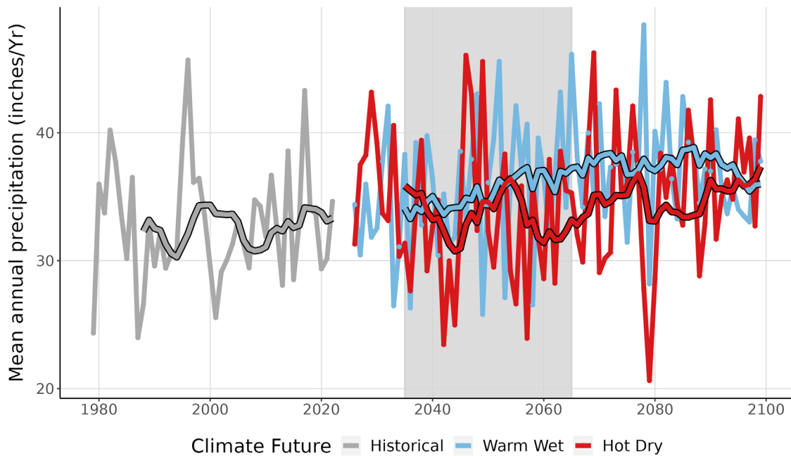
Figure 4. This graph compares observed average annual precipitation at YELL (inches/year) (1979-2022) with projected average annual precipitation for the two climate futures over the period 2023-2099. The historically observed data is shown in gray, the Warm Wet climate future in blue, and the Hot Dry climate future in red. The smooth line running through each projection is the 10-year running average for historical observations and future projections. The gray-shaded area represents the time period that was averaged (2035-2065) to summarize future projections for the year 2050 (Appendix 1).
