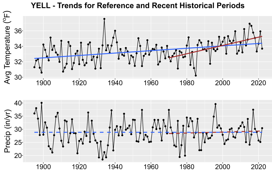
Figure 1. Historical trends in annual average temperature (upper plot) and annual total precipitation (lower plot) for YELL from 1895-2022. Black points show yearly values while blue lines are linear regressions for the entire period record and red lines for 1970-2022 trends. Solid lines are significant trends (i.e., p < 0.05 ); dashed lines are not statistically significant.
