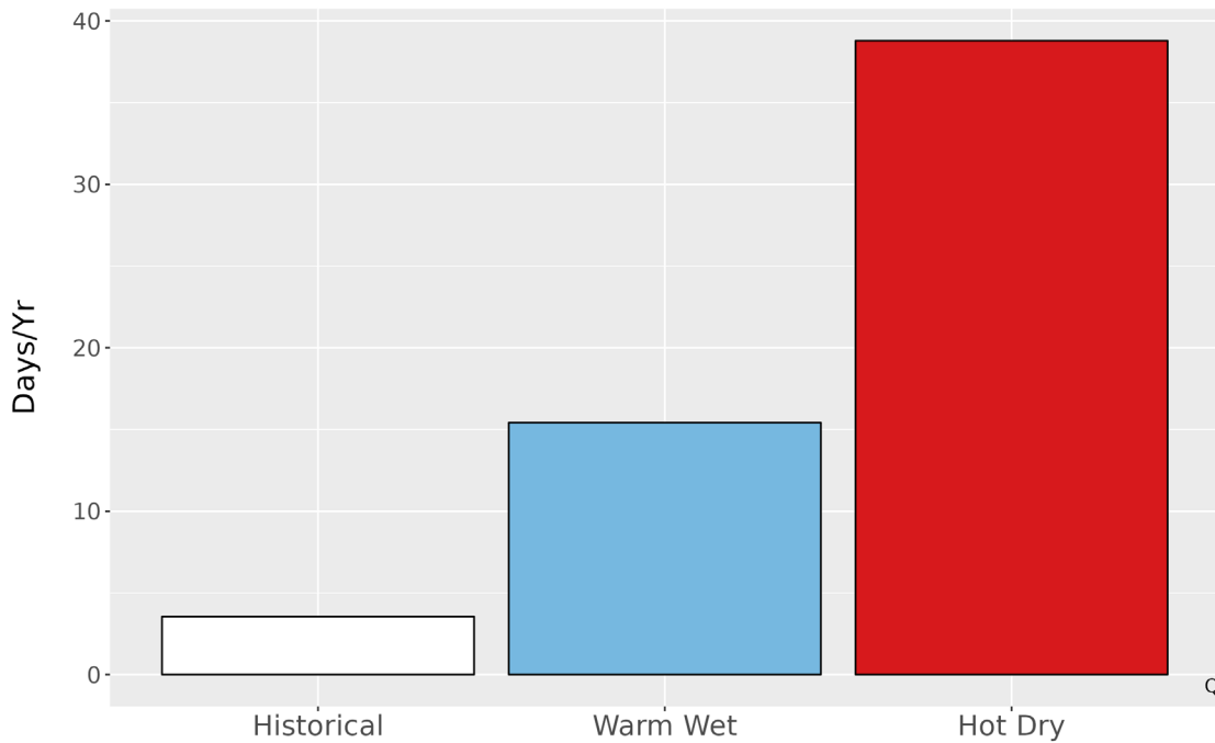
Figure 5. Metrics of extreme temperature at YELL. The bar graph represents the average number of days annually with temperatures greater than the historical 99th percentile (79.6 °F) historically (1979-2012) and for the two climate futures (2050).
