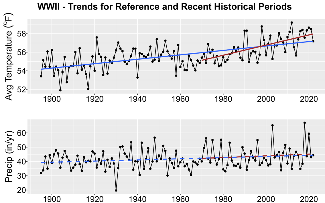
Figure 1. Historical trends in annual average temperature (upper plot) and annual total precipitation (lower plot) for WWII from 1895-2022. Black points show yearly values while blue lines are linear regressions for the entire period record and red lines for 1970-2022 trends. Solid lines are significant trends (i.e., p < 0.05 ); dashed lines are not statistically significant.
