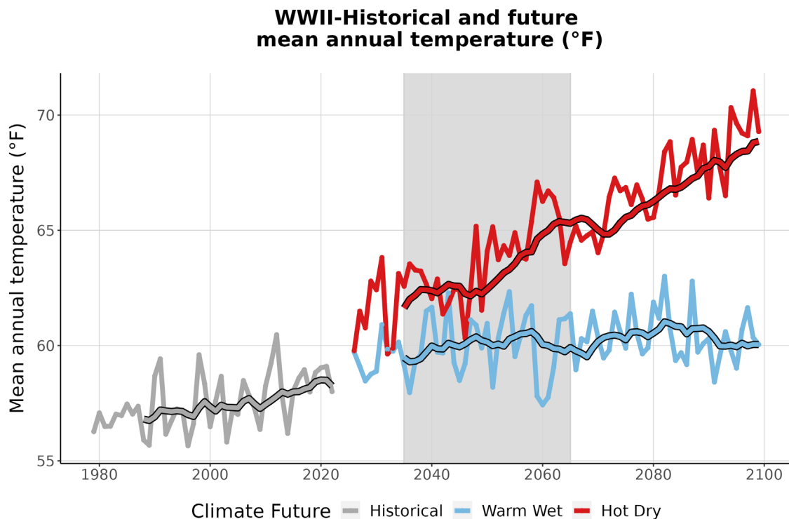
Figure 3. This graph compares observed average annual temperature at WWII (°F) (1979-2022) with projected average annual temperature for the two climate futures over the period 2023-2099. The historically observed data
