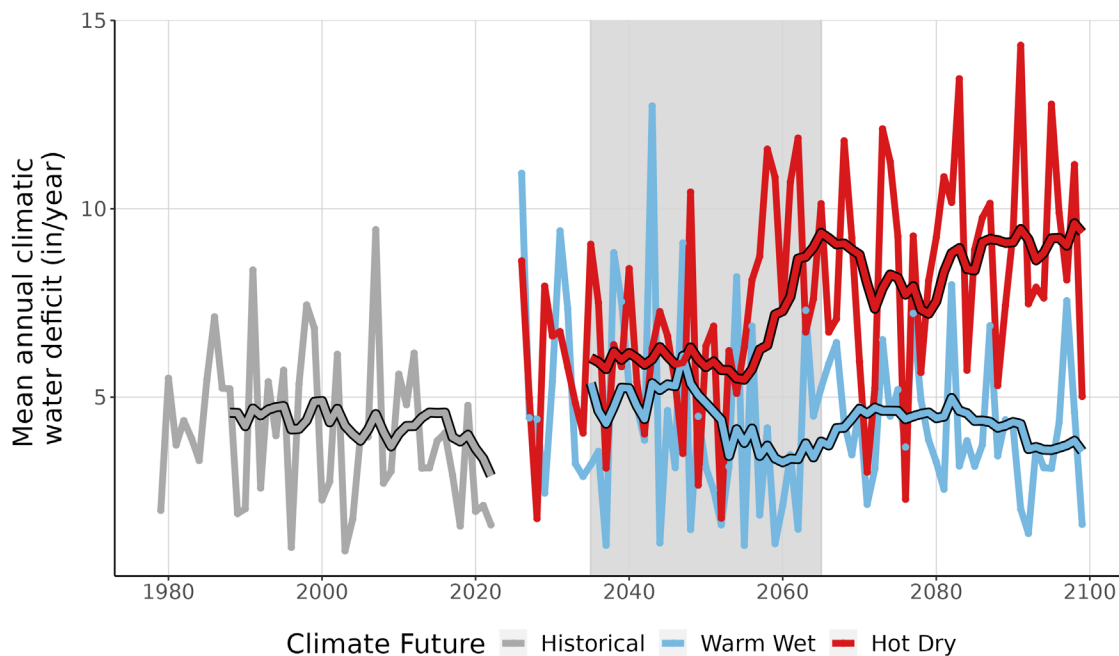
Figure 9. This line graph compares observed climatic water deficit at WWII (inches/year) (1979-2022) with projected climatic water deficit for the two climate futures over the period 2023-2099. The historical observation data is shown in gray, the Warm Wet climate future in blue, and the Hot Dry climate future in red. The smooth line running through each projection is the 10-year running average for historical observations and future projections. Gray-shaded area represents the time period that was averaged (2035-2065) to summarize future projections for the year 2050.
