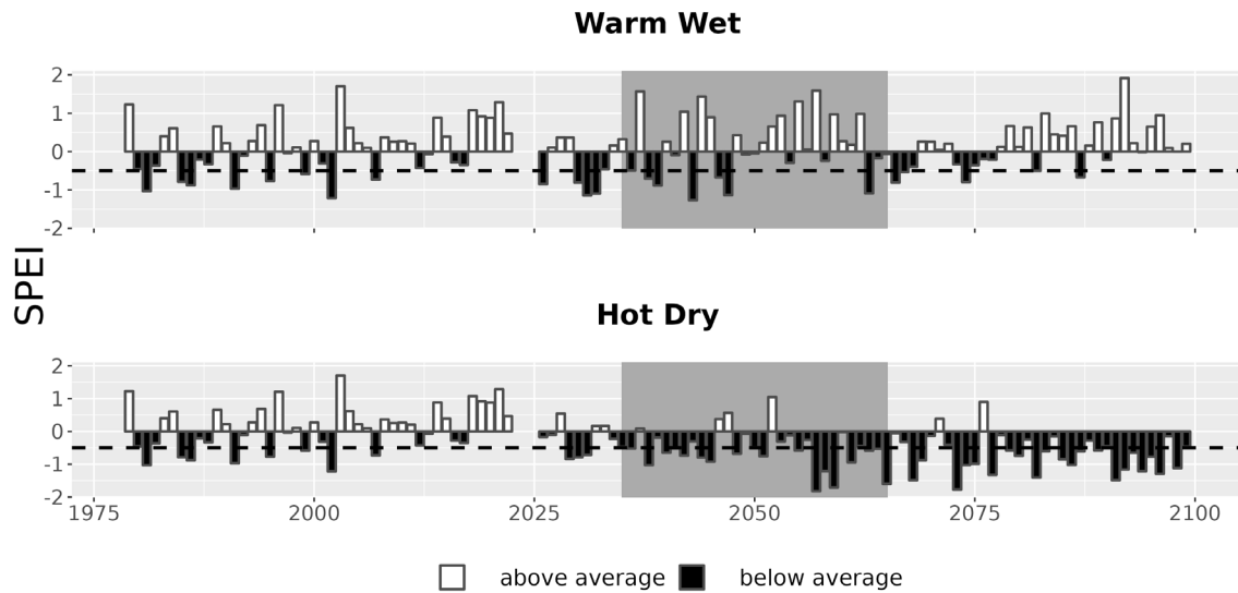
Figure 7. Drought metrics for WWII. Drought index (SPEI; units = standard deviations from historical) timeseries for each climate future. Below-average SPEI (black bars) indicates dry conditions. The dotted line (SPEI = -0.5) indicates drought conditions.
