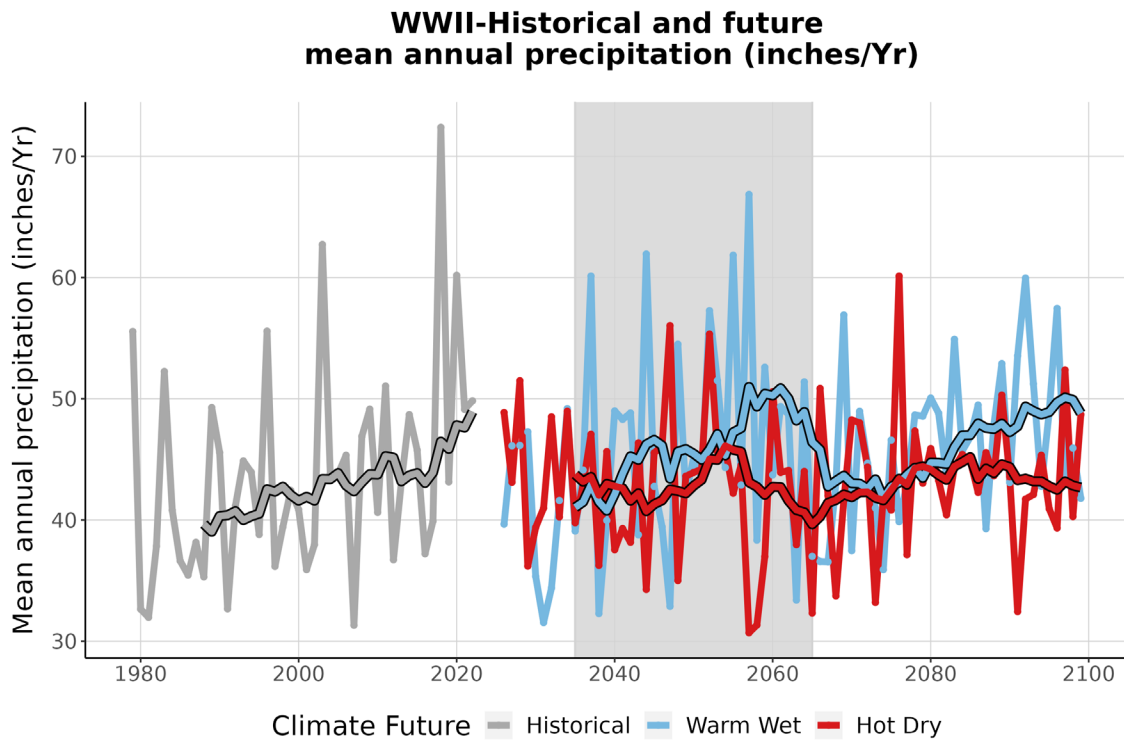
Figure 4. This graph compares observed average annual precipitation at WWII (inches/year) (1979-2022) with projected average annual precipitation for the two climate futures over the period 2023-2099. The historically observed data is shown in gray, the Warm Wet climate future in blue, and the Hot Dry climate future in red. The smooth line running through each projection is the 10-year running average for historical observations and future projections. The gray-shaded area represents the time period that was averaged (2035-2065) to summarize future projections for the year 2050 (Appendix 1).
