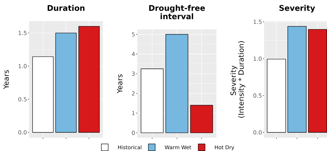
Figure 8. Drought metrics for WWII. (Left) Average drought duration (years) historically (1979-2012) and under each climate future. (Middle) Average drought return interval (years), indicating the expected amount of time between periods of drought, historically and under each climate future. (Right) Average drought severity, a measure of drought intensity multiplied by duration, historically and under each climate future.
