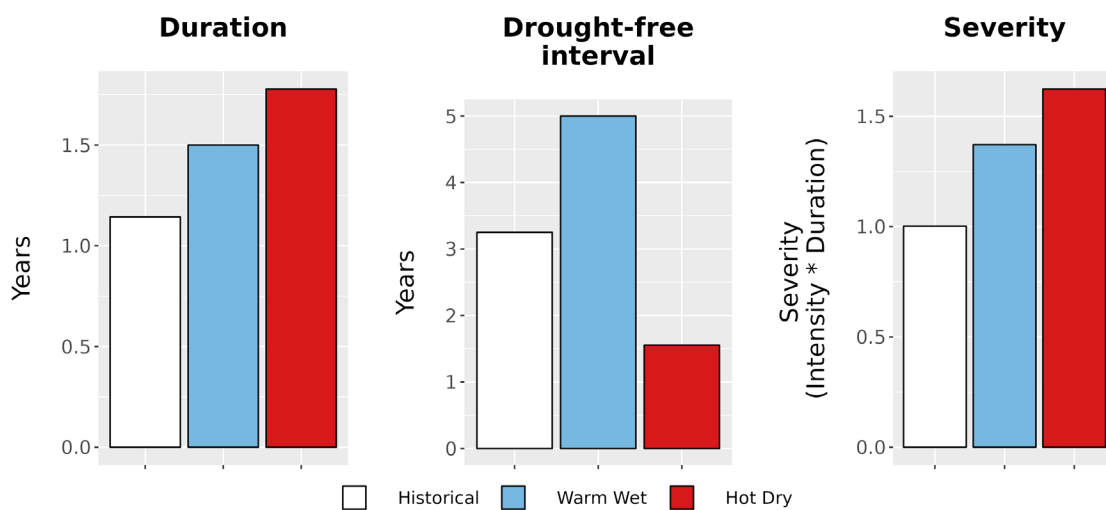
Figure 8. Drought metrics for WOTR. (Left) Average drought duration (years) historically (1979-2012) and under each climate future. (Middle) Average drought return interval (years), indicating the expected amount of time between periods of drought, historically and under each climate future. (Right) Average drought severity, a measure of drought intensity multiplied by duration, historically and under each climate future.
