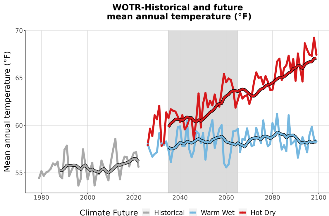
Figure 3. This graph compares observed average annual temperature at WOTR (°F) (1979-2022) with projected average annual temperature for the two climate futures over the period 2023-2099. The historically observed data
