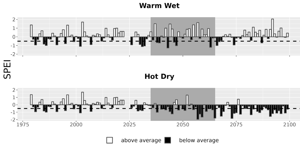
Figure 7. Drought metrics for WOTR. Drought index (SPEI; units = standard deviations from historical) timeseries for each climate future. Below-average SPEI (black bars) indicates dry conditions. The dotted line (SPEI = -0.5) indicates drought conditions.
