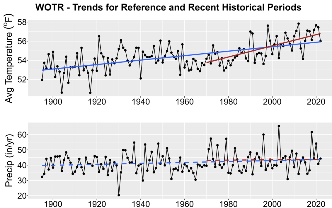
Figure 1. Historical trends in annual average temperature (upper plot) and annual total precipitation (lower plot) for WOTR from 1895-2022. Black points show yearly values while blue lines are linear regressions for the entire period record and red lines for 1970-2022 trends. Solid lines are significant trends (i.e., p < 0.05 ); dashed lines are not statistically significant.
