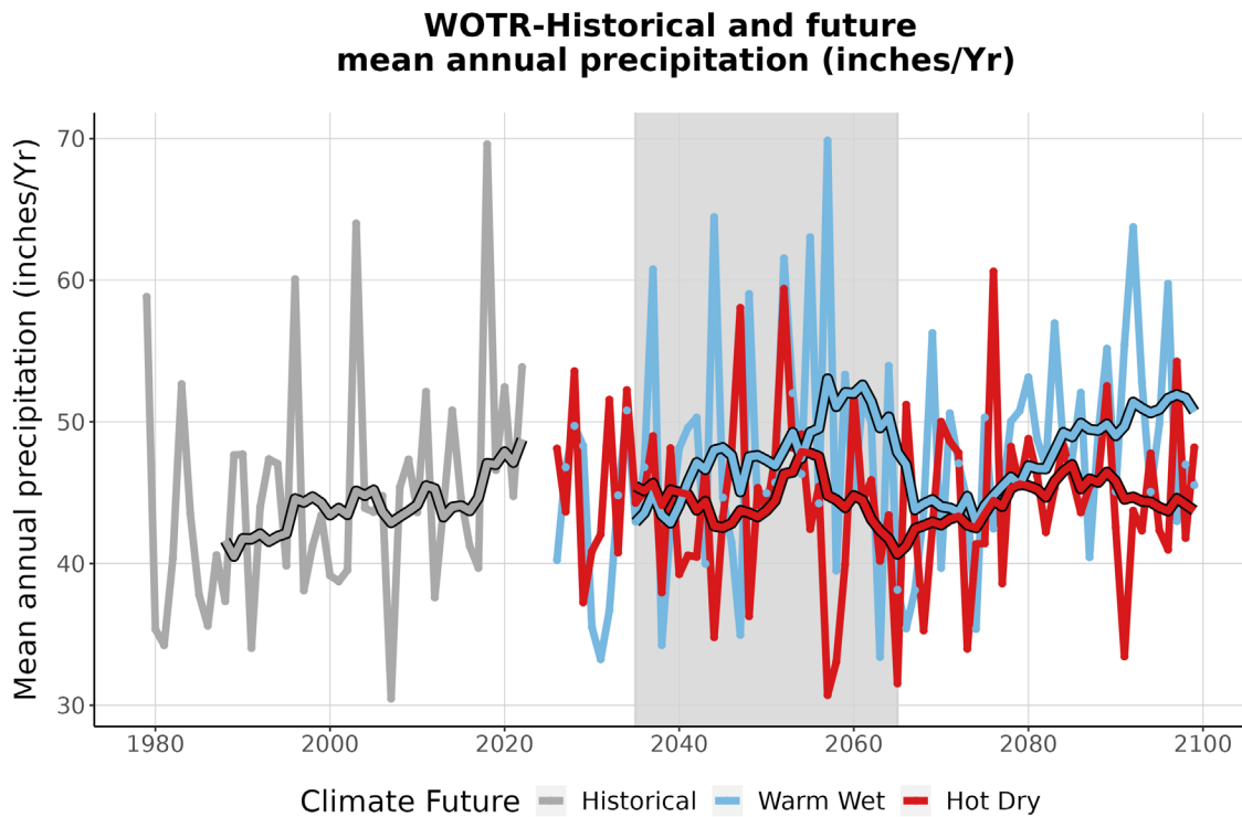
Figure 4. This graph compares observed average annual precipitation at WOTR (inches/year) (1979-2022) with projected average annual precipitation for the two climate futures over the period 2023-2099. The historically observed data is shown in gray, the Warm Wet climate future in blue, and the Hot Dry climate future in red. The smooth line running through each projection is the 10-year running average for historical observations and future projections. The gray-shaded area represents the time period that was averaged (2035-2065) to summarize future projections for the year 2050 (Appendix 1).
