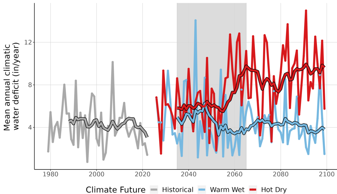
Figure 9. This line graph compares observed climatic water deficit at WOTR (inches/year) (1979-2022) with projected climatic water deficit for the two climate futures over the period 2023-2099. The historical observation data is shown in gray, the Warm Wet climate future in blue, and the Hot Dry climate future in red. The smooth line running through each projection is the 10-year running average for historical observations and future projections. Gray-shaded area represents the time period that was averaged (2035-2065) to summarize future projections for the year 2050.
