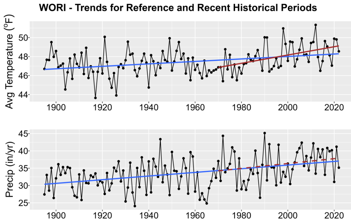
Figure 1. Historical trends in annual average temperature (upper plot) and annual total precipitation (lower plot) for WORI from 1895-2022. Black points show yearly values while blue lines are linear regressions for the entire period record and red lines for 1970-2022 trends. Solid lines are significant trends (i.e., p < 0.05 ); dashed lines are not statistically significant.
