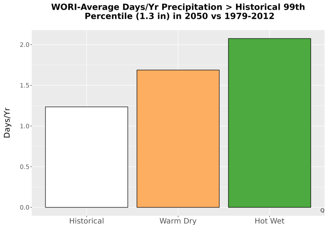
Figure 6. Average number of days annually with precipitation exceeding the 99th percentile (1.3 in.) of precipitation from the historical period 1979-2012 and for each climate future.
