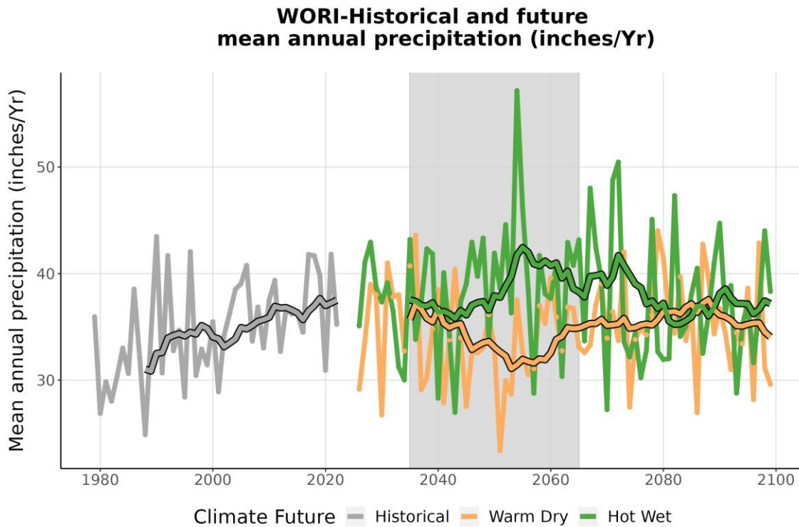
Figure 4. This graph compares observed average annual precipitation at WOR1 (inches/year) (1979-2022) with projected average annual precipitation for the two climate futures over the period 2023-2099. The historically observed data is shown in gray, the Warm Dry climate future in orange, and the Hot Wet climate future in green. The smooth line running through each projection is the 10-year running average for historical observations and future projections. The gray-shaded area represents the time period that was averaged (2035-2065) to summarize future projections for the year 2050 (Appendix 1).
