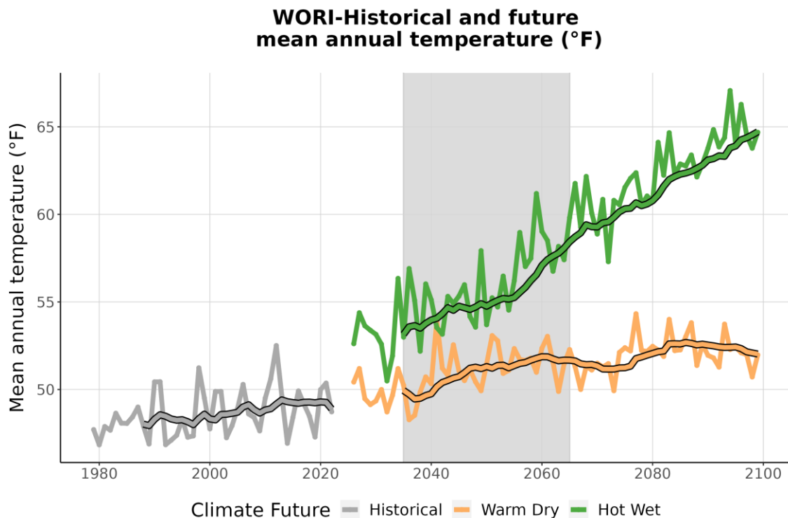
Figure 3. This graph compares observed average annual temperature at WORI (°F) (1979-2022) with projected average annual temperature for the two climate futures over the period 2023-2099. The historically observed data
