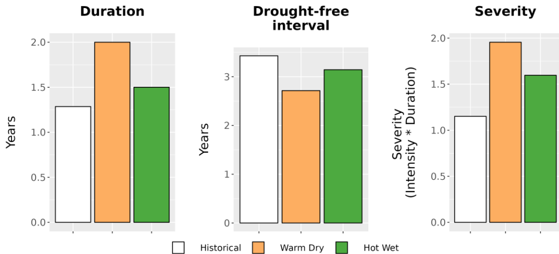
Figure 8. Drought metrics for WORI. (Left) Average drought duration (years) historically (1979-2012) and under each climate future. (Middle) Average drought return interval (years), indicating the expected amount of time between periods of drought, historically and under each climate future. (Right) Average drought severity, a measure of drought intensity multiplied by duration, historically and under each climate future.
