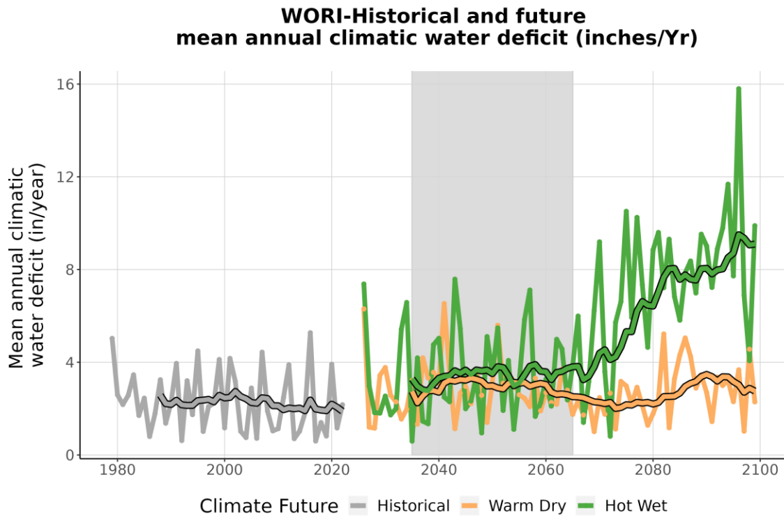
Figure 9. This line graph compares observed climatic water deficit at WORI (inches/year) (1979-2022) with projected climatic water deficit for the two climate futures over the period 2023-2099. The historical observation data is shown in gray, the Warm Dry climate future in orange, and the Hot Wet climate future in green. The smooth line running through each projection is the 10-year running average for historical observations and future projections. Gray-shaded area represents the time period that was averaged (2035-2065) to summarize future projections for the year 2050.
