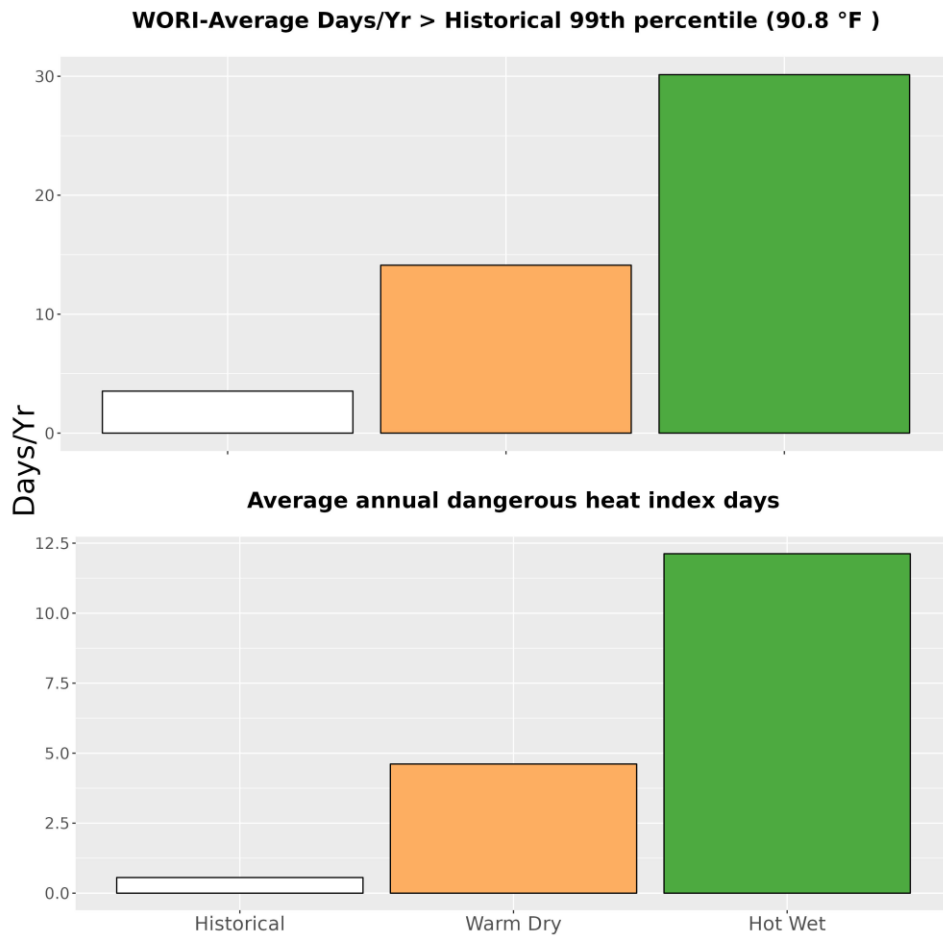
Figure 5. The upper bar graph represents the average number of days annually with temperatures greater than the historical 99th percentile (90.8 °F) historically (1979-2012) and for the two climate futures (2050). The bottom bar graph represents the average annual number of dangerous heat index days historically and for the two climate futures. Dangerous heat index days are days that exceed 105 °F.
