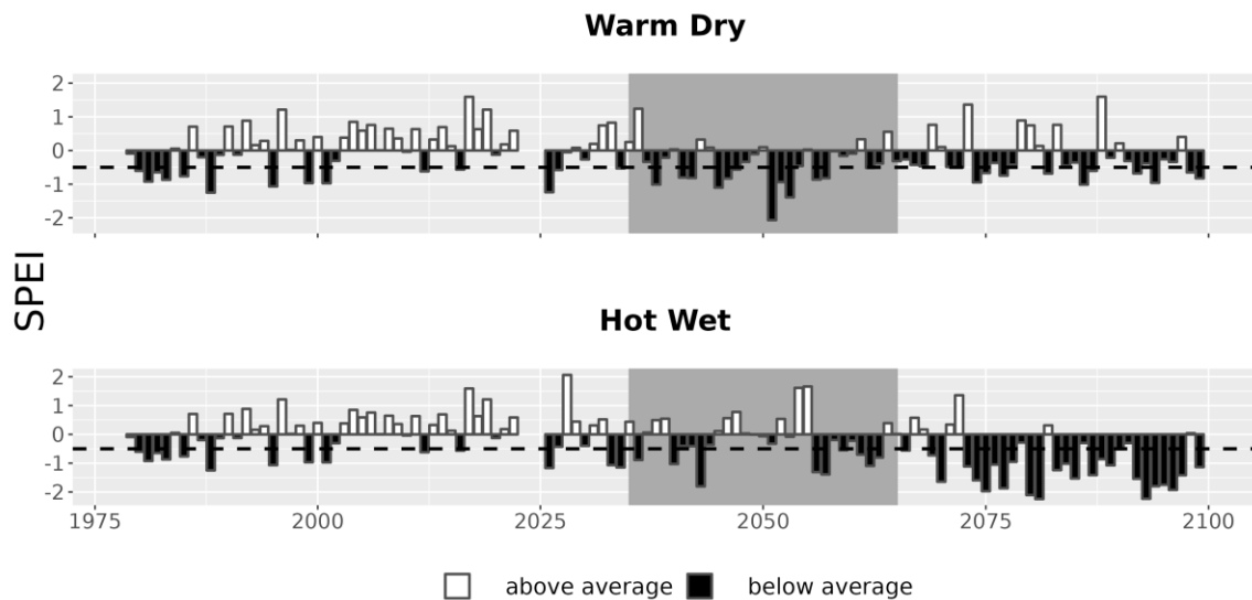
Figure 7. Drought metrics for WORL. Drought index (SPEI; units = standard deviations from historical) timeseries for each climate future. Below-average SPEI (black bars) indicates dry conditions. The dotted line (SPEI = -0.5) indicates drought conditions.
