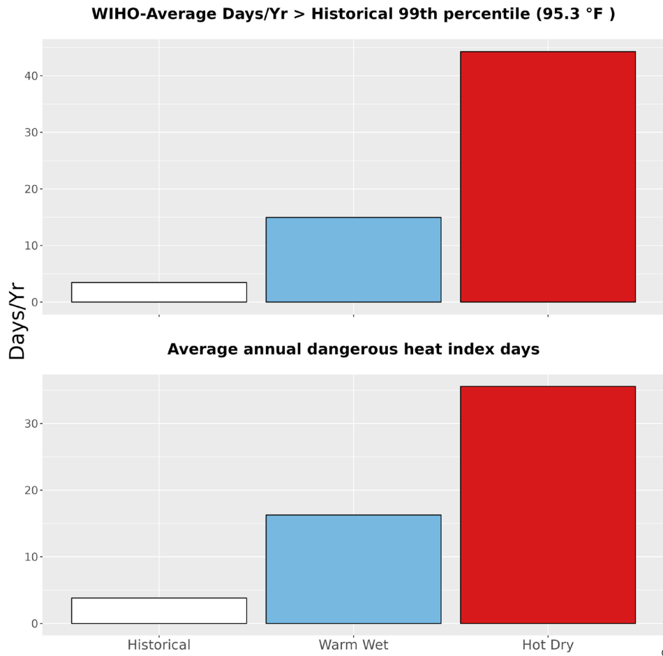
Figure 5. The upper bar graph represents the average number of days annually with temperatures greater than the historical 99th percentile (95.3 °F) historically (1979-2012) and for the two climate futures (2050). The bottom bar graph represents the average annual number of dangerous heat index days historically and for the two climate futures. Dangerous heat index days are days that exceed 105 °F.
