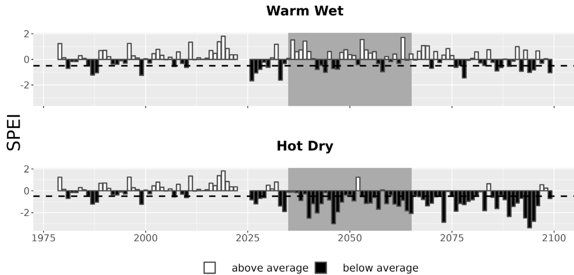
Figure 7. Drought metrics for WIHO. Drought index (SPEI; units = standard deviations from historical) timeseries for each climate future. Below-average SPEI (black bars) indicates dry conditions. The dotted line (SPEI = -0.5) indicates drought conditions.
