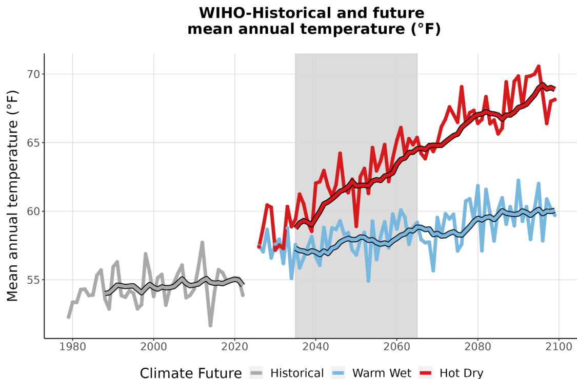
Figure 3. This graph compares observed average annual temperature at WIHO (°F) (1979-2022) with projected average annual temperature for the two climate futures over the period 2023-2099. The historically observed data
