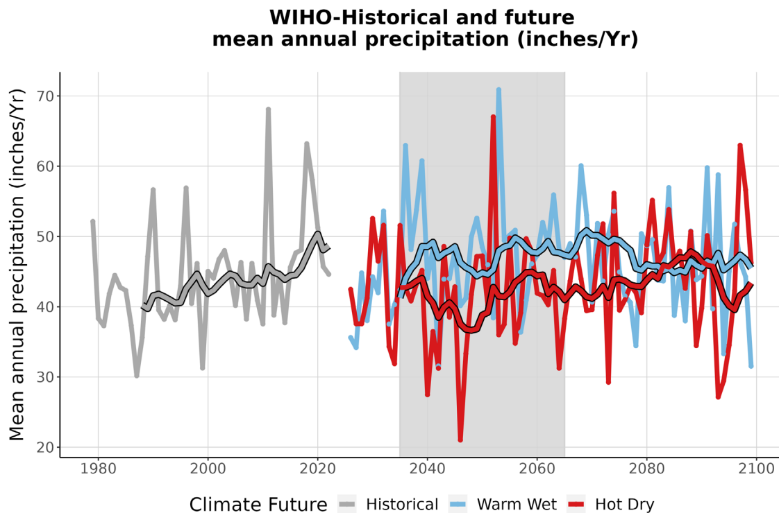
Figure 4. This graph compares observed average annual precipitation at WIHO (inches/year) (1979-2022) with projected average annual precipitation for the two climate futures over the period 2023-2099. The historically observed data is shown in gray, the Warm Wet climate future in blue, and the Hot Dry climate future in red. The smooth line running through each projection is the 10-year running average for historical observations and future projections. The gray-shaded area represents the time period that was averaged (2035-2065) to summarize future projections for the year 2050 (Appendix 1).
