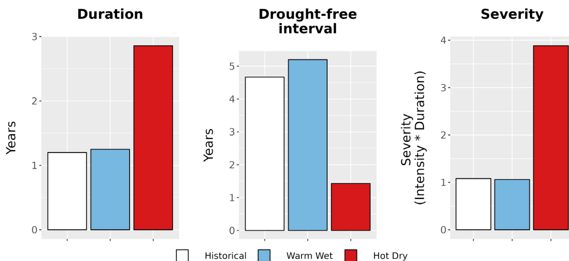
Figure 8. Drought metrics for WIHO. (Left) Average drought duration (years) historically (1979-2012) and under each climate future. (Middle) Average drought return interval (years), indicating the expected amount of time between periods of drought, historically and under each climate future. (Right) Average drought severity, a measure of drought intensity multiplied by duration, historically and under each climate future.
