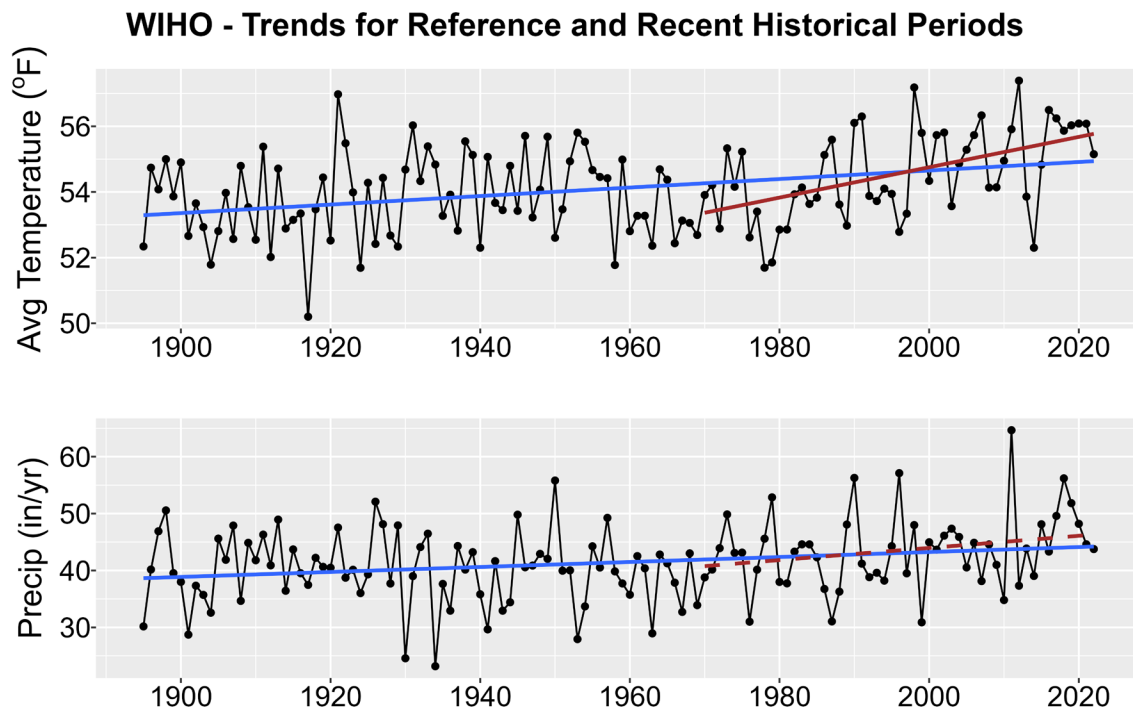
Figure 1. Historical trends in annual average temperature (upper plot) and annual total precipitation (lower plot) for WIHO from 1895-2022. Black points show yearly values while blue lines are linear regressions for the entire period record and red lines for 1970-2022 trends. Solid lines are significant trends (i.e., p < 0.05 ); dashed lines are not statistically significant.
