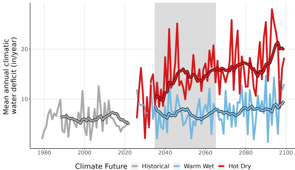
Figure 9. This line graph compares observed climatic water deficit at WIHO (inches/year) (1979-2022) with projected climatic water deficit for the two climate futures over the period 2023-2099. The historical observation data is shown in gray, the Warm Wet climate future in blue, and the Hot Dry climate future in red. The smooth line running through each projection is the 10-year running average for historical observations and future projections. Gray-shaded area represents the time period that was averaged (2035-2065) to summarize future projections for the year 2050.
