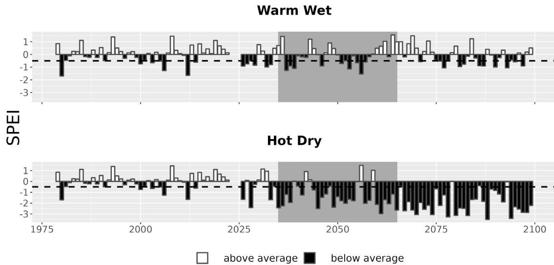
Figure 7. Drought metrics for WICR. Drought index (SPEI; units = standard deviations from historical) timeseries for each climate future. Below-average SPEI (black bars) indicates dry conditions. The dotted line (SPEI = -0.5) indicates drought conditions.
