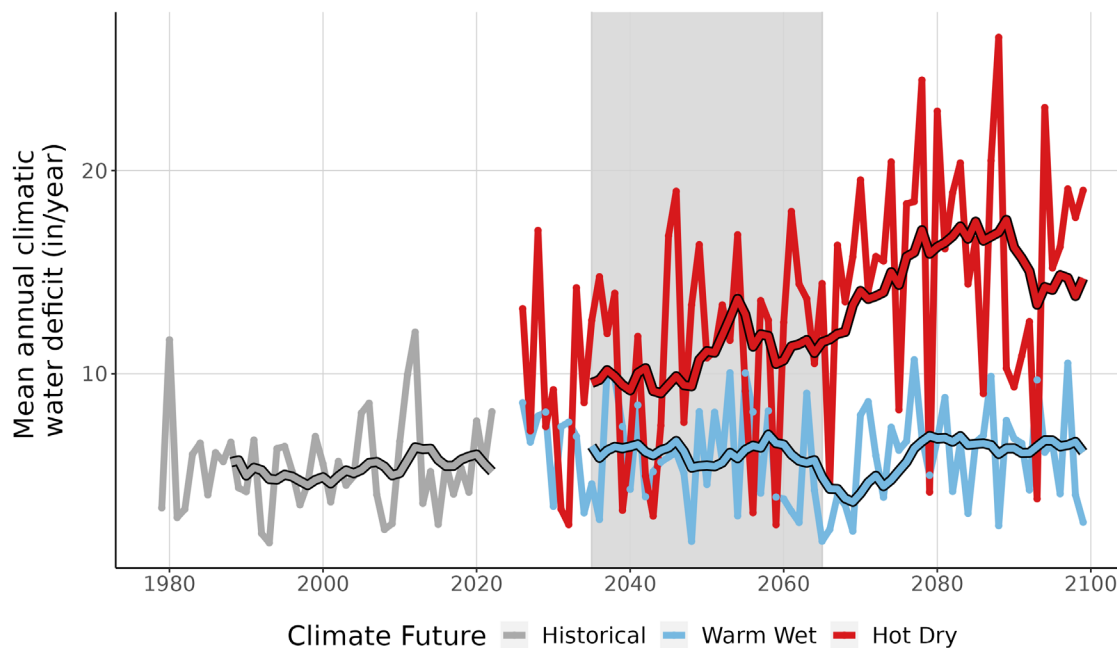
Figure 9. This line graph compares observed climatic water deficit at WICR (inches/year) (1979-2022) with projected climatic water deficit for the two climate futures over the period 2023-2099. The historical observation data is shown in gray, the Warm Wet climate future in blue, and the Hot Dry climate future in red. The smooth line running through each projection is the 10-year running average for historical observations and future projections. Gray-shaded area represents the time period that was averaged (2035-2065) to summarize future projections for the year 2050.
