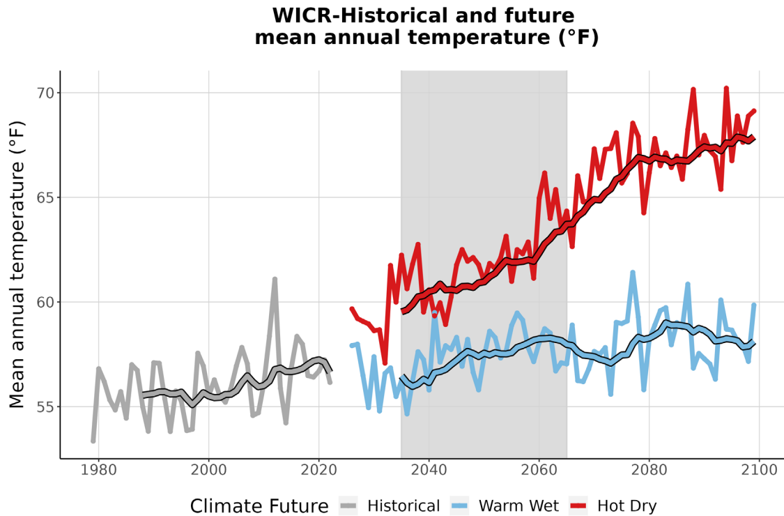
Figure 3. This graph compares observed average annual temperature at WICR (°F) (1979-2022) with projected average annual temperature for the two climate futures over the period 2023-2099. The historically observed data
