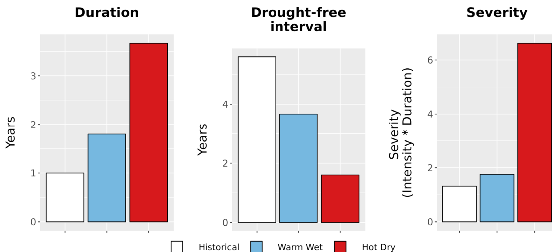
Figure 8. Drought metrics for WICR. (Left) Average drought duration (years) historically (1979-2012) and under each climate future. (Middle) Average drought return interval (years), indicating the expected amount of time between periods of drought, historically and under each climate future. (Right) Average drought severity, a measure of drought intensity multiplied by duration, historically and under each climate future.
