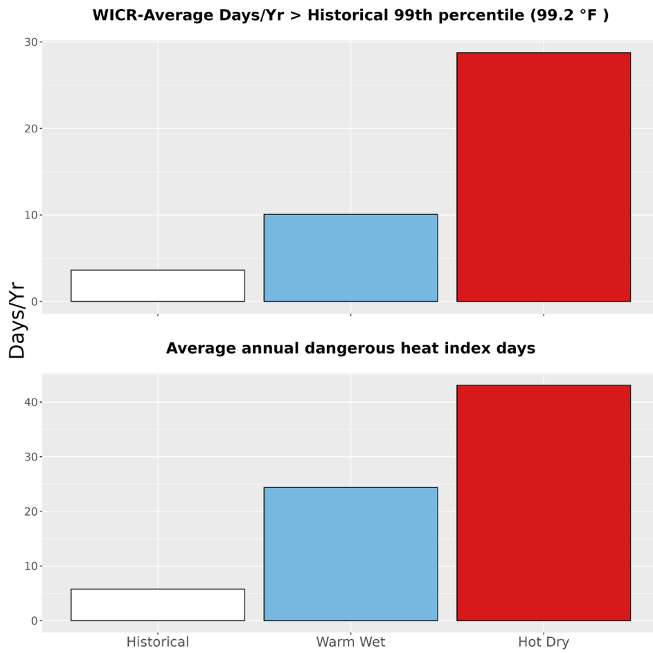
Figure 5. The upper bar graph represents the average number of days annually with temperatures greater than the historical 99th percentile (99.2 °F) historically (1979-2012) and for the two climate futures (2050). The bottom bar graph represents the average annual number of dangerous heat index days historically and for the two climate futures. Dangerous heat index days are days that exceed 105 °F.
