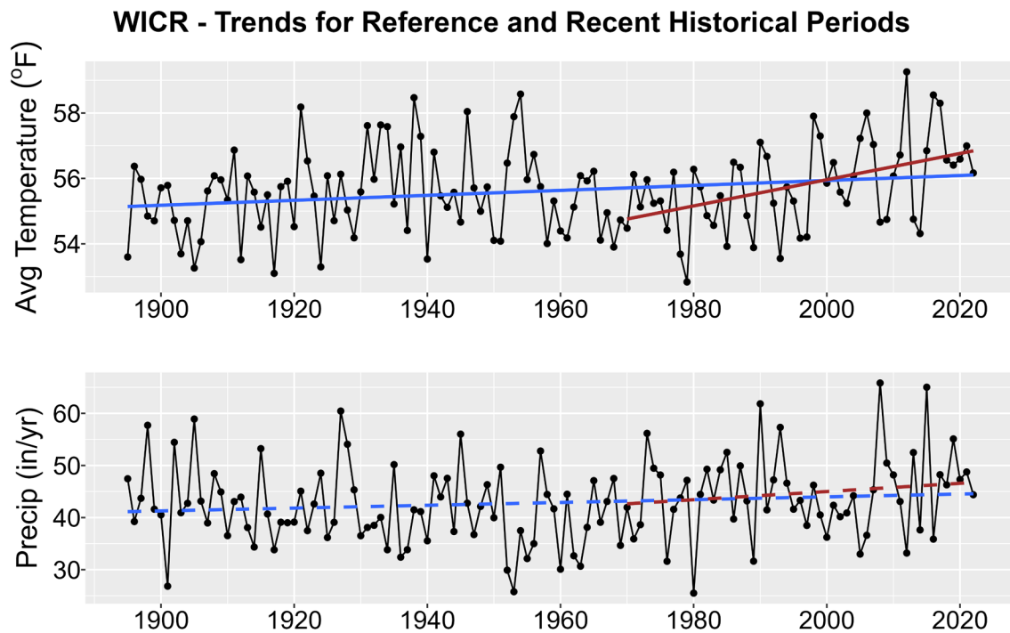
Figure 1. Historical trends in annual average temperature (upper plot) and annual total precipitation (lower plot) for WICR from 1895-2022. Black points show yearly values while blue lines are linear regressions for the entire period record and red lines for 1970-2022 trends. Solid lines are significant trends (i.e., p < 0.05 ); dashed lines are not statistically significant.
