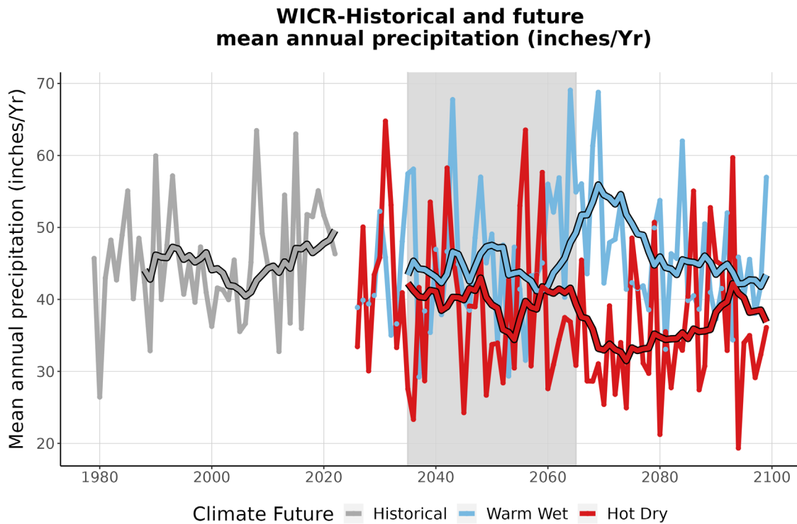
Figure 4. This graph compares observed average annual precipitation at WICR (inches/year) (1979-2022) with projected average annual precipitation for the two climate futures over the period 2023-2099. The historically observed data is shown in gray, the Warm Wet climate future in blue, and the Hot Dry climate future in red. The smooth line running through each projection is the 10-year running average for historical observations and future projections. The gray-shaded area represents the time period that was averaged (2035-2065) to summarize future projections for the year 2050 (Appendix 1).
