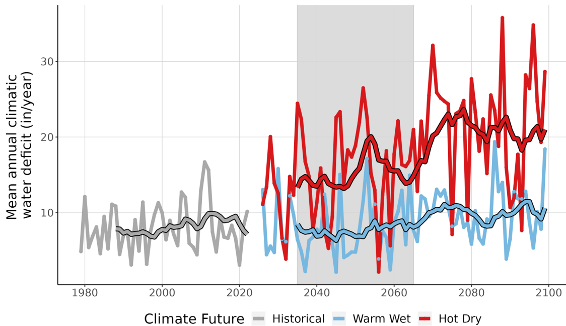
Figure 9. This line graph compares observed climatic water deficit at WICL (inches/year) (1979-2022) with projected climatic water deficit for the two climate futures over the period 2023-2099. The historical observation data is shown in gray, the Warm Wet climate future in blue, and the Hot Dry climate future in red. The smooth line running through each projection is the 10-year running average for historical observations and future projections. Gray-shaded area represents the time period that was averaged (2035-2065) to summarize future projections for the year 2050.
