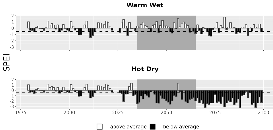
Figure 7. Drought metrics for WICL. Drought index (SPEI; units = standard deviations from historical) timeseries for each climate future. Below-average SPEI (black bars) indicates dry conditions. The dotted line (SPEI = -0.5) indicates drought conditions.
