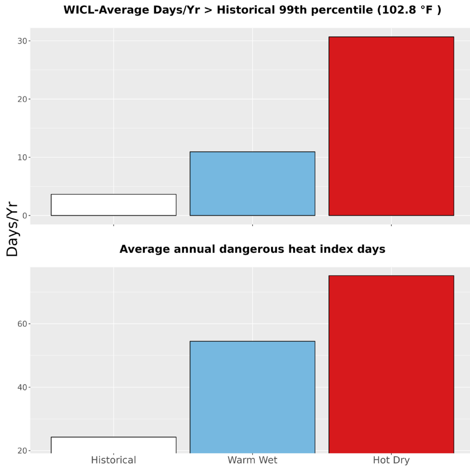
Figure 5. The upper bar graph represents the average number of days annually with temperatures greater than the historical 99th percentile (102.8 °F) historically (1979-2012) and for the two climate futures (2050). The bottom bar graph represents the average annual number of dangerous heat index days historically and for the two climate futures. Dangerous heat index days are days that exceed 105 °F.
