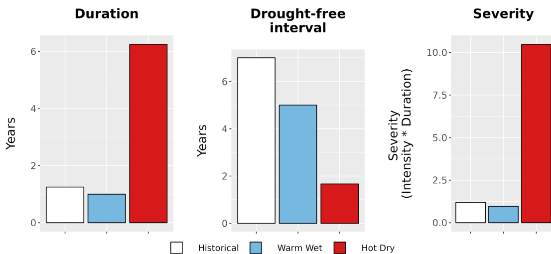
Figure 8. Drought metrics for WICL. (Left) Average drought duration (years) historically (1979-2012) and under each climate future. (Middle) Average drought return interval (years), indicating the expected amount of time between periods of drought, historically and under each climate future. (Right) Average drought severity, a measure of drought intensity multiplied by duration, historically and under each climate future.
