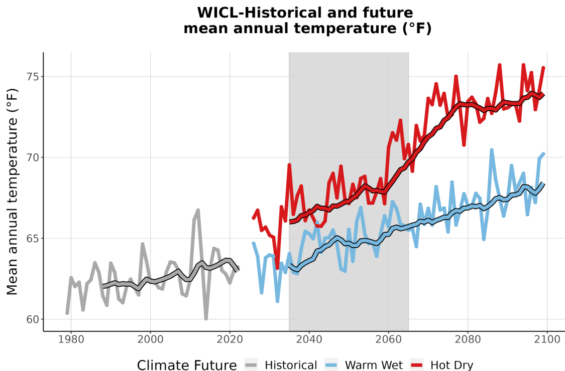
Figure 3. This graph compares observed average annual temperature at WICL (°F) (1979-2022) with projected average annual temperature for the two climate futures over the period 2023-2099. The historically observed data
