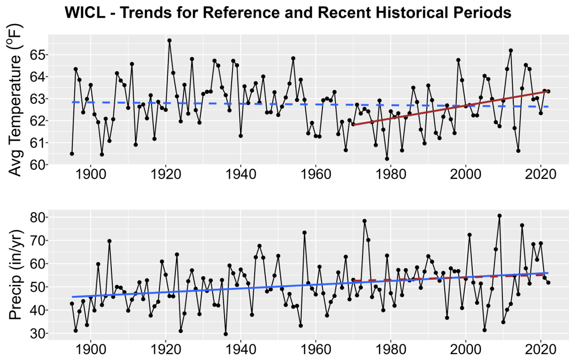
Figure 1. Historical trends in annual average temperature (upper plot) and annual total precipitation (lower plot) for WICL from 1895-2022. Black points show yearly values while blue lines are linear regressions for the entire period record and red lines for 1970-2022 trends. Solid lines are significant trends (i.e., p < 0.05 ); dashed lines are not statistically significant.
