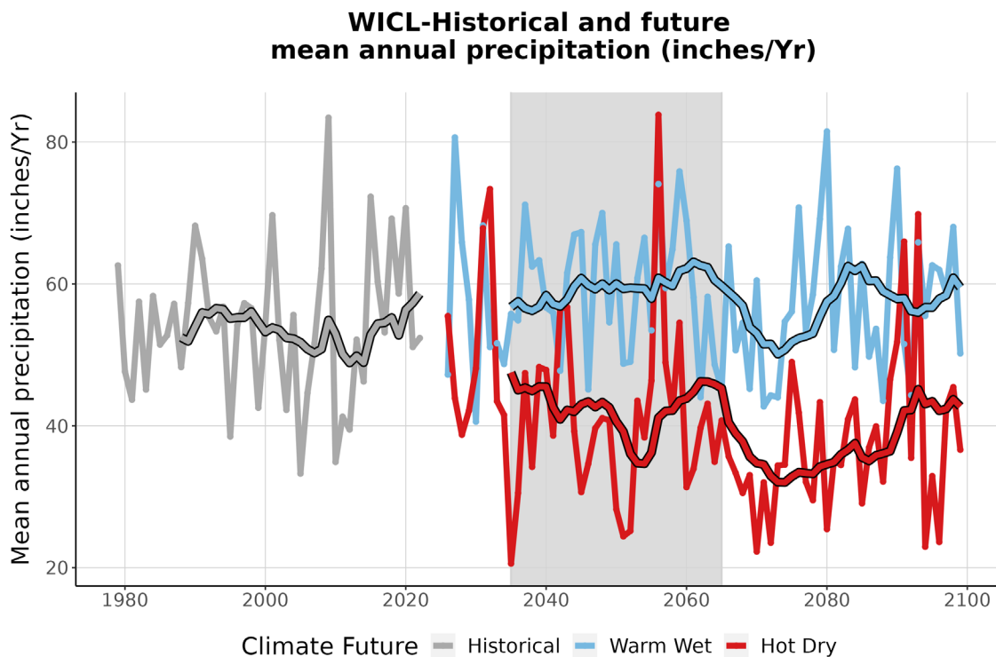
Figure 4. This graph compares observed average annual precipitation at WICL (inches/year) (1979-2022) with projected average annual precipitation for the two climate futures over the period 2023-2099. The historically observed data is shown in gray, the Warm Wet climate future in blue, and the Hot Dry climate future in red. The smooth line running through each projection is the 10-year running average for historical observations and future projections. The gray-shaded area represents the time period that was averaged (2035-2065) to summarize future projections for the year 2050 (Appendix 1).
