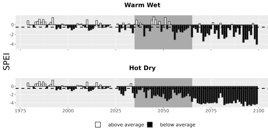
Figure 7. Drought metrics for WHSA. Drought index (SPEI; units = standard deviations from historical) timeseries for each climate future. Below-average SPEI (black bars) indicates dry conditions. The dotted line (SPEI = -0.5) indicates drought conditions.
