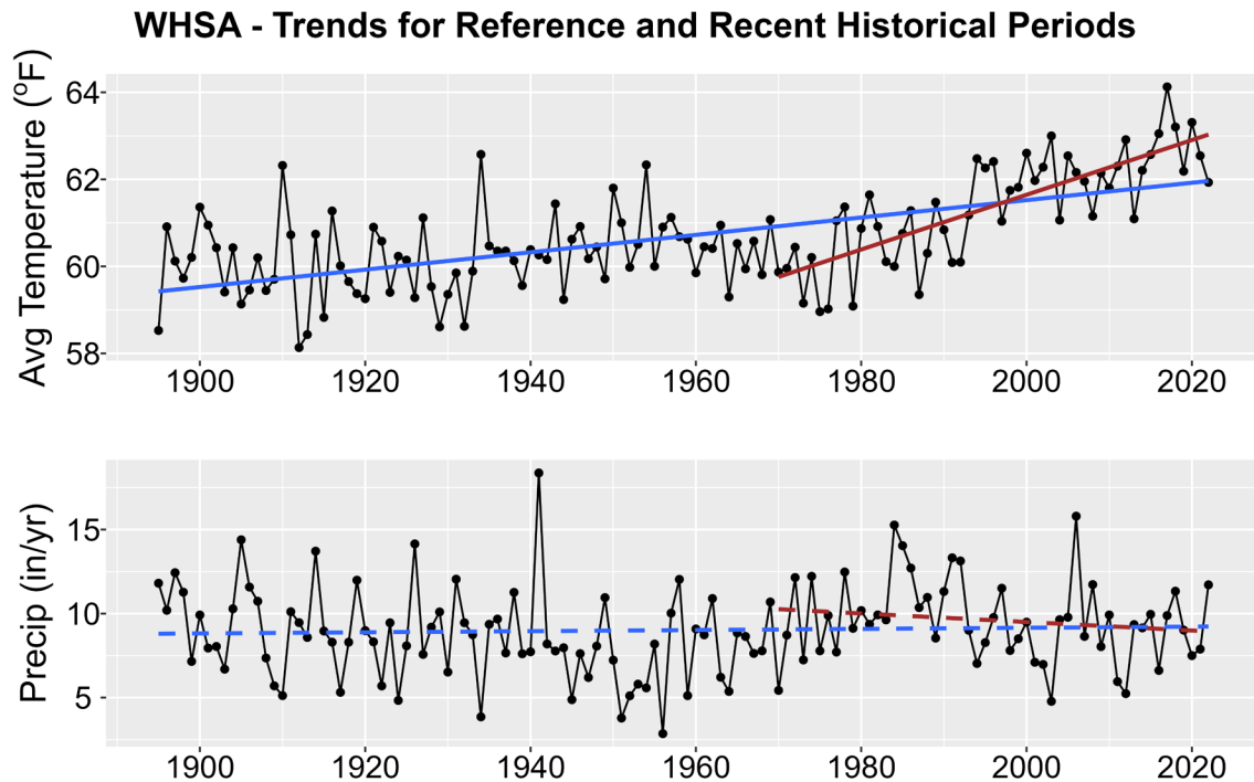
Figure 1. Historical trends in annual average temperature (upper plot) and annual total precipitation (lower plot) for WHSA from 1895-2022. Black points show yearly values while blue lines are linear regressions for the entire period record and red lines for 1970-2022 trends. Solid lines are significant trends (i.e., p < 0.05 ); dashed lines are not statistically significant.
