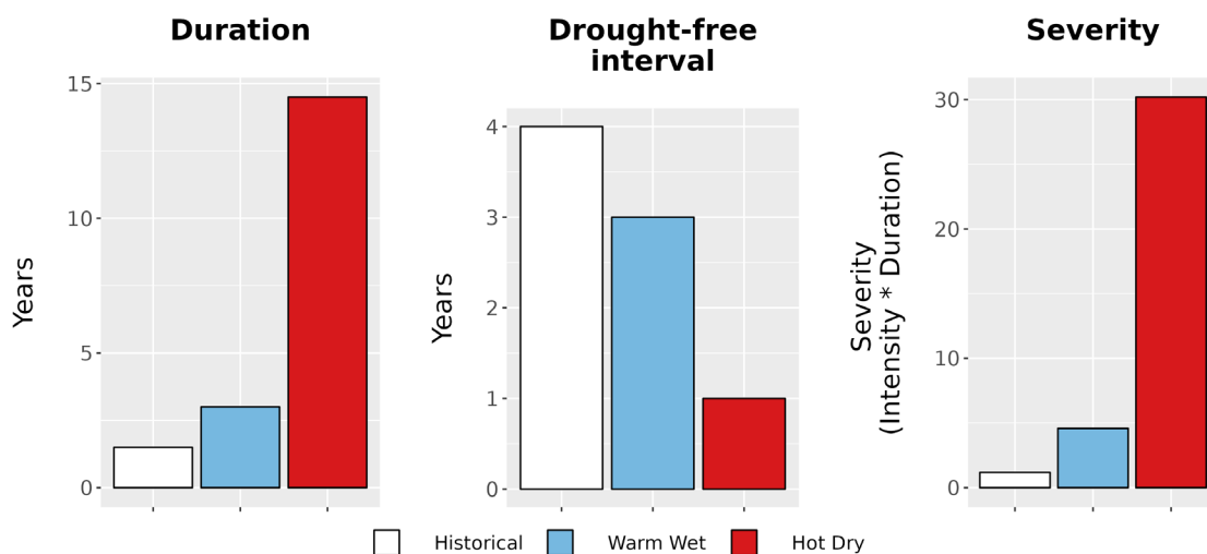
Figure 8. Drought metrics for WWSA. (Left) Average drought duration (years) historically (1979-2012) and under each climate future. (Middle) Average drought return interval (years), indicating the expected amount of time between periods of drought, historically and under each climate future. (Right) Average drought severity, a measure of drought intensity multiplied by duration, historically and under each climate future.
