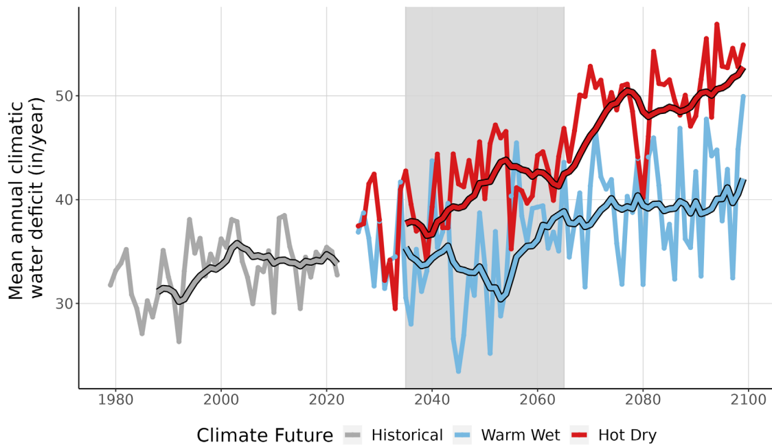
Figure 9. This line graph compares observed climatic water deficit at WHSA (inches/year) (1979-2022) with projected climatic water deficit for the two climate futures over the period 2023-2099. The historical observation data is shown in gray, the Warm Wet climate future in blue, and the Hot Dry climate future in red. The smooth line running through each projection is the 10-year running average for historical observations and future projections. Gray-shaded area represents the time period that was averaged (2035-2065) to summarize future projections for the year 2050.
