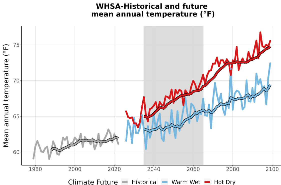
Figure 3. This graph compares observed average annual temperature at WHSA (°F) (1979-2022) with projected average annual temperature for the two climate futures over the period 2023-2099. The historically observed data
