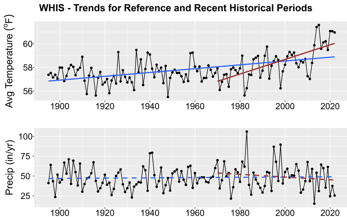
Figure 1. Historical trends in annual average temperature (upper plot) and annual total precipitation (lower plot) for WHIS from 1895-2022. Black points show yearly values while blue lines are linear regressions for the entire period record and red lines for 1970-2022 trends. Solid lines are significant trends (i.e., p < 0.05 ); dashed lines are not statistically significant.
