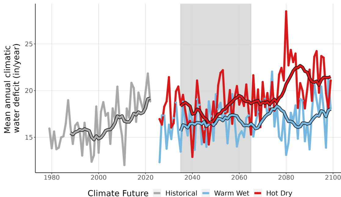
Figure 9. This line graph compares observed climatic water deficit at WHIS (inches/year) (1979-2022) with projected climatic water deficit for the two climate futures over the period 2023-2099. The historical observation data is shown in gray, the Warm Wet climate future in blue, and the Hot Dry climate future in red. The smooth line running through each projection is the 10-year running average for historical observations and future projections. Gray-shaded area represents the time period that was averaged (2035-2065) to summarize future projections for the year 2050.
