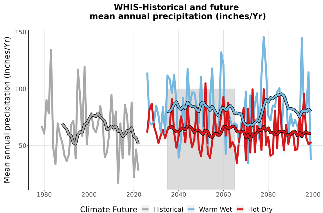
Figure 4. This graph compares observed average annual precipitation at WHIS (inches/year) (1979-2022) with projected average annual precipitation for the two climate futures over the period 2023-2099. The historically observed data is shown in gray, the Warm Wet climate future in blue, and the Hot Dry climate future in red. The smooth line running through each projection is the 10-year running average for historical observations and future projections. The gray-shaded area represents the time period that was averaged (2035-2065) to summarize future projections for the year 2050 (Appendix 1).
