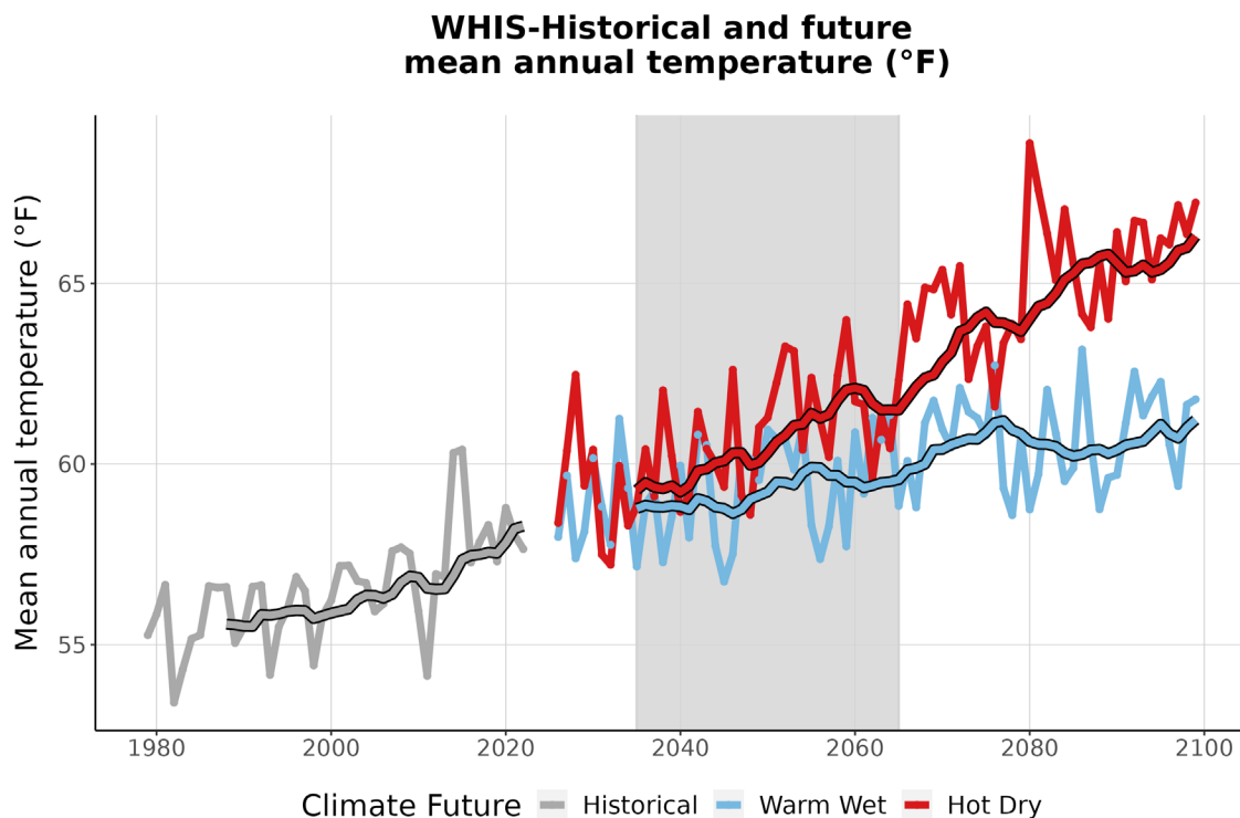
Figure 3. This graph compares observed average annual temperature at WHIS (°F) (1979-2022) with projected average annual temperature for the two climate futures over the period 2023-2099. The historically observed data
