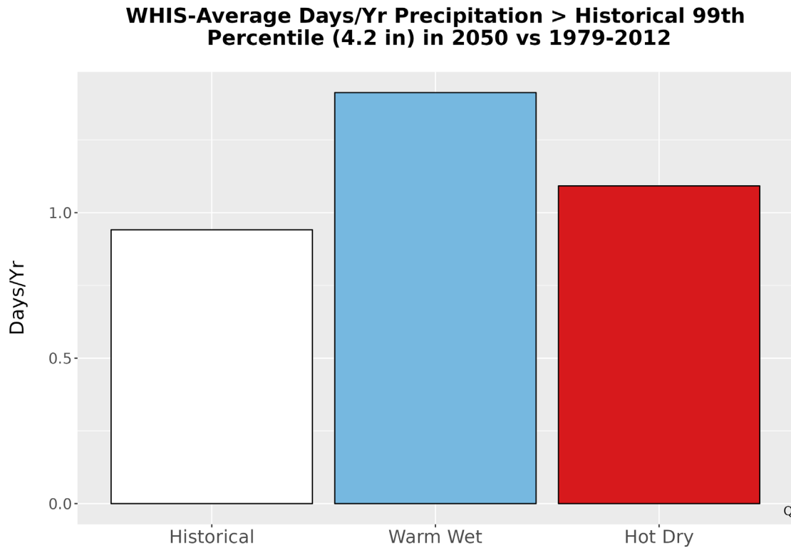
Figure 6. Average number of days annually with precipitation exceeding the 99th percentile (4.2 in.) of precipitation from the historical period 1979-2012 and for each climate future.
