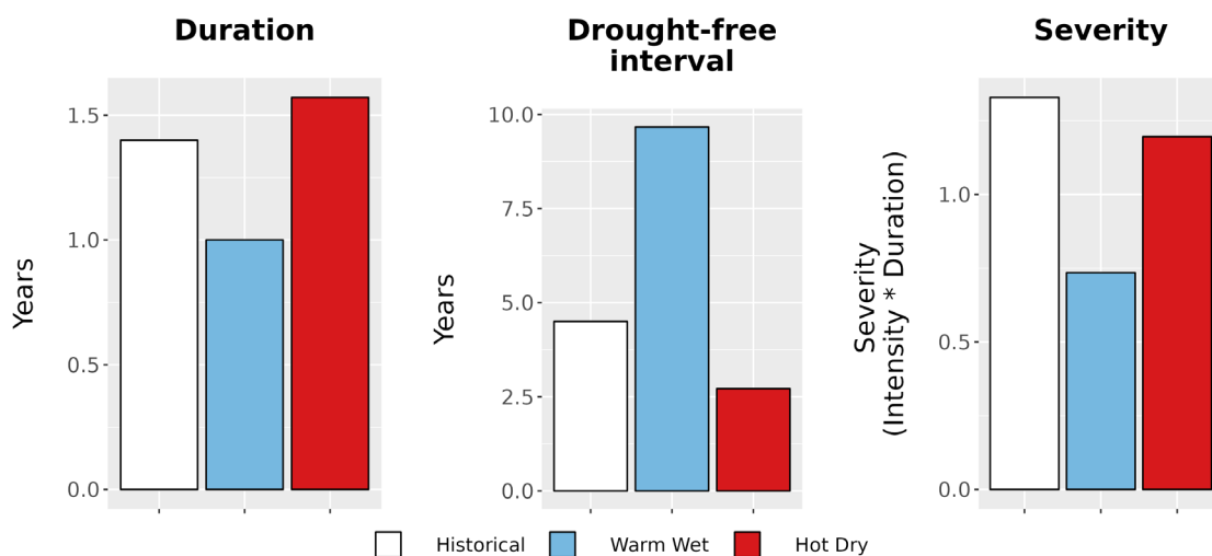
Figure 8. Drought metrics for WHIS. (Left) Average drought duration (years) historically (1979-2012) and under each climate future. (Middle) Average drought return interval (years), indicating the expected amount of time between periods of drought, historically and under each climate future. (Right) Average drought severity, a measure of drought intensity multiplied by duration, historically and under each climate future.
