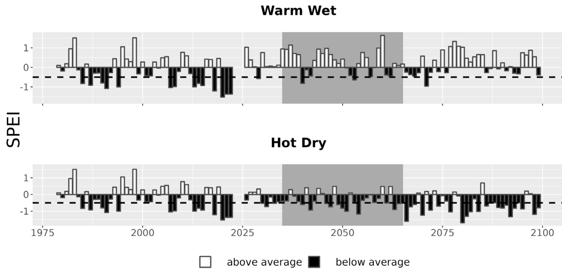
Figure 7. Drought metrics for WHIS. Drought index (SPEI; units = standard deviations from historical) timeseries for each climate future. Below-average SPEI (black bars) indicates dry conditions. The dotted line (SPEI = -0.5) indicates drought conditions.
