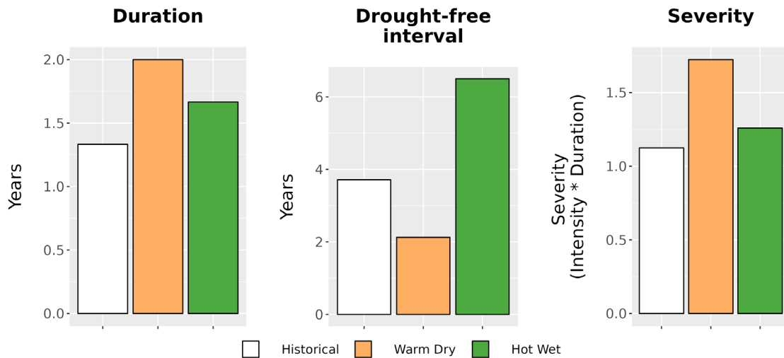
Figure 8. Drought metrics for WEFA. (Left) Average drought duration (years) historically (1979-2012) and under each climate future. (Middle) Average drought return interval (years), indicating the expected amount of time between periods of drought, historically and under each climate future. (Right) Average drought severity, a measure of drought intensity multiplied by duration, historically and under each climate future.
