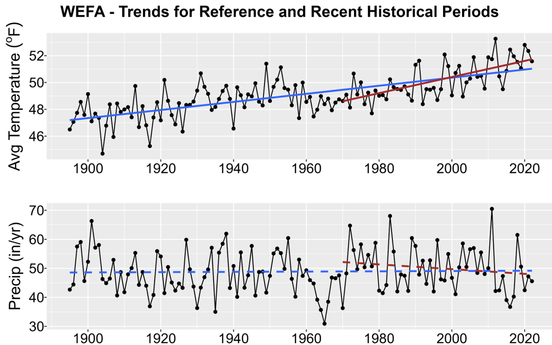
Figure 1. Historical trends in annual average temperature (upper plot) and annual total precipitation (lower plot) for WEFA from 1895-2022. Black points show yearly values while blue lines are linear regressions for the entire period record and red lines for 1970-2022 trends. Solid lines are significant trends (i.e., p < 0.05 ); dashed lines are not statistically significant.
