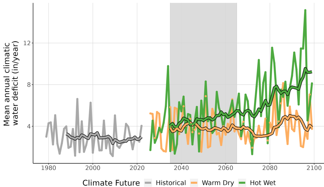
Figure 9. This line graph compares observed climatic water deficit at WEFA (inches/year) (1979-2022) with projected climatic water deficit for the two climate futures over the period 2023-2099. The historical observation data is shown in gray, the Warm Dry climate future in orange, and the Hot Wet climate future in green. The smooth line running through each projection is the 10-year running average for historical observations and future projections. Gray-shaded area represents the time period that was averaged (2035-2065) to summarize future projections for the year 2050.
