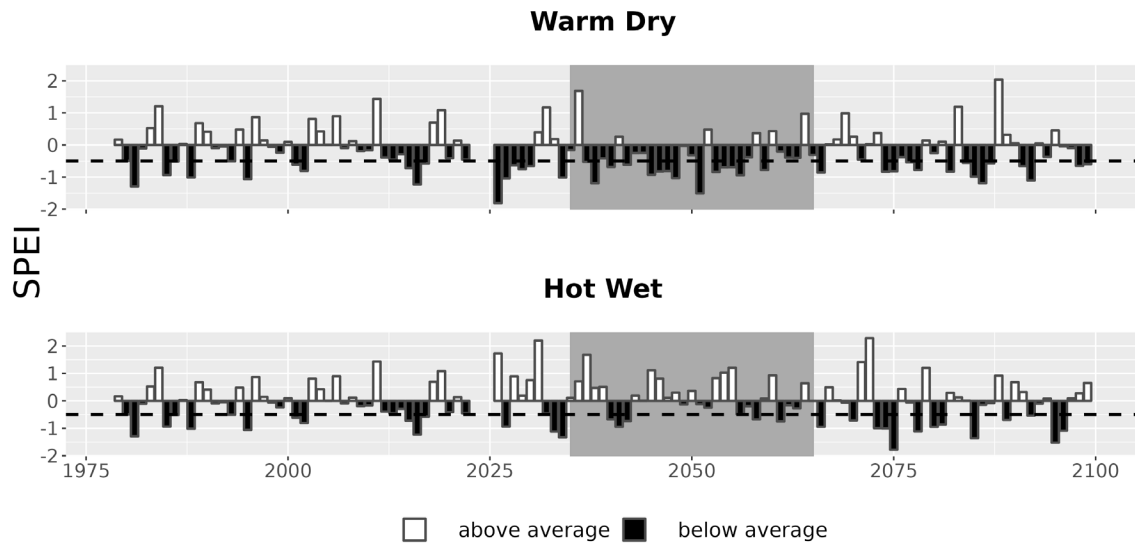
Figure 7. Drought metrics for WEFA. Drought index (SPEI; units = standard deviations from historical) timeseries for each climate future. Below-average SPEI (black bars) indicates dry conditions. The dotted line (SPEI = -0.5) indicates drought conditions.
