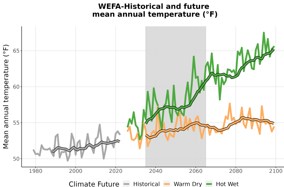
Figure 3. This graph compares observed average annual temperature at WEFA (°F) (1979-2022) with projected average annual temperature for the two climate futures over the period 2023-2099. The historically observed data
