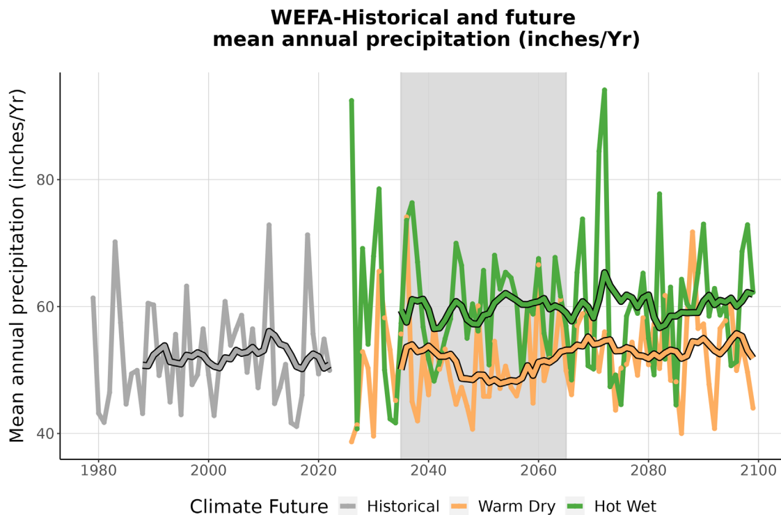
Figure 4. This graph compares observed average annual precipitation at WEFA (inches/year) (1979-2022) with projected average annual precipitation for the two climate futures over the period 2023-2099. The historically observed data is shown in gray, the Warm Dry climate future in orange, and the Hot Wet climate future in green. The smooth line running through each projection is the 10-year running average for historical observations and future projections. The gray-shaded area represents the time period that was averaged (2035-2065) to summarize future projections for the year 2050 (Appendix 1).
