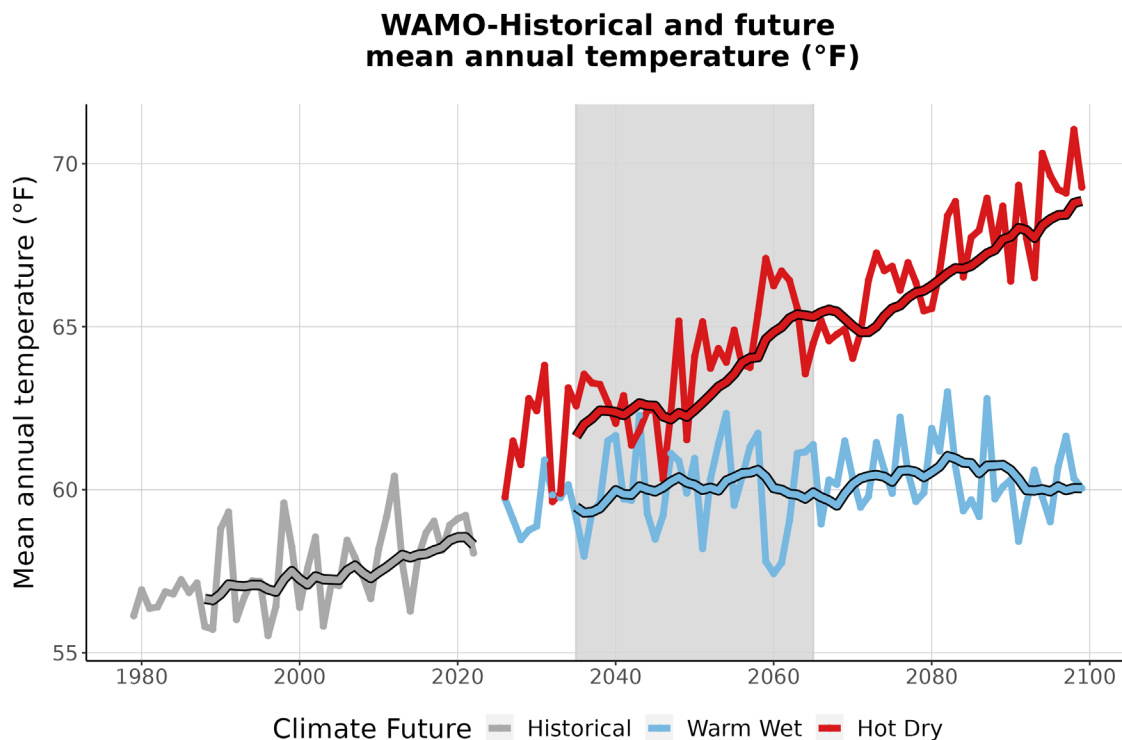
Figure 3. This graph compares observed average annual temperature at WAMO (°F) (1979-2022) with projected average annual temperature for the two climate futures over the period 2023-2099. The historically observed data
