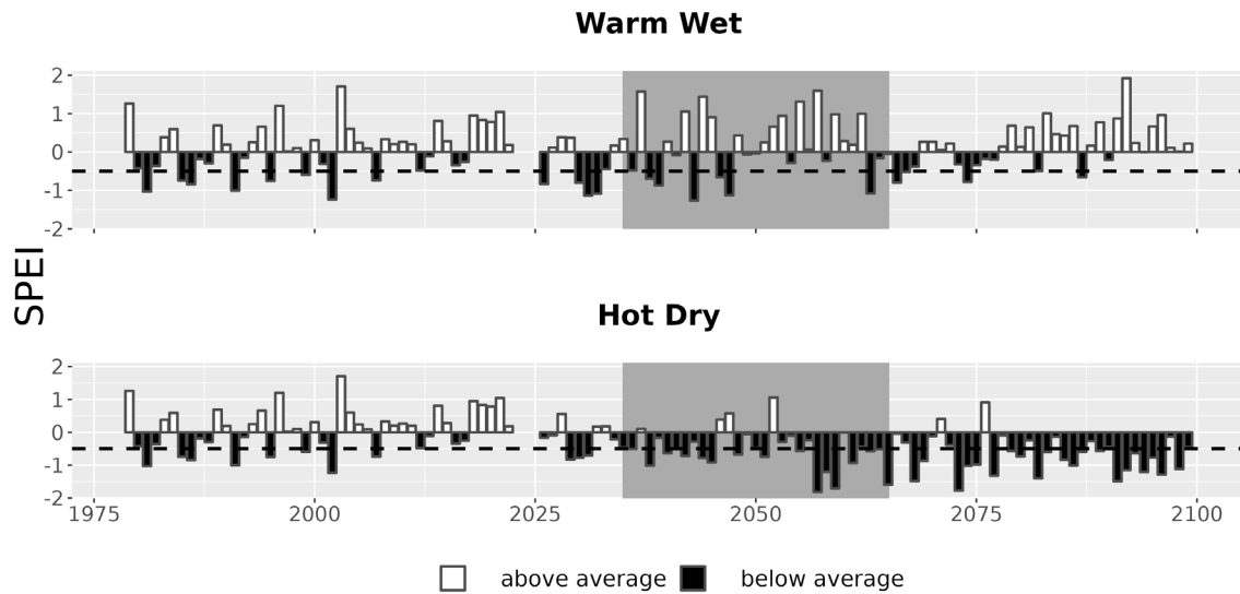
Figure 7. Drought metrics for WAMO. Drought index (SPEI; units = standard deviations from historical) timeseries for each climate future. Below-average SPEI (black bars) indicates dry conditions. The dotted line (SPEI = -0.5) indicates drought conditions.
