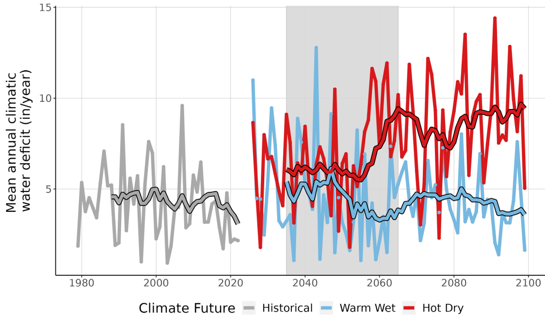
Figure 9. This line graph compares observed climatic water deficit at WAMO (inches/year) (1979-2022) with projected climatic water deficit for the two climate futures over the period 2023-2099. The historical observation data is shown in gray, the Warm Wet climate future in blue, and the Hot Dry climate future in red. The smooth line running through each projection is the 10-year running average for historical observations and future projections. Gray-shaded area represents the time period that was averaged (2035-2065) to summarize future projections for the year 2050.
