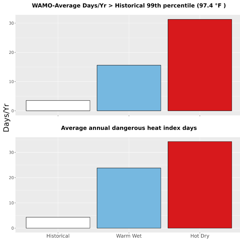
Figure 5. The upper bar graph represents the average number of days annually with temperatures greater than the historical 99th percentile (97.4 °F) historically (1979-2012) and for the two climate futures (2050). The bottom bar graph represents the average annual number of dangerous heat index days historically and for the two climate futures. Dangerous heat index days are days that exceed 105 °F.
