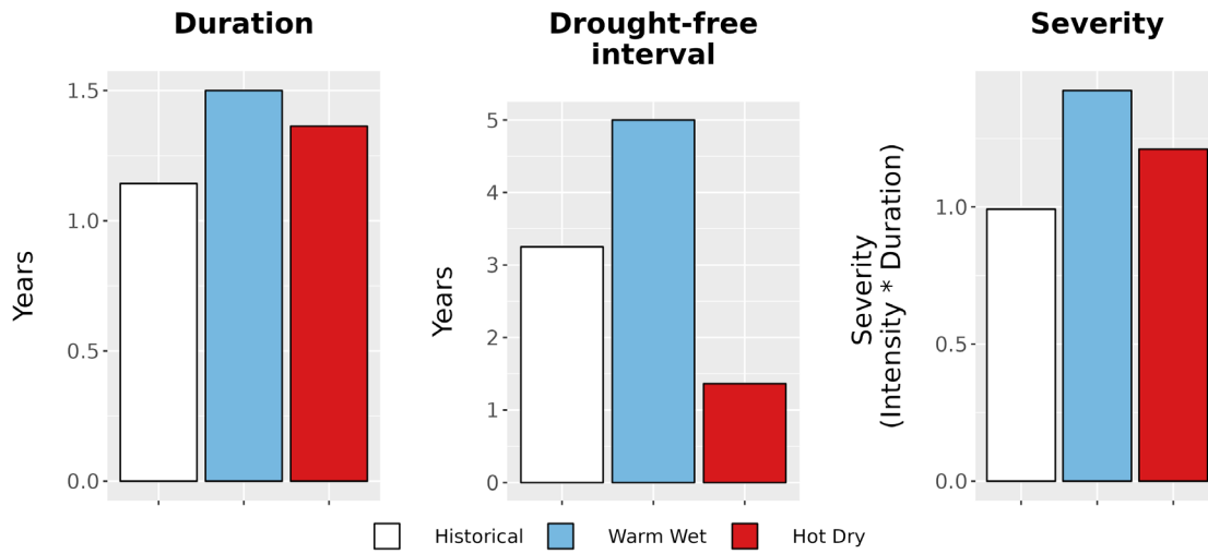
Figure 8. Drought metrics for WAMO. (Left) Average drought duration (years) historically (1979-2012) and under each climate future. (Middle) Average drought return interval (years), indicating the expected amount of time between periods of drought, historically and under each climate future. (Right) Average drought severity, a measure of drought intensity multiplied by duration, historically and under each climate future.
