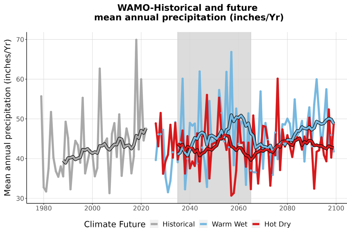
Figure 4. This graph compares observed average annual precipitation at WAMO (inches/year) (1979-2022) with projected average annual precipitation for the two climate futures over the period 2023-2099. The historically observed data is shown in gray, the Warm Wet climate future in blue, and the Hot Dry climate future in red. The smooth line running through each projection is the 10-year running average for historical observations and future projections. The gray-shaded area represents the time period that was averaged (2035-2065) to summarize future projections for the year 2050 (Appendix 1).
