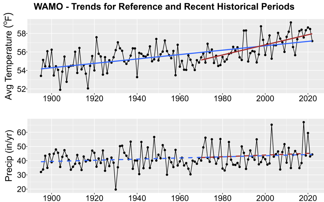
Figure 1. Historical trends in annual average temperature (upper plot) and annual total precipitation (lower plot) for WAMO from 1895-2022. Black points show yearly values while blue lines are linear regressions for the entire period record and red lines for 1970-2022 trends. Solid lines are significant trends (i.e., p < 0.05 ); dashed lines are not statistically significant.
