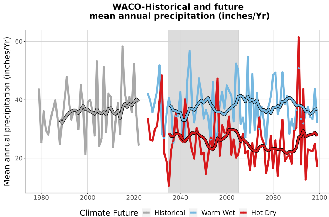
Figure 4. This graph compares observed average annual precipitation at WACO (inches/year) (1979-2022) with projected average annual precipitation for the two climate futures over the period 2023-2099. The historically observed data is shown in gray, the Warm Wet climate future in blue, and the Hot Dry climate future in red. The smooth line running through each projection is the 10-year running average for historical observations and future projections. The gray-shaded area represents the time period that was averaged (2035-2065) to summarize future projections for the year 2050 (Appendix 1).
