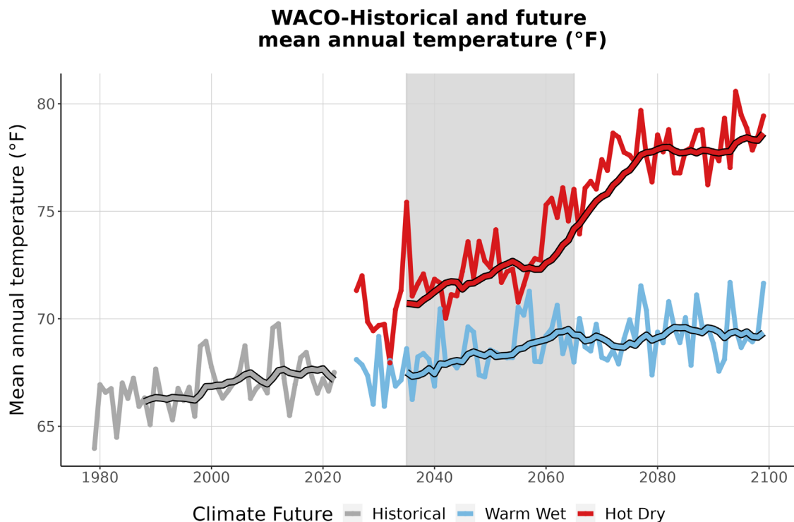
Figure 3. This graph compares observed average annual temperature at WACO (°F) (1979-2022) with projected average annual temperature for the two climate futures over the period 2023-2099. The historically observed data
