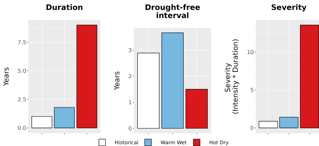
Figure 8. Drought metrics for WACO. (Left) Average drought duration (years) historically (1979-2012) and under each climate future. (Middle) Average drought return interval (years), indicating the expected amount of time between periods of drought, historically and under each climate future. (Right) Average drought severity, a measure of drought intensity multiplied by duration, historically and under each climate future.
