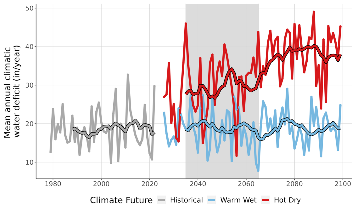
Figure 9. This line graph compares observed climatic water deficit at WACO (inches/year) (1979-2022) with projected climatic water deficit for the two climate futures over the period 2023-2099. The historical observation data is shown in gray, the Warm Wet climate future in blue, and the Hot Dry climate future in red. The smooth line running through each projection is the 10-year running average for historical observations and future projections. Gray-shaded area represents the time period that was averaged (2035-2065) to summarize future projections for the year 2050.
