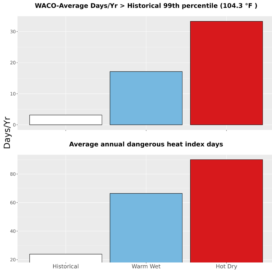
Figure 5. The upper bar graph represents the average number of days annually with temperatures greater than the historical 99th percentile (104.3 °F) historically (1979-2012) and for the two climate futures (2050). The bottom bar graph represents the average annual number of dangerous heat index days historically and for the two climate futures. Dangerous heat index days are days that exceed 105 °F.
