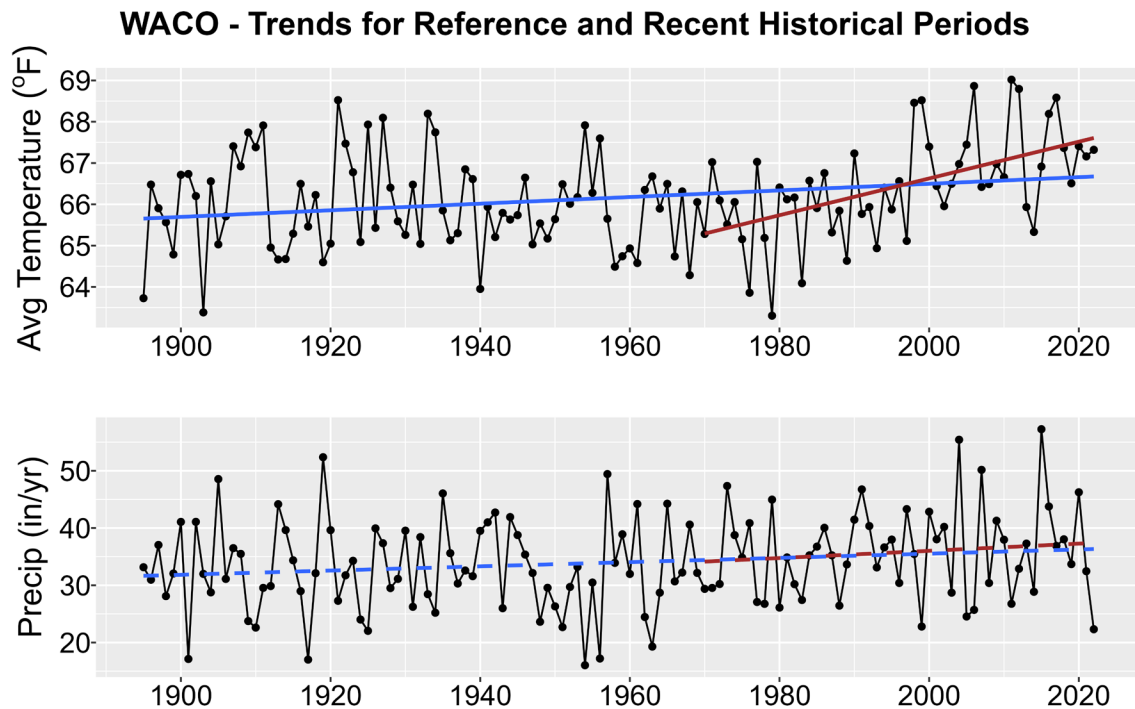
Figure 1. Historical trends in annual average temperature (upper plot) and annual total precipitation (lower plot) for WACO from 1895-2022. Black points show yearly values while blue lines are linear regressions for the entire period record and red lines for 1970-2022 trends. Solid lines are significant trends (i.e., p < 0.05 ); dashed lines are not statistically significant.
