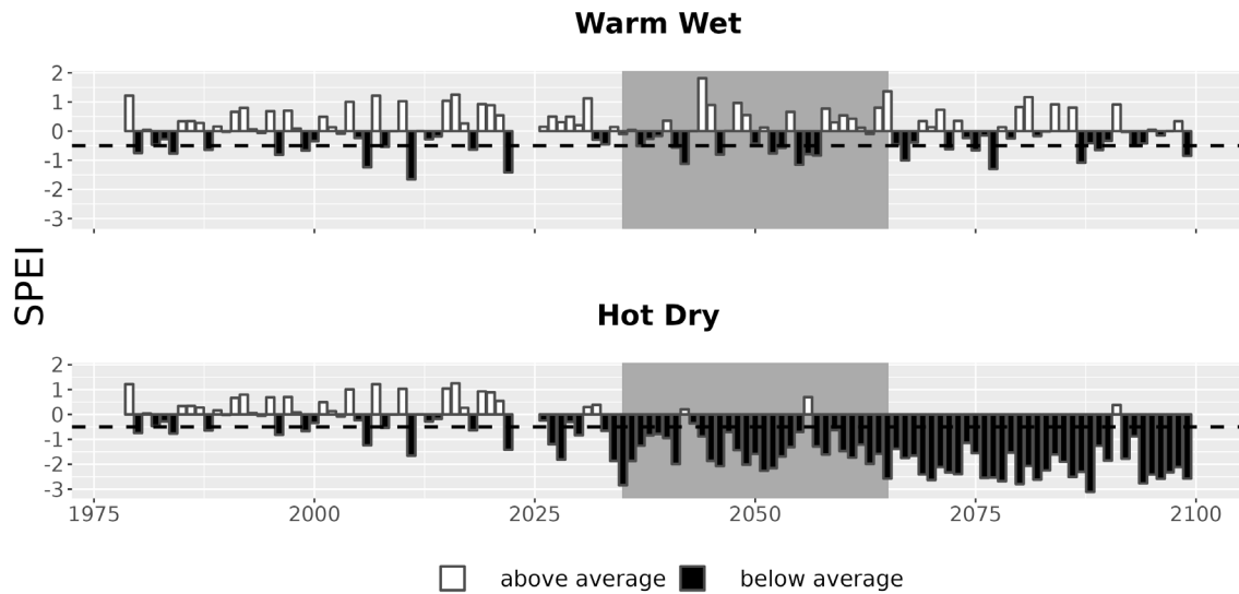
Figure 7. Drought metrics for WACO. Drought index (SPEI; units = standard deviations from historical) timeseries for each climate future. Below-average SPEI (black bars) indicates dry conditions. The dotted line (SPEI = -0.5) indicates drought conditions.
