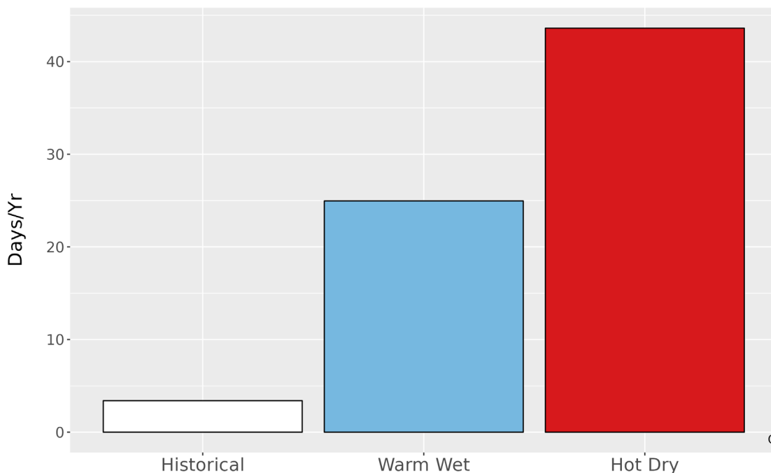
Figure 5. Metrics of extreme temperature at WACA. The bar graph represents the average number of days annually with temperatures greater than the historical 99th percentile (90.6 °F) historically (1979-2012) and for the two climate futures (2050).
