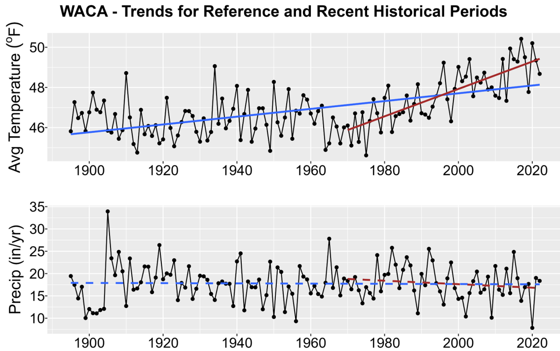
Figure 1. Historical trends in annual average temperature (upper plot) and annual total precipitation (lower plot) for WACA from 1895-2022. Black points show yearly values while blue lines are linear regressions for the entire period record and red lines for 1970-2022 trends. Solid lines are significant trends (i.e., p < 0.05 ); dashed lines are not statistically significant.
