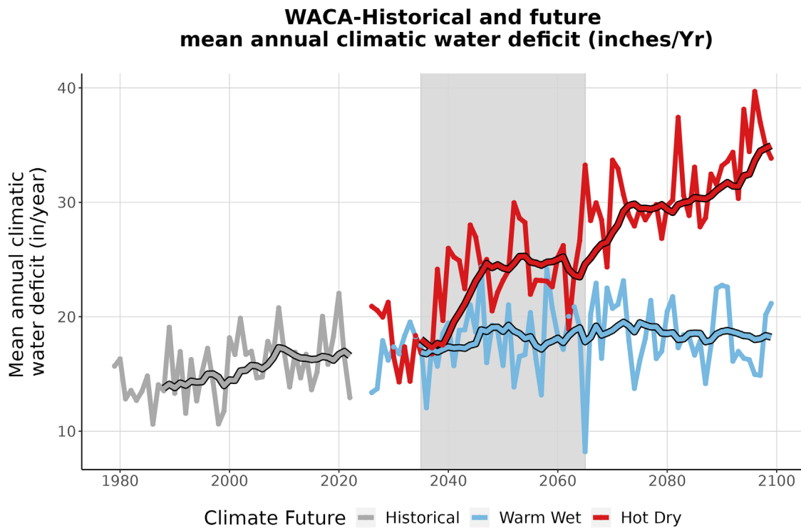
Figure 9. This line graph compares observed climatic water deficit at WACA (inches/year) (1979-2022) with projected climatic water deficit for the two climate futures over the period 2023-2099. The historical observation data is shown in gray, the Warm Wet climate future in blue, and the Hot Dry climate future in red. The smooth line running through each projection is the 10-year running average for historical observations and future projections. Gray-shaded area represents the time period that was averaged (2035-2065) to summarize future projections for the year 2050.
