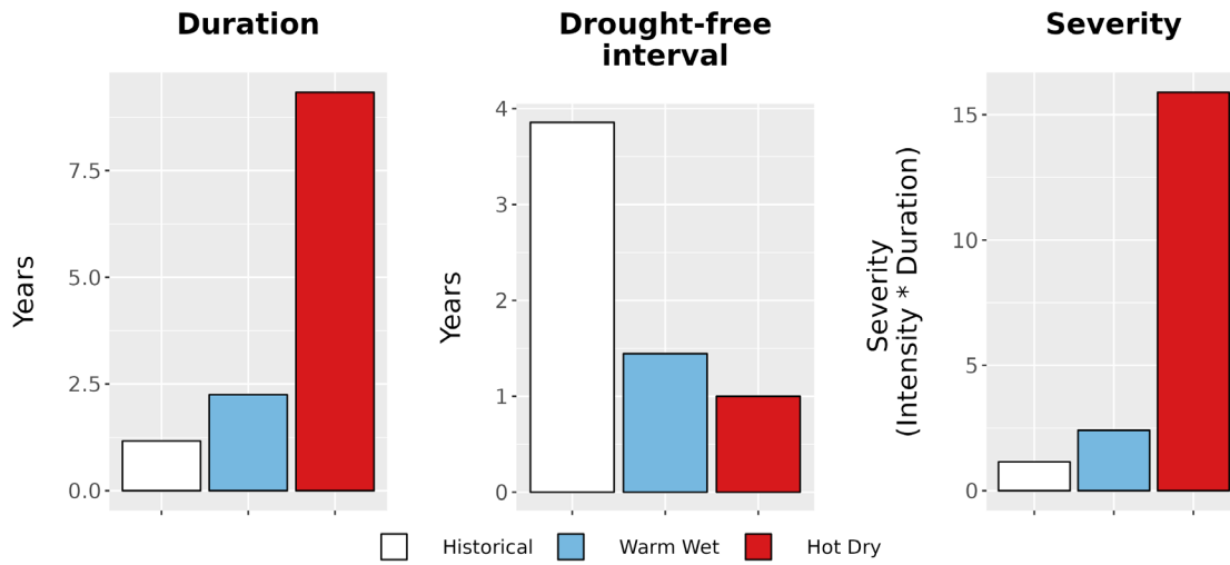
Figure 8. Drought metrics for WACA. (Left) Average drought duration (years) historically (1979-2012) and under each climate future. (Middle) Average drought return interval (years), indicating the expected amount of time between periods of drought, historically and under each climate future. (Right) Average drought severity, a measure of drought intensity multiplied by duration, historically and under each climate future.
