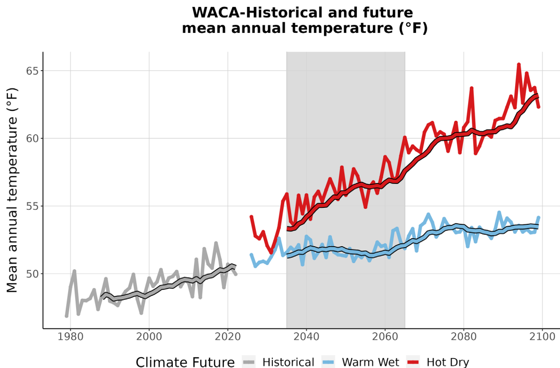
Figure 3. This graph compares observed average annual temperature at WACA (°F) (1979-2022) with projected average annual temperature for the two climate futures over the period 2023-2099. The historically observed data
