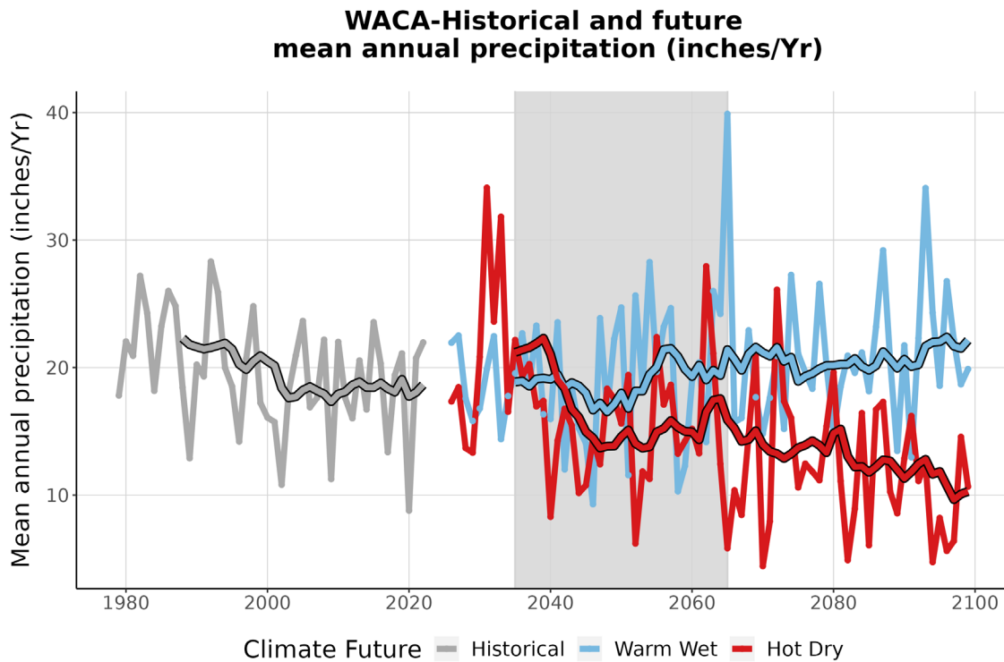
Figure 4. This graph compares observed average annual precipitation at WACA (inches/year) (1979-2022) with projected average annual precipitation for the two climate futures over the period 2023-2099. The historically observed data is shown in gray, the Warm Wet climate future in blue, and the Hot Dry climate future in red. The smooth line running through each projection is the 10-year running average for historical observations and future projections. The gray-shaded area represents the time period that was averaged (2035-2065) to summarize future projections for the year 2050 (Appendix 1).
