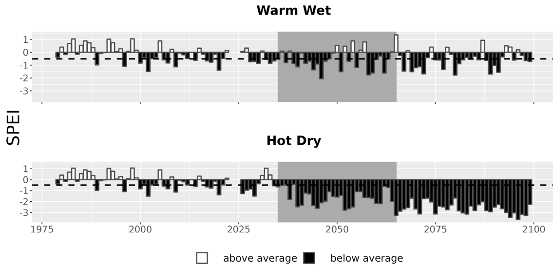
Figure 7. Drought metrics for WACA. Drought index (SPEI; units = standard deviations from historical) timeseries for each climate future. Below-average SPEI (black bars) indicates dry conditions. The dotted line (SPEI = -0.5) indicates drought conditions.
