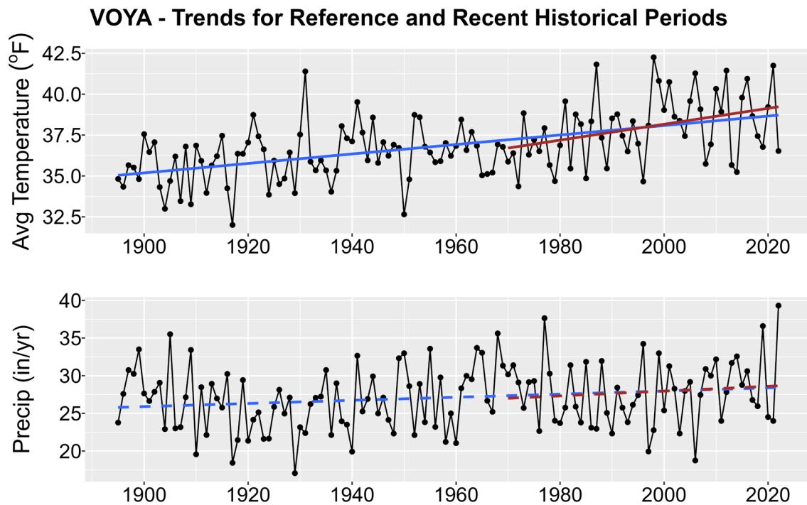
Figure 1. Historical trends in annual average temperature (upper plot) and annual total precipitation (lower plot) for VOYA from 1895-2022. Black points show yearly values while blue lines are linear regressions for the entire period record and red lines for 1970-2022 trends. Solid lines are significant trends (i.e., p < 0.05 ); dashed lines are not statistically significant.
