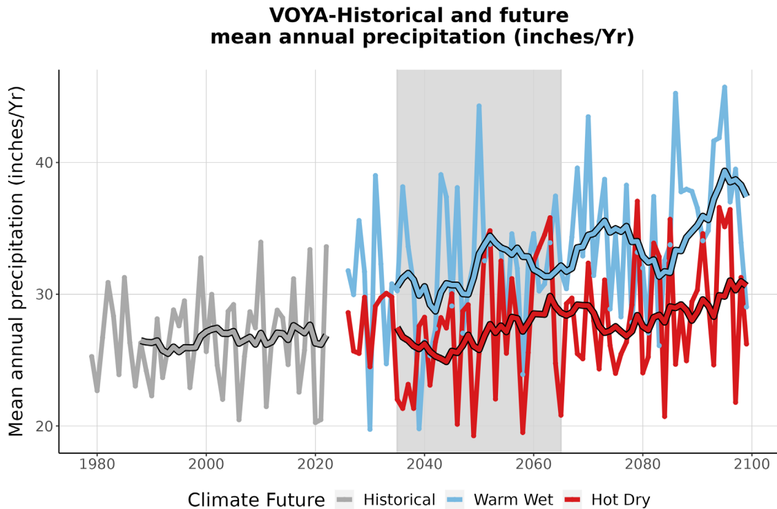
Figure 4. This graph compares observed average annual precipitation at VOYA (inches/year) (1979-2022) with projected average annual precipitation for the two climate futures over the period 2023-2099. The historically observed data is shown in gray, the Warm Wet climate future in blue, and the Hot Dry climate future in red. The smooth line running through each projection is the 10-year running average for historical observations and future projections. The gray-shaded area represents the time period that was averaged (2035-2065) to summarize future projections for the year 2050 (Appendix 1).
