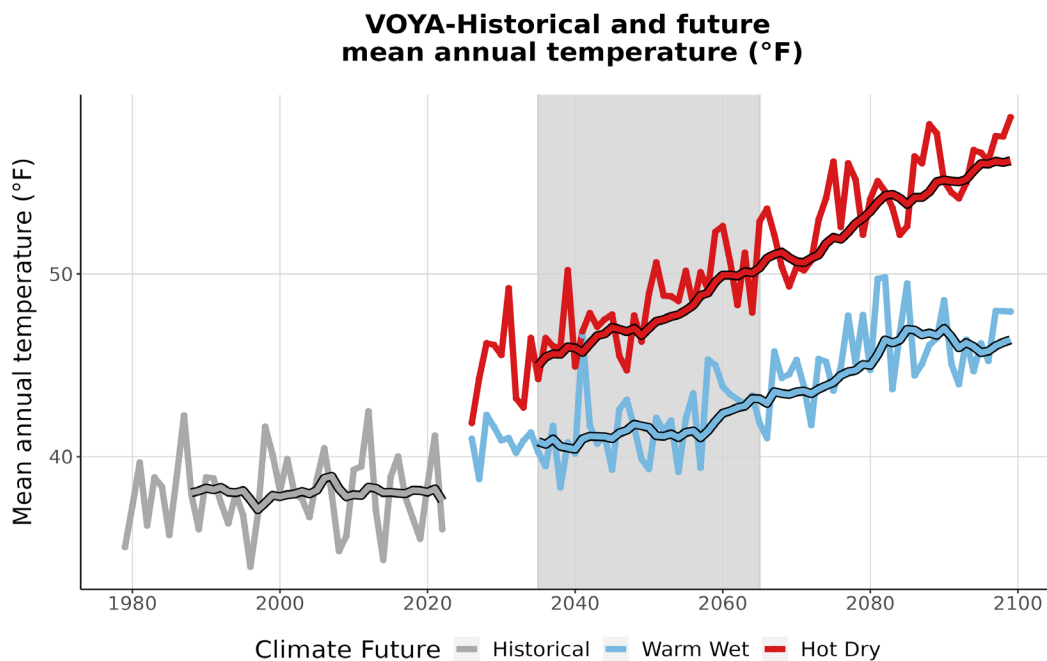
Figure 3. This graph compares observed average annual temperature at VOYA (°F) (1979-2022) with projected average annual temperature for the two climate futures over the period 2023-2099. The historically observed data is shown in gray, the Warm Wet climate future in blue, and the Hot Dry climate future in red. The smooth line running through each projection is the 10-year running average for historical observations and future projections. Gray-shaded area represents the time period that was averaged (2035-2065) to summarize future projections for the year 2050 (Appendix 1).
