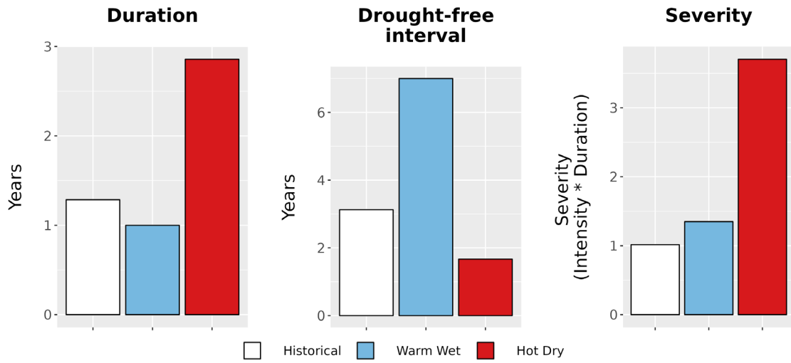
Figure 8. Drought metrics for VOYA. (Left) Average drought duration (years) historically (1979-2012) and under each climate future. (Middle) Average drought return interval (years), indicating the expected amount of time between periods of drought, historically and under each climate future. (Right) Average drought severity, a measure of drought intensity multiplied by duration, historically and under each climate future.
