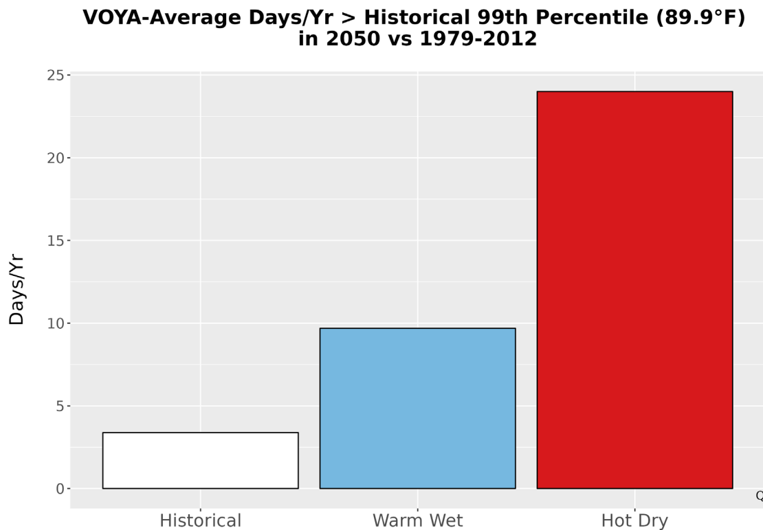
Figure 5. Metrics of extreme temperature at VOYA. The bar graph represents the average number of days annually with temperatures greater than the historical 99th percentile (89.9 °F) historically (1979-2012) and for the two climate futures (2050).
