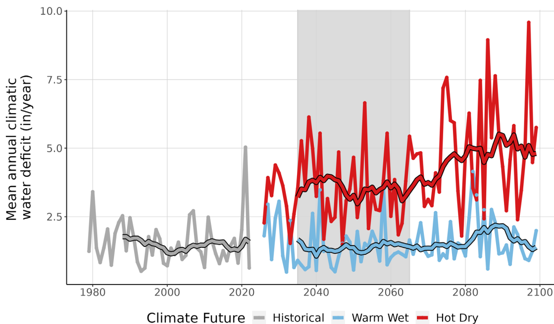
Figure 9. This line graph compares observed climatic water deficit at VOYA (inches/year) (1979-2022) with projected climatic water deficit for the two climate futures over the period 2023-2099. The historical observation data is shown in gray, the Warm Wet climate future in blue, and the Hot Dry climate future in red. The smooth line running through each projection is the 10-year running average for historical observations and future projections. Gray-shaded area represents the time period that was averaged (2035-2065) to summarize future projections for the year 2050.
