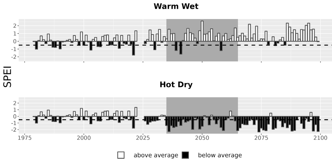
Figure 7. Drought metrics for VOYA. Drought index (SPEI; units = standard deviations from historical) timeseries for each climate future. Below-average SPEI (black bars) indicates dry conditions. The dotted line (SPEI = -0.5) indicates drought conditions.
