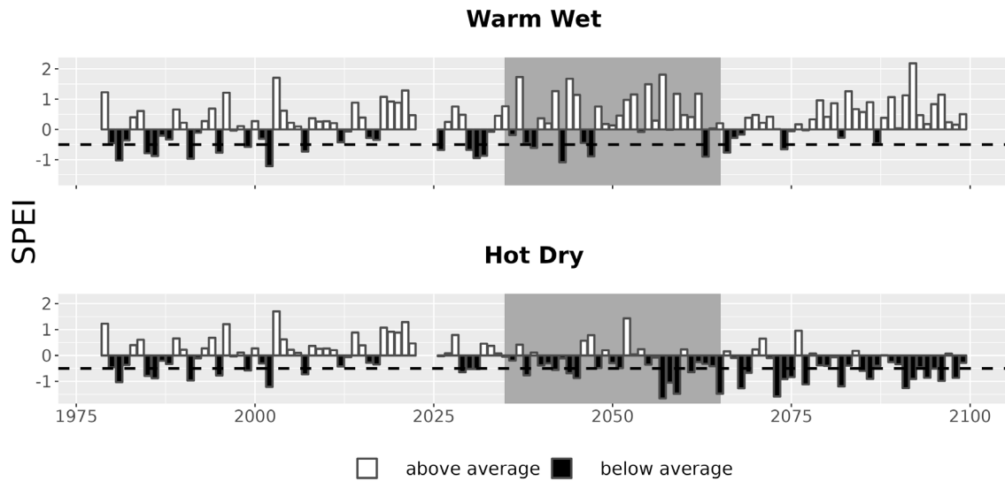
Figure 7. Drought metrics for VIVE. Drought index (SPEI; units = standard deviations from historical) timeseries for each climate future. Below-average SPEI (black bars) indicates dry conditions. The dotted line (SPEI = -0.5) indicates drought conditions.
