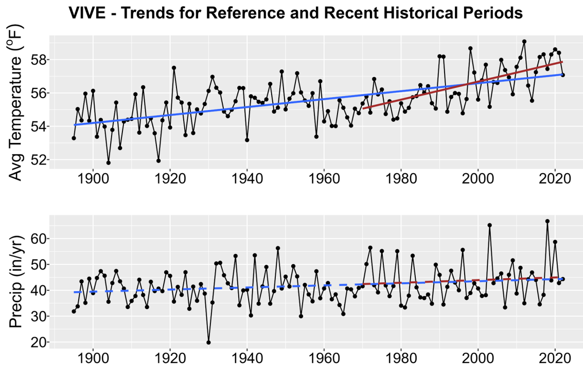
Figure 1. Historical trends in annual average temperature (upper plot) and annual total precipitation (lower plot) for VIVE from 1895-2022. Black points show yearly values while blue lines are linear regressions for the entire period record and red lines for 1970-2022 trends. Solid lines are significant trends (i.e., p < 0.05 ); dashed lines are not statistically significant.
