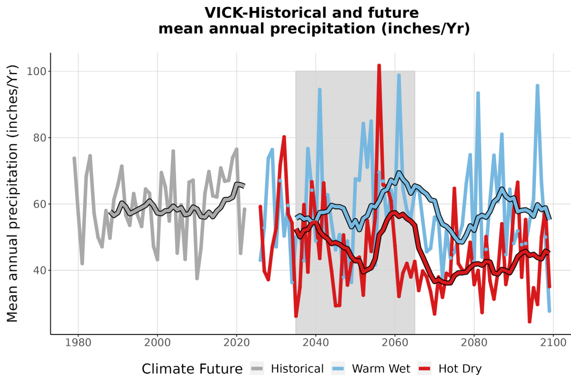
Figure 4. This graph compares observed average annual precipitation at VICK (inches/year) (1979-2022) with projected average annual precipitation for the two climate futures over the period 2023-2099. The historically observed data is shown in gray, the Warm Wet climate future in blue, and the Hot Dry climate future in red. The smooth line running through each projection is the 10-year running average for historical observations and future projections. The gray-shaded area represents the time period that was averaged (2035-2065) to summarize future projections for the year 2050 (Appendix 1).
