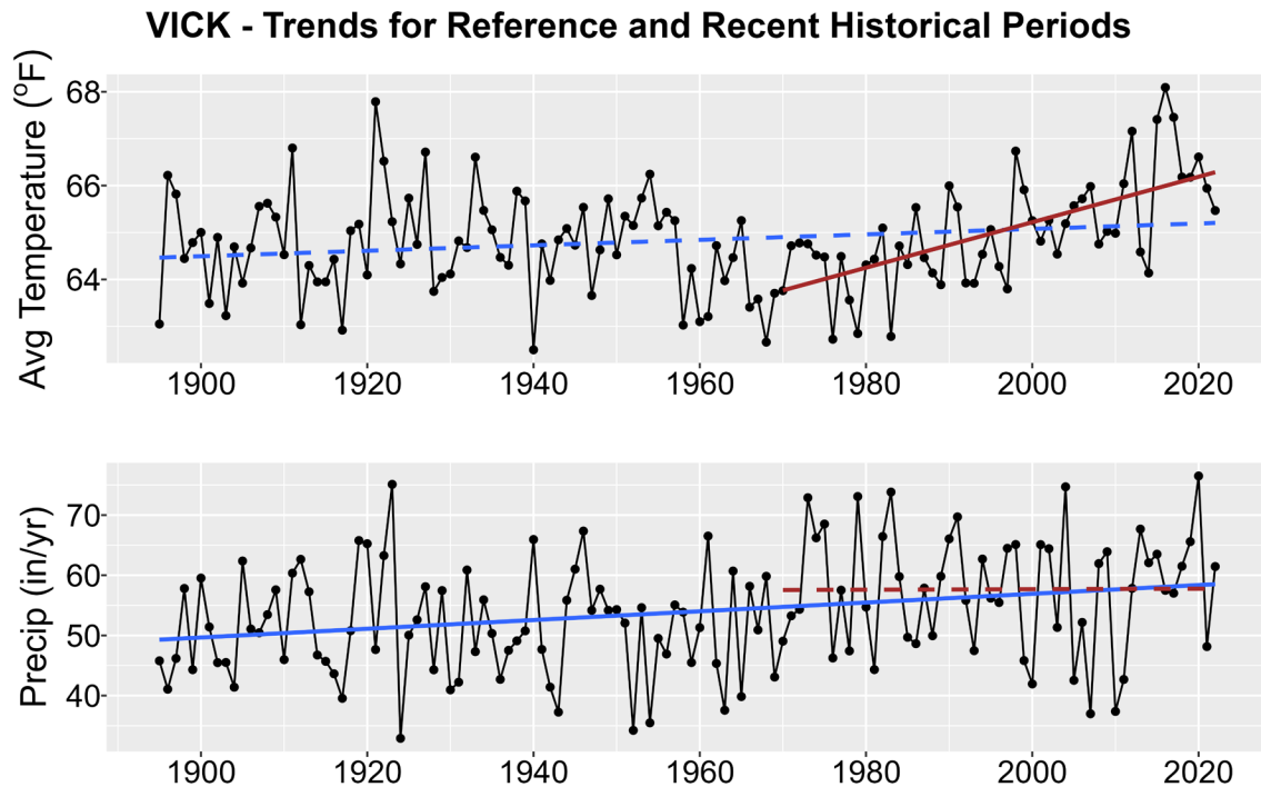
Figure 1. Historical trends in annual average temperature (upper plot) and annual total precipitation (lower plot) for VICK from 1895-2022. Black points show yearly values while blue lines are linear regressions for the entire period record and red lines for 1970-2022 trends. Solid lines are significant trends (i.e., p < 0.05 ); dashed lines are not statistically significant.
