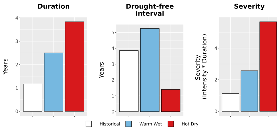
Figure 8. Drought metrics for VICK. (Left) Average drought duration (years) historically (1979-2012) and under each climate future. (Middle) Average drought return interval (years), indicating the expected amount of time between periods of drought, historically and under each climate future. (Right) Average drought severity, a measure of drought intensity multiplied by duration, historically and under each climate future.
