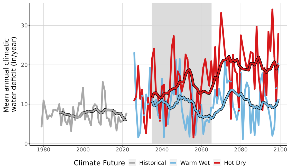
Figure 9. This line graph compares observed climatic water deficit at VICK (inches/year) (1979-2022) with projected climatic water deficit for the two climate futures over the period 2023-2099. The historical observation data is shown in gray, the Warm Wet climate future in blue, and the Hot Dry climate future in red. The smooth line running through each projection is the 10-year running average for historical observations and future projections. Gray-shaded area represents the time period that was averaged (2035-2065) to summarize future projections for the year 2050.
