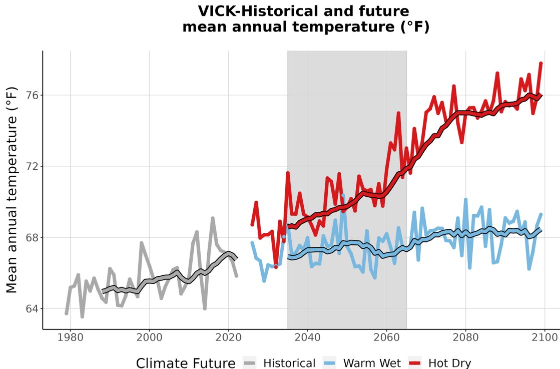
Figure 3. This graph compares observed average annual temperature at VICK (°F) (1979-2022) with projected average annual temperature for the two climate futures over the period 2023-2099. The historically observed data
