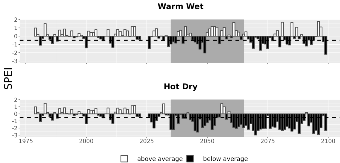
Figure 7. Drought metrics for VICK. Drought index (SPEI; units = standard deviations from historical) timeseries for each climate future. Below-average SPEI (black bars) indicates dry conditions. The dotted line (SPEI = -0.5) indicates drought conditions.
