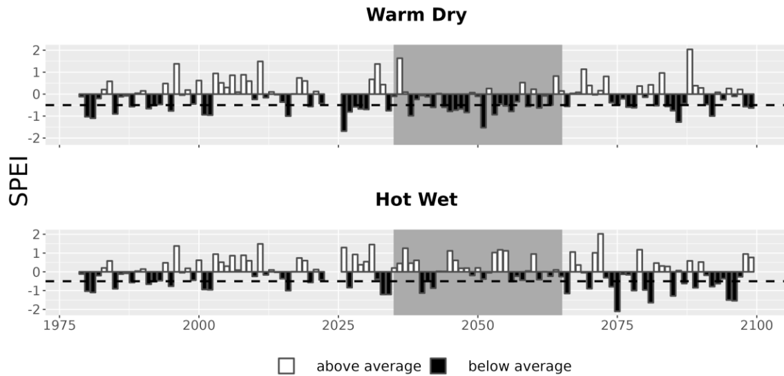
Figure 7. Drought metrics for VAMA. Drought index (SPEI; units = standard deviations from historical) timeseries for each climate future. Below-average SPEI (black bars) indicates dry conditions. The dotted line (SPEI = -0.5) indicates drought conditions.
