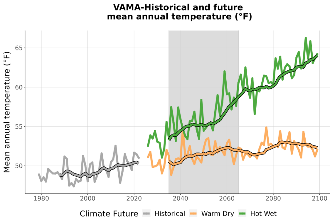
Figure 3. This graph compares observed average annual temperature at VAMA (°F) (1979-2022) with projected average annual temperature for the two climate futures over the period 2023-2099. The historically observed data
