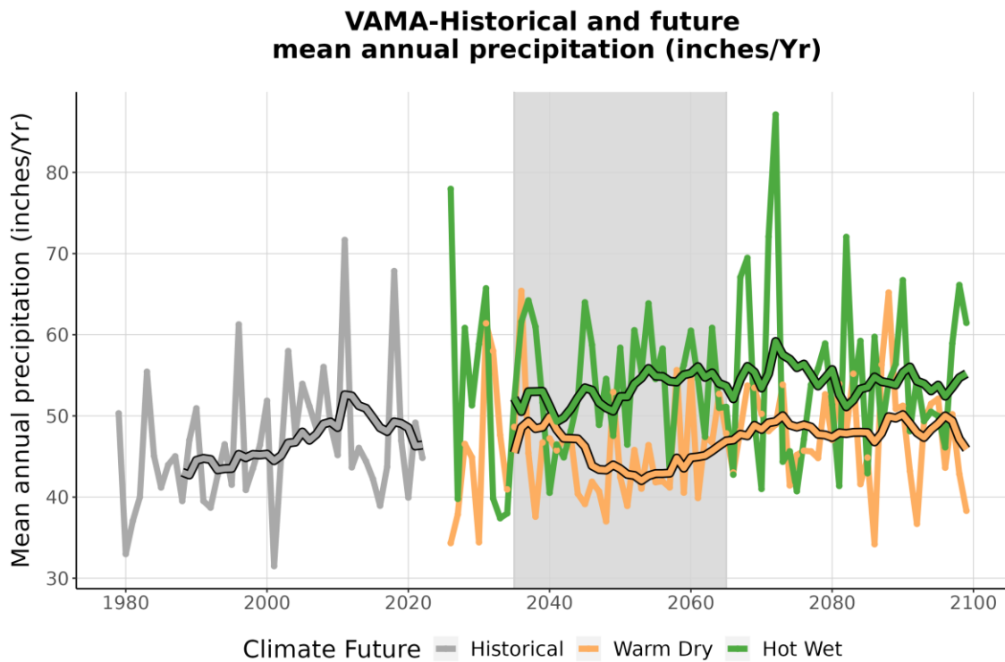
Figure 4. This graph compares observed average annual precipitation at VAMA (inches/year) (1979-2022) with projected average annual precipitation for the two climate futures over the period 2023-2099. The historically observed data is shown in gray, the Warm Dry climate future in orange, and the Hot Wet climate future in green. The smooth line running through each projection is the 10-year running average for historical observations and future projections. The gray-shaded area represents the time period that was averaged (2035-2065) to summarize future projections for the year 2050 (Appendix 1).
