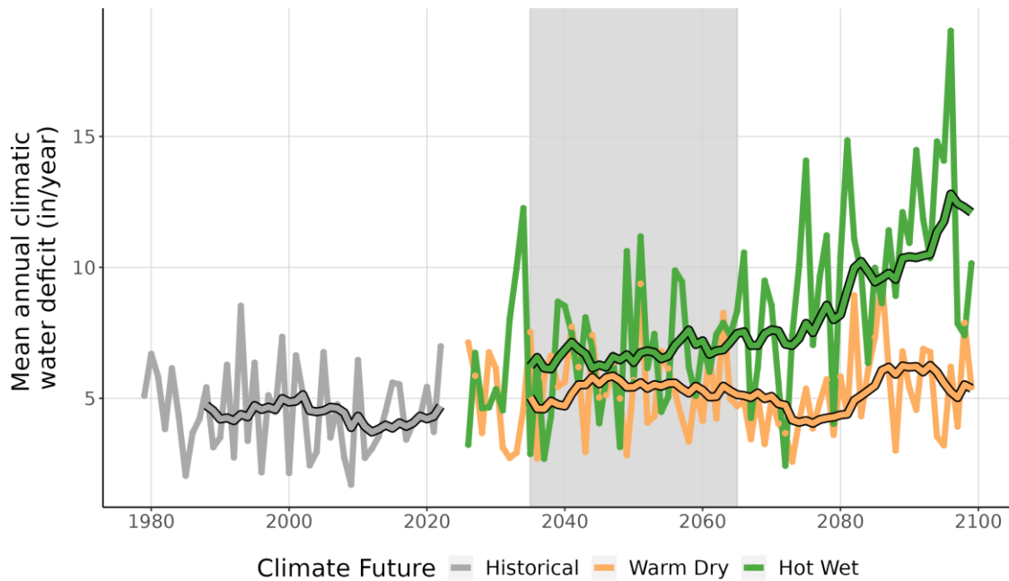
Figure 9. This line graph compares observed climatic water deficit at VAMA (inches/year) (1979-2022) with projected climatic water deficit for the two climate futures over the period 2023-2099. The historical observation data is shown in gray, the Warm Dry climate future in orange, and the Hot Wet climate future in green. The smooth line running through each projection is the 10-year running average for historical observations and future projections. Gray-shaded area represents the time period that was averaged (2035-2065) to summarize future projections for the year 2050.
