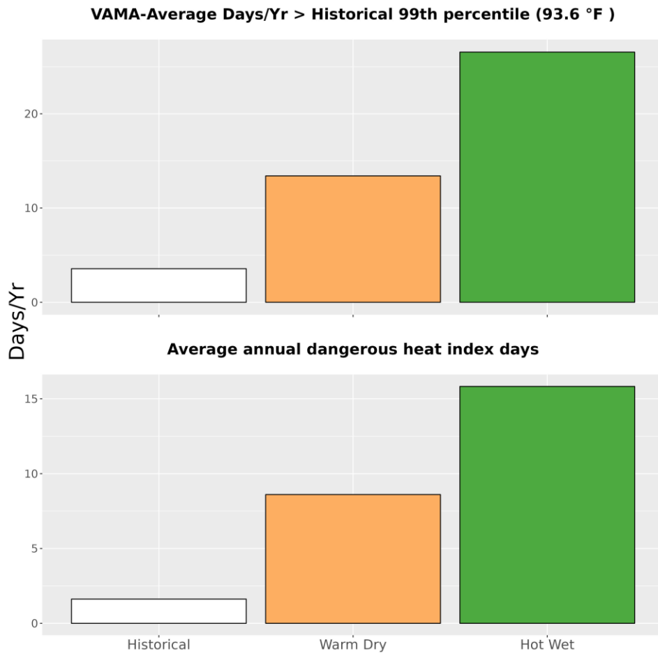
Figure 5. The upper bar graph represents the average number of days annually with temperatures greater than the historical 99th percentile (93.6 °F) historically (1979-2012) and for the two climate futures (2050). The bottom bar graph represents the average annual number of dangerous heat index days historically and for the two climate futures. Dangerous heat index days are days that exceed 105 °F.
