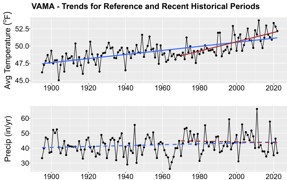
Figure 1. Historical trends in annual average temperature (upper plot) and annual total precipitation (lower plot) for VAMA from 1895-2022. Black points show yearly values while blue lines are linear regressions for the entire period record and red lines for 1970-2022 trends. Solid lines are significant trends (i.e., p < 0.05 ); dashed lines are not statistically significant.
