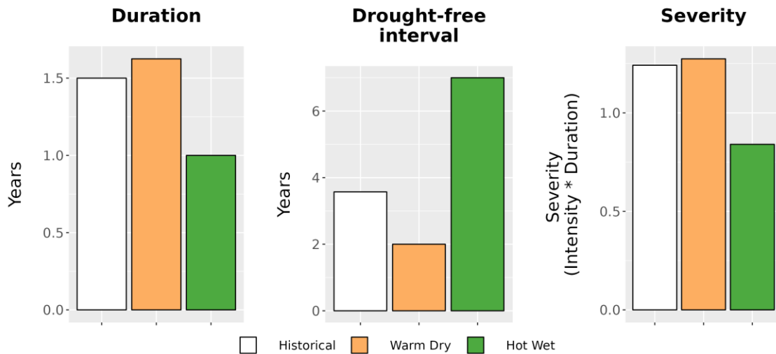
Figure 8. Drought metrics for VAMA. (Left) Average drought duration (years) historically (1979-2012) and under each climate future. (Middle) Average drought return interval (years), indicating the expected amount of time between periods of drought, historically and under each climate future. (Right) Average drought severity, a measure of drought intensity multiplied by duration, historically and under each climate future.
