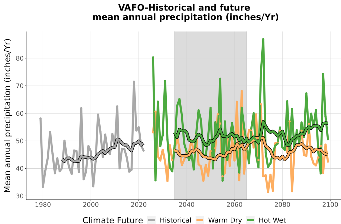
Figure 4. This graph compares observed average annual precipitation at VAFO (inches/year) (1979-2022) with projected average annual precipitation for the two climate futures over the period 2023-2099. The historically observed data is shown in gray, the Warm Dry climate future in orange, and the Hot Wet climate future in green. The smooth line running through each projection is the 10-year running average for historical observations and future projections. The gray-shaded area represents the time period that was averaged (2035-2065) to summarize future projections for the year 2050 (Appendix 1).
