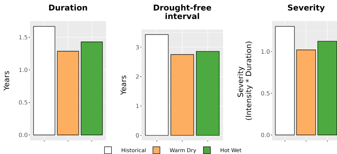
Figure 8. Drought metrics for VAFO. (Left) Average drought duration (years) historically (1979-2012) and under each climate future. (Middle) Average drought return interval (years), indicating the expected amount of time between periods of drought, historically and under each climate future. (Right) Average drought severity, a measure of drought intensity multiplied by duration, historically and under each climate future.
