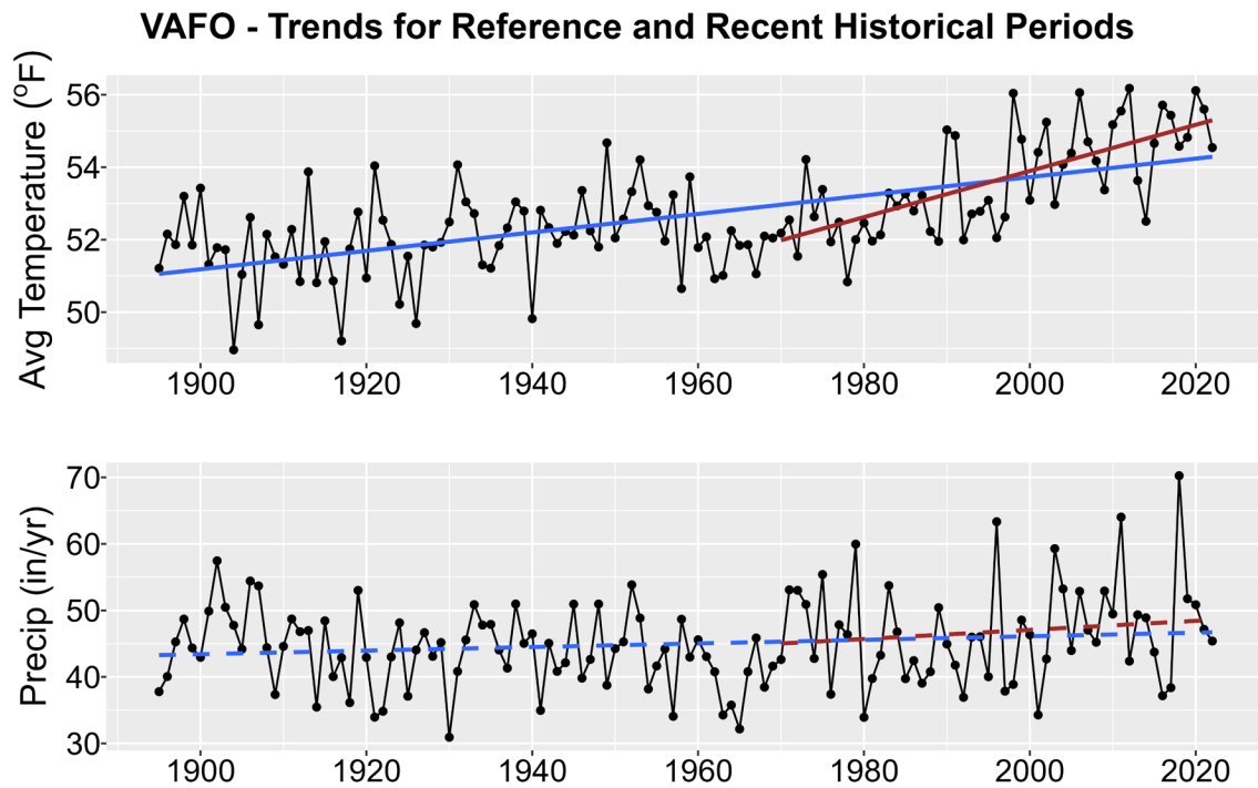
Figure 1. Historical trends in annual average temperature (upper plot) and annual total precipitation (lower plot) for VAFO from 1895-2022. Black points show yearly values while blue lines are linear regressions for the entire period record and red lines for 1970-2022 trends. Solid lines are significant trends (i.e., p < 0.05 ); dashed lines are not statistically significant.
