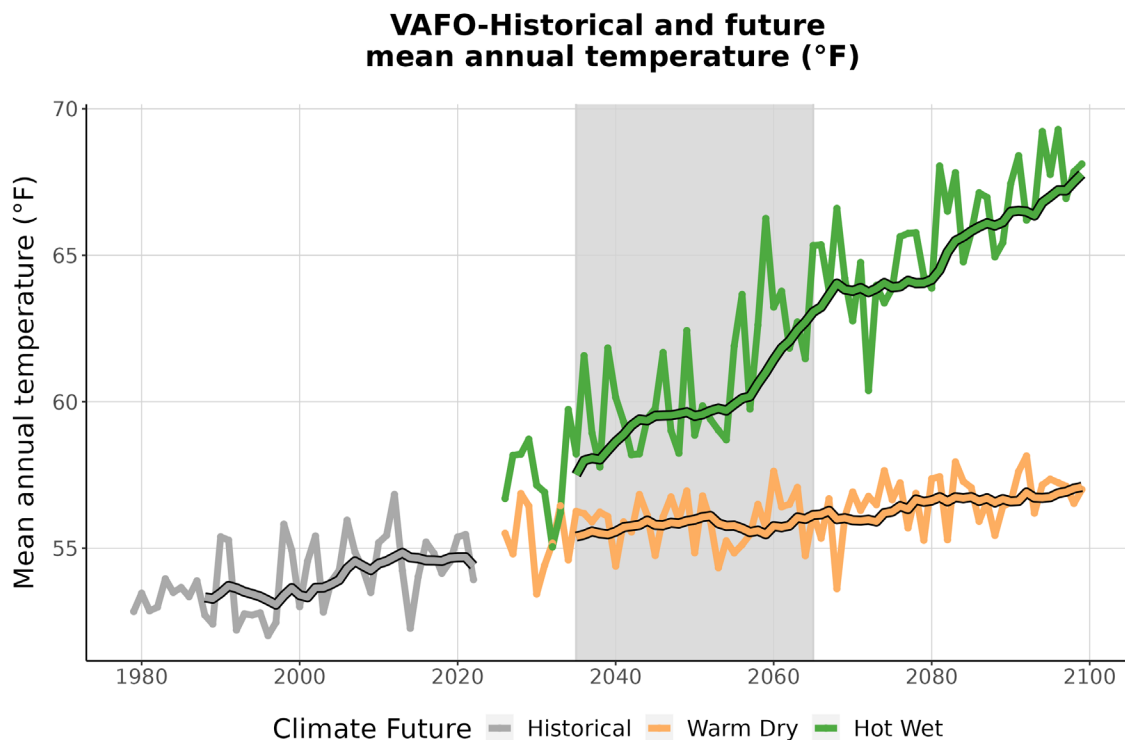
Figure 3. This graph compares observed average annual temperature at VAFO (°F) (1979-2022) with projected average annual temperature for the two climate futures over the period 2023-2099. The historically observed data
