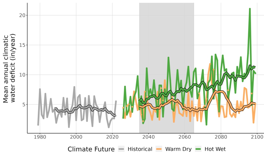
Figure 9. This line graph compares observed climatic water deficit at VAFO (inches/year) (1979-2022) with projected climatic water deficit for the two climate futures over the period 2023-2099. The historical observation data is shown in gray, the Warm Dry climate future in orange, and the Hot Wet climate future in green. The smooth line running through each projection is the 10-year running average for historical observations and future projections. Gray-shaded area represents the time period that was averaged (2035-2065) to summarize future projections for the year 2050.
