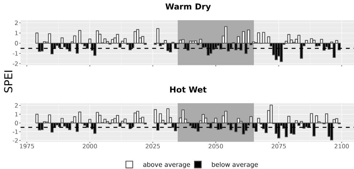
Figure 7. Drought metrics for VAFO. Drought index (SPEI; units = standard deviations from historical) timeseries for each climate future. Below-average SPEI (black bars) indicates dry conditions. The dotted line (SPEI = -0.5) indicates drought conditions.
