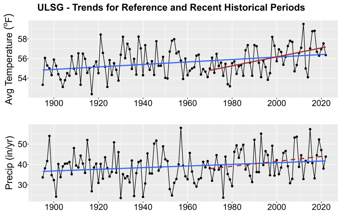
Figure 1. Historical trends in annual average temperature (upper plot) and annual total precipitation (lower plot) for ULSG from 1895-2022. Black points show yearly values while blue lines are linear regressions for the entire period record and red lines for 1970-2022 trends. Solid lines are significant trends (i.e., p < 0.05 ); dashed lines are not statistically significant.
