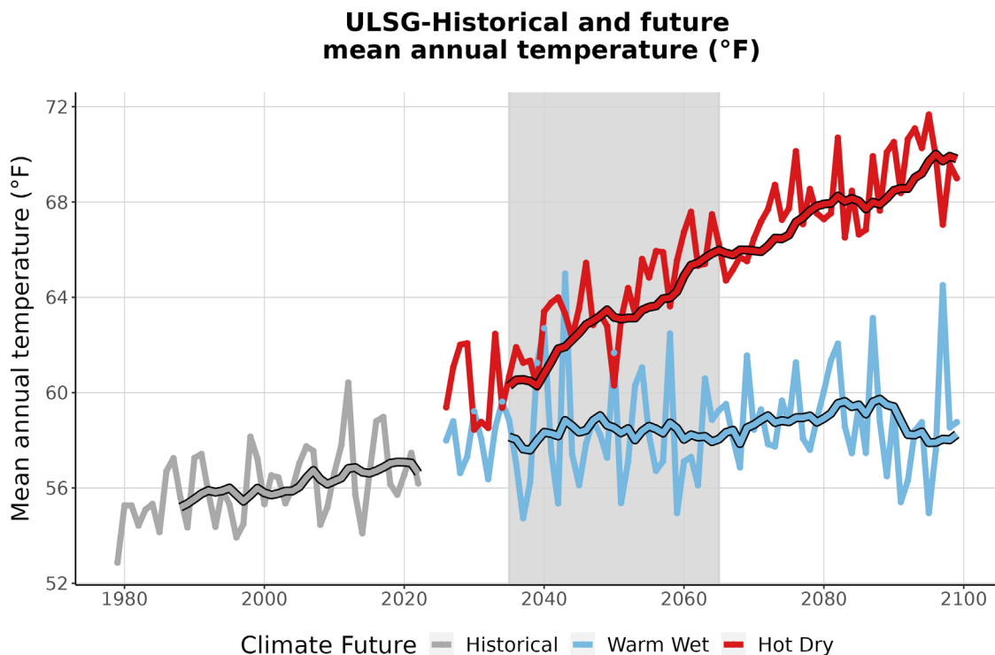
Figure 3. This graph compares observed average annual temperature at ULSG (°F) (1979-2022) with projected average annual temperature for the two climate futures over the period 2023-2099. The historically observed data
