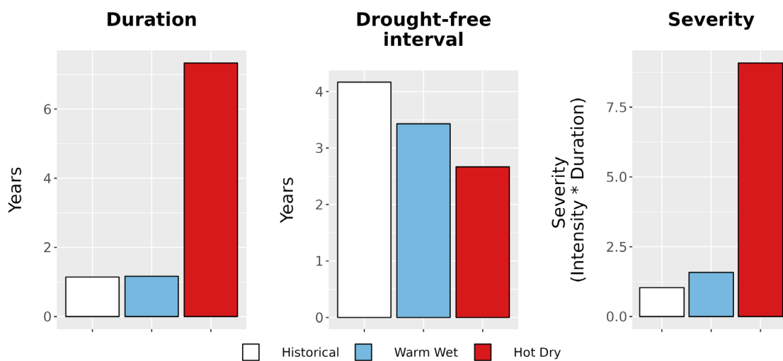
Figure 8. Drought metrics for ULSG. (Left) Average drought duration (years) historically (1979-2012) and under each climate future. (Middle) Average drought return interval (years), indicating the expected amount of time between periods of drought, historically and under each climate future. (Right) Average drought severity, a measure of drought intensity multiplied by duration, historically and under each climate future.
