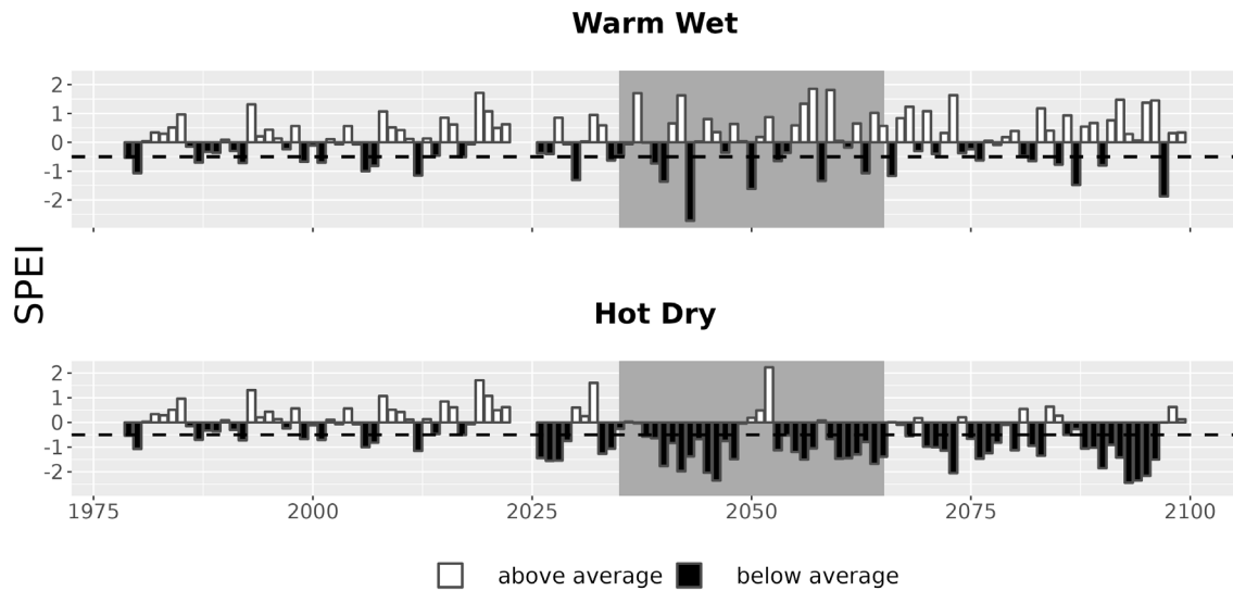
Figure 7. Drought metrics for ULSG. Drought index (SPEI; units = standard deviations from historical) timeseries for each climate future. Below-average SPEI (black bars) indicates dry conditions. The dotted line (SPEI = -0.5) indicates drought conditions.
