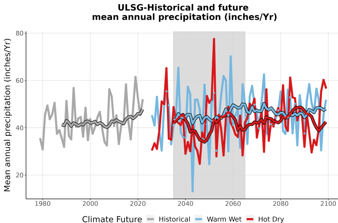
Figure 4. This graph compares observed average annual precipitation at ULSG (inches/year) (1979-2022) with projected average annual precipitation for the two climate futures over the period 2023-2099. The historically observed data is shown in gray, the Warm Wet climate future in blue, and the Hot Dry climate future in red. The smooth line running through each projection is the 10-year running average for historical observations and future projections. The gray-shaded area represents the time period that was averaged (2035-2065) to summarize future projections for the year 2050 (Appendix 1).
