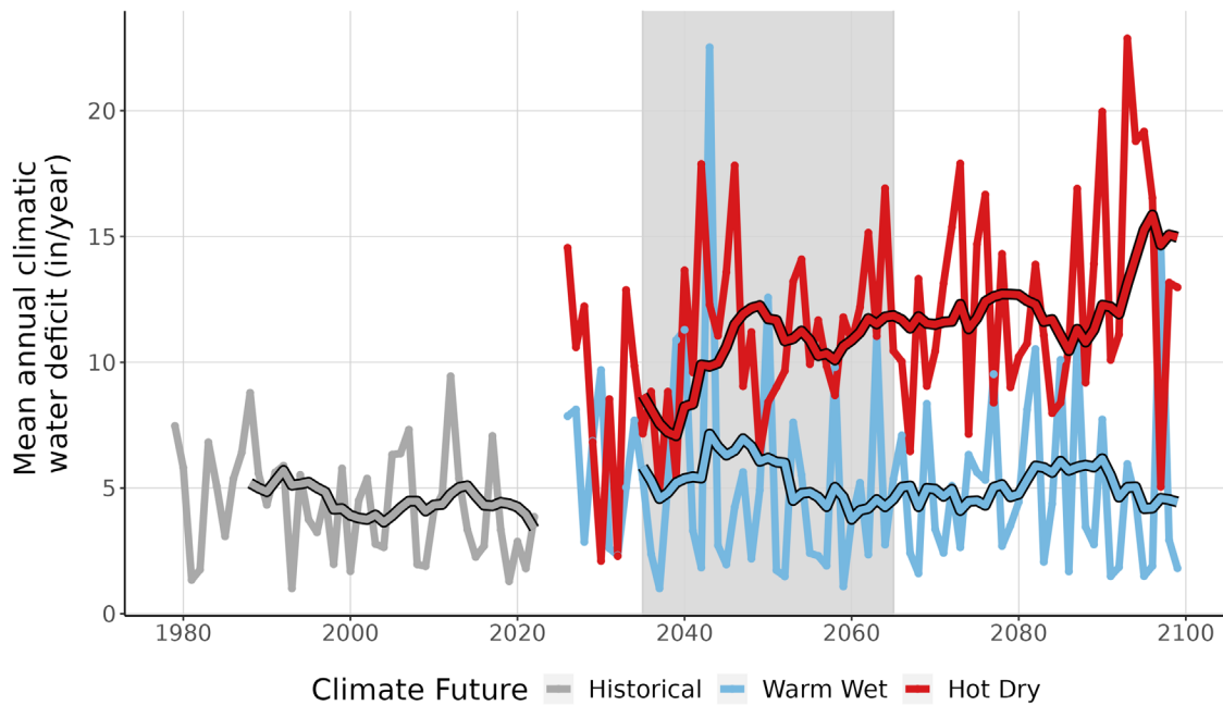
Figure 9. This line graph compares observed climatic water deficit at ULSG (inches/year) (1979-2022) with projected climatic water deficit for the two climate futures over the period 2023-2099. The historical observation data is shown in gray, the Warm Wet climate future in blue, and the Hot Dry climate future in red. The smooth line running through each projection is the 10-year running average for historical observations and future projections. Gray-shaded area represents the time period that was averaged (2035-2065) to summarize future projections for the year 2050.
