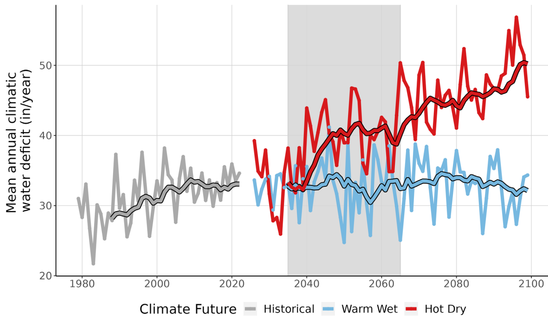
Figure 9. This line graph compares observed climatic water deficit at TUZI (inches/year) (1979-2022) with projected climatic water deficit for the two climate futures over the period 2023-2099. The historical observation data is shown in gray, the Warm Wet climate future in blue, and the Hot Dry climate future in red. The smooth line running through each projection is the 10-year running average for historical observations and future projections. Gray-shaded area represents the time period that was averaged (2035-2065) to summarize future projections for the year 2050.
