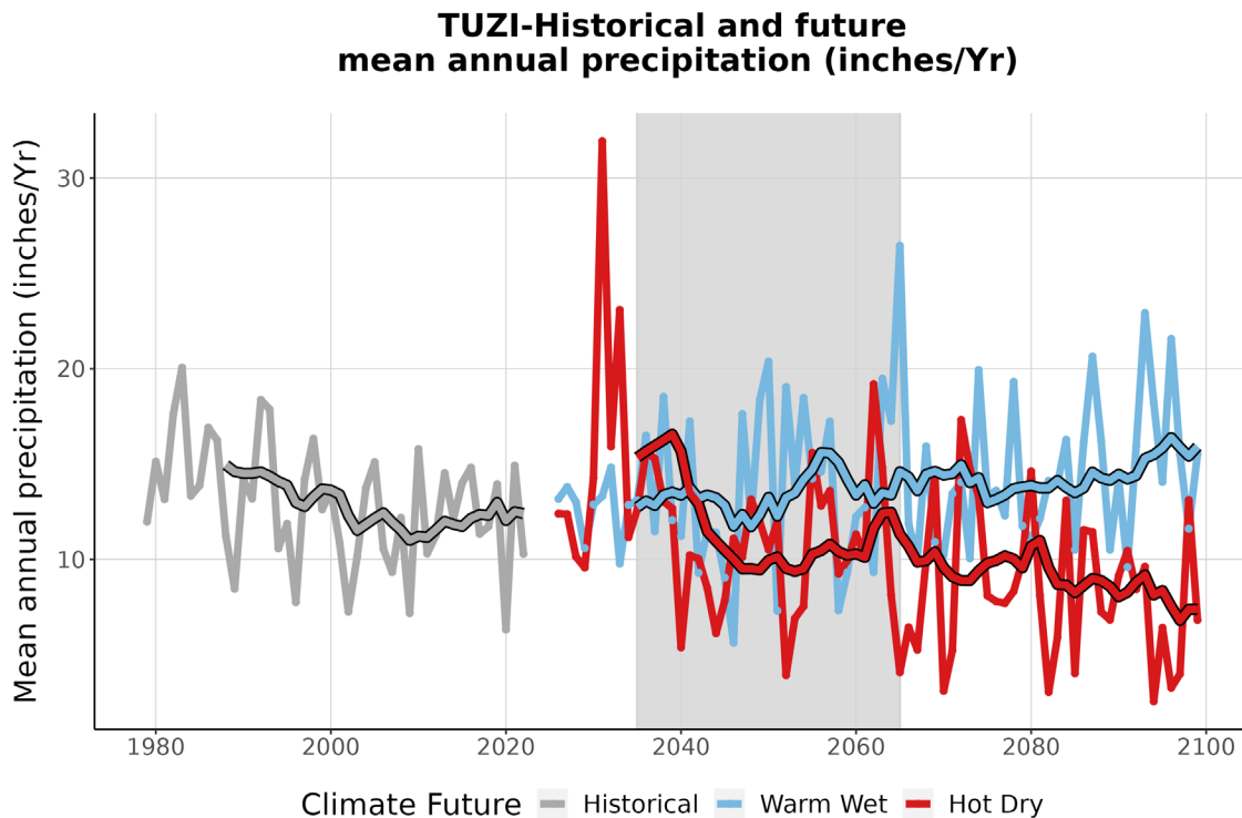
Figure 4. This graph compares observed average annual precipitation at TUZI (inches/year) (1979-2022) with projected average annual precipitation for the two climate futures over the period 2023-2099. The historically observed data is shown in gray, the Warm Wet climate future in blue, and the Hot Dry climate future in red. The smooth line running through each projection is the 10-year running average for historical observations and future projections. The gray-shaded area represents the time period that was averaged (2035-2065) to summarize future projections for the year 2050 (Appendix 1).
