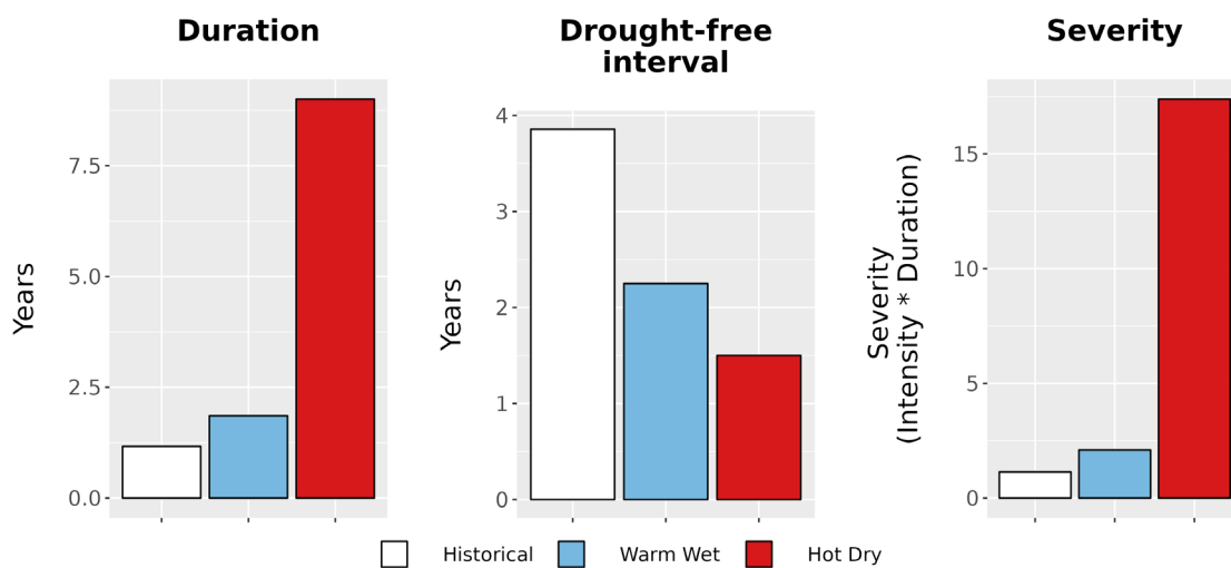
Figure 8. Drought metrics for TUZI. (Left) Average drought duration (years) historically (1979-2012) and under each climate future. (Middle) Average drought return interval (years), indicating the expected amount of time between periods of drought, historically and under each climate future. (Right) Average drought severity, a measure of drought intensity multiplied by duration, historically and under each climate future.
