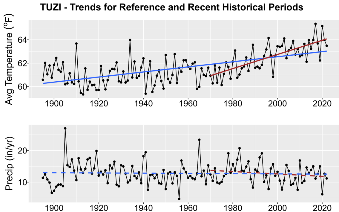
Figure 1. Historical trends in annual average temperature (upper plot) and annual total precipitation (lower plot) for TUZI from 1895-2022. Black points show yearly values while blue lines are linear regressions for the entire period record and red lines for 1970-2022 trends. Solid lines are significant trends (i.e., p < 0.05 ); dashed lines are not statistically significant.
