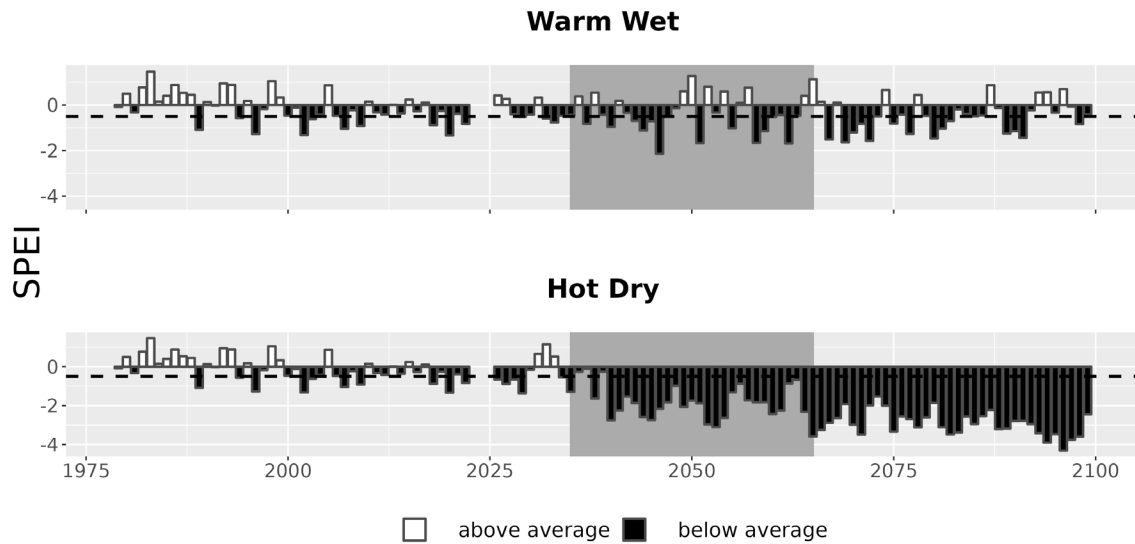
Figure 7. Drought metrics for TUZI. Drought index (SPEI; units = standard deviations from historical) timeseries for each climate future. Below-average SPEI (black bars) indicates dry conditions. The dotted line (SPEI = -0.5) indicates drought conditions.
