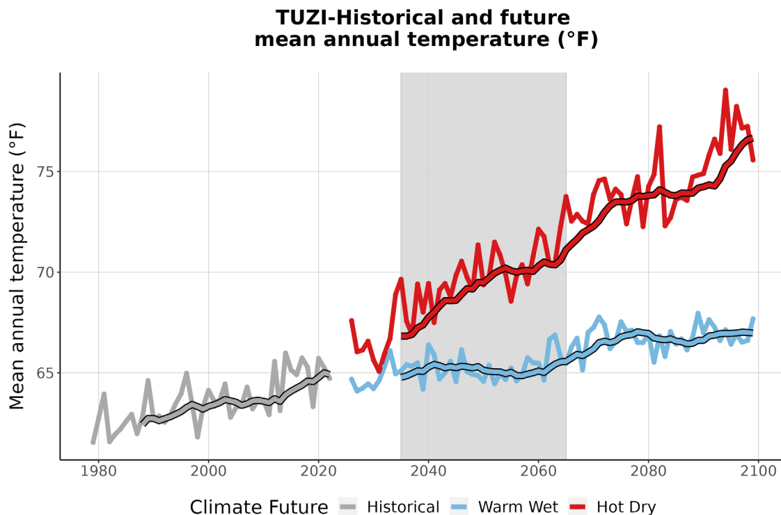
Figure 3. This graph compares observed average annual temperature at TUZI (°F) (1979-2022) with projected average annual temperature for the two climate futures over the period 2023-2099. The historically observed data
