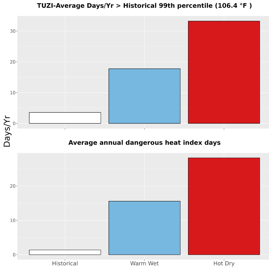
Figure 5. The upper bar graph represents the average number of days annually with temperatures greater than the historical 99th percentile (106.4 °F) historically (1979-2012) and for the two climate futures (2050). The bottom bar graph represents the average annual number of dangerous heat index days historically and for the two climate futures. Dangerous heat index days are days that exceed 105 °F.
