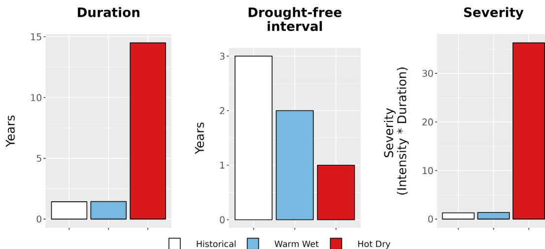
Figure 8. Drought metrics for TUSK. (Left) Average drought duration (years) historically (1979-2012) and under each climate future. (Middle) Average drought return interval (years), indicating the expected amount of time between periods of drought, historically and under each climate future. (Right) Average drought severity, a measure of drought intensity multiplied by duration, historically and under each climate future.
