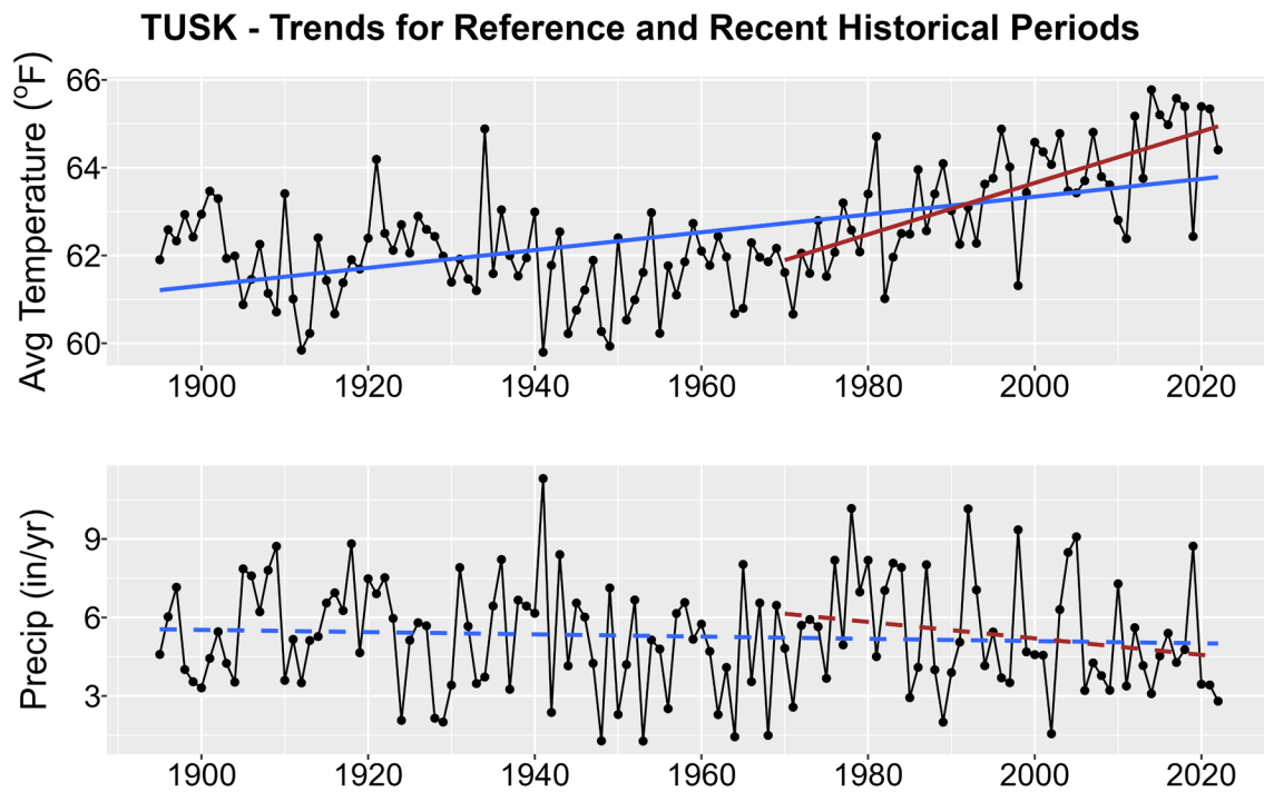
Figure 1. Historical trends in annual average temperature (upper plot) and annual total precipitation (lower plot) for TUSK from 1895-2022. Black points show yearly values while blue lines are linear regressions for the entire period record and red lines for 1970-2022 trends. Solid lines are significant trends (i.e., p < 0.05 ); dashed lines are not statistically significant.
