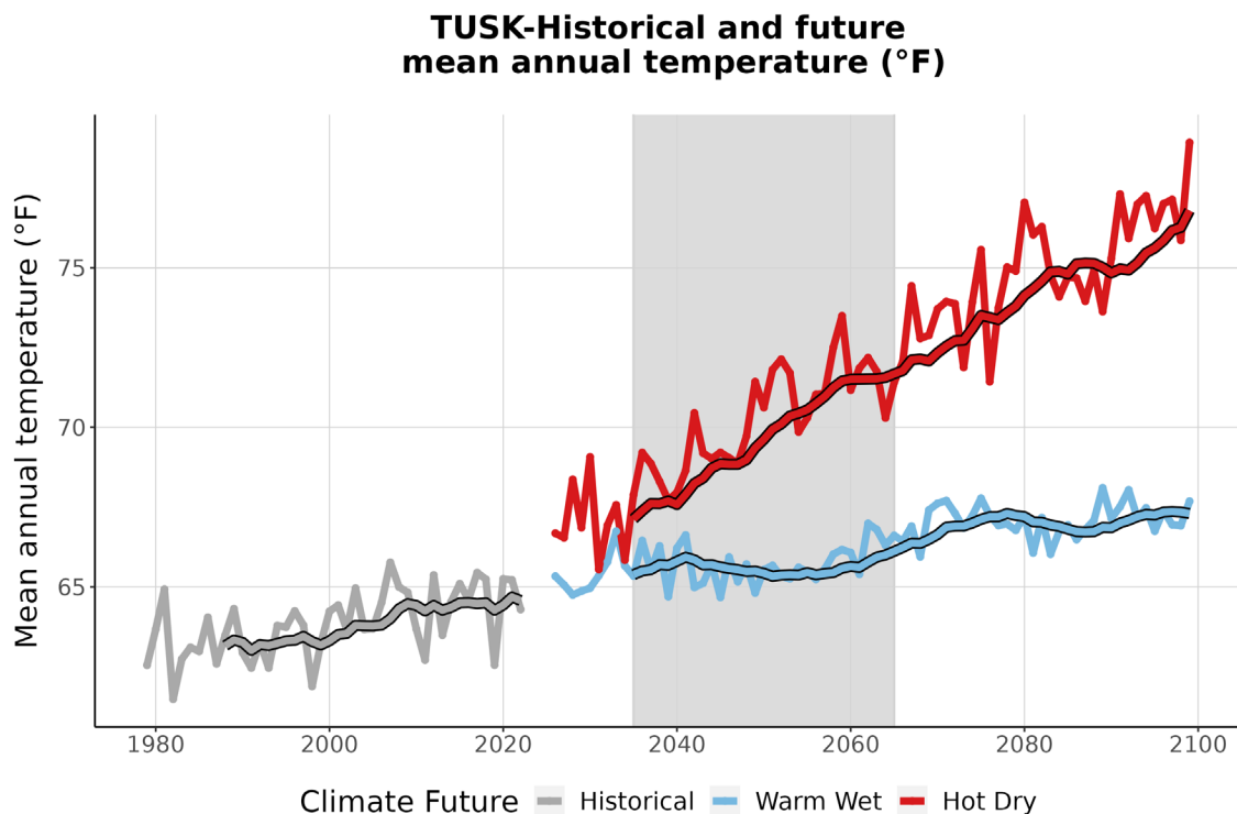
Figure 3. This graph compares observed average annual temperature at TUSK (°F) (1979-2022) with projected average annual temperature for the two climate futures over the period 2023-2099. The historically observed data
