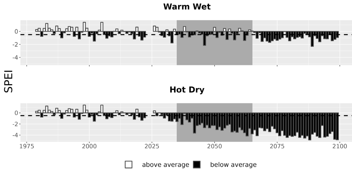
Figure 7. Drought metrics for TUSK. Drought index (SPEI; units = standard deviations from historical) timeseries for each climate future. Below-average SPEI (black bars) indicates dry conditions. The dotted line (SPEI = -0.5) indicates drought conditions.
