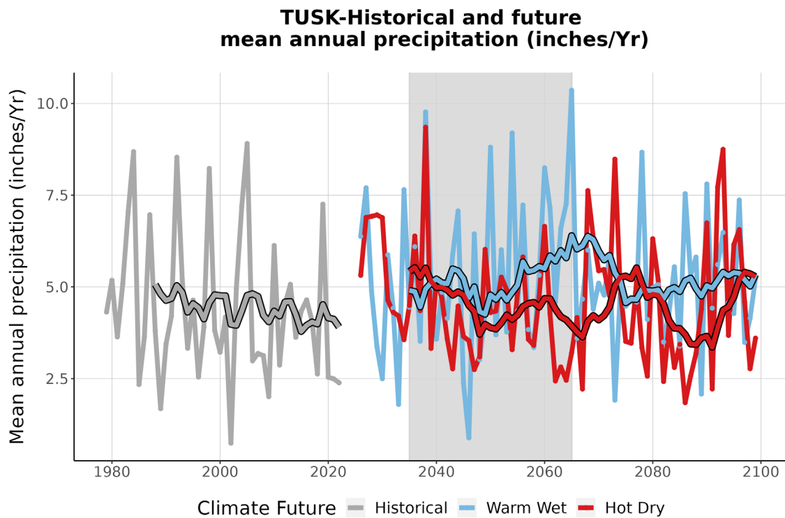
Figure 4. This graph compares observed average annual precipitation at TUSK (inches/year) (1979-2022) with projected average annual precipitation for the two climate futures over the period 2023-2099. The historically observed data is shown in gray, the Warm Wet climate future in blue, and the Hot Dry climate future in red. The smooth line running through each projection is the 10-year running average for historical observations and future projections. The gray-shaded area represents the time period that was averaged (2035-2065) to summarize future projections for the year 2050 (Appendix 1).
