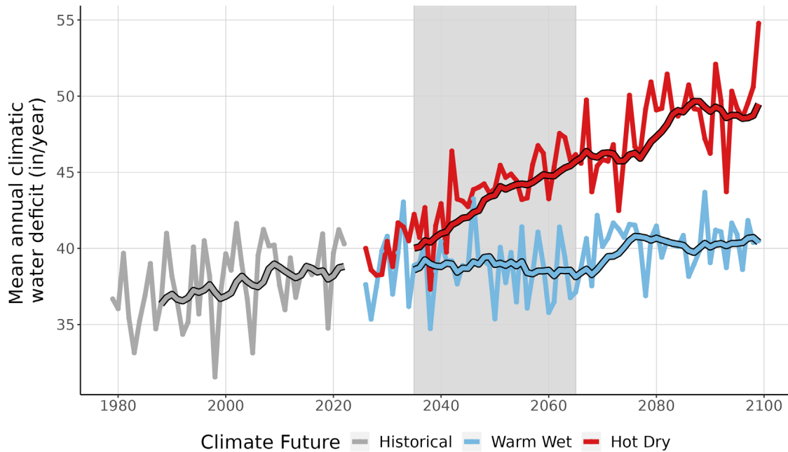
Figure 9. This line graph compares observed climatic water deficit at TUSK (inches/year) (1979-2022) with projected climatic water deficit for the two climate futures over the period 2023-2099. The historical observation data is shown in gray, the Warm Wet climate future in blue, and the Hot Dry climate future in red. The smooth line running through each projection is the 10-year running average for historical observations and future projections. Gray-shaded area represents the time period that was averaged (2035-2065) to summarize future projections for the year 2050.
