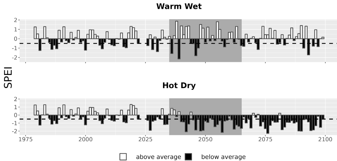
Figure 7. Drought metrics for TUPE. Drought index (SPEI; units = standard deviations from historical) timeseries for each climate future. Below-average SPEI (black bars) indicates dry conditions. The dotted line (SPEI = -0.5) indicates drought conditions.
