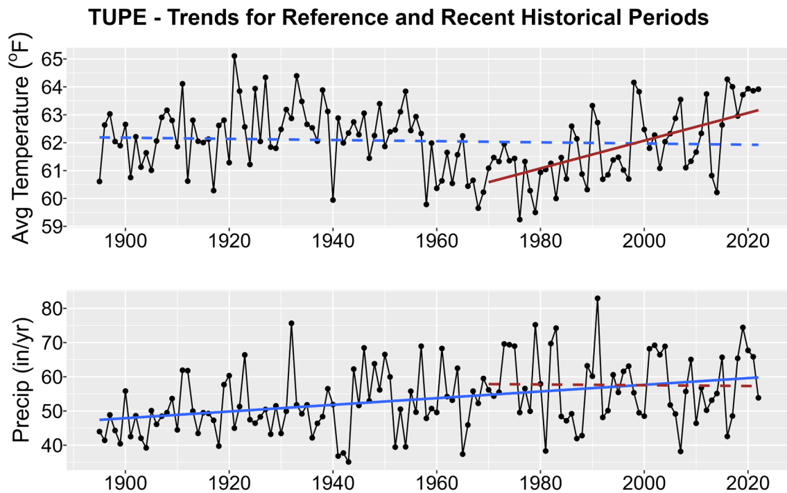
Figure 1. Historical trends in annual average temperature (upper plot) and annual total precipitation (lower plot) for TUPE from 1895-2022. Black points show yearly values while blue lines are linear regressions for the entire period record and red lines for 1970-2022 trends. Solid lines are significant trends (i.e., p < 0.05 ); dashed lines are not statistically significant.
