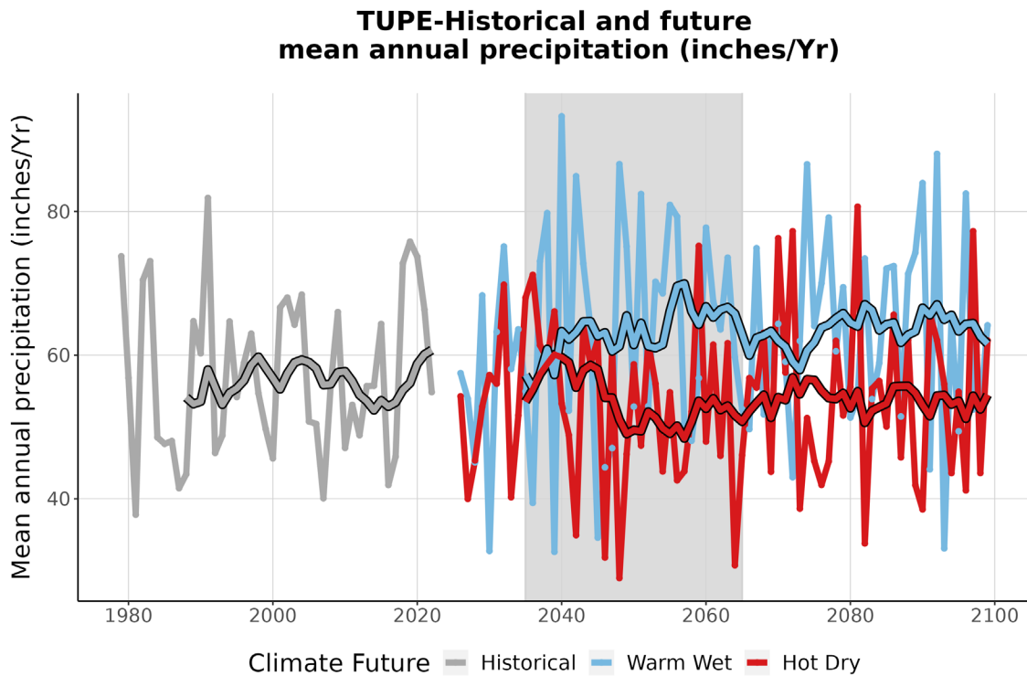
Figure 4. This graph compares observed average annual precipitation at TUPE (inches/year) (1979-2022) with projected average annual precipitation for the two climate futures over the period 2023-2099. The historically observed data is shown in gray, the Warm Wet climate future in blue, and the Hot Dry climate future in red. The smooth line running through each projection is the 10-year running average for historical observations and future projections. The gray-shaded area represents the time period that was averaged (2035-2065) to summarize future projections for the year 2050 (Appendix 1).
