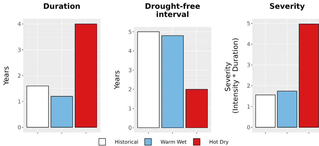
Figure 8. Drought metrics for TUPE. (Left) Average drought duration (years) historically (1979-2012) and under each climate future. (Middle) Average drought return interval (years), indicating the expected amount of time between periods of drought, historically and under each climate future. (Right) Average drought severity, a measure of drought intensity multiplied by duration, historically and under each climate future.
