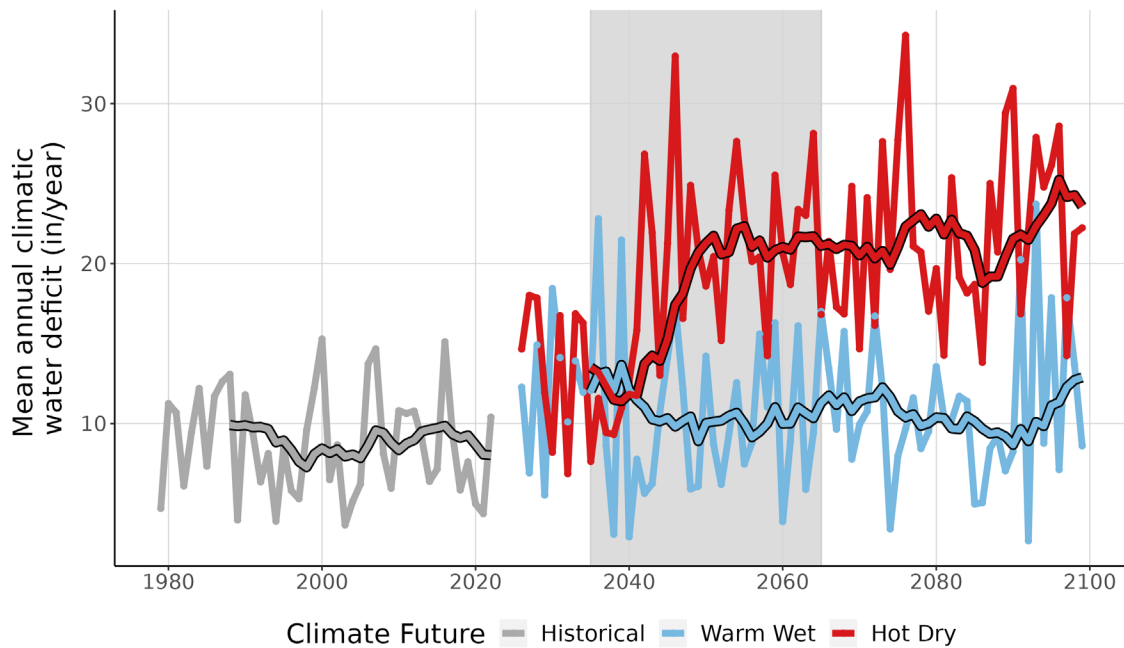
Figure 9. This line graph compares observed climatic water deficit at TUPE (inches/year) (1979-2022) with projected climatic water deficit for the two climate futures over the period 2023-2099. The historical observation data is shown in gray, the Warm Wet climate future in blue, and the Hot Dry climate future in red. The smooth line running through each projection is the 10-year running average for historical observations and future projections. Gray-shaded area represents the time period that was averaged (2035-2065) to summarize future projections for the year 2050.
