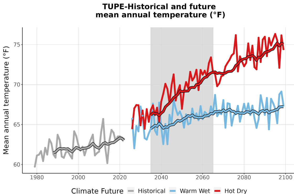
Figure 3. This graph compares observed average annual temperature at TUPE (°F) (1979-2022) with projected average annual temperature for the two climate futures over the period 2023-2099. The historically observed data
