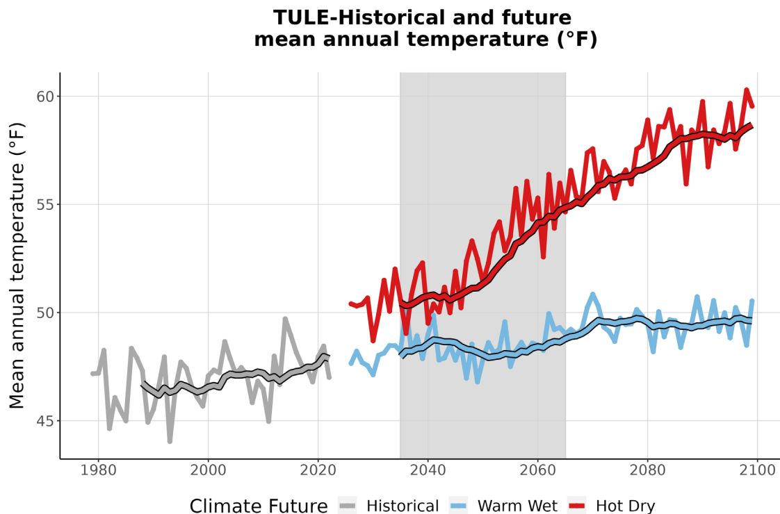
Figure 3. This graph compares observed average annual temperature at TULE (°F) (1979-2022) with projected average annual temperature for the two climate futures over the period 2023-2099. The historically observed data
