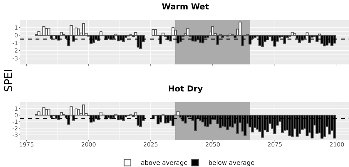
Figure 7. Drought metrics for TULE. Drought index (SPEI; units = standard deviations from historical) timeseries for each climate future. Below-average SPEI (black bars) indicates dry conditions. The dotted line (SPEI = -0.5) indicates drought conditions.
