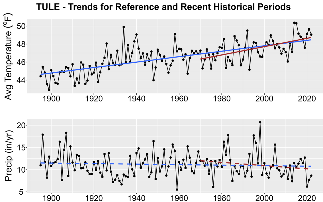
Figure 1. Historical trends in annual average temperature (upper plot) and annual total precipitation (lower plot) for TULE from 1895-2022. Black points show yearly values while blue lines are linear regressions for the entire period record and red lines for 1970-2022 trends. Solid lines are significant trends (i.e., p < 0.05 ); dashed lines are not statistically significant.
