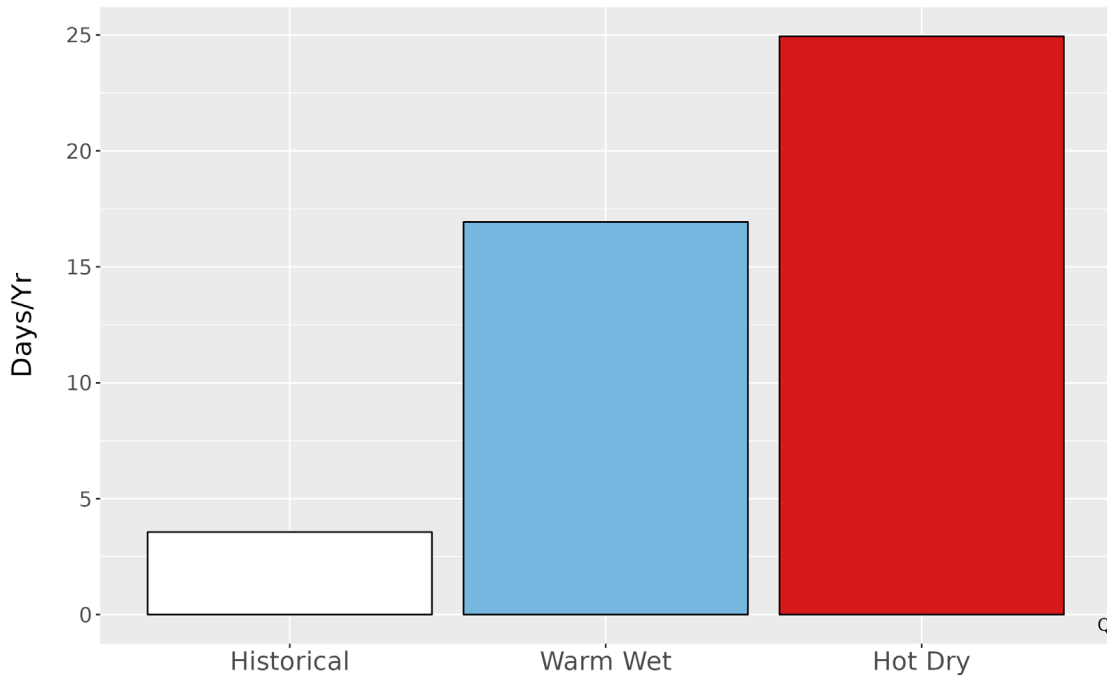
Figure 5. Metrics of extreme temperature at TULE. The bar graph represents the average number of days annually with temperatures greater than the historical 99th percentile (94.4 °F) historically (1979-2012) and for the two climate futures (2050).
