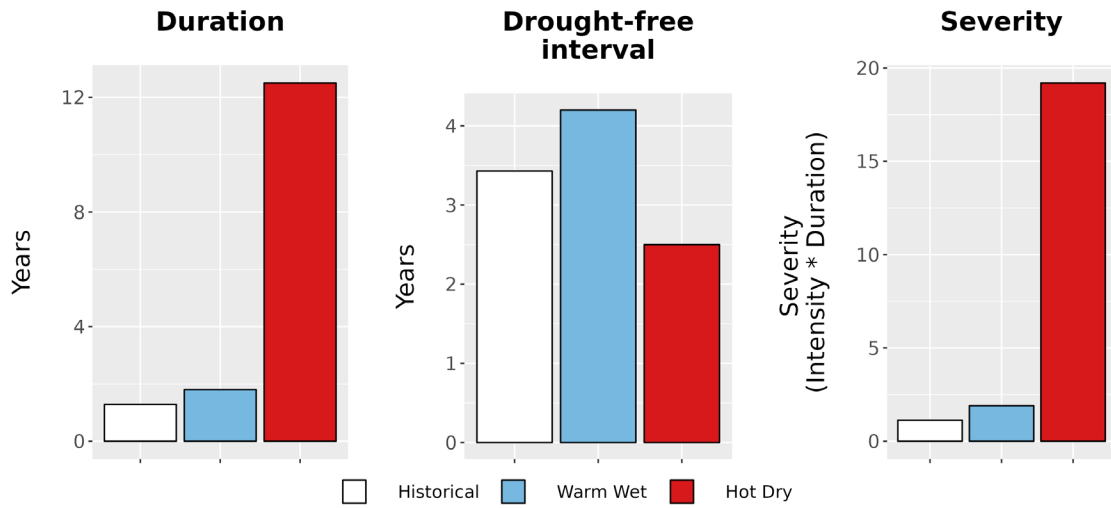
Figure 8. Drought metrics for TULE. (Left) Average drought duration (years) historically (1979-2012) and under each climate future. (Middle) Average drought return interval (years), indicating the expected amount of time between periods of drought, historically and under each climate future. (Right) Average drought severity, a measure of drought intensity multiplied by duration, historically and under each climate future.
