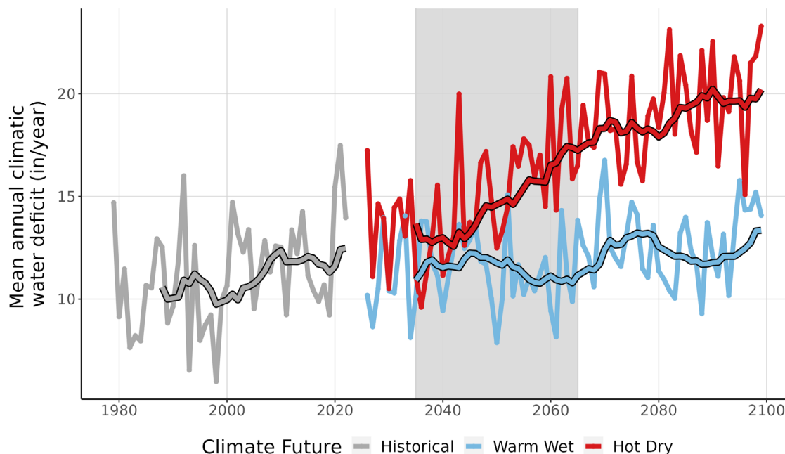
Figure 9. This line graph compares observed climatic water deficit at TULE (inches/year) (1979-2022) with projected climatic water deficit for the two climate futures over the period 2023-2099. The historical observation data is shown in gray, the Warm Wet climate future in blue, and the Hot Dry climate future in red. The smooth line running through each projection is the 10-year running average for historical observations and future projections. Gray-shaded area represents the time period that was averaged (2035-2065) to summarize future projections for the year 2050.
