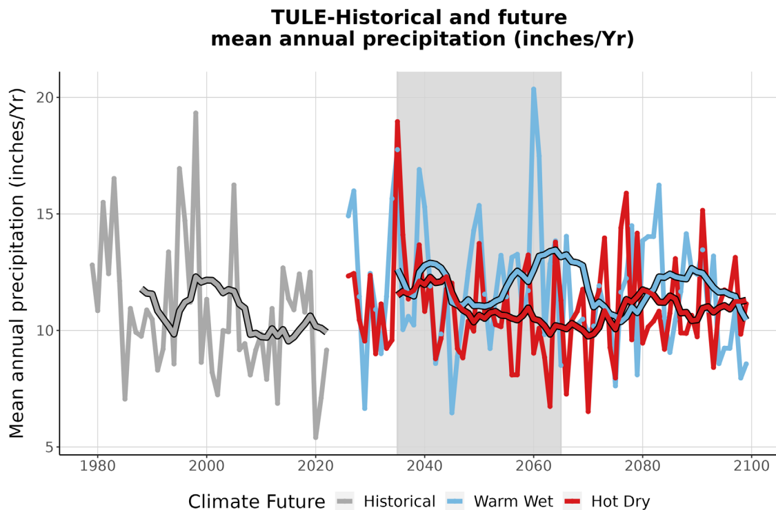
Figure 4. This graph compares observed average annual precipitation at TULE (inches/year) (1979-2022) with projected average annual precipitation for the two climate futures over the period 2023-2099. The historically observed data is shown in gray, the Warm Wet climate future in blue, and the Hot Dry climate future in red. The smooth line running through each projection is the 10-year running average for historical observations and future projections. The gray-shaded area represents the time period that was averaged (2035-2065) to summarize future projections for the year 2050 (Appendix 1).
