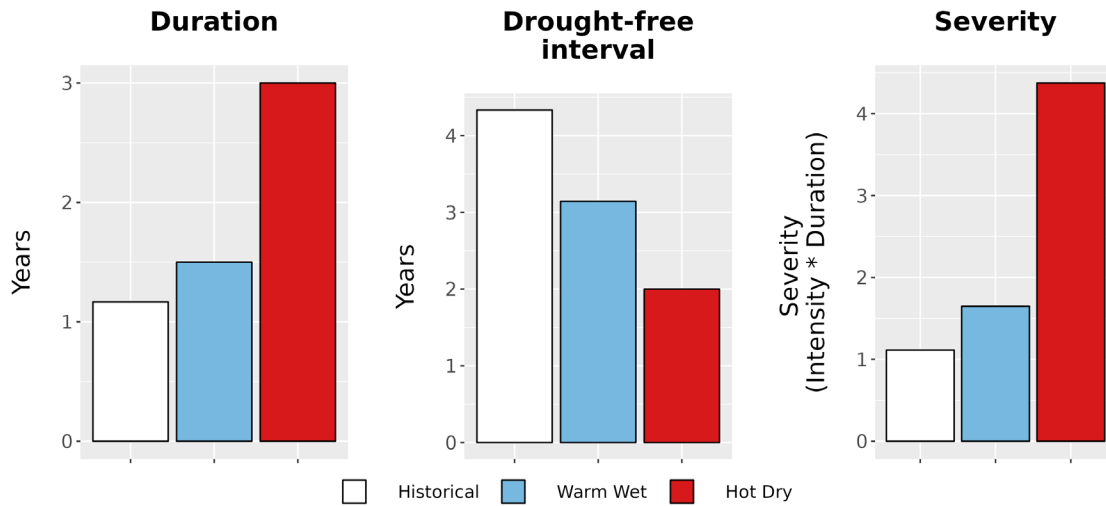
Figure 8. Drought metrics for TUIN. (Left) Average drought duration (years) historically (1979-2012) and under each climate future. (Middle) Average drought return interval (years), indicating the expected amount of time between periods of drought, historically and under each climate future. (Right) Average drought severity, a measure of drought intensity multiplied by duration, historically and under each climate future.
