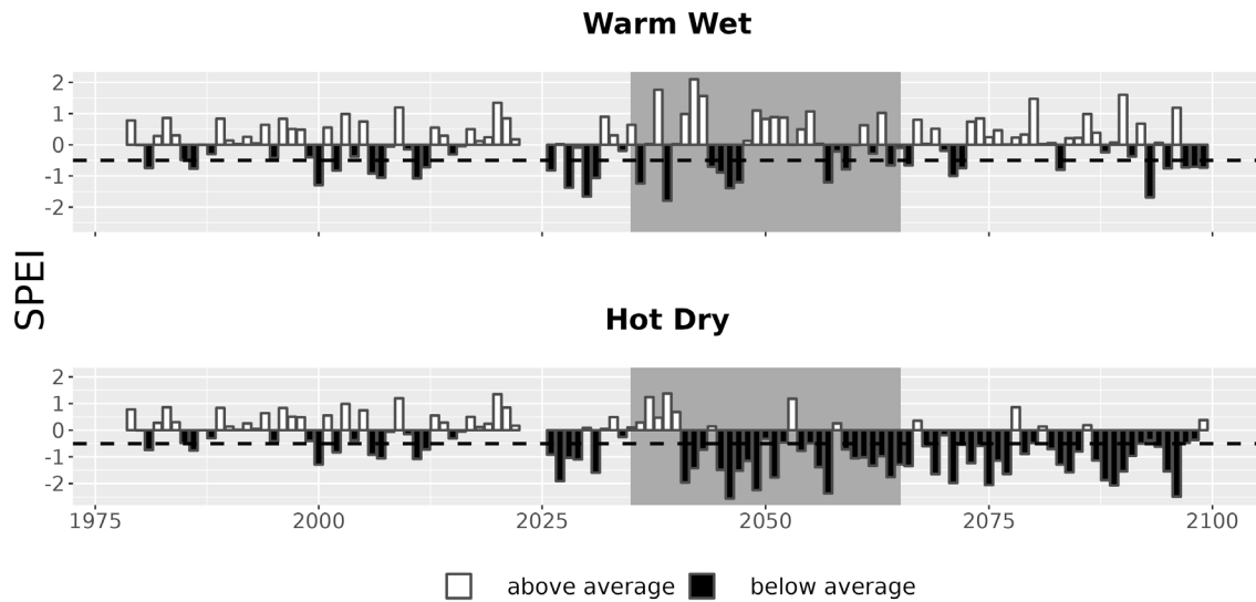
Figure 7. Drought metrics for TUIN. Drought index (SPEI; units = standard deviations from historical) timeseries for each climate future. Below-average SPEI (black bars) indicates dry conditions. The dotted line (SPEI = -0.5) indicates drought conditions.
