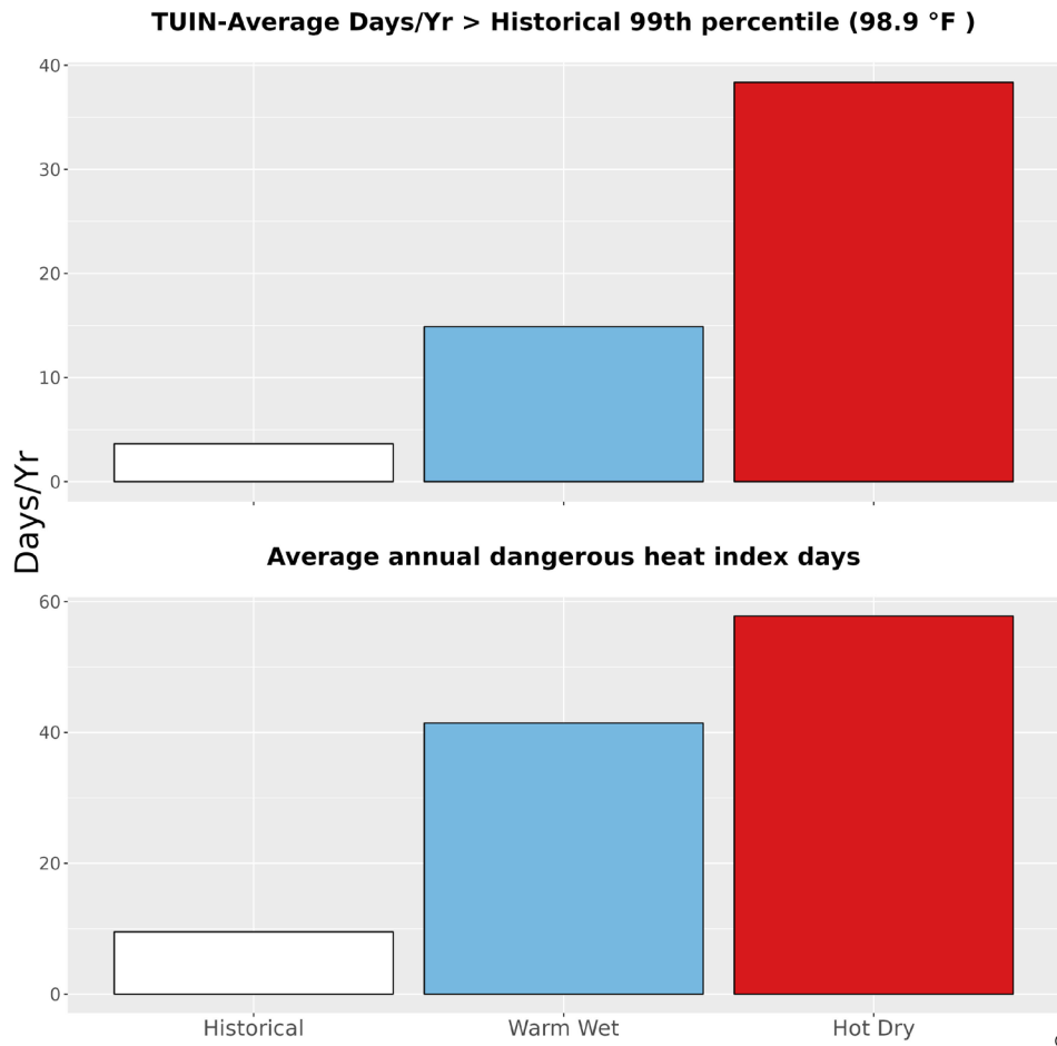
Figure 5. The upper bar graph represents the average number of days annually with temperatures greater than the historical 99th percentile (98.9 °F) historically (1979-2012) and for the two climate futures (2050). The bottom bar graph represents the average annual number of dangerous heat index days historically and for the two climate futures. Dangerous heat index days are days that exceed 105 °F.
