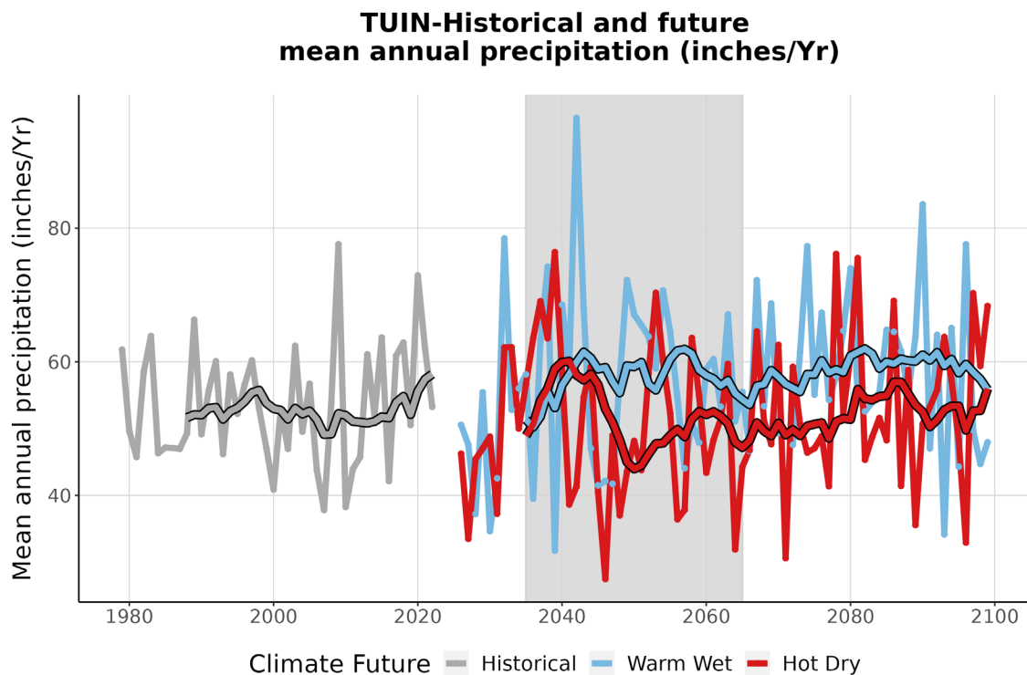
Figure 4. This graph compares observed average annual precipitation at TUIN (inches/year) (1979-2022) with projected average annual precipitation for the two climate futures over the period 2023-2099. The historically observed data is shown in gray, the Warm Wet climate future in blue, and the Hot Dry climate future in red. The smooth line running through each projection is the 10-year running average for historical observations and future projections. The gray-shaded area represents the time period that was averaged (2035-2065) to summarize future projections for the year 2050 (Appendix 1).
