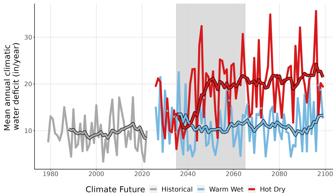
Figure 9. This line graph compares observed climatic water deficit at TUIN (inches/year) (1979-2022) with projected climatic water deficit for the two climate futures over the period 2023-2099. The historical observation data is shown in gray, the Warm Wet climate future in blue, and the Hot Dry climate future in red. The smooth line running through each projection is the 10-year running average for historical observations and future projections. Gray-shaded area represents the time period that was averaged (2035-2065) to summarize future projections for the year 2050.
