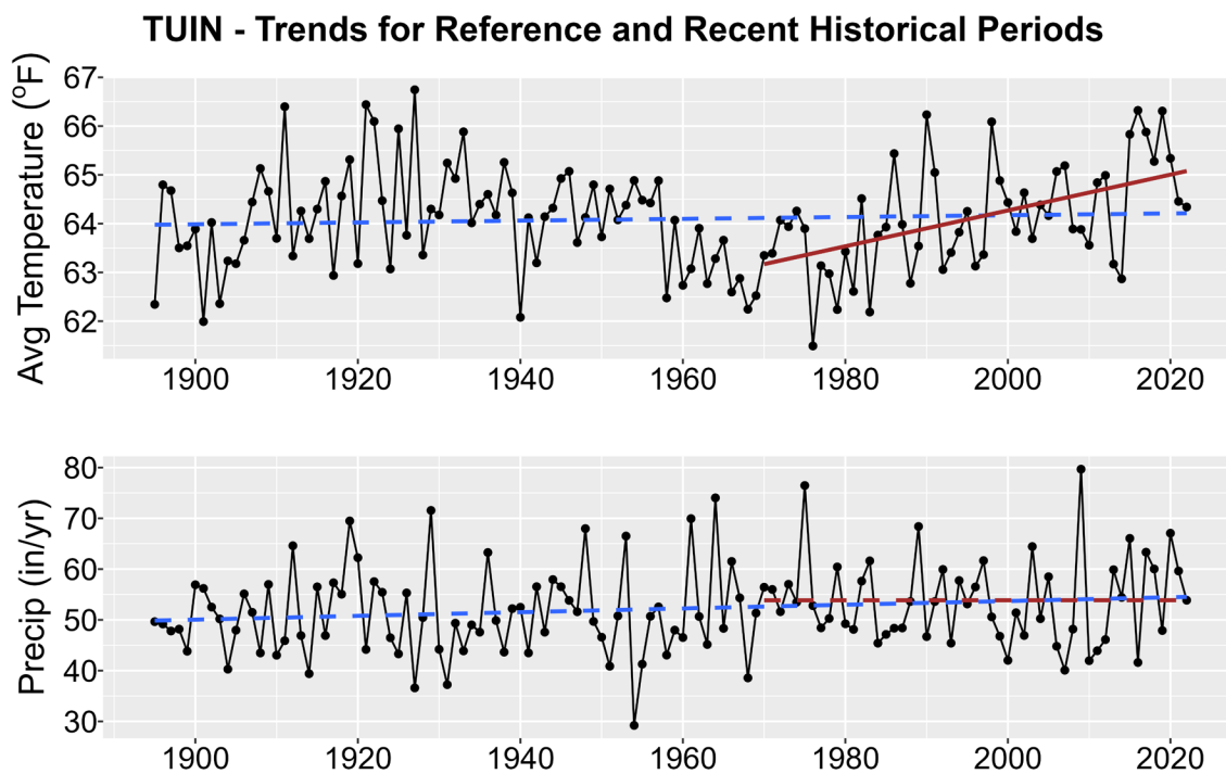
Figure 1. Historical trends in annual average temperature (upper plot) and annual total precipitation (lower plot) for TUIN from 1895-2022. Black points show yearly values while blue lines are linear regressions for the entire period record and red lines for 1970-2022 trends. Solid lines are significant trends (i.e., p < 0.05 ); dashed lines are not statistically significant.
