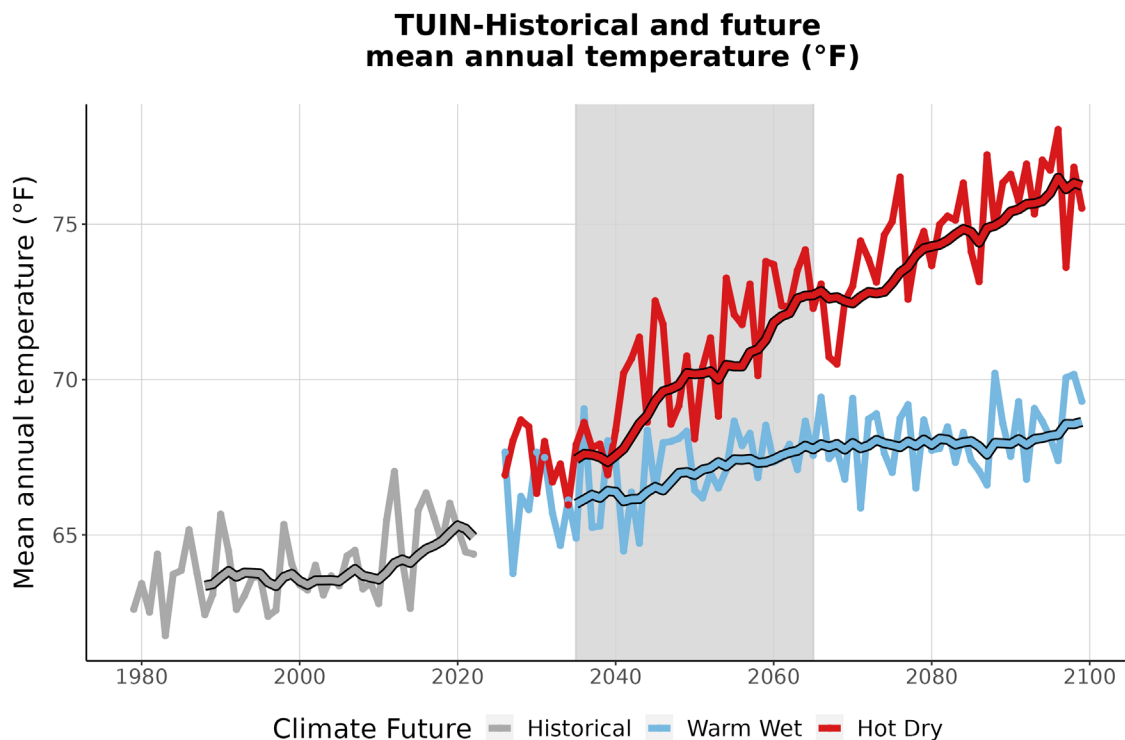
Figure 3. This graph compares observed average annual temperature at TUIN (°F) (1979-2022) with projected average annual temperature for the two climate futures over the period 2023-2099. The historically observed data
