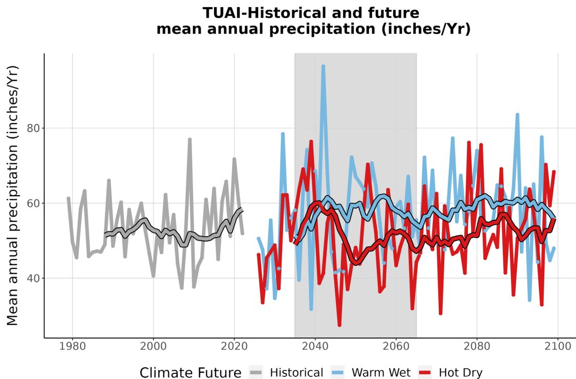
Figure 4. This graph compares observed average annual precipitation at TUAI (inches/year) (1979-2022) with projected average annual precipitation for the two climate futures over the period 2023-2099. The historically observed data is shown in gray, the Warm Wet climate future in blue, and the Hot Dry climate future in red. The smooth line running through each projection is the 10-year running average for historical observations and future projections. The gray-shaded area represents the time period that was averaged (2035-2065) to summarize future projections for the year 2050 (Appendix 1).
