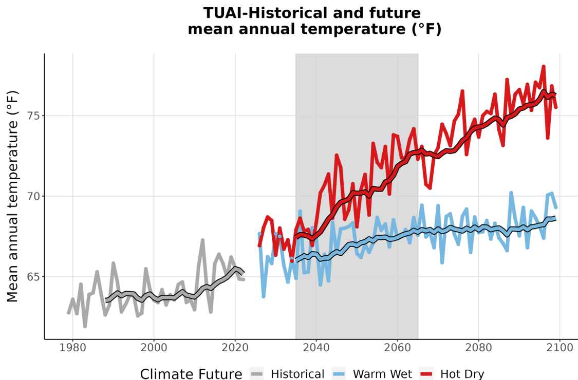
Figure 3. This graph compares observed average annual temperature at TUAI (°F) (1979-2022) with projected average annual temperature for the two climate futures over the period 2023-2099. The historically observed data
