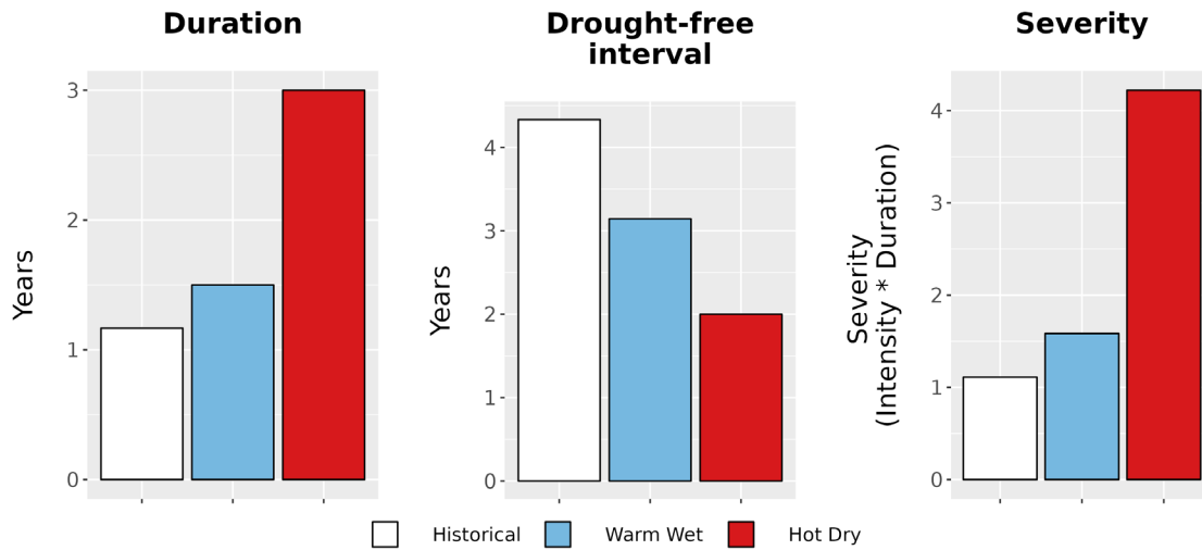
Figure 8. Drought metrics for TUAI. (Left) Average drought duration (years) historically (1979-2012) and under each climate future. (Middle) Average drought return interval (years), indicating the expected amount of time between periods of drought, historically and under each climate future. (Right) Average drought severity, a measure of drought intensity multiplied by duration, historically and under each climate future.
