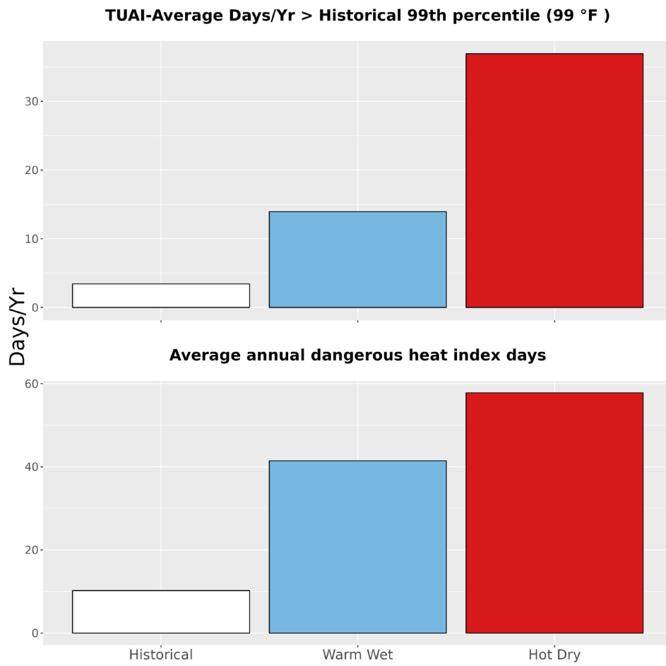
Figure 5. The upper bar graph represents the average number of days annually with temperatures greater than the historical 99th percentile (99 °F) historically (1979-2012) and for the two climate futures (2050). The bottom bar graph represents the average annual number of dangerous heat index days historically and for the two climate futures. Dangerous heat index days are days that exceed 105 °F.
