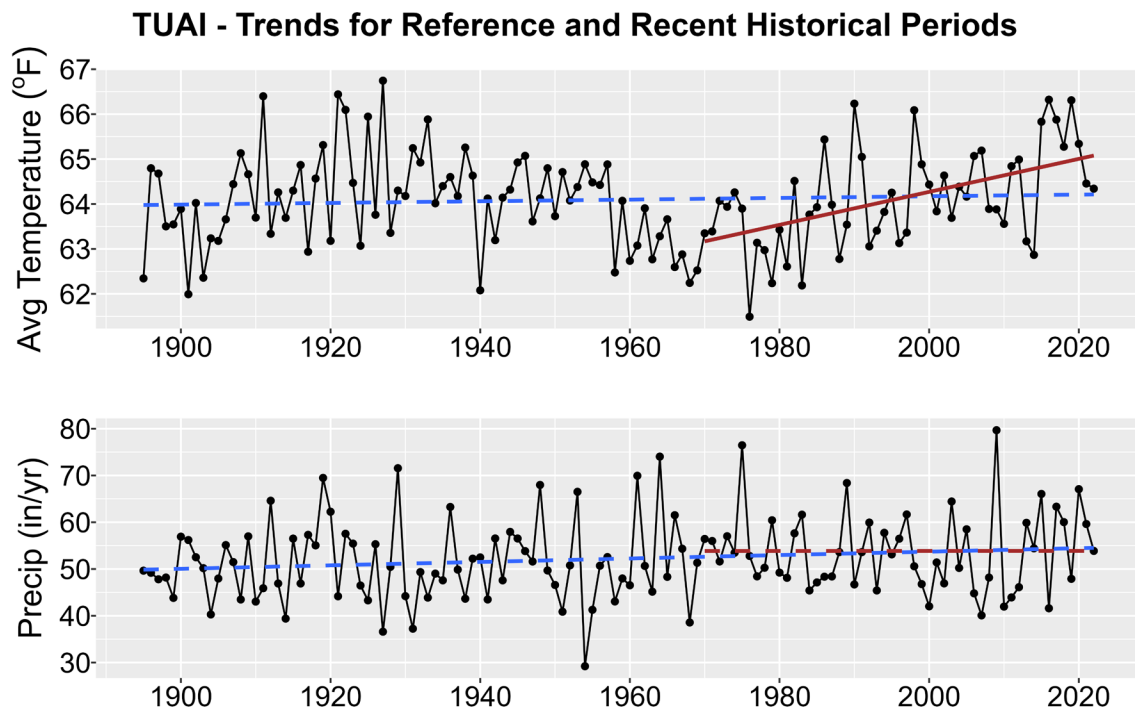
Figure 1. Historical trends in annual average temperature (upper plot) and annual total precipitation (lower plot) for TUAI from 1895-2022. Black points show yearly values while blue lines are linear regressions for the entire period record and red lines for 1970-2022 trends. Solid lines are significant trends (i.e., p < 0.05 ); dashed lines are not statistically significant.
