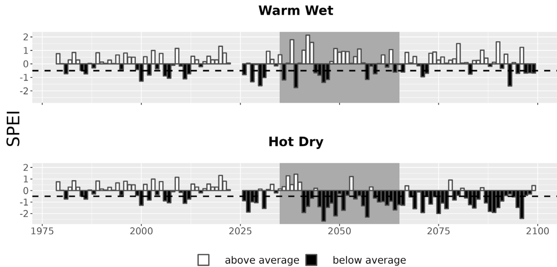
Figure 7. Drought metrics for TUAI. Drought index (SPEI; units = standard deviations from historical) timeseries for each climate future. Below-average SPEI (black bars) indicates dry conditions. The dotted line (SPEI = -0.5) indicates drought conditions.
