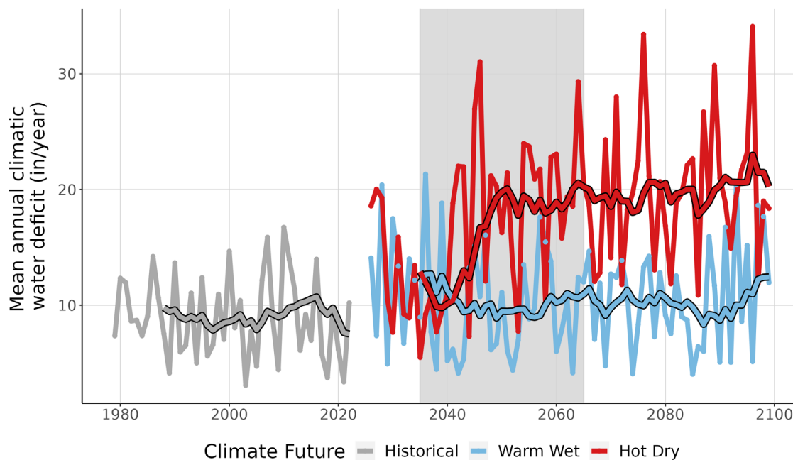
Figure 9. This line graph compares observed climatic water deficit at TUAI (inches/year) (1979-2022) with projected climatic water deficit for the two climate futures over the period 2023-2099. The historical observation data is shown in gray, the Warm Wet climate future in blue, and the Hot Dry climate future in red. The smooth line running through each projection is the 10-year running average for historical observations and future projections. Gray-shaded area represents the time period that was averaged (2035-2065) to summarize future projections for the year 2050.
