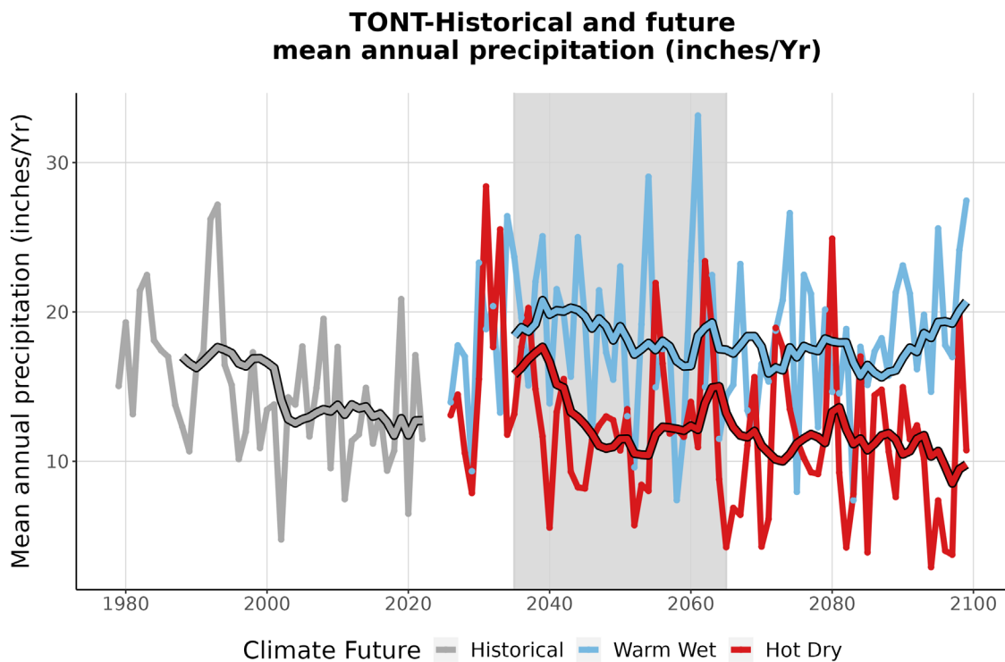
Figure 4. This graph compares observed average annual precipitation at TONT (inches/year) (1979-2022) with projected average annual precipitation for the two climate futures over the period 2023-2099. The historically observed data is shown in gray, the Warm Wet climate future in blue, and the Hot Dry climate future in red. The smooth line running through each projection is the 10-year running average for historical observations and future projections. The gray-shaded area represents the time period that was averaged (2035-2065) to summarize future projections for the year 2050 (Appendix 1).
