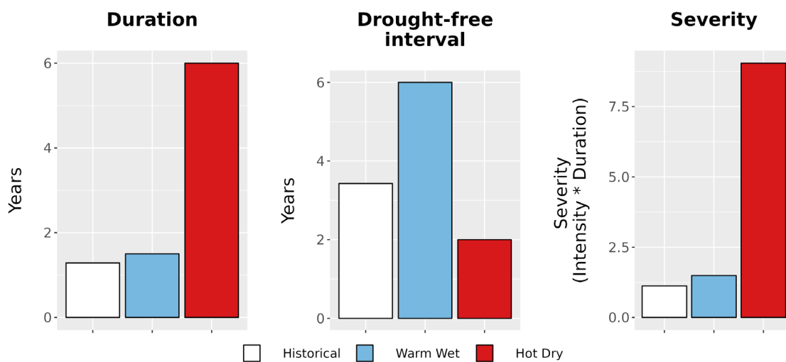
Figure 8. Drought metrics for TONT. (Left) Average drought duration (years) historically (1979-2012) and under each climate future. (Middle) Average drought return interval (years), indicating the expected amount of time between periods of drought, historically and under each climate future. (Right) Average drought severity, a measure of drought intensity multiplied by duration, historically and under each climate future.
