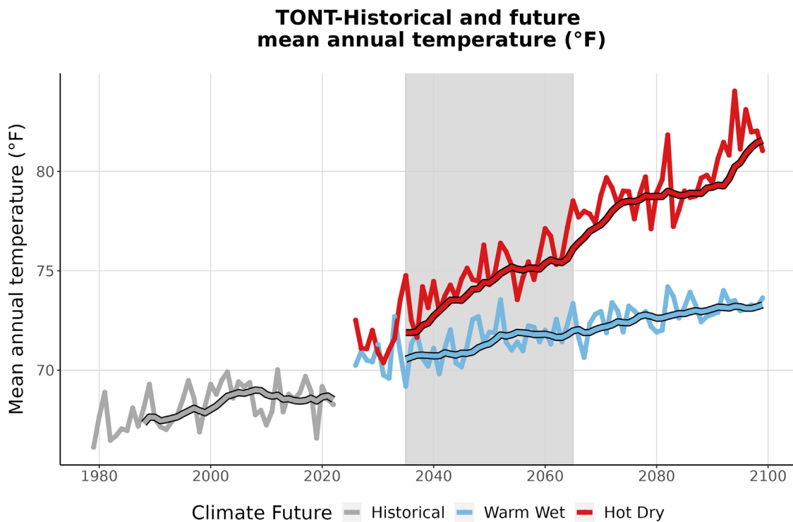
Figure 3. This graph compares observed average annual temperature at TONT (°F) (1979-2022) with projected average annual temperature for the two climate futures over the period 2023-2099. The historically observed data is shown in gray, the Warm Wet climate future in blue, and the Hot Dry climate future in red. The smooth line
