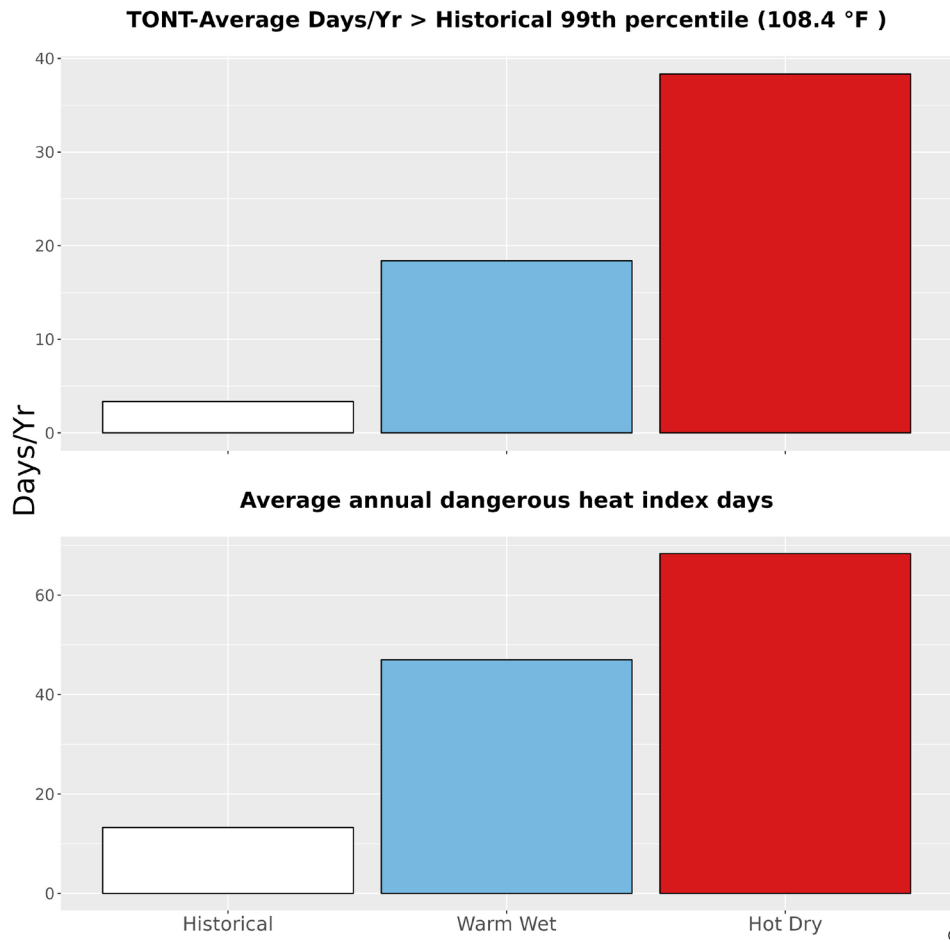
Figure 5. The upper bar graph represents the average number of days annually with temperatures greater than the historical 99th percentile (108.4 °F) historically (1979-2012) and for the two climate futures (2050). The bottom bar graph represents the average annual number of dangerous heat index days historically and for the two climate futures. Dangerous heat index days are days that exceed 105 °F.
