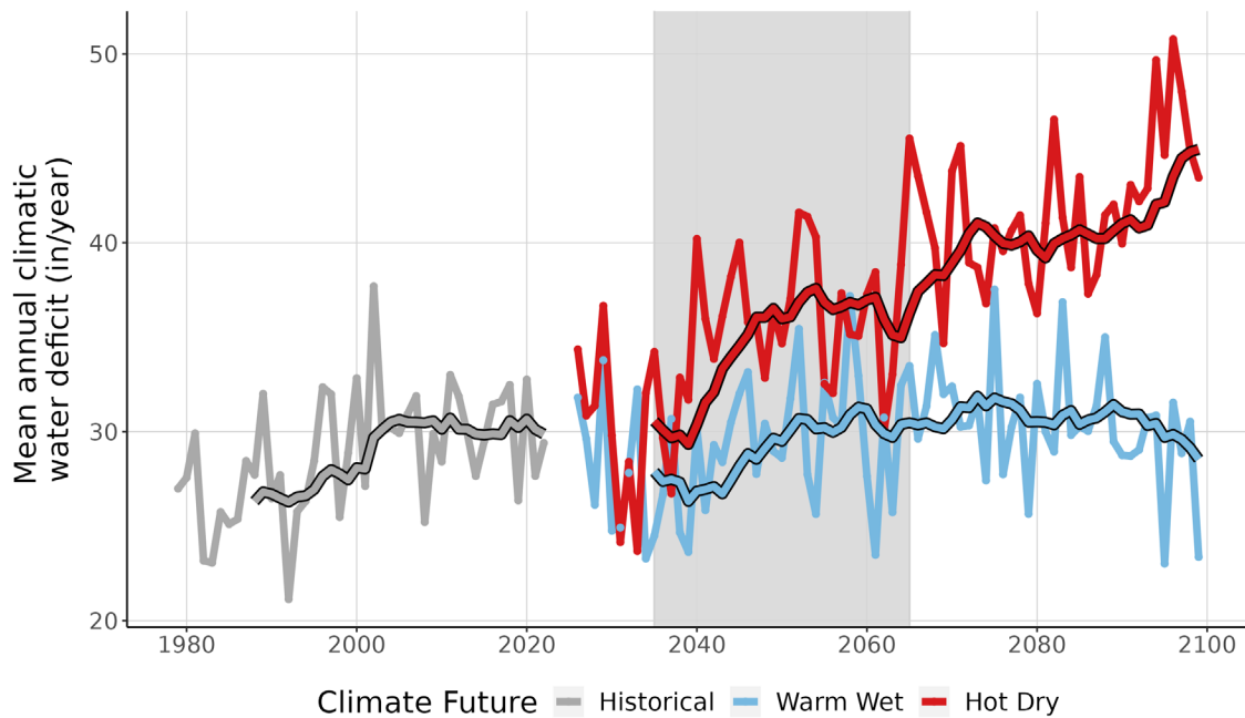
Figure 9. This line graph compares observed climatic water deficit at TONT (inches/year) (1979-2022) with projected climatic water deficit for the two climate futures over the period 2023-2099. The historical observation data is shown in gray, the Warm Wet climate future in blue, and the Hot Dry climate future in red. The smooth line running through each projection is the 10-year running average for historical observations and future projections. Gray-shaded area represents the time period that was averaged (2035-2065) to summarize future projections for the year 2050.
