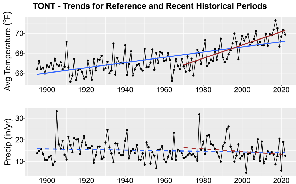
Figure 1. Historical trends in annual average temperature (upper plot) and annual total precipitation (lower plot) for TONT from 1895-2022. Black points show yearly values while blue lines are linear regressions for the entire period record and red lines for 1970-2022 trends. Solid lines are significant trends (i.e., p < 0.05 ); dashed lines are not statistically significant.
