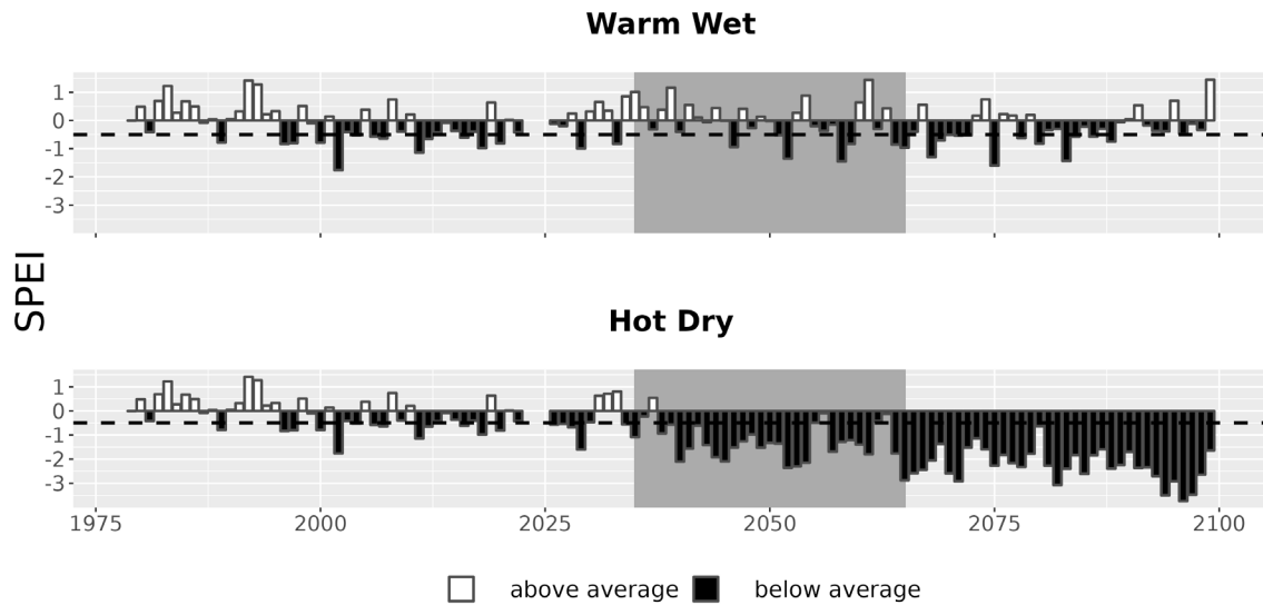
Figure 7. Drought metrics for TONT. Drought index (SPEI; units = standard deviations from historical) timeseries for each climate future. Below-average SPEI (black bars) indicates dry conditions. The dotted line (SPEI = -0.5) indicates drought conditions.
