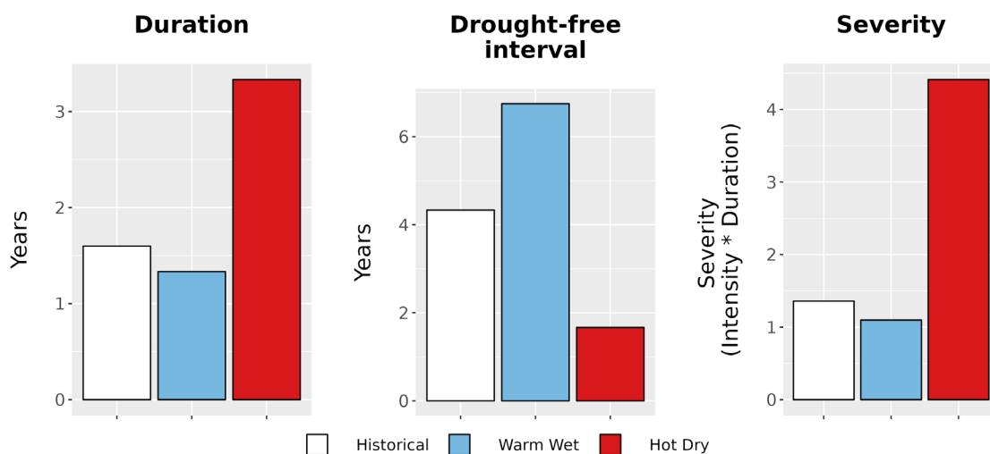
Figure 8. Drought metrics for TIMU. (Left) Average drought duration (years) historically (1979-2012) and under each climate future. (Middle) Average drought return interval (years), indicating the expected amount of time between periods of drought, historically and under each climate future. (Right) Average drought severity, a measure of drought intensity multiplied by duration, historically and under each climate future.
