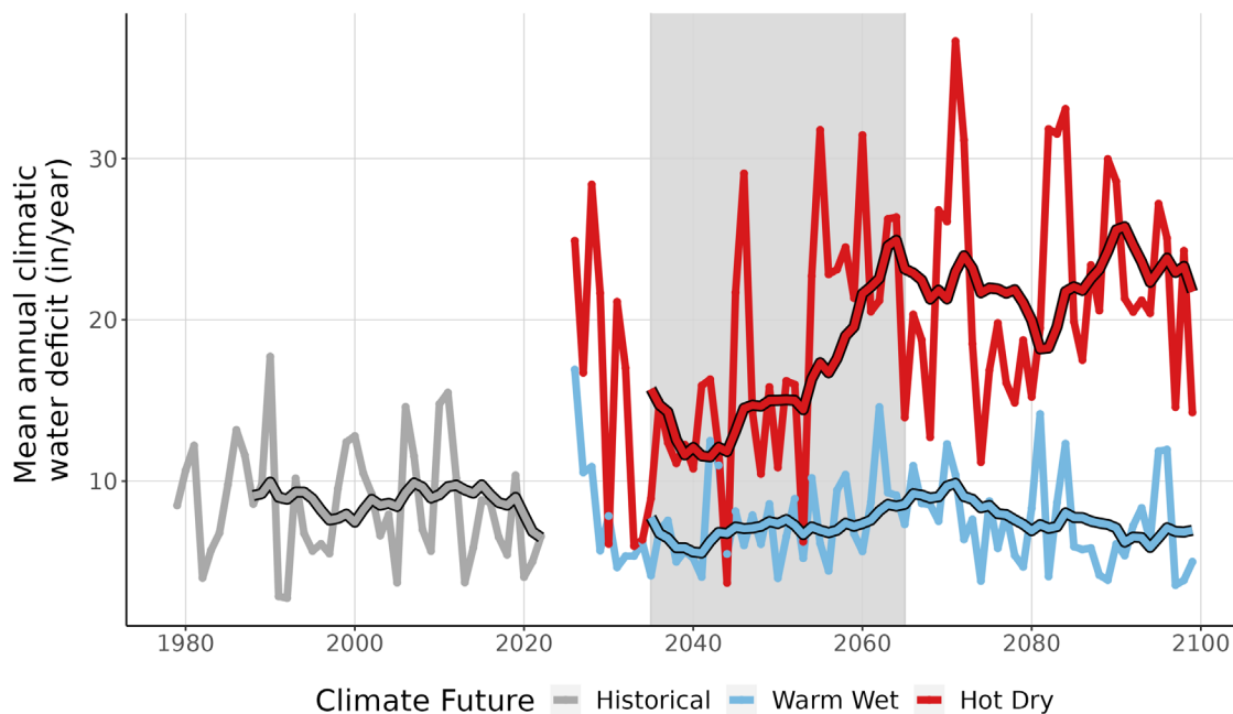
Figure 9. This line graph compares observed climatic water deficit at TIMU (inches/year) (1979-2022) with projected climatic water deficit for the two climate futures over the period 2023-2099. The historical observation data is shown in gray, the Warm Wet climate future in blue, and the Hot Dry climate future in red. The smooth line running through each projection is the 10-year running average for historical observations and future projections. Gray-shaded area represents the time period that was averaged (2035-2065) to summarize future projections for the year 2050.
