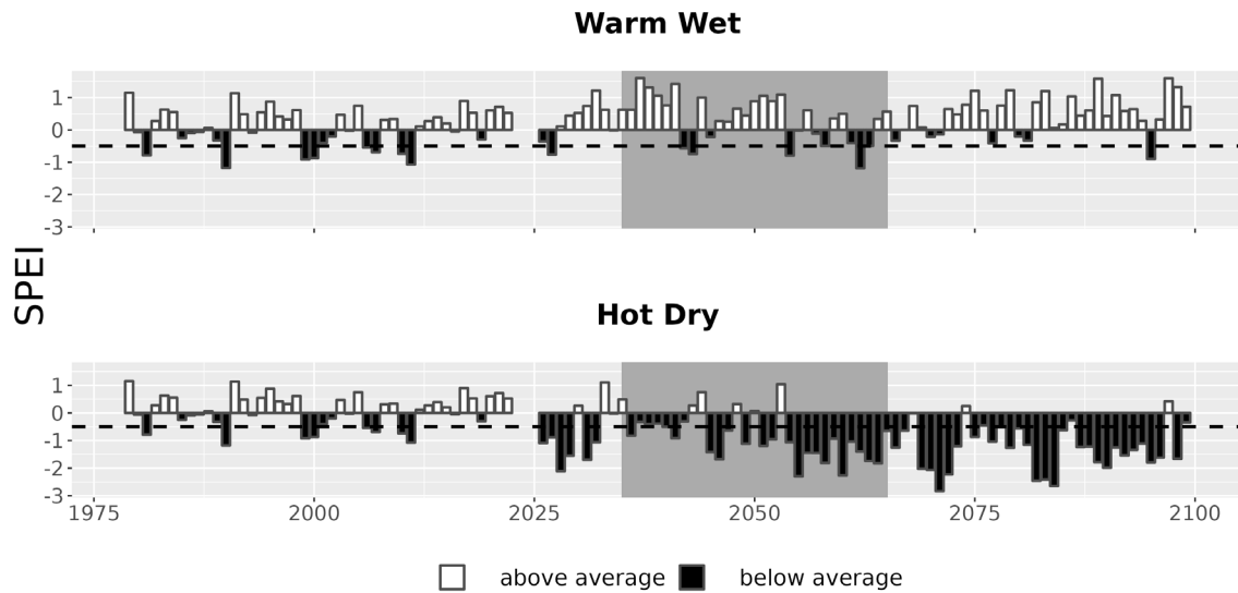
Figure 7. Drought metrics for TIMU. Drought index (SPEI; units = standard deviations from historical) timeseries for each climate future. Below-average SPEI (black bars) indicates dry conditions. The dotted line (SPEI = -0.5) indicates drought conditions.
