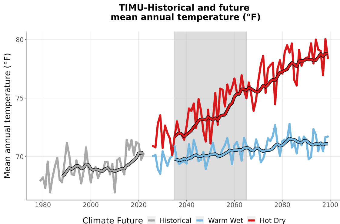
Figure 3. This graph compares observed average annual temperature at TIMU (°F) (1979-2022) with projected average annual temperature for the two climate futures over the period 2023-2099. The historically observed data
