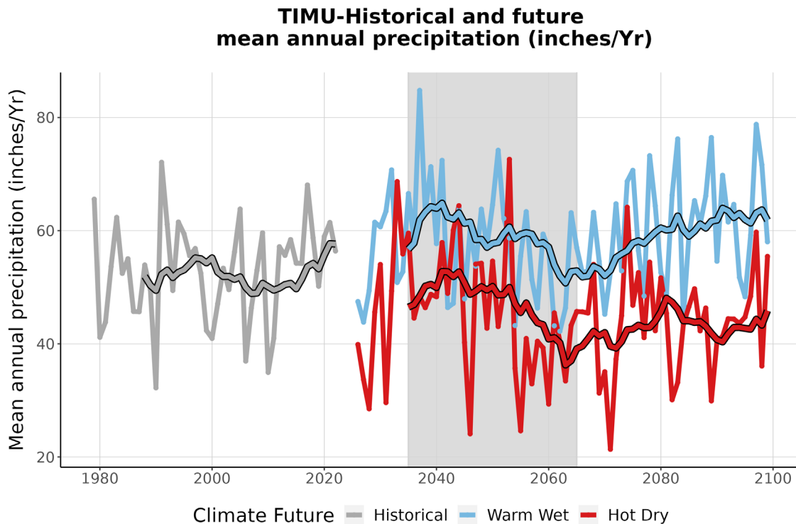
Figure 4. This graph compares observed average annual precipitation at TIMU (inches/year) (1979-2022) with projected average annual precipitation for the two climate futures over the period 2023-2099. The historically observed data is shown in gray, the Warm Wet climate future in blue, and the Hot Dry climate future in red. The smooth line running through each projection is the 10-year running average for historical observations and future projections. The gray-shaded area represents the time period that was averaged (2035-2065) to summarize future projections for the year 2050 (Appendix 1).
