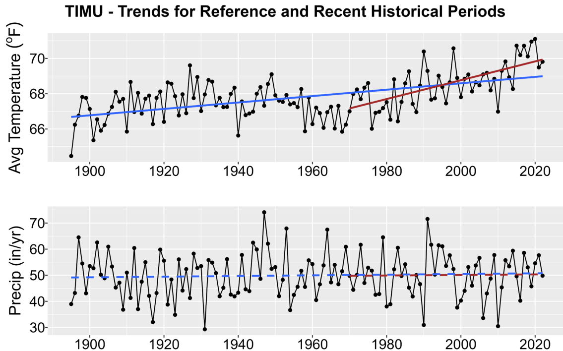
Figure 1. Historical trends in annual average temperature (upper plot) and annual total precipitation (lower plot) for TIMU from 1895-2022. Black points show yearly values while blue lines are linear regressions for the entire period record and red lines for 1970-2022 trends. Solid lines are significant trends (i.e., p < 0.05 ); dashed lines are not statistically significant.
