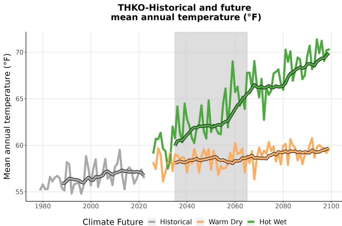
Figure 3. This graph compares observed average annual temperature at THKO (°F) (1979-2022) with projected average annual temperature for the two climate futures over the period 2023-2099. The historically observed data is shown in gray, the Warm Dry climate future in orange, and the Hot Wet climate future in green. The smooth line
