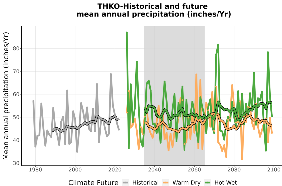
Figure 4. This graph compares observed average annual precipitation at THKO (inches/year) (1979-2022) with projected average annual precipitation for the two climate futures over the period 2023-2099. The historically observed data is shown in gray, the Warm Dry climate future in orange, and the Hot Wet climate future in green. The smooth line running through each projection is the 10-year running average for historical observations and future projections. The gray-shaded area represents the time period that was averaged (2035-2065) to summarize future projections for the year 2050 (Appendix 1).
