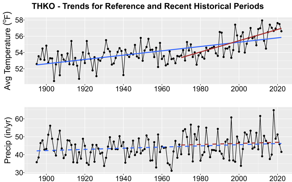
Figure 1. Historical trends in annual average temperature (upper plot) and annual total precipitation (lower plot) for THKO from 1895-2022. Black points show yearly values while blue lines are linear regressions for the entire period record and red lines for 1970-2022 trends. Solid lines are significant trends (i.e., p < 0.05 ); dashed lines are not statistically significant.
