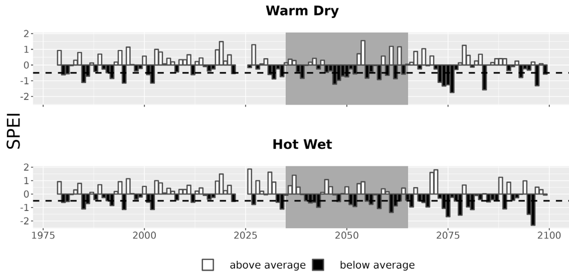
Figure 7. Drought metrics for THKO. Drought index (SPEI; units = standard deviations from historical) timeseries for each climate future. Below-average SPEI (black bars) indicates dry conditions. The dotted line (SPEI = -0.5) indicates drought conditions.
