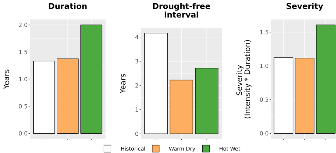
Figure 8. Drought metrics for THKO. (Left) Average drought duration (years) historically (1979-2012) and under each climate future. (Middle) Average drought return interval (years), indicating the expected amount of time between periods of drought, historically and under each climate future. (Right) Average drought severity, a measure of drought intensity multiplied by duration, historically and under each climate future.
