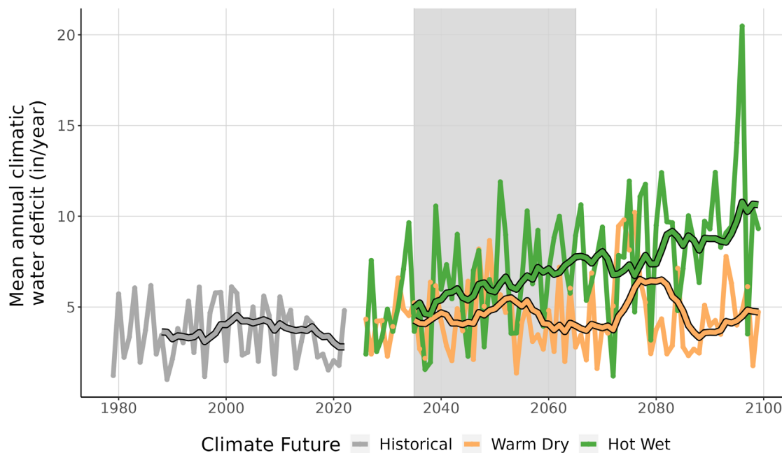
Figure 9. This line graph compares observed climatic water deficit at THKO (inches/year) (1979-2022) with projected climatic water deficit for the two climate futures over the period 2023-2099. The historical observation data is shown in gray, the Warm Dry climate future in orange, and the Hot Wet climate future in green. The smooth line running through each projection is the 10-year running average for historical observations and future projections. Gray-shaded area represents the time period that was averaged (2035-2065) to summarize future projections for the year 2050.
