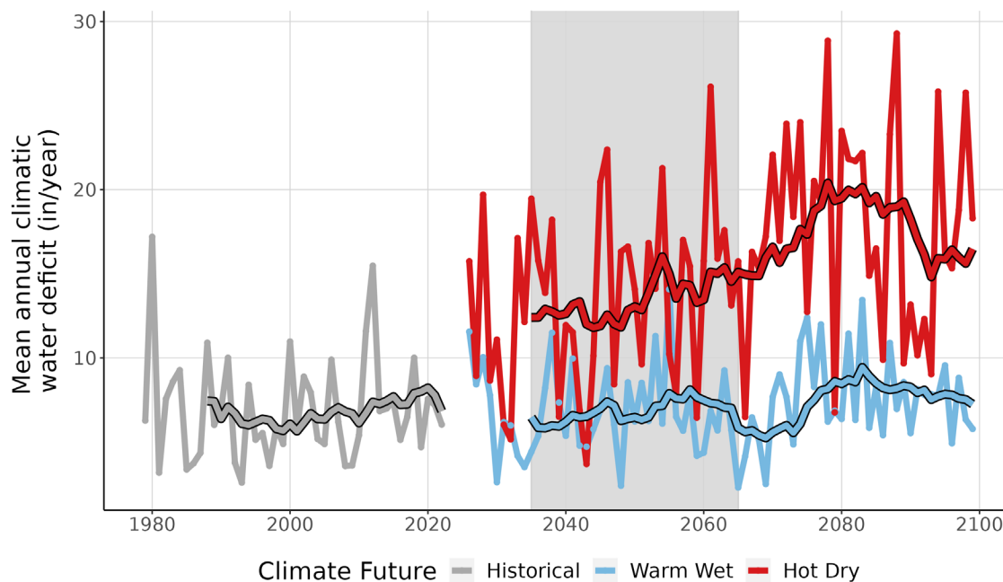
Figure 9. This line graph compares observed climatic water deficit at TAPR (inches/year) (1979-2022) with projected climatic water deficit for the two climate futures over the period 2023-2099. The historical observation data is shown in gray, the Warm Wet climate future in blue, and the Hot Dry climate future in red. The smooth line running through each projection is the 10-year running average for historical observations and future projections. Gray-shaded area represents the time period that was averaged (2035-2065) to summarize future projections for the year 2050.
