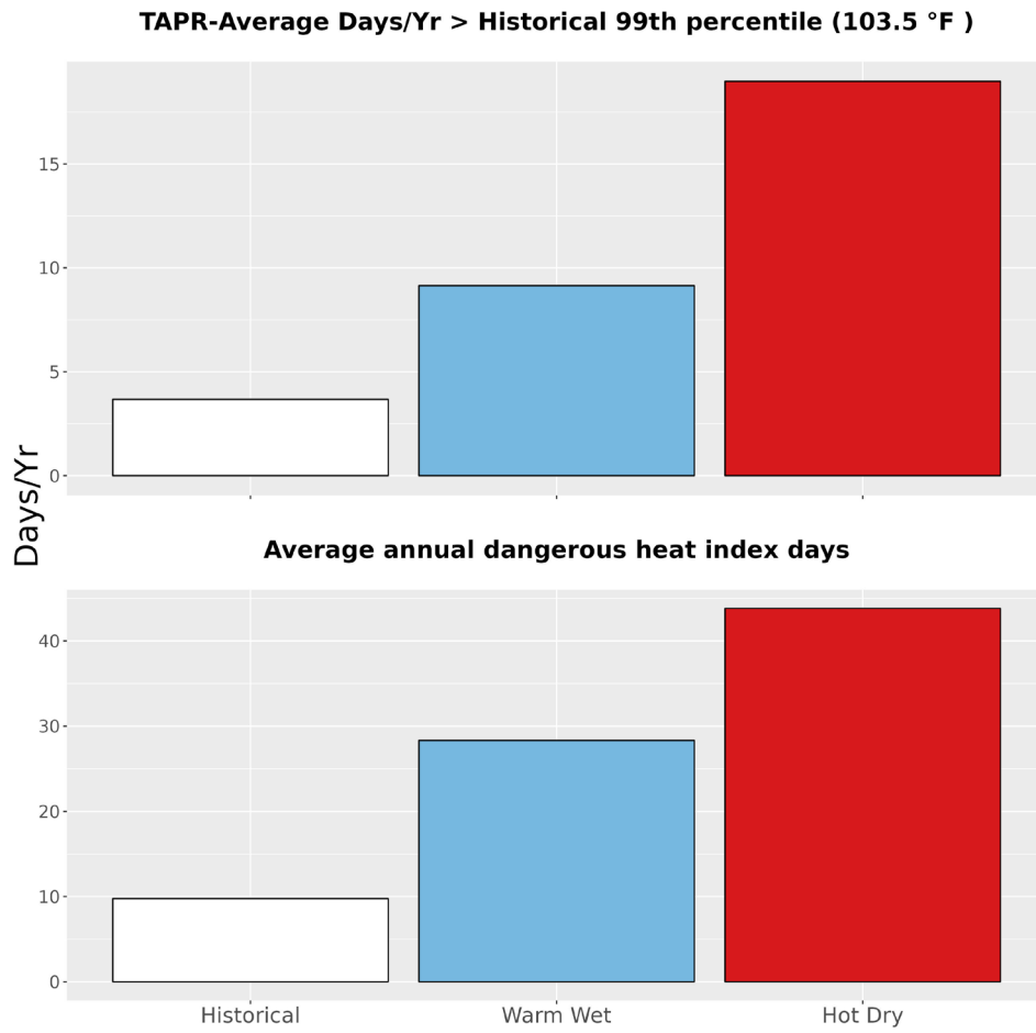
Figure 5. The upper bar graph represents the average number of days annually with temperatures greater than the historical 99th percentile (103.5 °F) historically (1979-2012) and for the two climate futures (2050). The bottom bar graph represents the average annual number of dangerous heat index days historically and for the two climate futures. Dangerous heat index days are days that exceed 105 °F.
