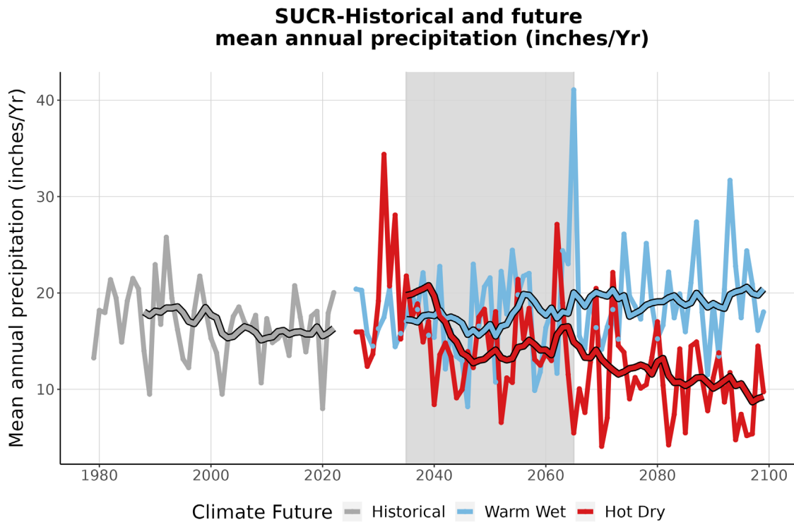
Figure 4. This graph compares observed average annual precipitation at SUCR (inches/year) (1979-2022) with projected average annual precipitation for the two climate futures over the period 2023-2099. The historically observed data is shown in gray, the Warm Wet climate future in blue, and the Hot Dry climate future in red. The smooth line running through each projection is the 10-year running average for historical observations and future projections. The gray-shaded area represents the time period that was averaged (2035-2065) to summarize future projections for the year 2050 (Appendix 1).
