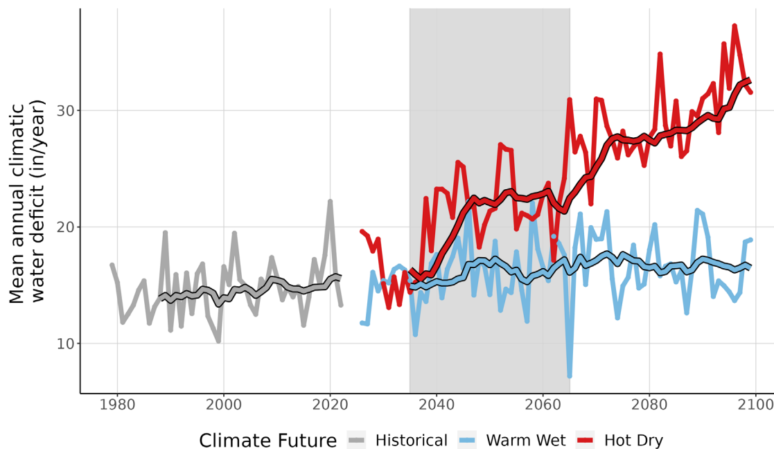
Figure 9. This line graph compares observed climatic water deficit at SUCR (inches/year) (1979-2022) with projected climatic water deficit for the two climate futures over the period 2023-2099. The historical observation data is shown in gray, the Warm Wet climate future in blue, and the Hot Dry climate future in red. The smooth line running through each projection is the 10-year running average for historical observations and future projections. Gray-shaded area represents the time period that was averaged (2035-2065) to summarize future projections for the year 2050.
