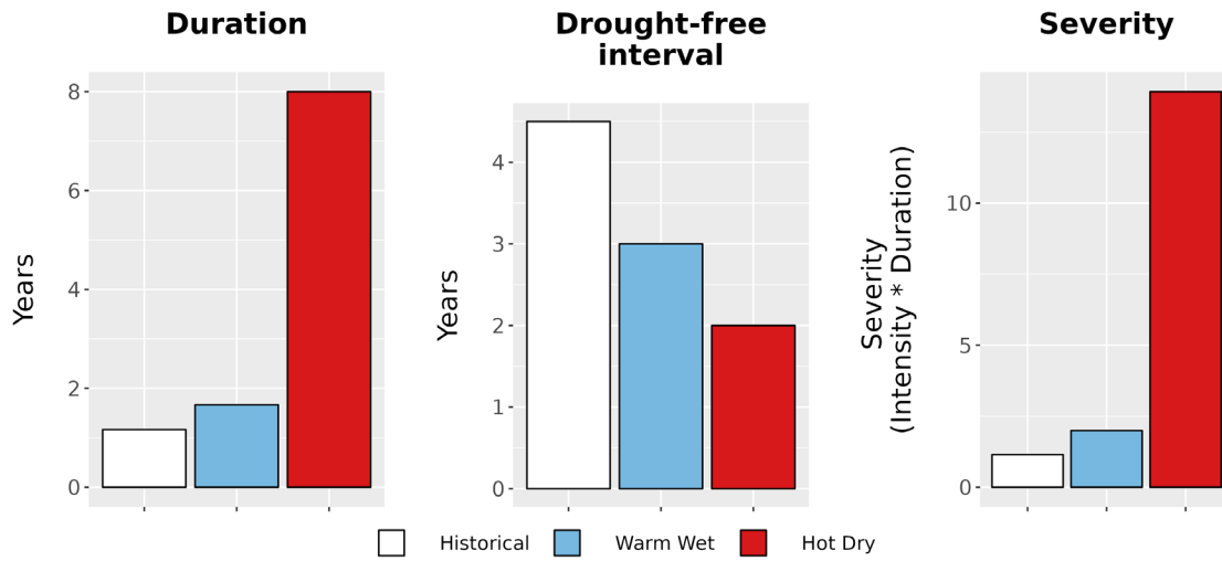
Figure 8. Drought metrics for SUCR. (Left) Average drought duration (years) historically (1979-2012) and under each climate future. (Middle) Average drought return interval (years), indicating the expected amount of time between periods of drought, historically and under each climate future. (Right) Average drought severity, a measure of drought intensity multiplied by duration, historically and under each climate future.
