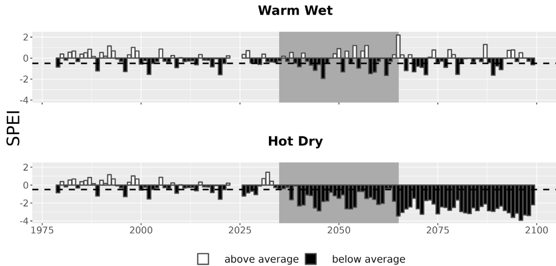
Figure 7. Drought metrics for SUCR. Drought index (SPEI; units = standard deviations from historical) timeseries for each climate future. Below-average SPEI (black bars) indicates dry conditions. The dotted line (SPEI = -0.5) indicates drought conditions.
