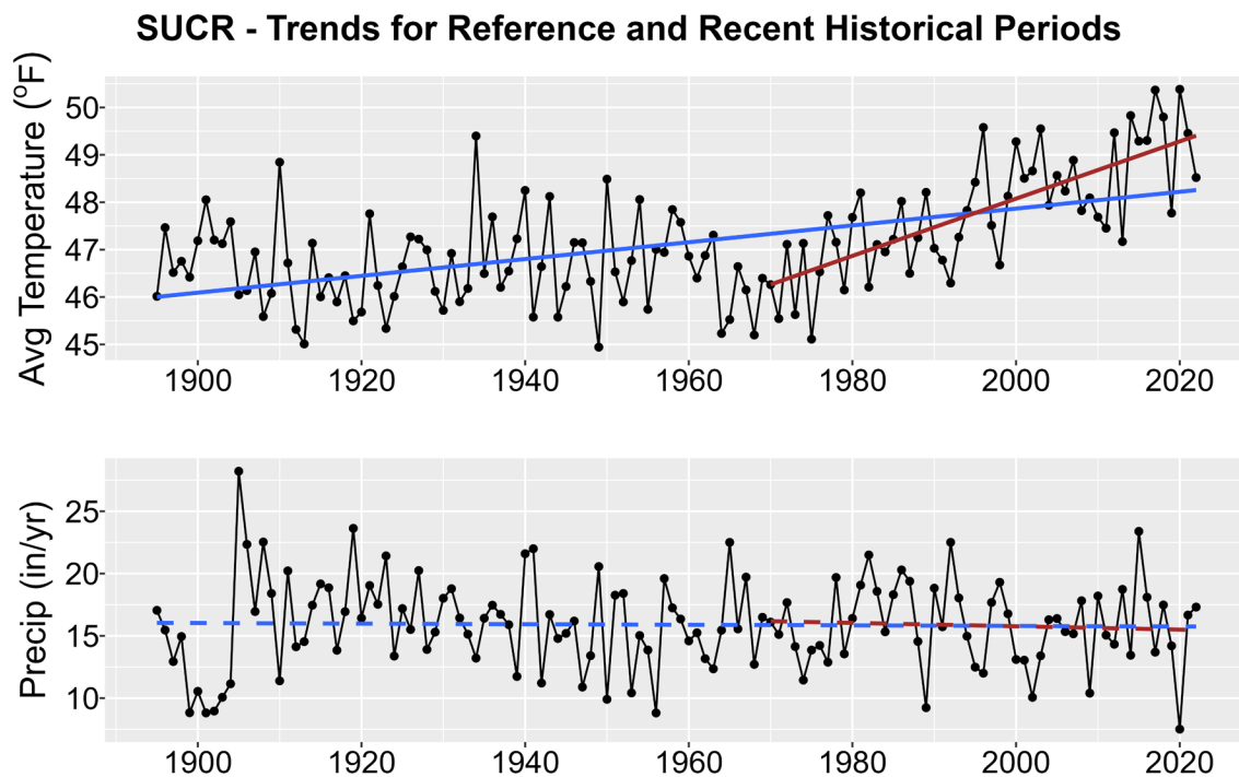
Figure 1. Historical trends in annual average temperature (upper plot) and annual total precipitation (lower plot) for SUCR from 1895-2022. Black points show yearly values while blue lines are linear regressions for the entire period record and red lines for 1970-2022 trends. Solid lines are significant trends (i.e., p < 0.05 ); dashed lines are not statistically significant.
