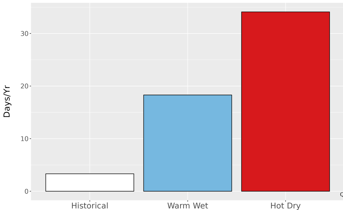
Figure 5. Metrics of extreme temperature at SUCR. The bar graph represents the average number of days annually with temperatures greater than the historical 99th percentile (90.9 °F) historically (1979-2012) and for the two climate futures (2050).
