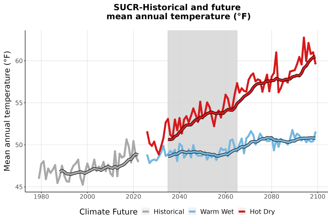
Figure 3. This graph compares observed average annual temperature at SUCR (°F) (1979-2022) with projected average annual temperature for the two climate futures over the period 2023-2099. The historically observed data
