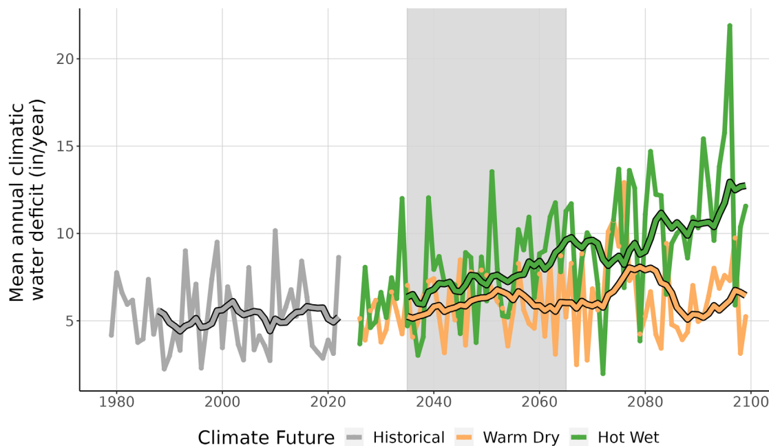
Figure 9. This line graph compares observed climatic water deficit at STLI (inches/year) (1979-2022) with projected climatic water deficit for the two climate futures over the period 2023-2099. The historical observation data is shown in gray, the Warm Dry climate future in orange, and the Hot Wet climate future in green. The smooth line running through each projection is the 10-year running average for historical observations and future projections. Gray-shaded area represents the time period that was averaged (2035-2065) to summarize future projections for the year 2050.
