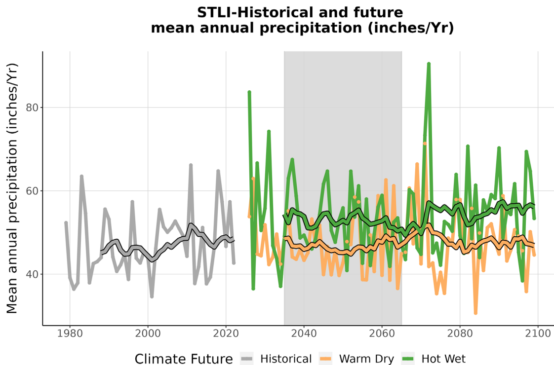
Figure 4. This graph compares observed average annual precipitation at STLI (inches/year) (1979-2022) with projected average annual precipitation for the two climate futures over the period 2023-2099. The historically observed data is shown in gray, the Warm Dry climate future in orange, and the Hot Wet climate future in green. The smooth line running through each projection is the 10-year running average for historical observations and future projections. The gray-shaded area represents the time period that was averaged (2035-2065) to summarize future projections for the year 2050 (Appendix 1).
