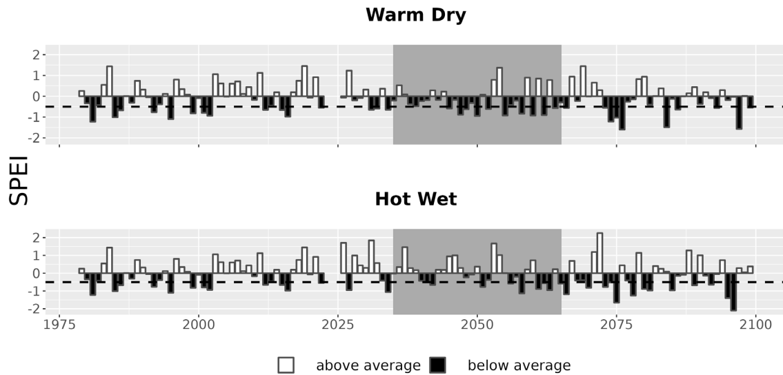
Figure 7. Drought metrics for STLI. Drought index (SPEI; units = standard deviations from historical) timeseries for each climate future. Below-average SPEI (black bars) indicates dry conditions. The dotted line (SPEI = -0.5) indicates drought conditions.
