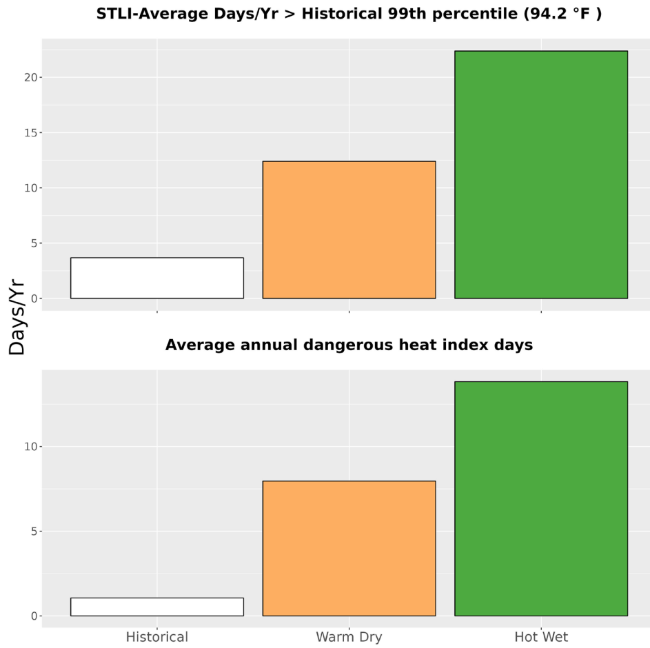
Figure 5. The upper bar graph represents the average number of days annually with temperatures greater than the historical 99th percentile (94.2 °F) historically (1979-2012) and for the two climate futures (2050). The bottom bar graph represents the average annual number of dangerous heat index days historically and for the two climate futures. Dangerous heat index days are days that exceed 105 °F.
