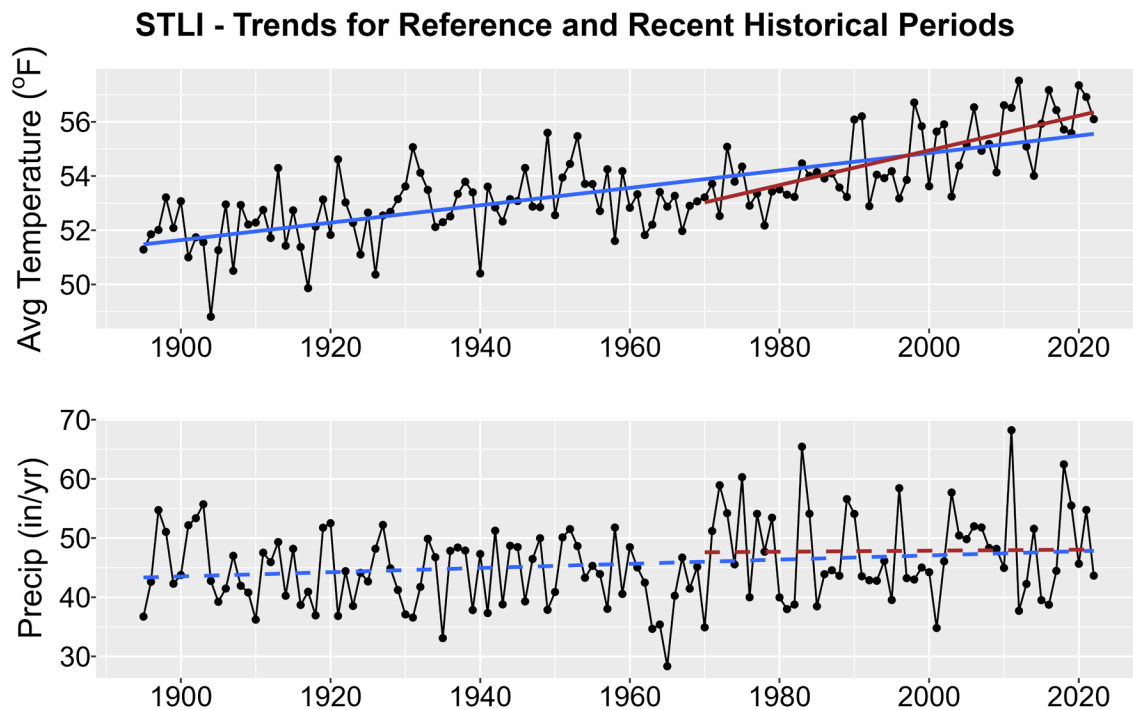
Figure 1. Historical trends in annual average temperature (upper plot) and annual total precipitation (lower plot) for STLI from 1895-2022. Black points show yearly values while blue lines are linear regressions for the entire period record and red lines for 1970-2022 trends. Solid lines are significant trends (i.e., p < 0.05 ); dashed lines are not statistically significant.
