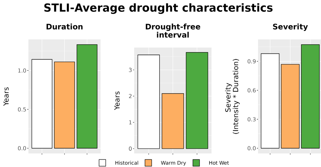
Figure 8. Drought metrics for STLI. (Left) Average drought duration (years) historically (1979-2012) and under each climate future. (Middle) Average drought return interval (years), indicating the expected amount of time between periods of drought, historically and under each climate future. (Right) Average drought severity, a measure of drought intensity multiplied by duration, historically and under each climate future.
