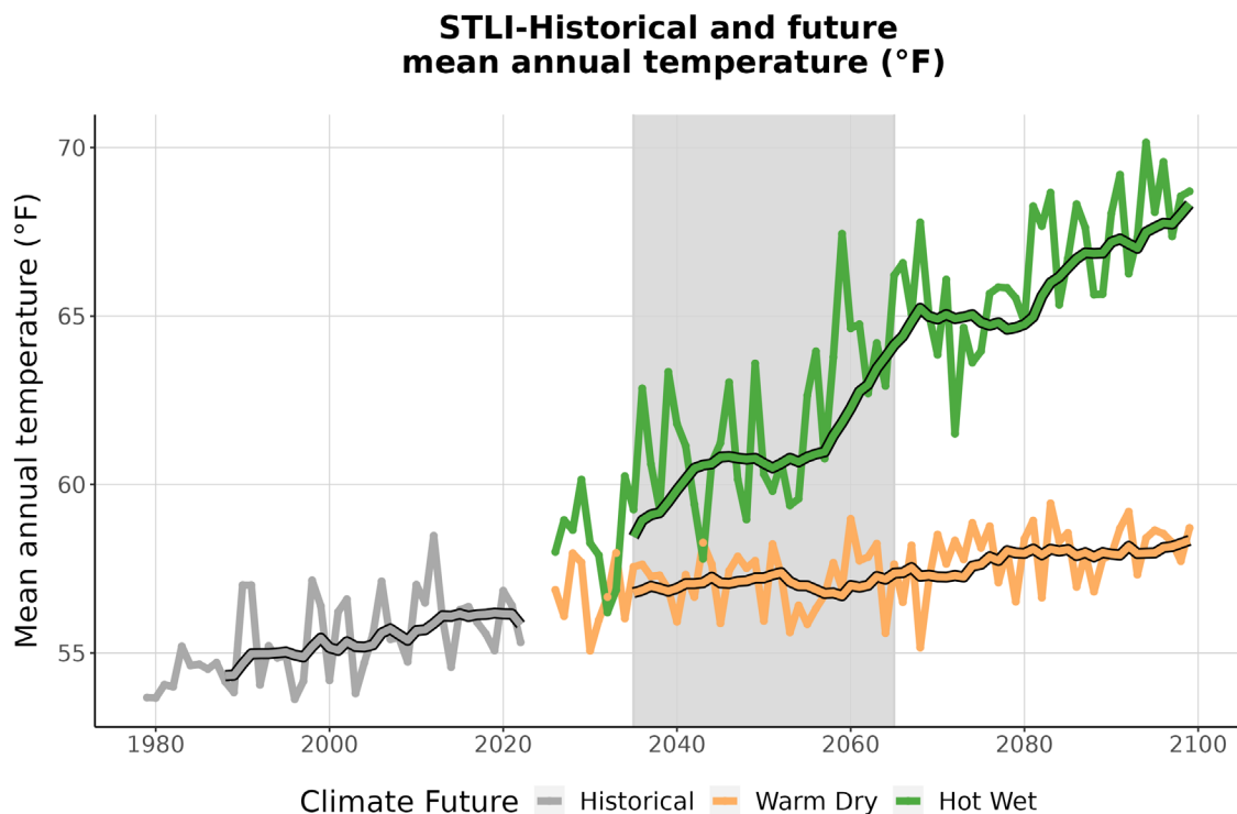
Figure 3. This graph compares observed average annual temperature at STLI (°F) (1979-2022) with projected average annual temperature for the two climate futures over the period 2023-2099. The historically observed data
