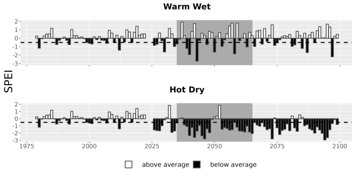
Figure 7. Drought metrics for STGE. Drought index (SPEI; units = standard deviations from historical) timeseries for each climate future. Below-average SPEI (black bars) indicates dry conditions. The dotted line (SPEI = -0.5) indicates drought conditions.
