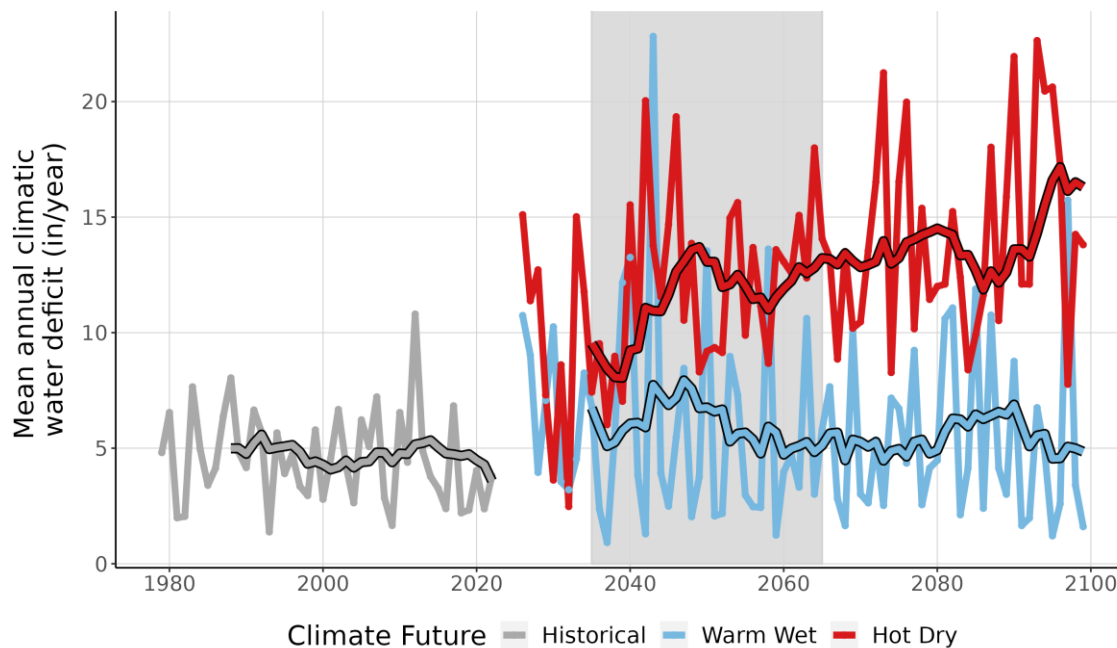
Figure 9. This line graph compares observed climatic water deficit at STGE (inches/year) (1979-2022) with projected climatic water deficit for the two climate futures over the period 2023-2099. The historical observation data is shown in gray, the Warm Wet climate future in blue, and the Hot Dry climate future in red. The smooth line running through each projection is the 10-year running average for historical observations and future projections. Gray-shaded area represents the time period that was averaged (2035-2065) to summarize future projections for the year 2050.
