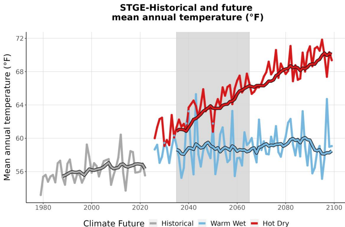
Figure 3. This graph compares observed average annual temperature at STGE (°F) (1979-2022) with projected average annual temperature for the two climate futures over the period 2023-2099. The historically observed data
