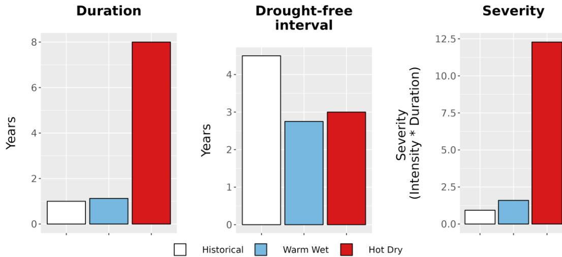
Figure 8. Drought metrics for STGE. (Left) Average drought duration (years) historically (1979-2012) and under each climate future. (Middle) Average drought return interval (years), indicating the expected amount of time between periods of drought, historically and under each climate future. (Right) Average drought severity, a measure of drought intensity multiplied by duration, historically and under each climate future.
