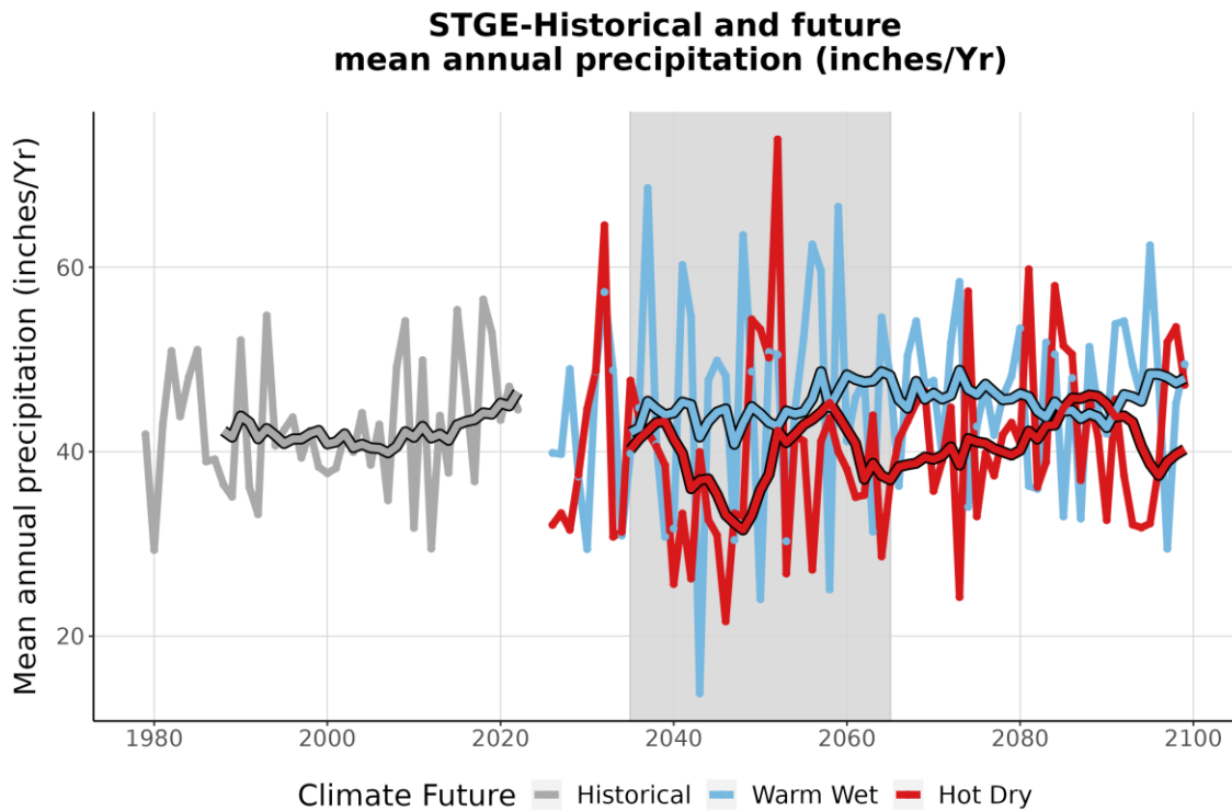
Figure 4. This graph compares observed average annual precipitation at STGE (inches/year) (1979-2022) with projected average annual precipitation for the two climate futures over the period 2023-2099. The historically observed data is shown in gray, the Warm Wet climate future in blue, and the Hot Dry climate future in red. The smooth line running through each projection is the 10-year running average for historical observations and future projections. The gray-shaded area represents the time period that was averaged (2035-2065) to summarize future projections for the year 2050 (Appendix 1).
