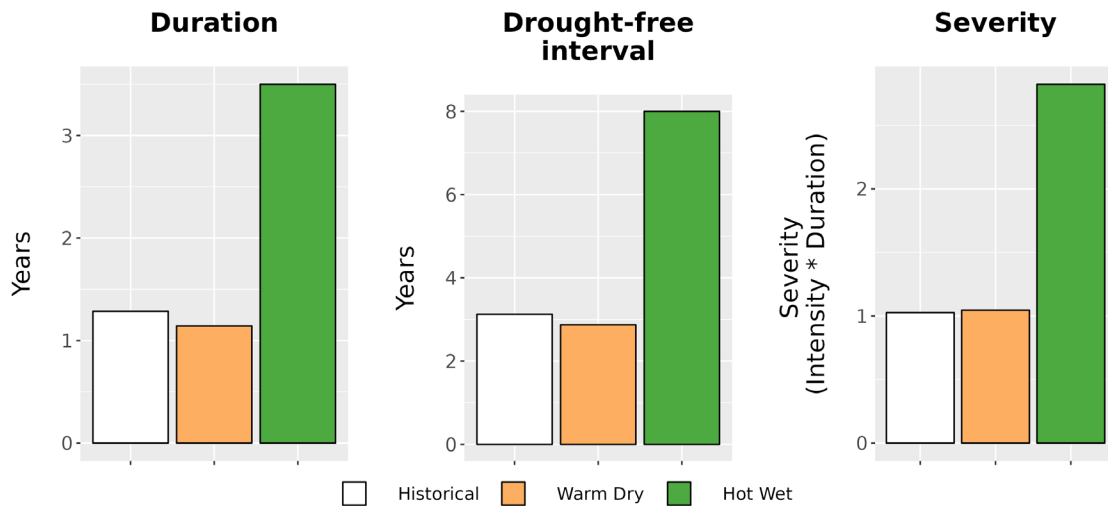
Figure 8. Drought metrics for STEA. (Left) Average drought duration (years) historically (1979-2012) and under each climate future. (Middle) Average drought return interval (years), indicating the expected amount of time between periods of drought, historically and under each climate future. (Right) Average drought severity, a measure of drought intensity multiplied by duration, historically and under each climate future.
