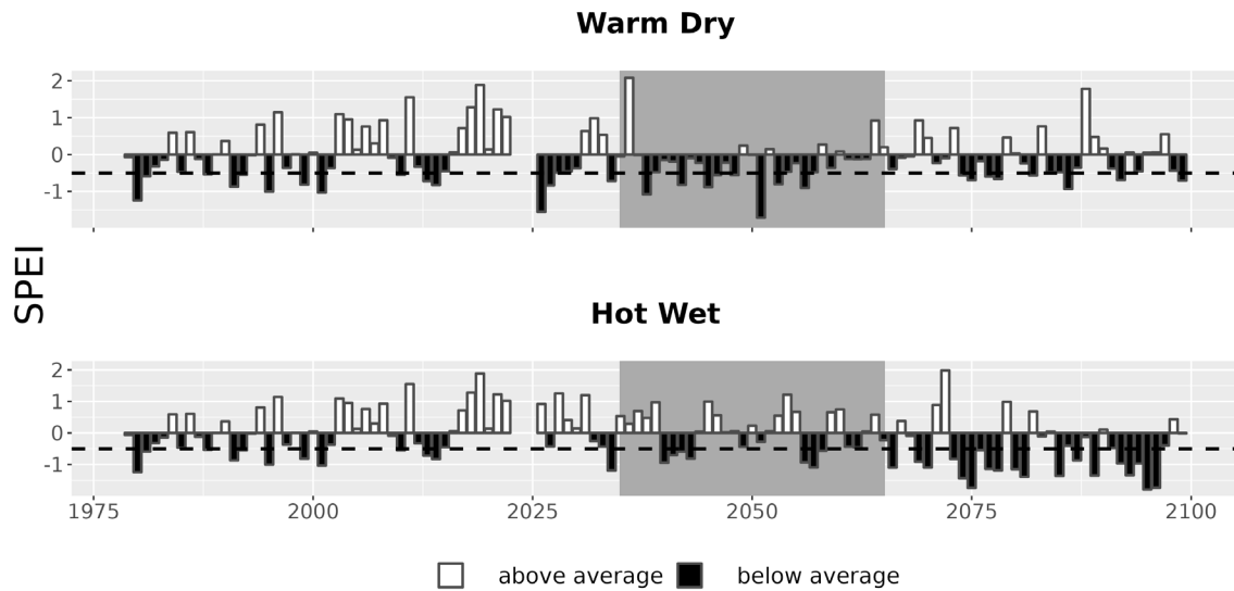
Figure 7. Drought metrics for STEA. Drought index (SPEI; units = standard deviations from historical) timeseries for each climate future. Below-average SPEI (black bars) indicates dry conditions. The dotted line (SPEI = -0.5) indicates drought conditions.
