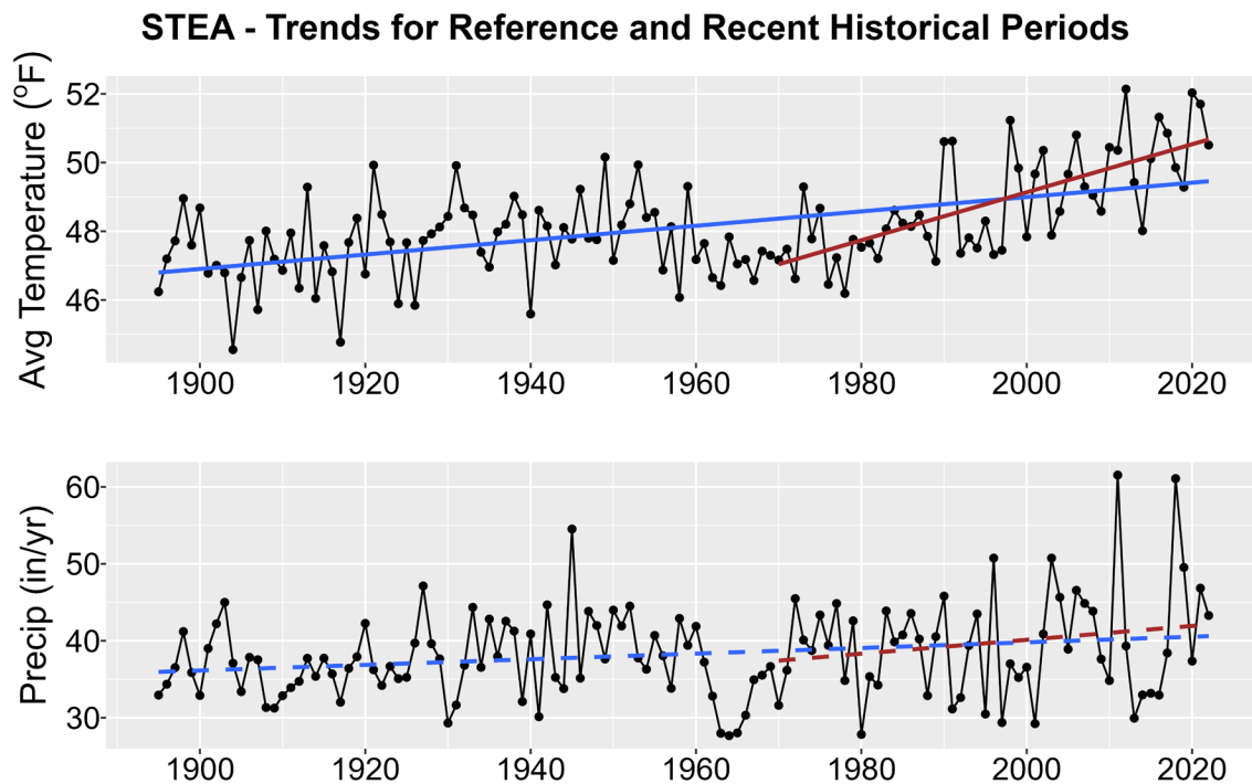
Figure 1. Historical trends in annual average temperature (upper plot) and annual total precipitation (lower plot) for STEA from 1895-2022. Black points show yearly values while blue lines are linear regressions for the entire period record and red lines for 1970-2022 trends. Solid lines are significant trends (i.e., p < 0.05 ); dashed lines are not statistically significant.
