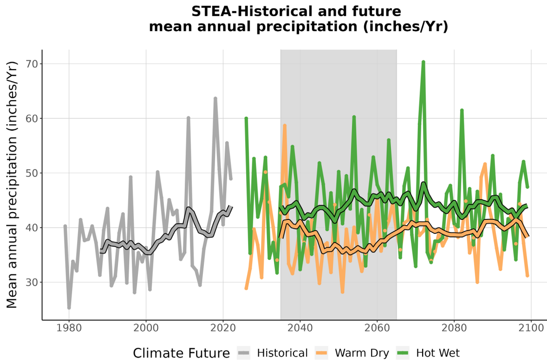
Figure 4. This graph compares observed average annual precipitation at STEA (inches/year) (1979-2022) with projected average annual precipitation for the two climate futures over the period 2023-2099. The historically observed data is shown in gray, the Warm Dry climate future in orange, and the Hot Wet climate future in green. The smooth line running through each projection is the 10-year running average for historical observations and future projections. The gray-shaded area represents the time period that was averaged (2035-2065) to summarize future projections for the year 2050 (Appendix 1).
