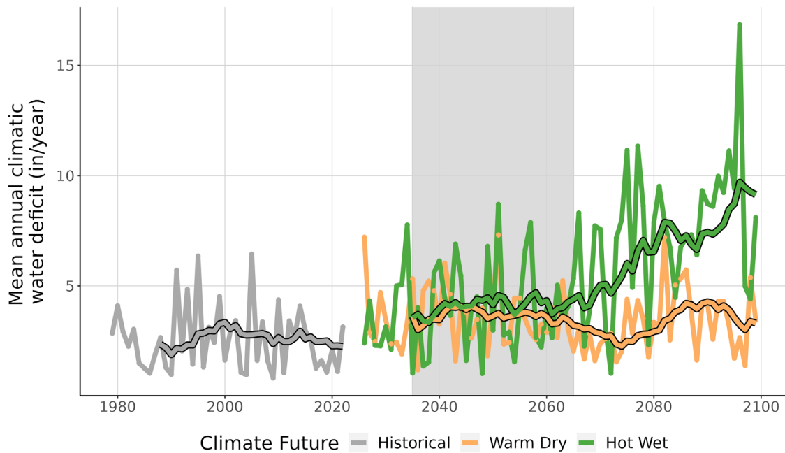
Figure 9. This line graph compares observed climatic water deficit at STEA (inches/year) (1979-2022) with projected climatic water deficit for the two climate futures over the period 2023-2099. The historical observation data is shown in gray, the Warm Dry climate future in orange, and the Hot Wet climate future in green. The smooth line running through each projection is the 10-year running average for historical observations and future projections. Gray-shaded area represents the time period that was averaged (2035-2065) to summarize future projections for the year 2050.
