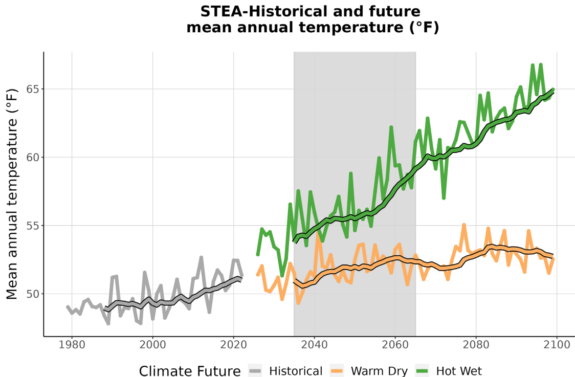
Figure 3. This graph compares observed average annual temperature at STEA (°F) (1979-2022) with projected average annual temperature for the two climate futures over the period 2023-2099. The historically observed data
