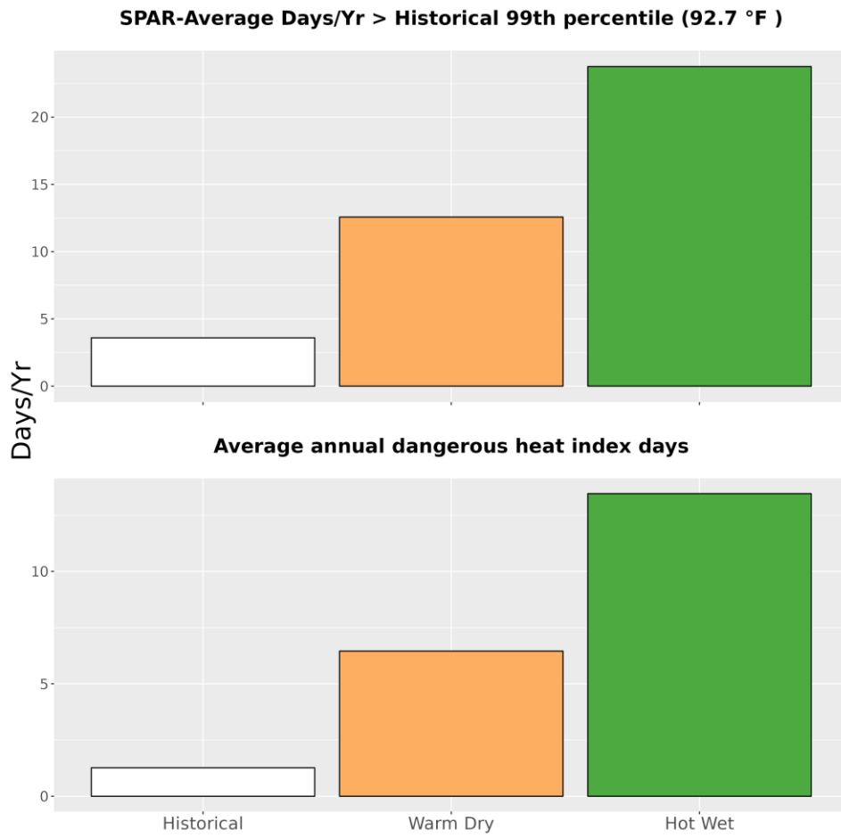
Figure 5. The upper bar graph represents the average number of days annually with temperatures greater than the historical 99 th percentile (92.7 °F) historically (1979-2012) and for the two climate futures (2050). The bottom bar graph represents the average annual number of dangerous heat index days historically and for the two climate futures. Dangerous heat index days are days that exceed 105 °F.
