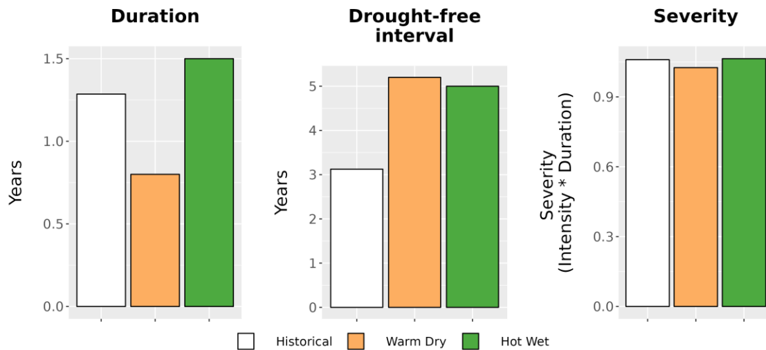
Figure 8. Drought metrics for SPAR. (Left) Average drought duration (years) historically (1979-2012) and under each climate future. (Middle) Average drought return interval (years), indicating the expected amount of time between periods of drought, historically and under each climate future. (Right) Average drought severity, a measure of drought intensity multiplied by duration, historically and under each climate future.
