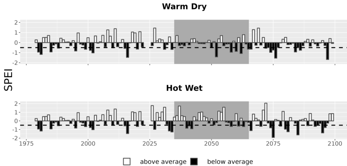
Figure 7. Drought metrics for SPAR. Drought index (SPEI; units = standard deviations from historical) timeseries for each climate future. Below-average SPEI (black bars) indicates dry conditions. The dotted line (SPEI = -0.5) indicates drought conditions.
