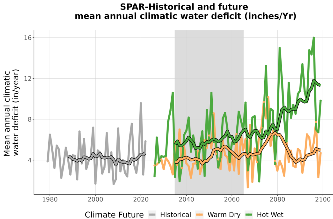
Figure 9. This line graph compares observed climatic water deficit at SPAR (inches/year) (1979-2022) with projected climatic water deficit for the two climate futures over the period 2023-2099. The historical observation data is shown in gray, the Warm Dry climate future in orange, and the Hot Wet climate future in green. The smooth line running through each projection is the 10-year running average for historical observations and future projections. Gray-shaded area represents the time period that was averaged (2035-2065) to summarize future projections for the year 2050.
