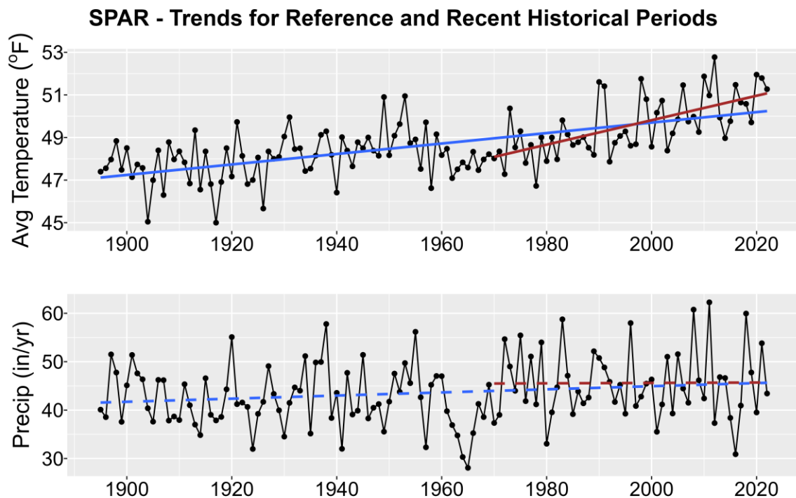
Figure 1. Historical trends in annual average temperature (upper plot) and annual total precipitation (lower plot) for SPAR from 1895-2022. Black points show yearly values while blue lines are linear regressions for the entire period record and red lines for 1970-2022 trends. Solid lines are significant trends (i.e., p < 0.05 ); dashed lines are not statistically significant.
