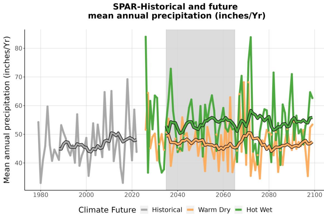
Figure 4. This graph compares observed average annual precipitation at SPAR (inches/year) (1979-2022) with projected average annual precipitation for the two climate futures over the period 2023-2099. The historically observed data is shown in gray, the Warm Dry climate future in orange, and the Hot Wet climate future in green. The smooth line running through each projection is the 10-year running average for historical observations and future projections. The gray-shaded area represents the time period that was averaged (2035-2065) to summarize future projections for the year 2050 (Appendix 1).
