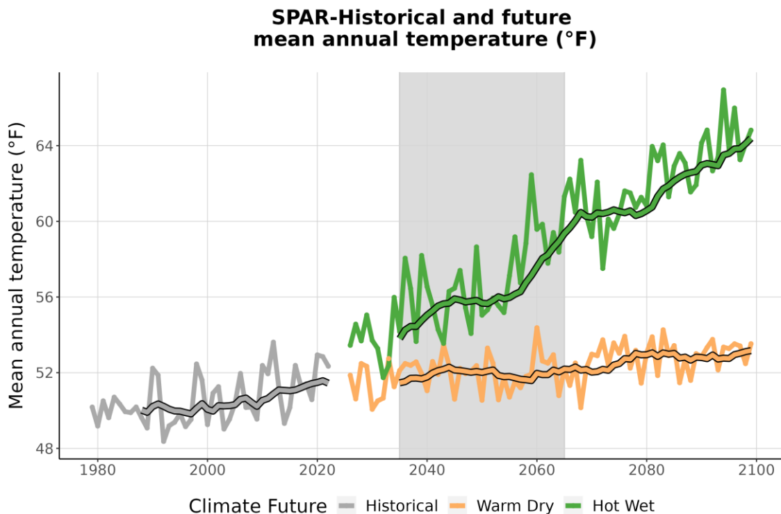
Figure 3. This graph compares observed average annual temperature at SPAR (°F) (1979-2022) with projected average annual temperature for the two climate futures over the period 2023-2099. The historically observed data
