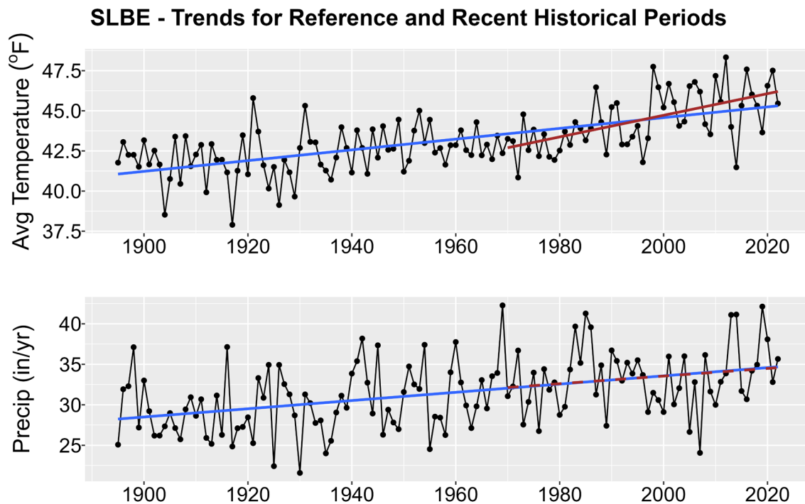
Figure 1. Historical trends in annual average temperature (upper plot) and annual total precipitation (lower plot) for SLBE from 1895-2022. Black points show yearly values while blue lines are linear regressions for the entire period record and red lines for 1970-2022 trends. Solid lines are significant trends (i.e., p < 0.05 ); dashed lines are not statistically significant.
