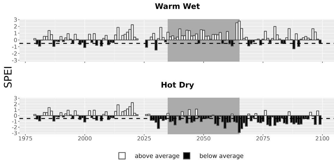
Figure 7. Drought metrics for SLBE. Drought index (SPEI; units = standard deviations from historical) timeseries for each climate future. Below-average SPEI (black bars) indicates dry conditions. The dotted line (SPEI = -0.5) indicates drought conditions.
