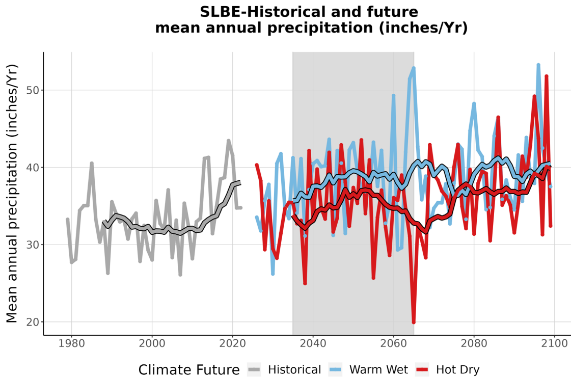
Figure 4. This graph compares observed average annual precipitation at SLBE (inches/year) (1979-2022) with projected average annual precipitation for the two climate futures over the period 2023-2099. The historically observed data is shown in gray, the Warm Wet climate future in blue, and the Hot Dry climate future in red. The smooth line running through each projection is the 10-year running average for historical observations and future projections. The gray-shaded area represents the time period that was averaged (2035-2065) to summarize future projections for the year 2050 (Appendix 1).
