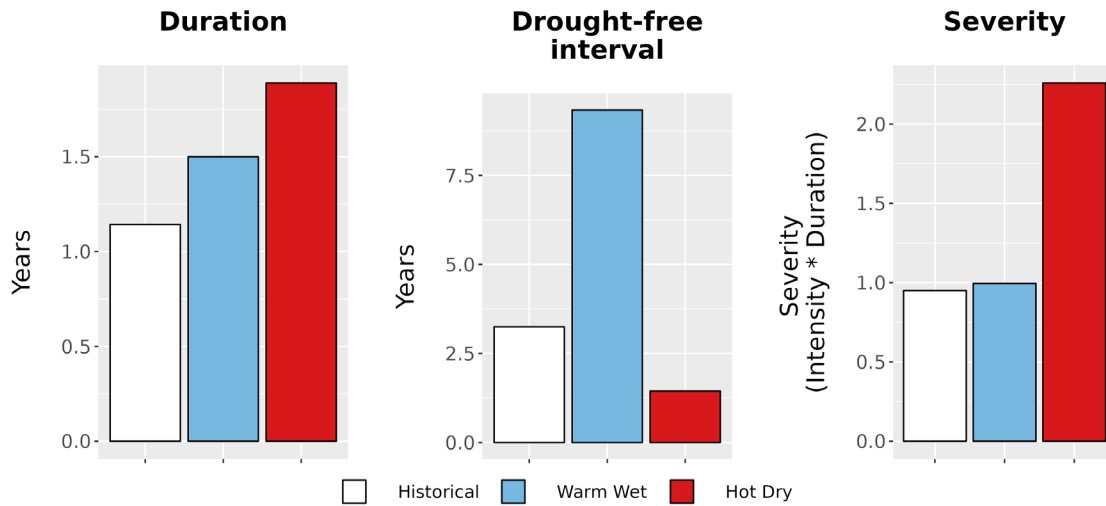
Figure 8. Drought metrics for SLBE. (Left) Average drought duration (years) historically (1979-2012) and under each climate future. (Middle) Average drought return interval (years), indicating the expected amount of time between periods of drought, historically and under each climate future. (Right) Average drought severity, a measure of drought intensity multiplied by duration, historically and under each climate future.
