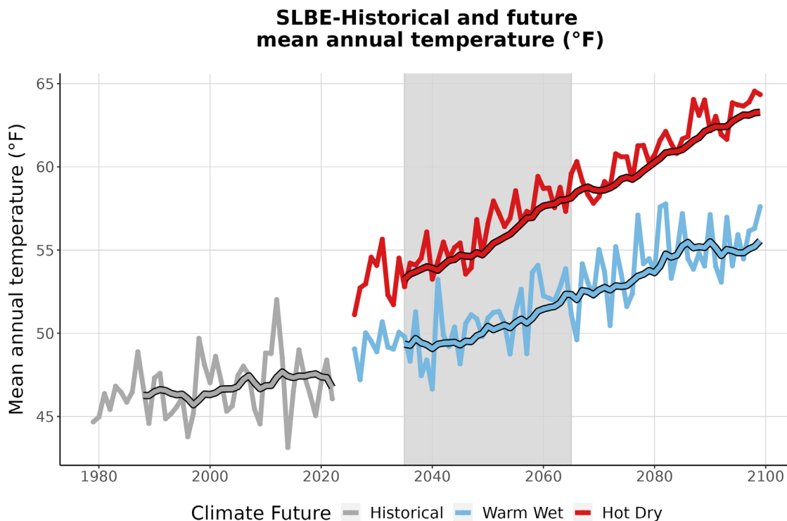
Figure 3. This graph compares observed average annual temperature at SLBE (°F) (1979-2022) with projected average annual temperature for the two climate futures over the period 2023-2099. The historically observed data
