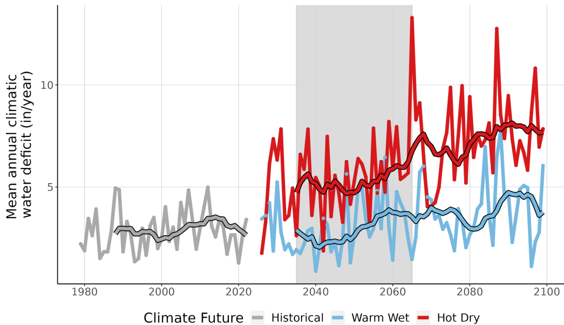
Figure 9. This line graph compares observed climatic water deficit at SLBE (inches/year) (1979-2022) with projected climatic water deficit for the two climate futures over the period 2023-2099. The historical observation data is shown in gray, the Warm Wet climate future in blue, and the Hot Dry climate future in red. The smooth line running through each projection is the 10-year running average for historical observations and future projections. Gray-shaded area represents the time period that was averaged (2035-2065) to summarize future projections for the year 2050.
