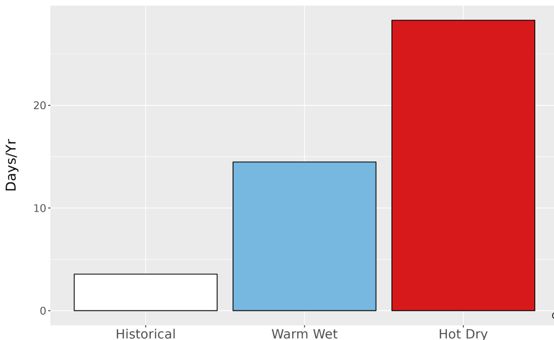
Figure 5. Metrics of extreme temperature at SLBE. The bar graph represents the average number of days annually with temperatures greater than the historical 99th percentile (86.3 °F) historically (1979-2012) and for the two climate futures (2050).
