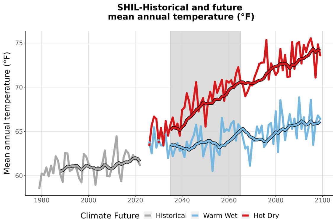
Figure 3. This graph compares observed average annual temperature at SHIL (°F) (1979-2022) with projected average annual temperature for the two climate futures over the period 2023-2099. The historically observed data
