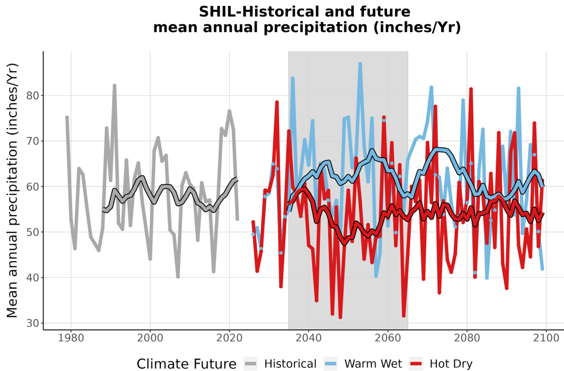
Figure 4. This graph compares observed average annual precipitation at SHIL (inches/year) (1979-2022) with projected average annual precipitation for the two climate futures over the period 2023-2099. The historically observed data is shown in gray, the Warm Wet climate future in blue, and the Hot Dry climate future in red. The smooth line running through each projection is the 10-year running average for historical observations and future projections. The gray-shaded area represents the time period that was averaged (2035-2065) to summarize future projections for the year 2050 (Appendix 1).
