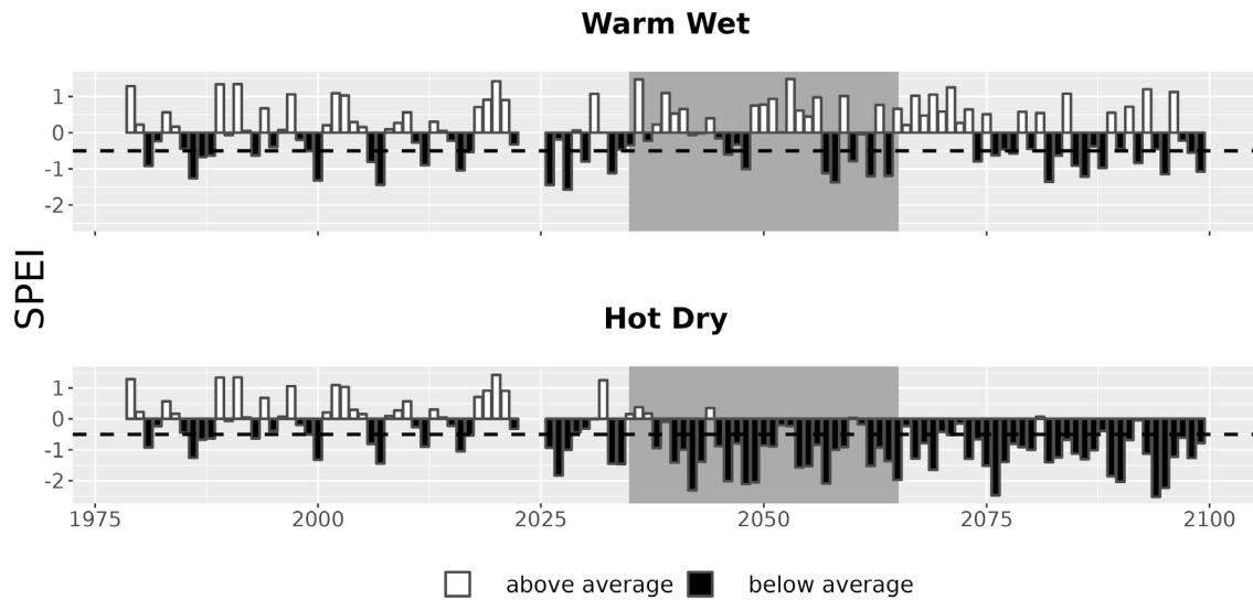
Figure 7. Drought metrics for SHIL. Drought index (SPEI; units = standard deviations from historical) timeseries for each climate future. Below-average SPEI (black bars) indicates dry conditions. The dotted line (SPEI = -0.5) indicates drought conditions.
