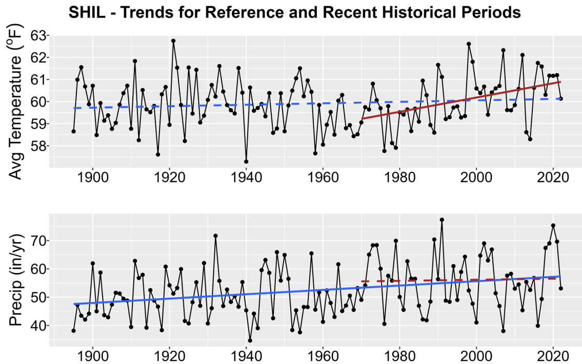
Figure 1. Historical trends in annual average temperature (upper plot) and annual total precipitation (lower plot) for SHIL from 1895-2022. Black points show yearly values while blue lines are linear regressions for the entire period record and red lines for 1970-2022 trends. Solid lines are significant trends (i.e., p < 0.05 ); dashed lines are not statistically significant.
