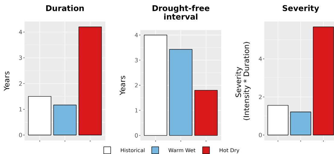
Figure 8. Drought metrics for SHIL. (Left) Average drought duration (years) historically (1979-2012) and under each climate future. (Middle) Average drought return interval (years), indicating the expected amount of time between periods of drought, historically and under each climate future. (Right) Average drought severity, a measure of drought intensity multiplied by duration, historically and under each climate future.
