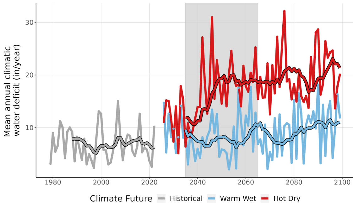
Figure 9. This line graph compares observed climatic water deficit at SHIL (inches/year) (1979-2022) with projected climatic water deficit for the two climate futures over the period 2023-2099. The historical observation data is shown in gray, the Warm Wet climate future in blue, and the Hot Dry climate future in red. The smooth line running through each projection is the 10-year running average for historical observations and future projections. Gray-shaded area represents the time period that was averaged (2035-2065) to summarize future projections for the year 2050.
