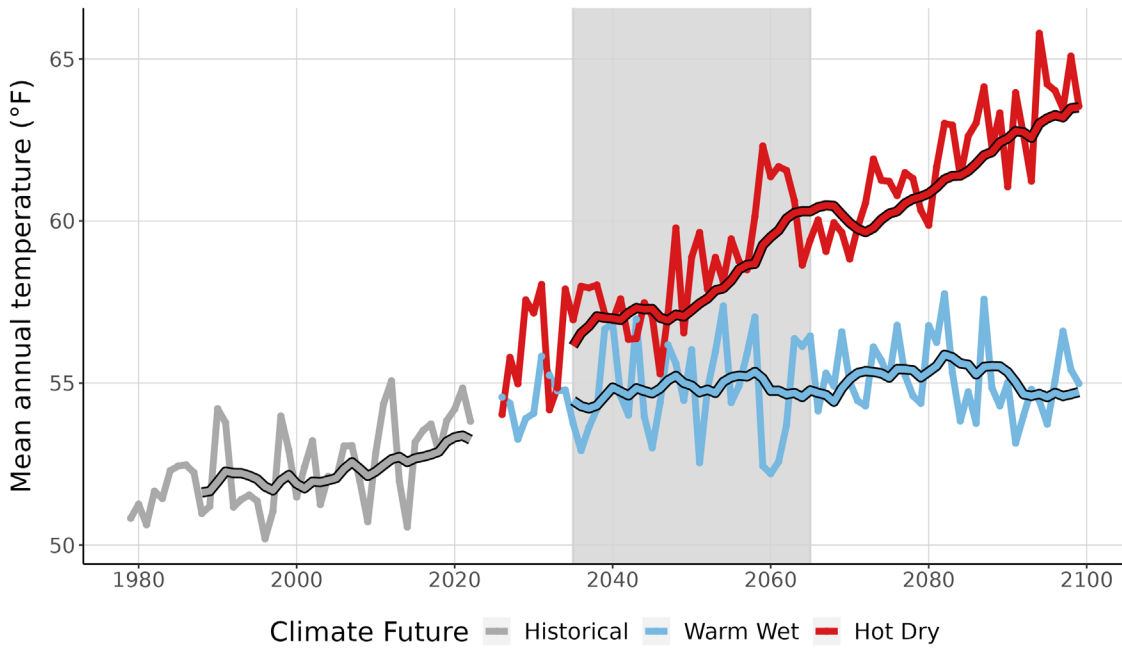
Figure 3. This graph compares observed average annual temperature at SHEN (°F) (1979-2022) with projected average annual temperature for the two climate futures over the period 2023-2099. The historically observed data is shown in gray, the Warm Wet climate future in blue, and the Hot Dry climate future in red. The smooth line running through each projection is the 10-year running average for historical observations and future projections. Gray-shaded area represents the time period that was averaged (2035-2065) to summarize future projections for the year 2050 (Appendix 1).
