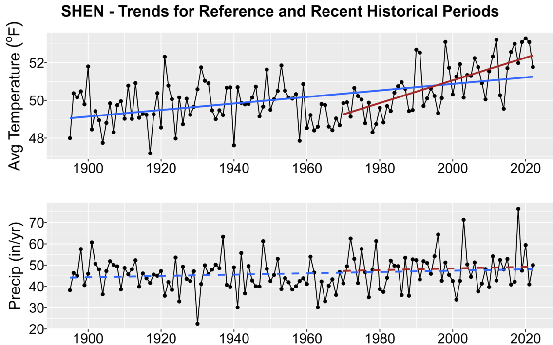
Figure 1. Historical trends in annual average temperature (upper plot) and annual total precipitation (lower plot) for SHEN from 1895-2022. Black points show yearly values while blue lines are linear regressions for the entire period record and red lines for 1970-2022 trends. Solid lines are significant trends (i.e., p < 0.05 ); dashed lines are not statistically significant.
