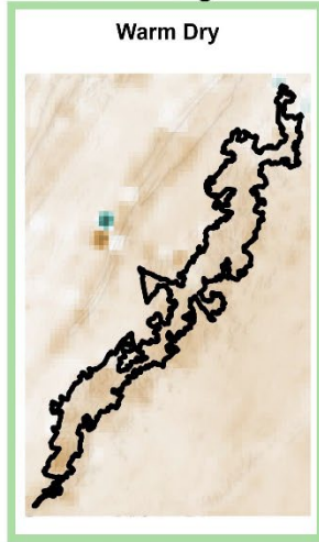
Figure A3. (Top) Map showing average annual climatic water deficit for the historical period (inches/year) and (bottom) change in average annual climatic water deficit for the two climate futures. Legends are located below each set of maps as a continuous color gradient. Gridded data is extracted from 30-year summary GIS layers for CONUS water balance model (Tercek et al 2021, 2023). ( http://screenedcleanedsummaries.s3-website-us-west-2.amazonaws.com/ ) accessed on 6/3/2024.
