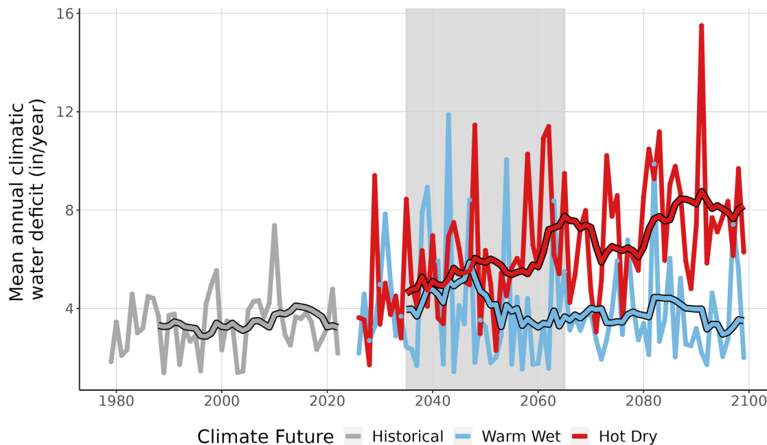
Figure 9. This line graph compares observed climatic water deficit at SHEN (inches/year) (1979-2022) with projected climatic water deficit for the two climate futures over the period 2023-2099. The historical observation data is shown in gray, the Warm Wet climate future in blue, and the Hot Dry climate future in red. The smooth line running through each projection is the 10-year running average for historical observations and future projections. Gray-shaded area represents the time period that was averaged (2035-2065) to summarize future projections for the year 2050.
