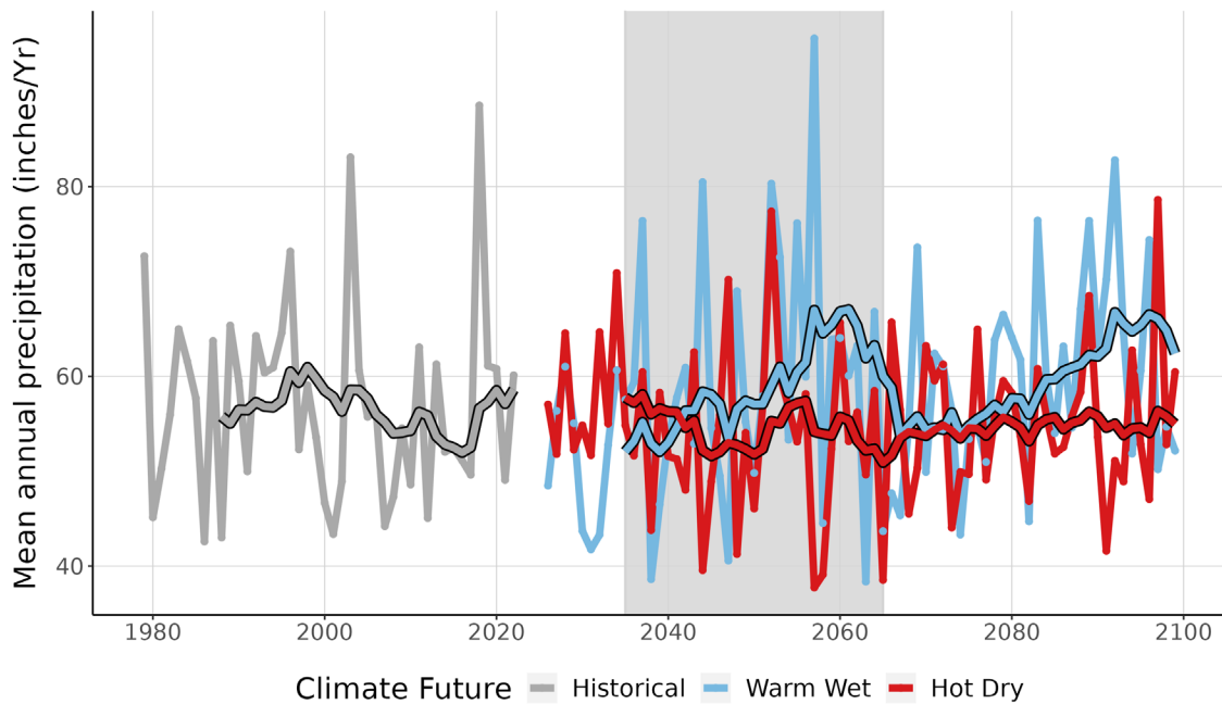
Figure 4. This graph compares observed average annual precipitation at SHEN (inches/year) (1979-2022) with projected average annual precipitation for the two climate futures over the period 2023-2099. The historically observed data is shown in gray, the Warm Wet climate future in blue, and the Hot Dry climate future in red. The smooth line running through each projection is the 10-year running average for historical observations and future projections. The gray-shaded area represents the time period that was averaged (2035-2065) to summarize future projections for the year 2050 (Appendix 1).
