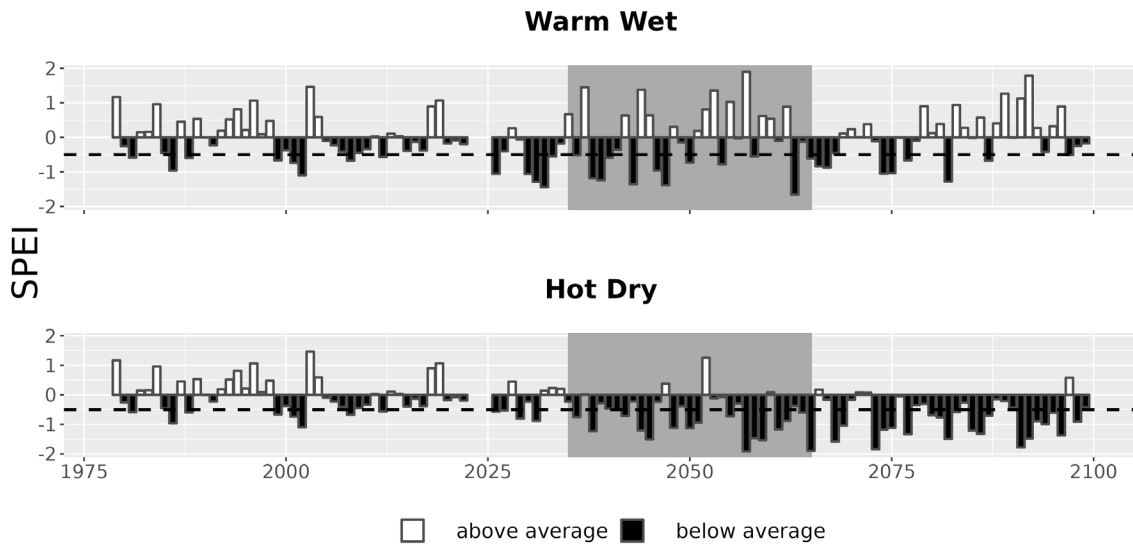
Figure 7. Drought metrics for SHEN. Drought index (SPEI; units = standard deviations from historical) timeseries for each climate future. Below-average SPEI (black bars) indicates dry conditions. The dotted line (SPEI = -0.5) indicates drought conditions.
