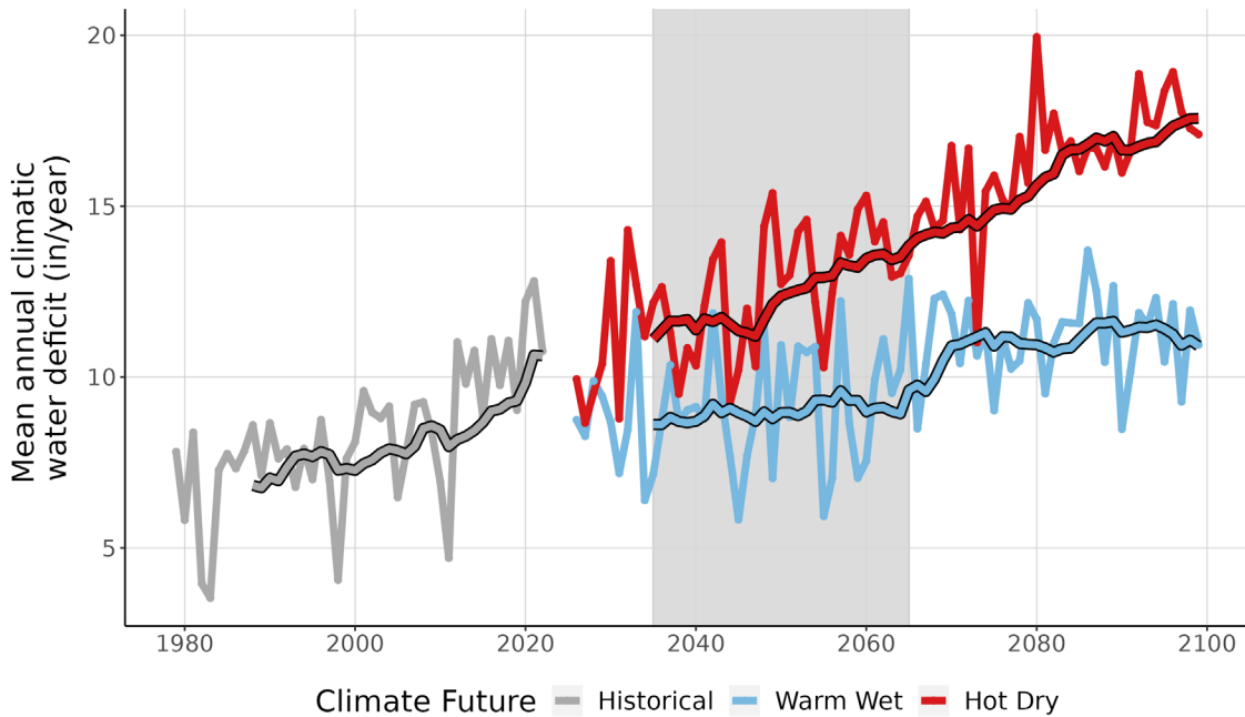
Figure 9. This line graph compares observed climatic water deficit at SEQU (inches/year) (1979-2022) with projected climatic water deficit for the two climate futures over the period 2023-2099. The historical observation data is shown in gray, the Warm Wet climate future in blue, and the Hot Dry climate future in red. The smooth line running through each projection is the 10-year running average for historical observations and future projections. Gray-shaded area represents the time period that was averaged (2035-2065) to summarize future projections for the year 2050.
