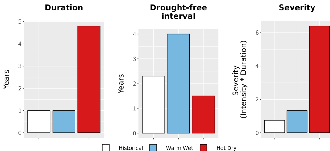
Figure 8. Drought metrics for SEQU. (Left) Average drought duration (years) historically (1979-2012) and under each climate future. (Middle) Average drought return interval (years), indicating the expected amount of time between periods of drought, historically and under each climate future. (Right) Average drought severity, a measure of drought intensity multiplied by duration, historically and under each climate future.
