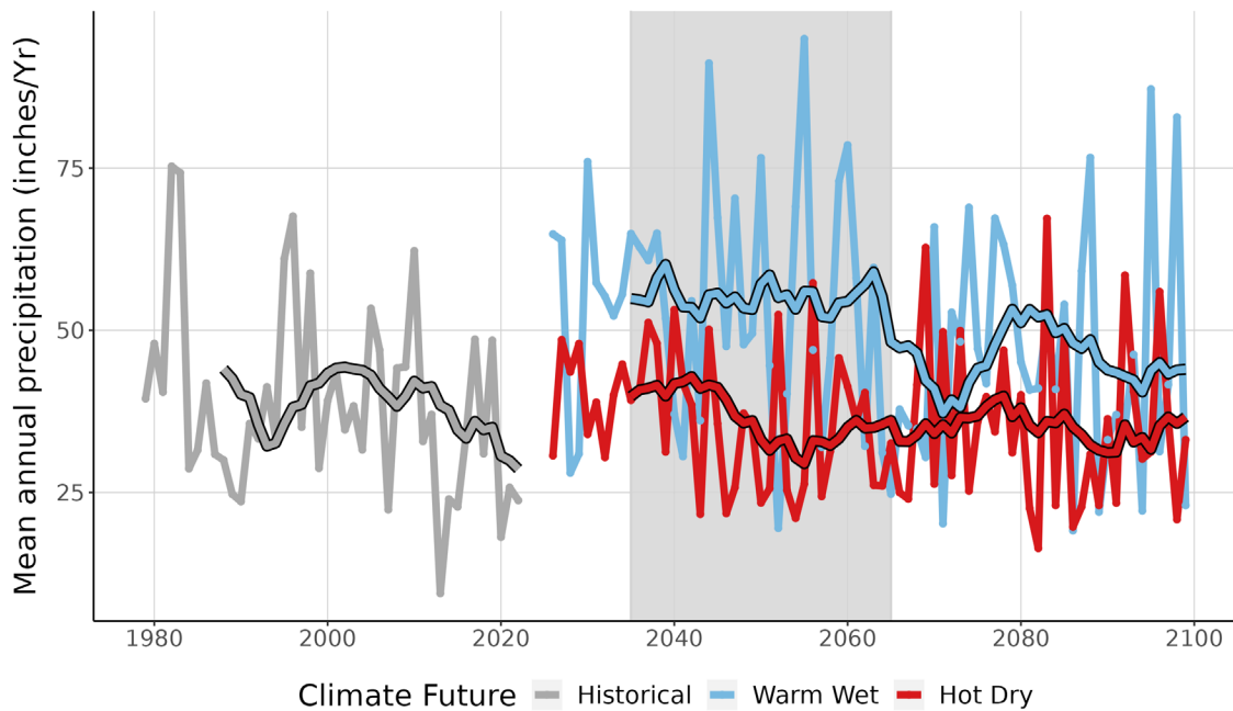
Figure 4. This graph compares observed average annual precipitation at SEQU (inches/year) (1979-2022) with projected average annual precipitation for the two climate futures over the period 2023-2099. The historically observed data is shown in gray, the Warm Wet climate future in blue, and the Hot Dry climate future in red. The smooth line running through each projection is the 10-year running average for historical observations and future projections. The gray-shaded area represents the time period that was averaged (2035-2065) to summarize future projections for the year 2050 (Appendix 1).
