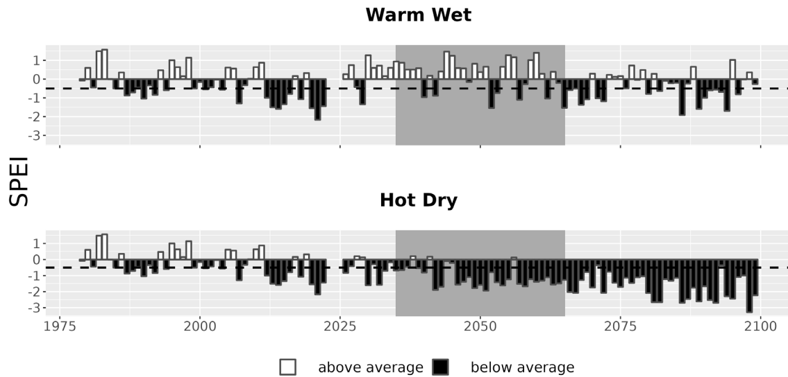
Figure 7. Drought metrics for SEQU. Drought index (SPEI; units = standard deviations from historical) timeseries for each climate future. Below-average SPEI (black bars) indicates dry conditions. The dotted line (SPEI = -0.5) indicates drought conditions.
