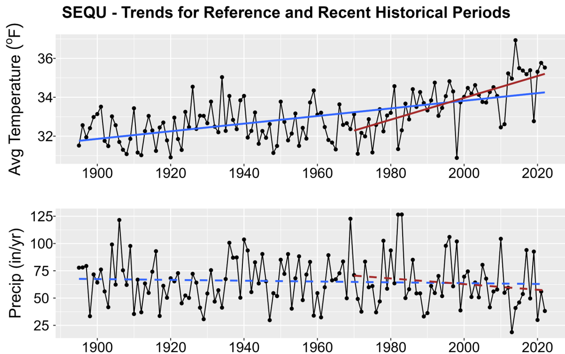
Figure 1. Historical trends in annual average temperature (upper plot) and annual total precipitation (lower plot) for SEQU from 1895-2022. Black points show yearly values while blue lines are linear regressions for the entire period record and red lines for 1970-2022 trends. Solid lines are significant trends (i.e., p < 0.05 ); dashed lines are not statistically significant.
