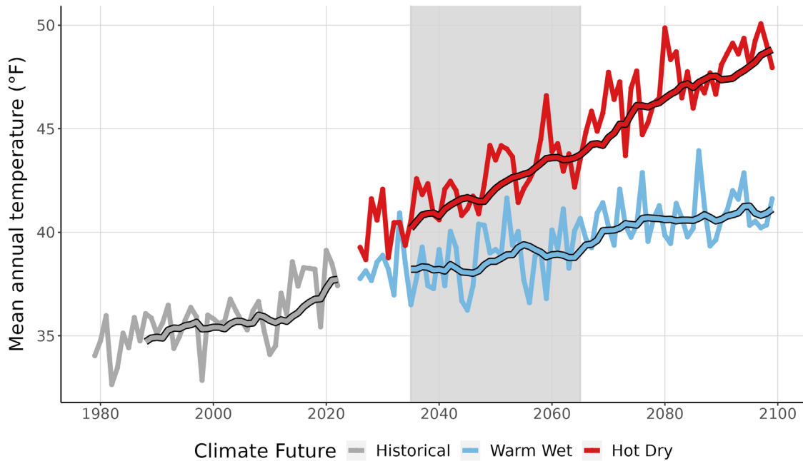
Figure 3. This graph compares observed average annual temperature at SEQU (°F) (1979-2022) with projected average annual temperature for the two climate futures over the period 2023-2099. The historically observed data is shown in gray, the Warm Wet climate future in blue, and the Hot Dry climate future in red. The smooth line running through each projection is the 10-year running average for historical observations and future projections. Gray-shaded area represents the time period that was averaged (2035-2065) to summarize future projections for the year 2050 (Appendix 1).
