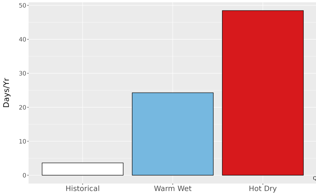
Figure 5. Metrics of extreme temperature at SEQU. The bar graph represents the average number of days annually with temperatures greater than the historical 99th percentile (68.4 °F) historically (1979-2012) and for the two climate futures (2050).
