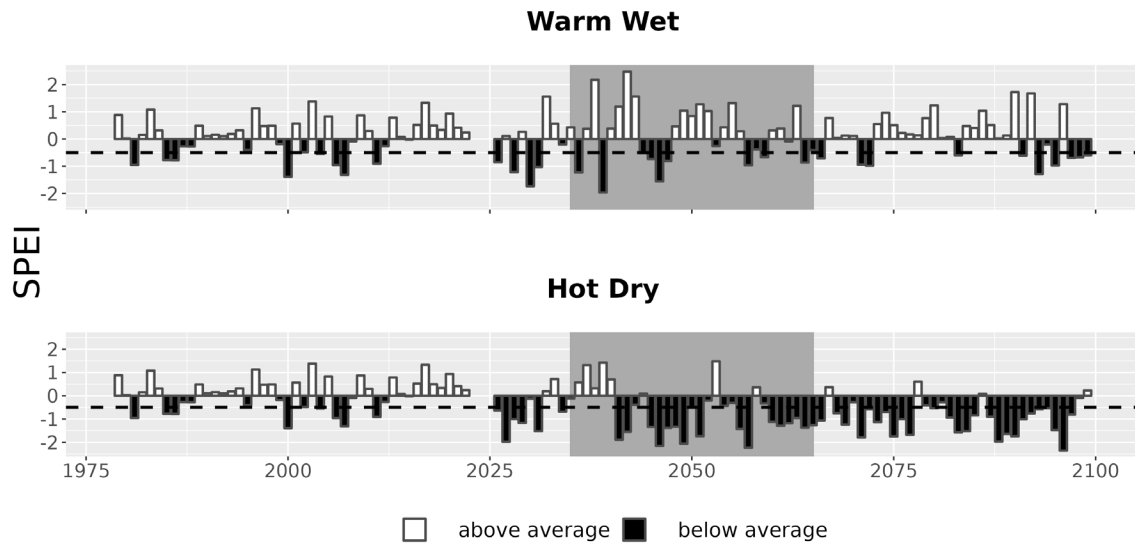
Figure 7. Drought metrics for SEMO. Drought index (SPEI; units = standard deviations from historical) timeseries for each climate future. Below-average SPEI (black bars) indicates dry conditions. The dotted line (SPEI = -0.5) indicates drought conditions.
