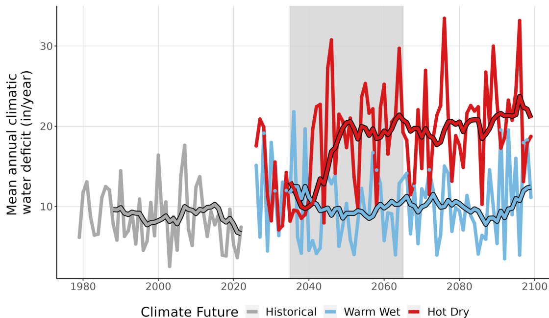
Figure 9. This line graph compares observed climatic water deficit at SEMO (inches/year) (1979-2022) with projected climatic water deficit for the two climate futures over the period 2023-2099. The historical observation data is shown in gray, the Warm Wet climate future in blue, and the Hot Dry climate future in red. The smooth line running through each projection is the 10-year running average for historical observations and future projections. Gray-shaded area represents the time period that was averaged (2035-2065) to summarize future projections for the year 2050.
