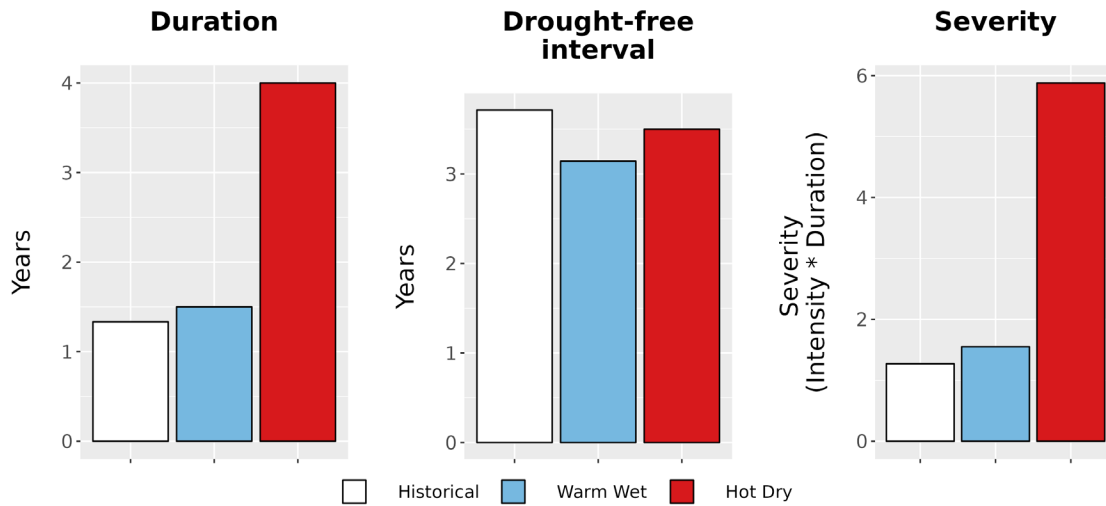
Figure 8. Drought metrics for SEMO. (Left) Average drought duration (years) historically (1979-2012) and under each climate future. (Middle) Average drought return interval (years), indicating the expected amount of time between periods of drought, historically and under each climate future. (Right) Average drought severity, a measure of drought intensity multiplied by duration, historically and under each climate future.
