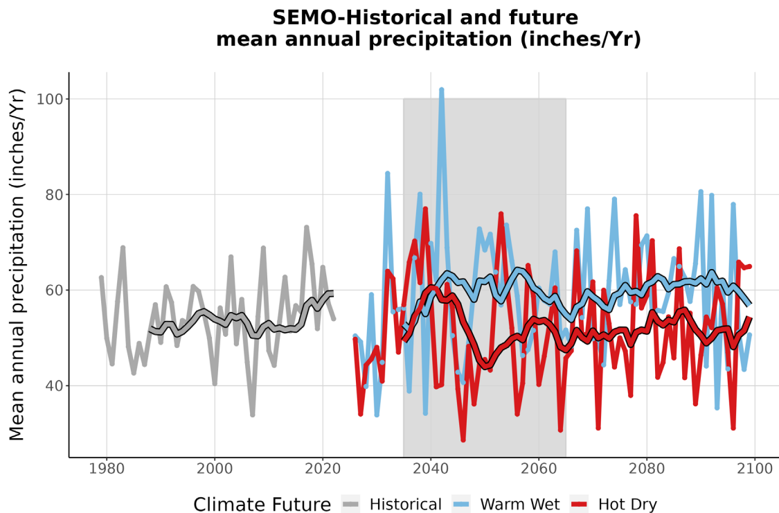
Figure 4. This graph compares observed average annual precipitation at SEMO (inches/year) (1979-2022) with projected average annual precipitation for the two climate futures over the period 2023-2099. The historically observed data is shown in gray, the Warm Wet climate future in blue, and the Hot Dry climate future in red. The smooth line running through each projection is the 10-year running average for historical observations and future projections. The gray-shaded area represents the time period that was averaged (2035-2065) to summarize future projections for the year 2050 (Appendix 1).
