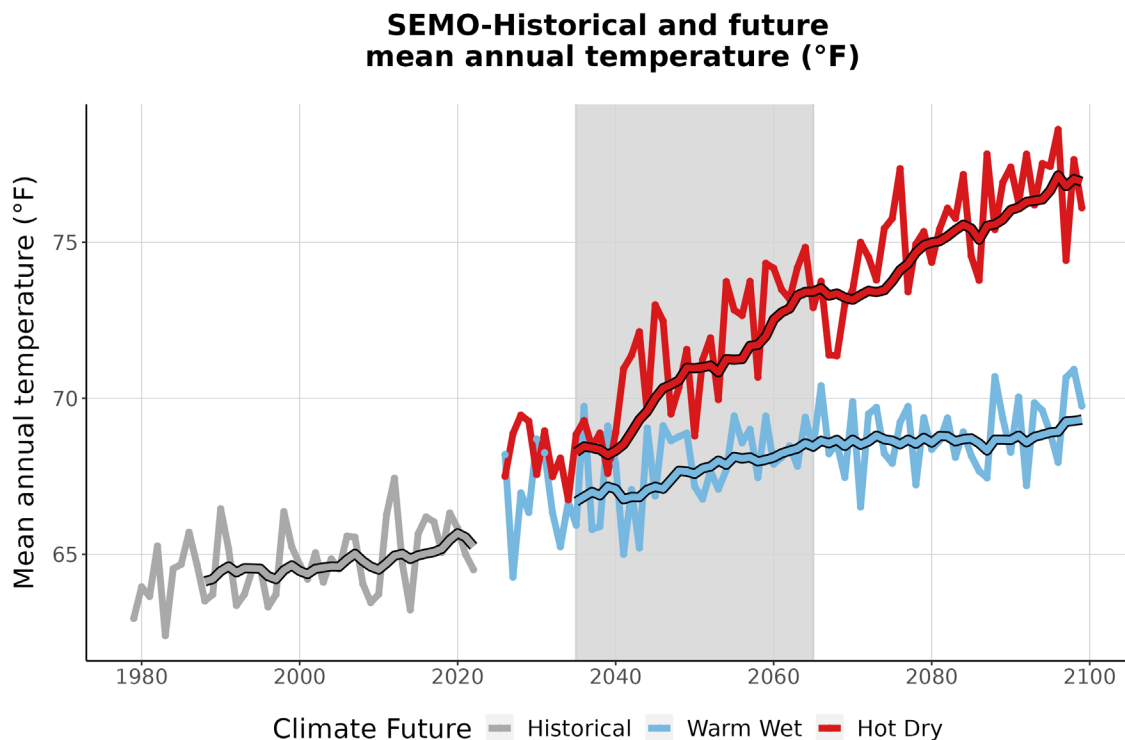
Figure 3. This graph compares observed average annual temperature at SEMO (°F) (1979-2022) with projected average annual temperature for the two climate futures over the period 2023-2099. The historically observed data
