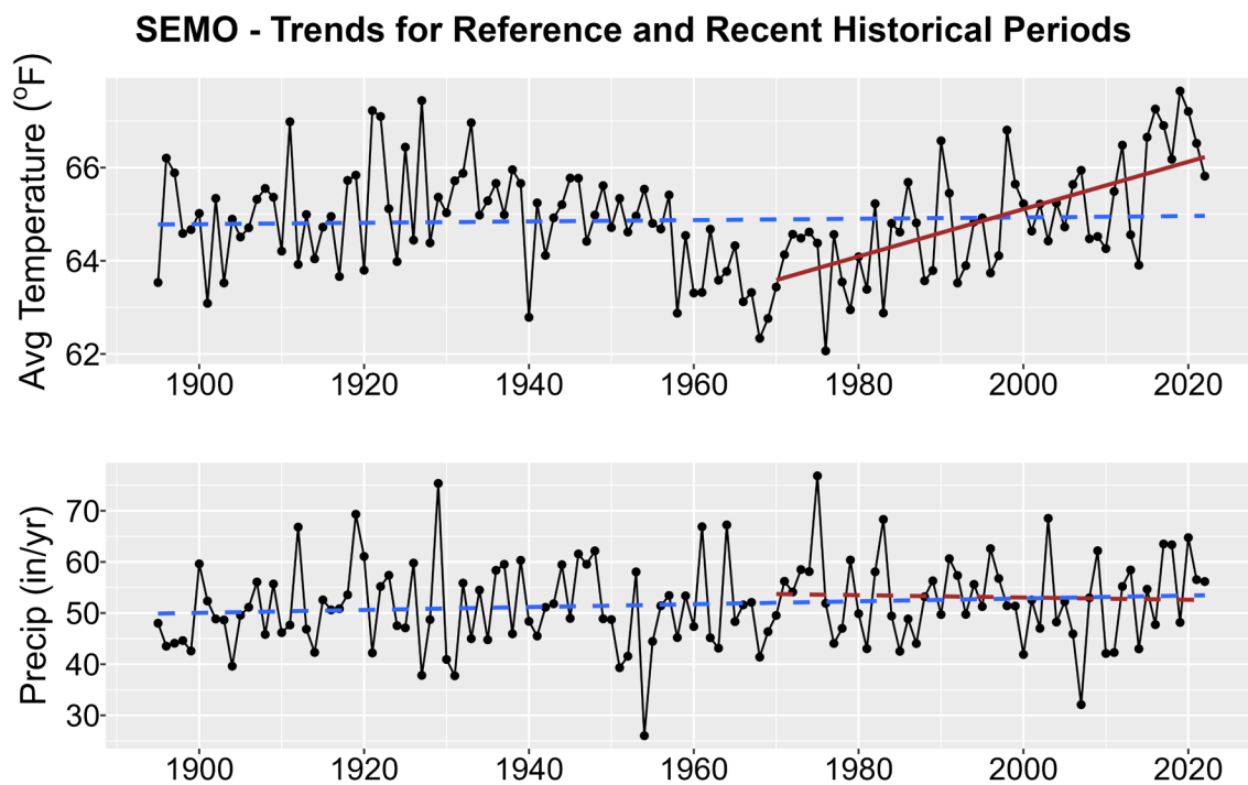
Figure 1. Historical trends in annual average temperature (upper plot) and annual total precipitation (lower plot) for SEMO from 1895-2022. Black points show yearly values while blue lines are linear regressions for the entire period record and red lines for 1970-2022 trends. Solid lines are significant trends (i.e., p < 0.05 ); dashed lines are not statistically significant.
