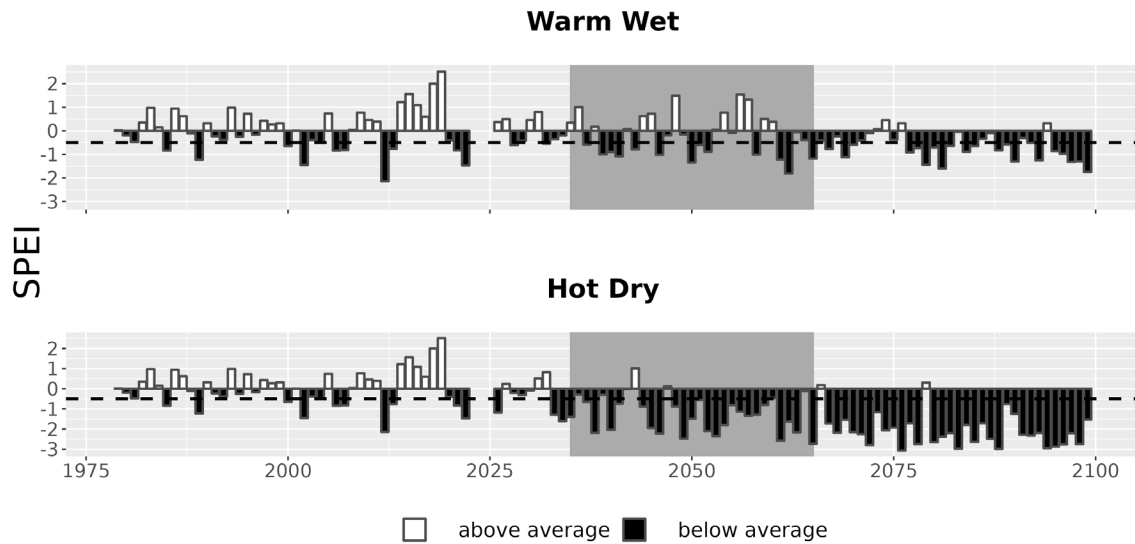
Figure 7. Drought metrics for SCBL. Drought index (SPEI; units = standard deviations from historical) timeseries for each climate future. Below-average SPEI (black bars) indicates dry conditions. The dotted line (SPEI = -0.5) indicates drought conditions.
