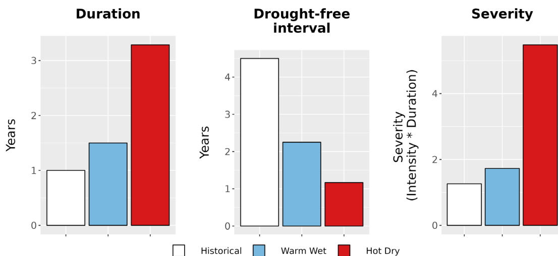
Figure 8. Drought metrics for SCBL. (Left) Average drought duration (years) historically (1979-2012) and under each climate future. (Middle) Average drought return interval (years), indicating the expected amount of time between periods of drought, historically and under each climate future. (Right) Average drought severity, a measure of drought intensity multiplied by duration, historically and under each climate future.
