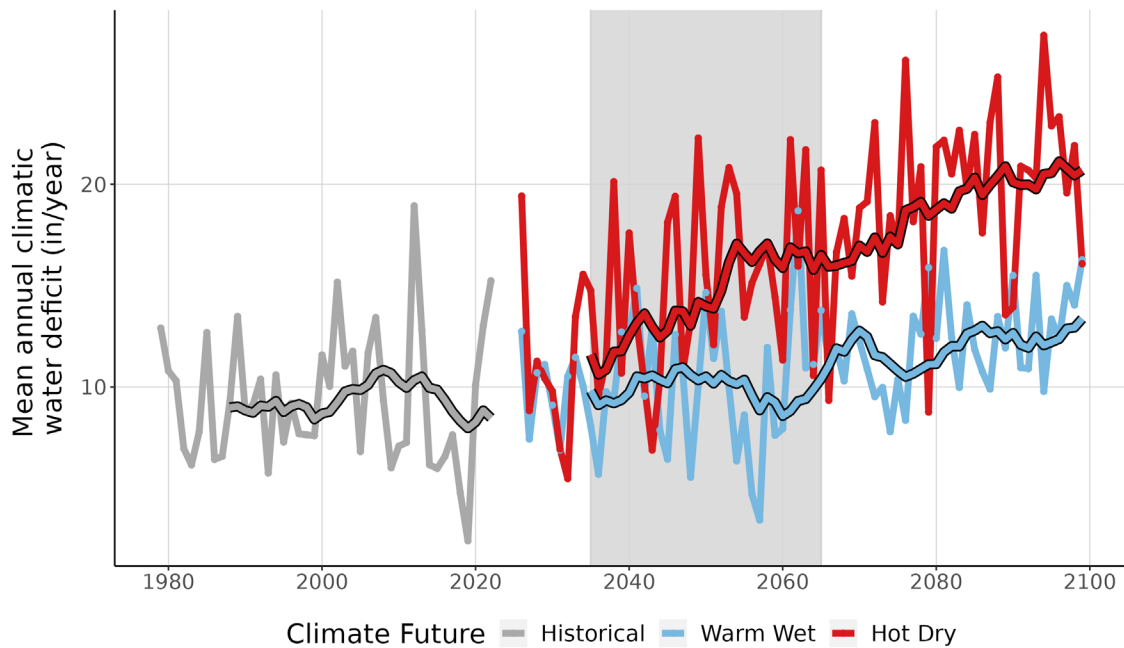
Figure 9. This line graph compares observed climatic water deficit at SCBL (inches/year) (1979-2022) with projected climatic water deficit for the two climate futures over the period 2023-2099. The historical observation data is shown in gray, the Warm Wet climate future in blue, and the Hot Dry climate future in red. The smooth line running through each projection is the 10-year running average for historical observations and future projections. Gray-shaded area represents the time period that was averaged (2035-2065) to summarize future projections for the year 2050.
