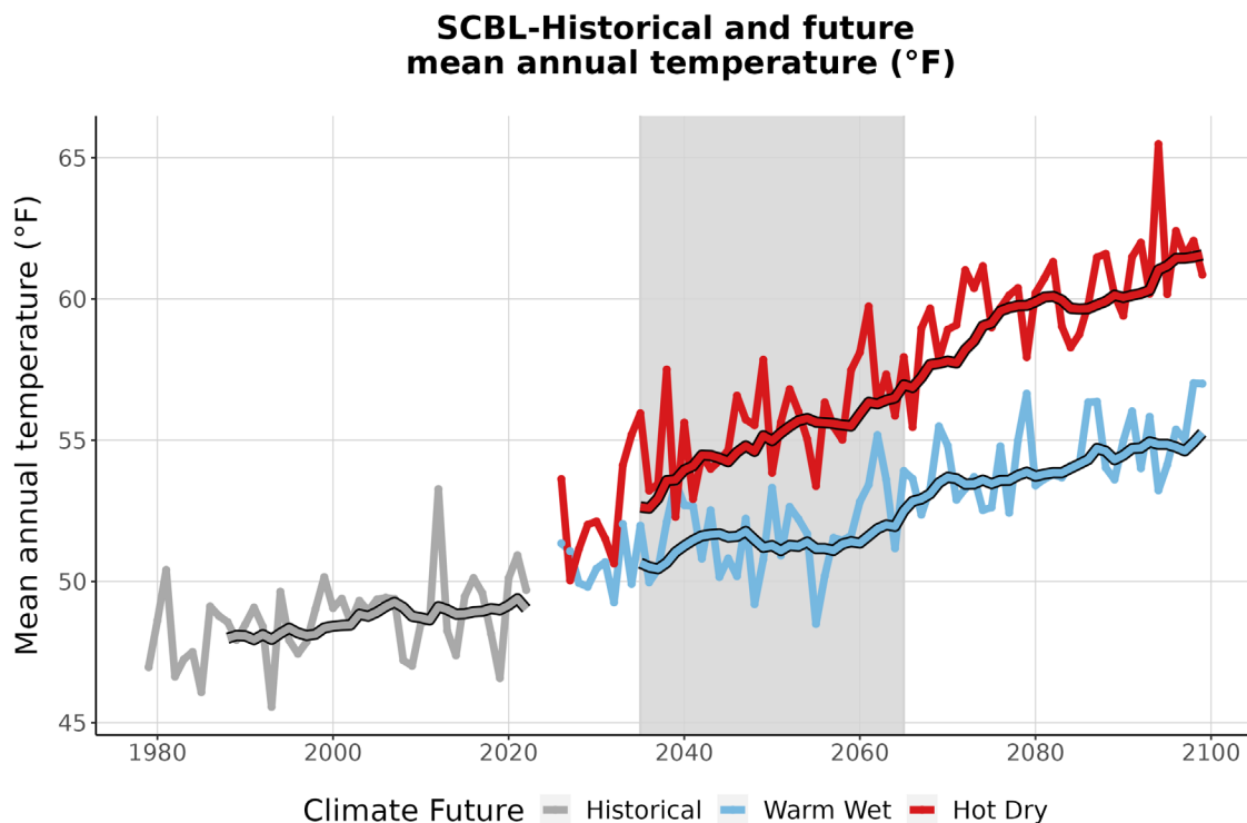
Figure 3. This graph compares observed average annual temperature at SCBL (°F) (1979-2022) with projected average annual temperature for the two climate futures over the period 2023-2099. The historically observed data
