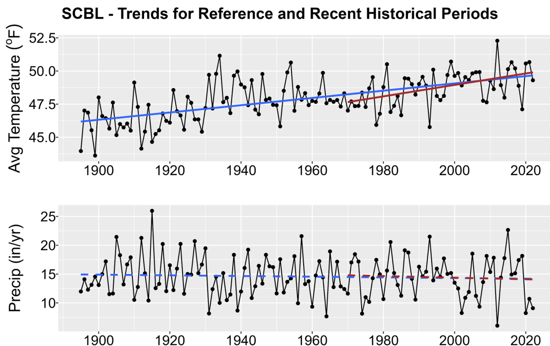
Figure 1. Historical trends in annual average temperature (upper plot) and annual total precipitation (lower plot) for SCBL from 1895-2022. Black points show yearly values while blue lines are linear regressions for the entire period record and red lines for 1970-2022 trends. Solid lines are significant trends (i.e., p < 0.05 ); dashed lines are not statistically significant.
