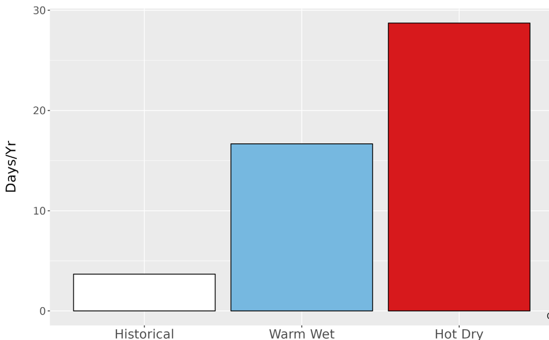
Figure 5. Metrics of extreme temperature at SCBL. The bar graph represents the average number of days annually with temperatures greater than the historical 99th percentile (98.5 °F) historically (1979-2012) and for the two climate futures (2050).
