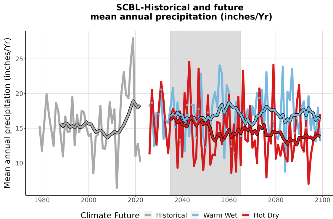
Figure 4. This graph compares observed average annual precipitation at SCBL (inches/year) (1979-2022) with projected average annual precipitation for the two climate futures over the period 2023-2099. The historically observed data is shown in gray, the Warm Wet climate future in blue, and the Hot Dry climate future in red. The smooth line running through each projection is the 10-year running average for historical observations and future projections. The gray-shaded area represents the time period that was averaged (2035-2065) to summarize future projections for the year 2050 (Appendix 1).
