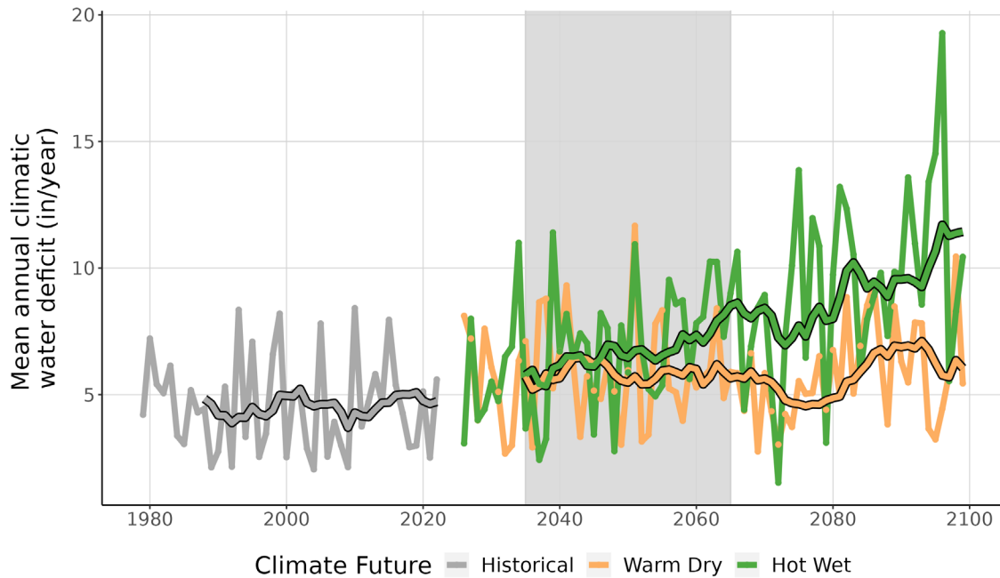
Figure 9. This line graph compares observed climatic water deficit at SAPA (inches/year) (1979-2022) with projected climatic water deficit for the two climate futures over the period 2023-2099. The historical observation data is shown in gray, the Warm Dry climate future in orange, and the Hot Wet climate future in green. The smooth line running through each projection is the 10-year running average for historical observations and future projections. Gray-shaded area represents the time period that was averaged (2035-2065) to summarize future projections for the year 2050.
