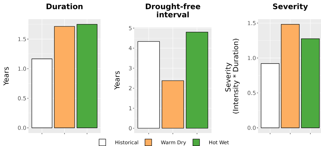
Figure 8. Drought metrics for SAPA. (Left) Average drought duration (years) historically (1979-2012) and under each climate future. (Middle) Average drought return interval (years), indicating the expected amount of time between periods of drought, historically and under each climate future. (Right) Average drought severity, a measure of drought intensity multiplied by duration, historically and under each climate future.
