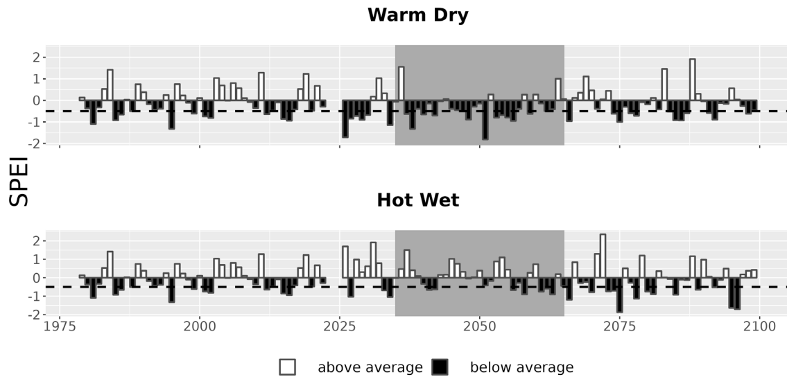
Figure 7. Drought metrics for SAPA. Drought index (SPEI; units = standard deviations from historical) timeseries for each climate future. Below-average SPEI (black bars) indicates dry conditions. The dotted line (SPEI = -0.5) indicates drought conditions.
