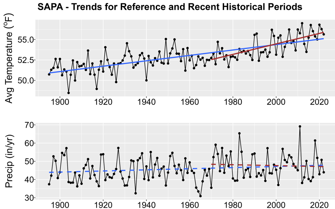
Figure 1. Historical trends in annual average temperature (upper plot) and annual total precipitation (lower plot) for SAPA from 1895-2022. Black points show yearly values while blue lines are linear regressions for the entire period record and red lines for 1970-2022 trends. Solid lines are significant trends (i.e., p < 0.05 ); dashed lines are not statistically significant.
