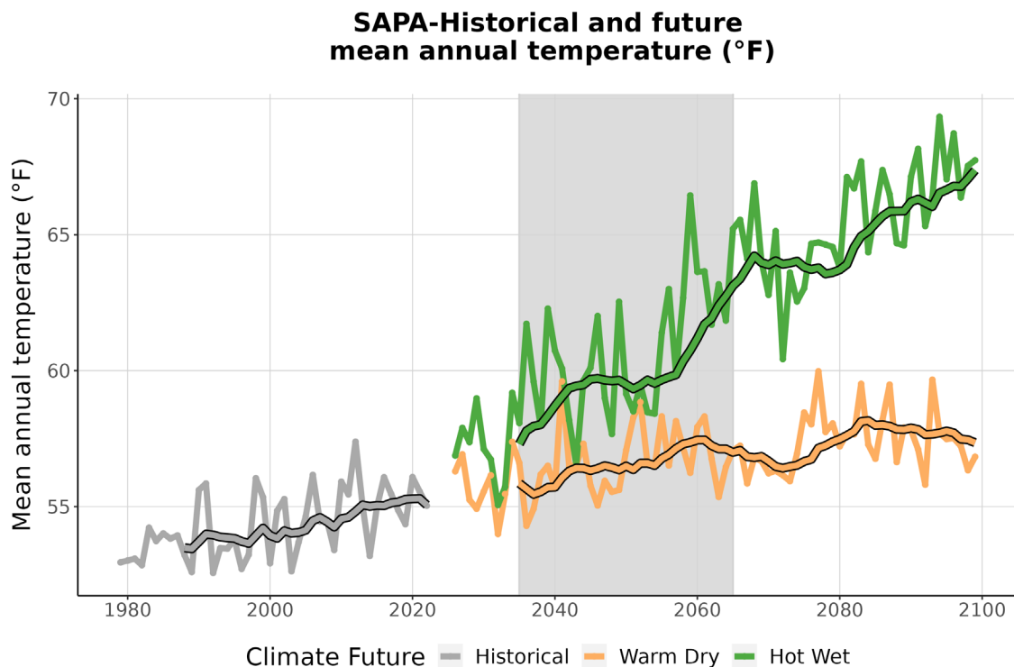
Figure 3. This graph compares observed average annual temperature at SAPA (°F) (1979-2022) with projected average annual temperature for the two climate futures over the period 2023-2099. The historically observed data
