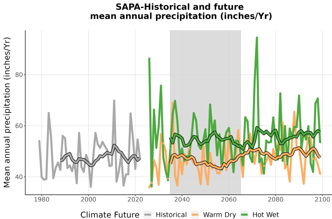
Figure 4. This graph compares observed average annual precipitation at SAPA (inches/year) (1979-2022) with projected average annual precipitation for the two climate futures over the period 2023-2099. The historically observed data is shown in gray, the Warm Dry climate future in orange, and the Hot Wet climate future in green. The smooth line running through each projection is the 10-year running average for historical observations and future projections. The gray-shaded area represents the time period that was averaged (2035-2065) to summarize future projections for the year 2050 (Appendix 1).
