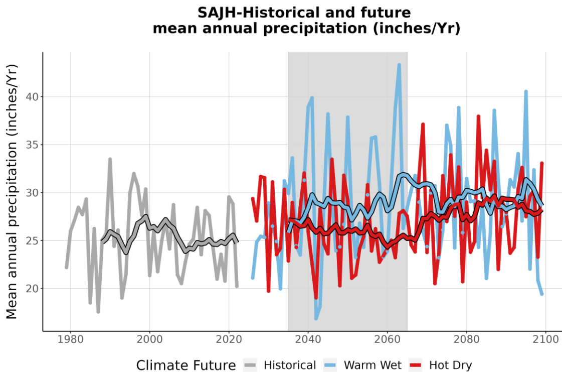
Figure 4. This graph compares observed average annual precipitation at SAJH (inches/year) (1979-2022) with projected average annual precipitation for the two climate futures over the period 2023-2099. The historically observed data is shown in gray, the Warm Wet climate future in blue, and the Hot Dry climate future in red. The smooth line running through each projection is the 10-year running average for historical observations and future projections. The gray-shaded area represents the time period that was averaged (2035-2065) to summarize future projections for the year 2050 (Appendix 1).
