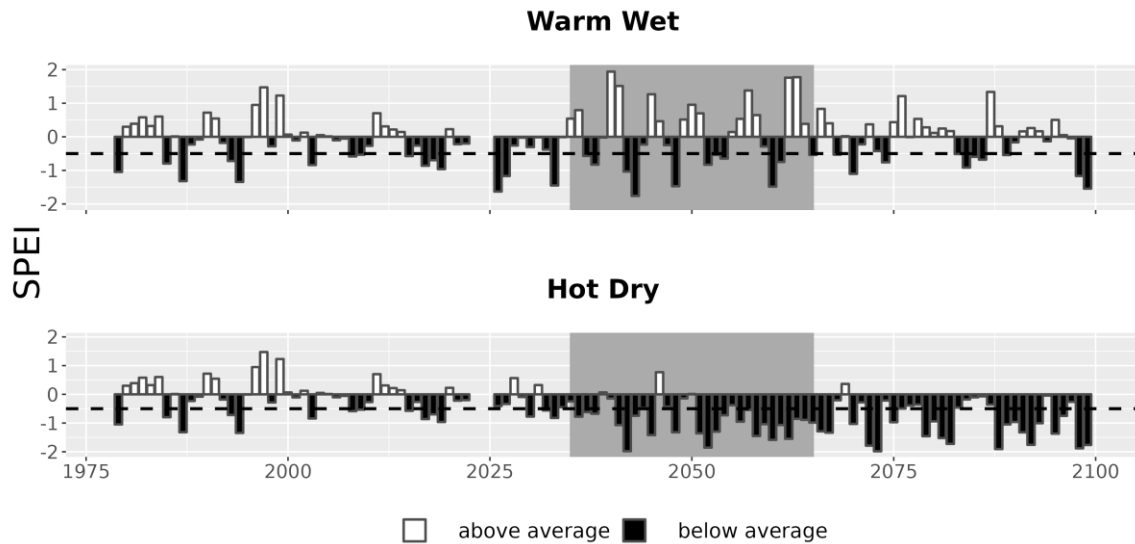
Figure 7. Drought metrics for SAJH. Drought index (SPEI; units = standard deviations from historical) timeseries for each climate future. Below-average SPEI (black bars) indicates dry conditions. The dotted line (SPEI = -0.5) indicates drought conditions.
