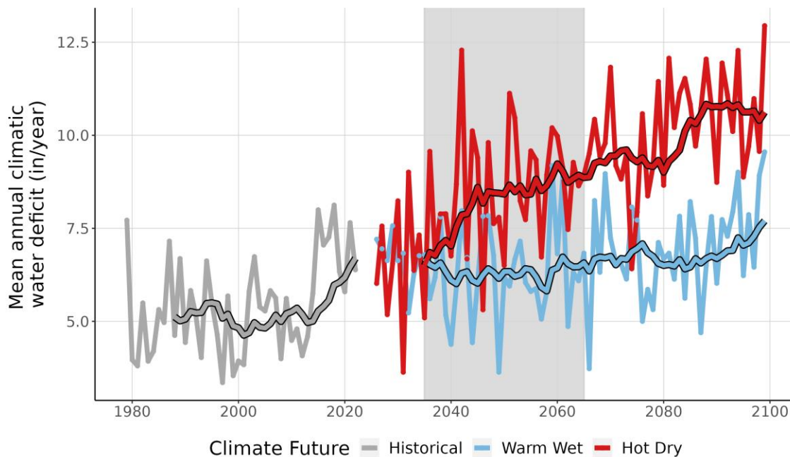
Figure 9. This line graph compares observed climatic water deficit at SAJH (inches/year) (1979-2022) with projected climatic water deficit for the two climate futures over the period 2023-2099. The historical observation data is shown in gray, the Warm Wet climate future in blue, and the Hot Dry climate future in red. The smooth line running through each projection is the 10-year running average for historical observations and future projections. Gray-shaded area represents the time period that was averaged (2035-2065) to summarize future projections for the year 2050.
