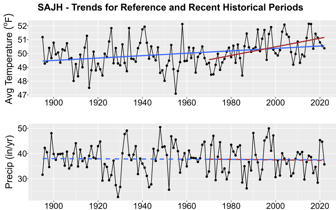
Figure 1. Historical trends in annual average temperature (upper plot) and annual total precipitation (lower plot) for SAJH from 1895-2022. Black points show yearly values while blue lines are linear regressions for the entire period record and red lines for 1970-2022 trends. Solid lines are significant trends (i.e., p < 0.05 ); dashed lines are not statistically significant.
