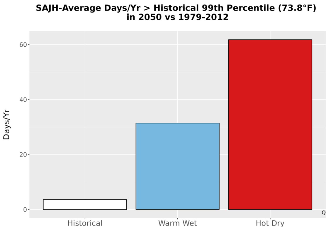
Figure 5. Metrics of extreme temperature at SAJH. The bar graph represents the average number of days annually with temperatures greater than the historical 99th percentile (73.8 °F) historically (1979-2012) and for the two climate futures (2050).
