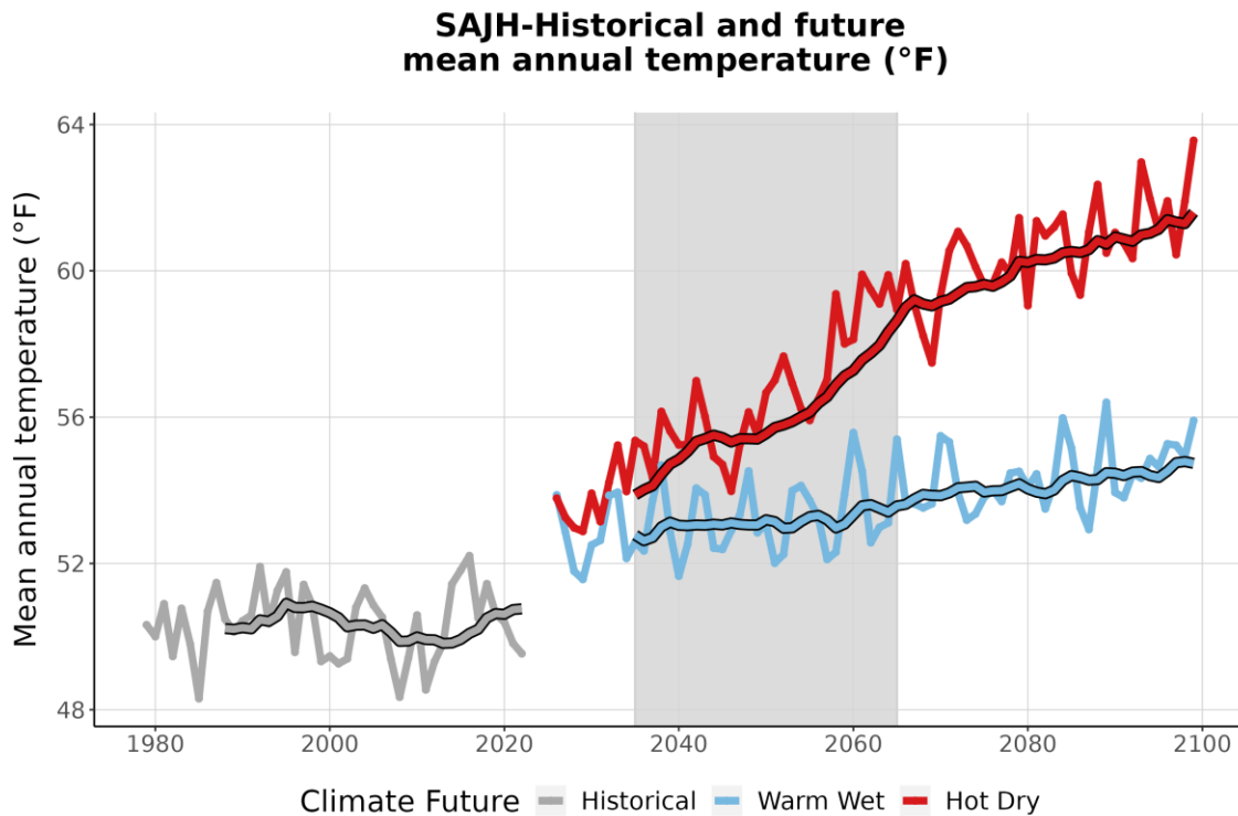
Figure 3. This graph compares observed average annual temperature at SAJH (°F) (1979-2022) with projected average annual temperature for the two climate futures over the period 2023-2099. The historically observed data is shown in gray, the Warm Wet climate future in blue, and the Hot Dry climate future in red. The smooth line
