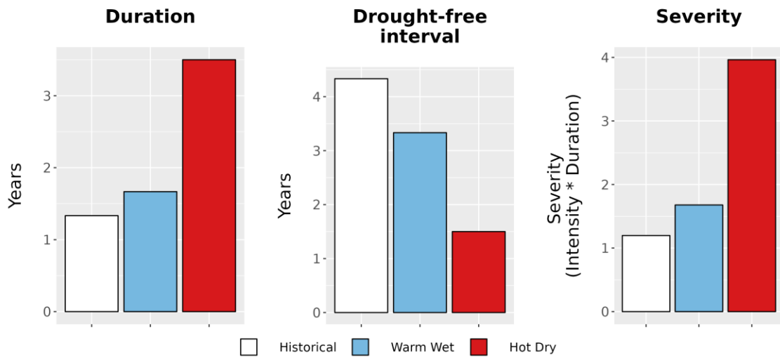
Figure 8. Drought metrics for SAJH. (Left) Average drought duration (years) historically (1979-2012) and under each climate future. (Middle) Average drought return interval (years), indicating the expected amount of time between periods of drought, historically and under each climate future. (Right) Average drought severity, a measure of drought intensity multiplied by duration, historically and under each climate future.
