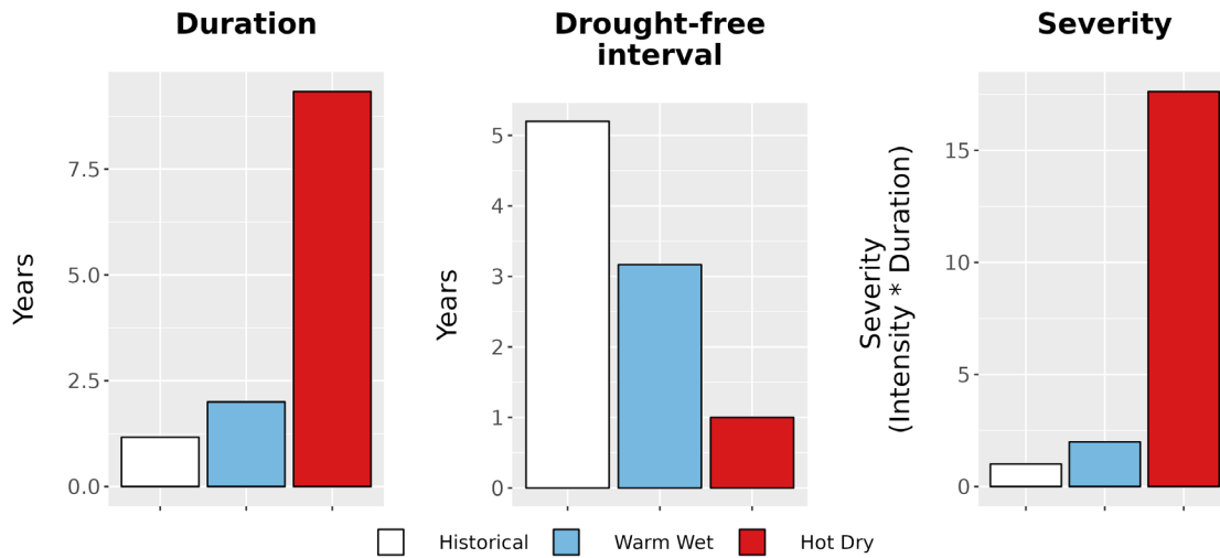
Figure 8. Drought metrics for SAGU. (Left) Average drought duration (years) historically (1979-2012) and under each climate future. (Middle) Average drought return interval (years), indicating the expected amount of time between periods of drought, historically and under each climate future. (Right) Average drought severity, a measure of drought intensity multiplied by duration, historically and under each climate future.
