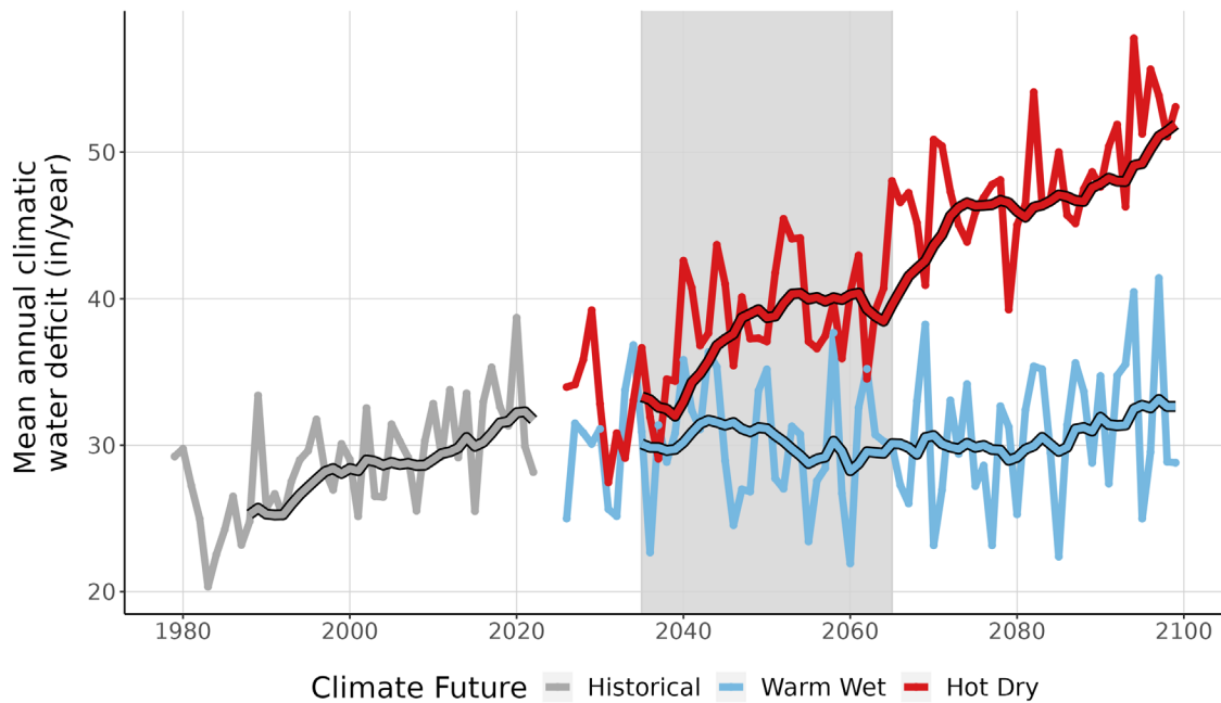
Figure 9. This line graph compares observed climatic water deficit at SAGU (inches/year) (1979-2022) with projected climatic water deficit for the two climate futures over the period 2023-2099. The historical observation data is shown in gray, the Warm Wet climate future in blue, and the Hot Dry climate future in red. The smooth line running through each projection is the 10-year running average for historical observations and future projections. Gray-shaded area represents the time period that was averaged (2035-2065) to summarize future projections for the year 2050.
