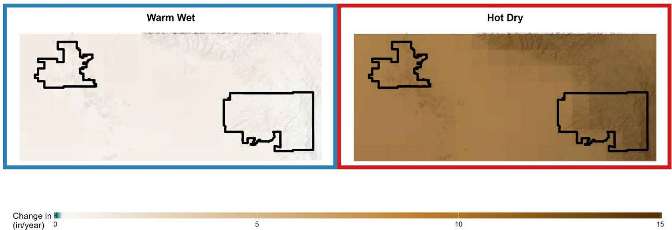
Figure A3. (Top) Map showing average annual climatic water deficit for the historical period (inches/year) and (bottom) change in average annual climatic water deficit for the two climate futures. Legends are located below each set of maps as a continuous color gradient. Gridded data is extracted from 30-year summary GIS layers for CONUS water balance model (Tercek et al 2021, 2023). ( http://screenedcleanedsummaries.s3-website-us-west-2.amazonaws.com/ ) accessed on 6/3/2024.
