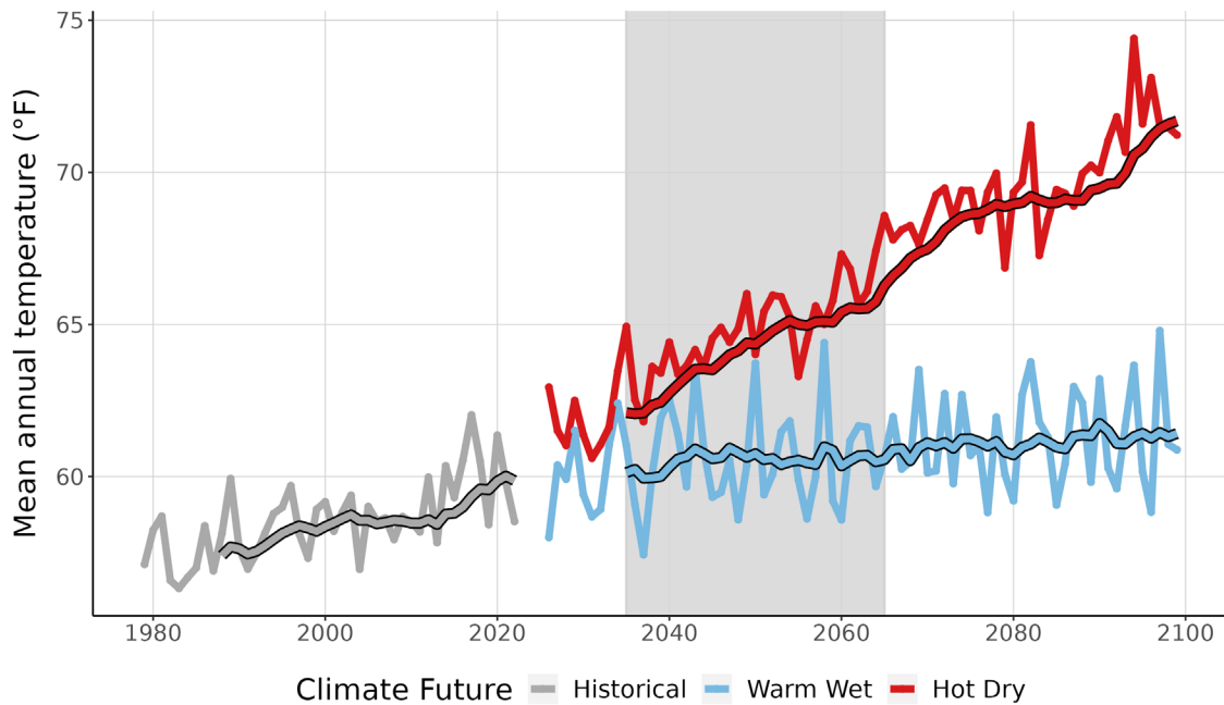
Figure 3. This graph compares observed average annual temperature at SAGU (°F) (1979-2022) with projected average annual temperature for the two climate futures over the period 2023-2099. The historically observed data is shown in gray, the Warm Wet climate future in blue, and the Hot Dry climate future in red. The smooth line running through each projection is the 10-year running average for historical observations and future projections. Gray-shaded area represents the time period that was averaged (2035-2065) to summarize future projections for the year 2050 (Appendix 1).
