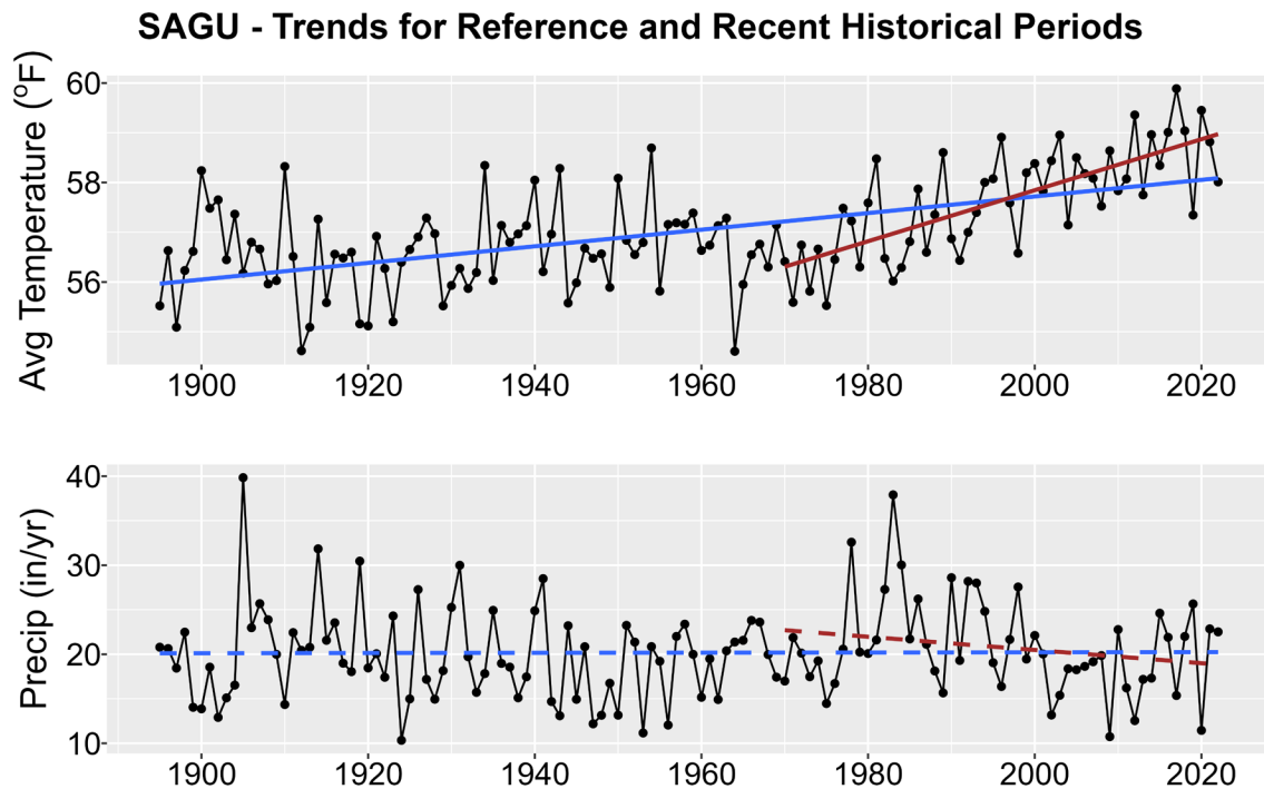
Figure 1. Historical trends in annual average temperature (upper plot) and annual total precipitation (lower plot) for SAGU from 1895-2022. Black points show yearly values while blue lines are linear regressions for the entire period record and red lines for 1970-2022 trends. Solid lines are significant trends (i.e., p < 0.05 ); dashed lines are not statistically significant.
