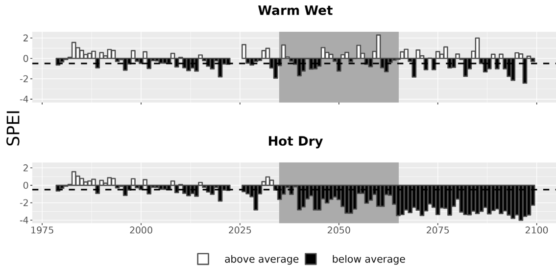
Figure 7. Drought metrics for SAGU. Drought index (SPEI; units = standard deviations from historical) timeseries for each climate future. Below-average SPEI (black bars) indicates dry conditions. The dotted line (SPEI = -0.5) indicates drought conditions.
