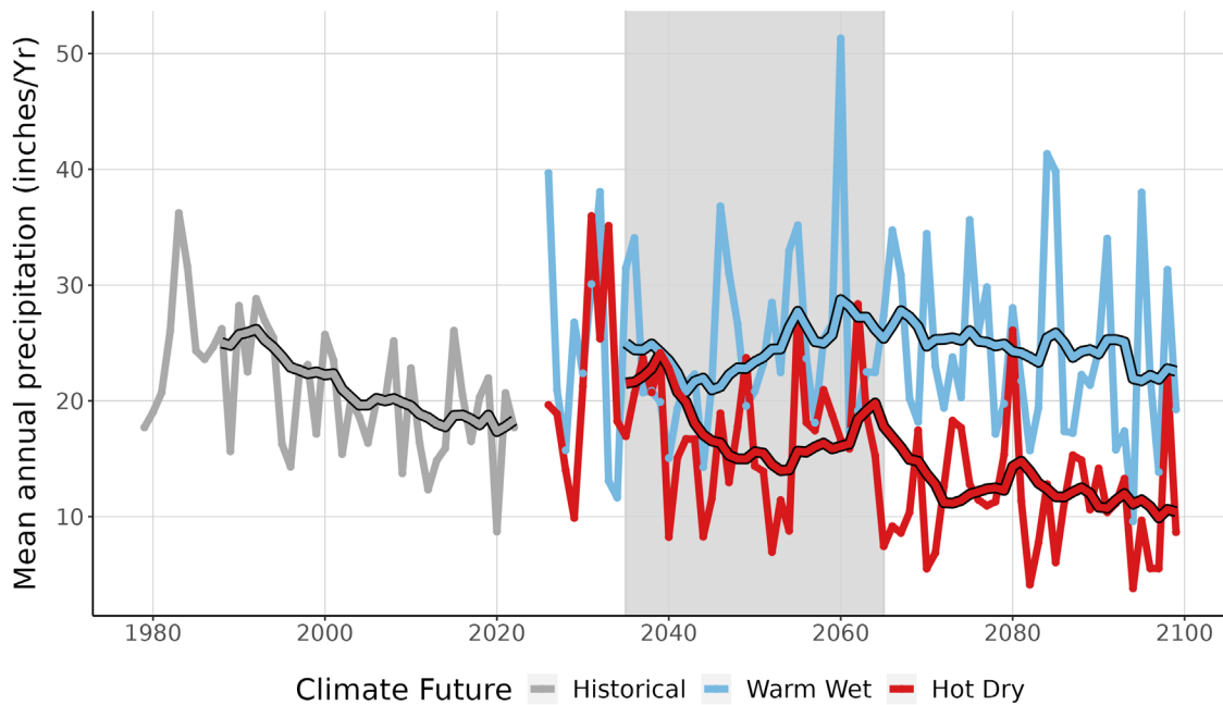
Figure 4. This graph compares observed average annual precipitation at SAGU (inches/year) (1979-2022) with projected average annual precipitation for the two climate futures over the period 2023-2099. The historically observed data is shown in gray, the Warm Wet climate future in blue, and the Hot Dry climate future in red. The smooth line running through each projection is the 10-year running average for historical observations and future projections. The gray-shaded area represents the time period that was averaged (2035-2065) to summarize future projections for the year 2050 (Appendix 1).
