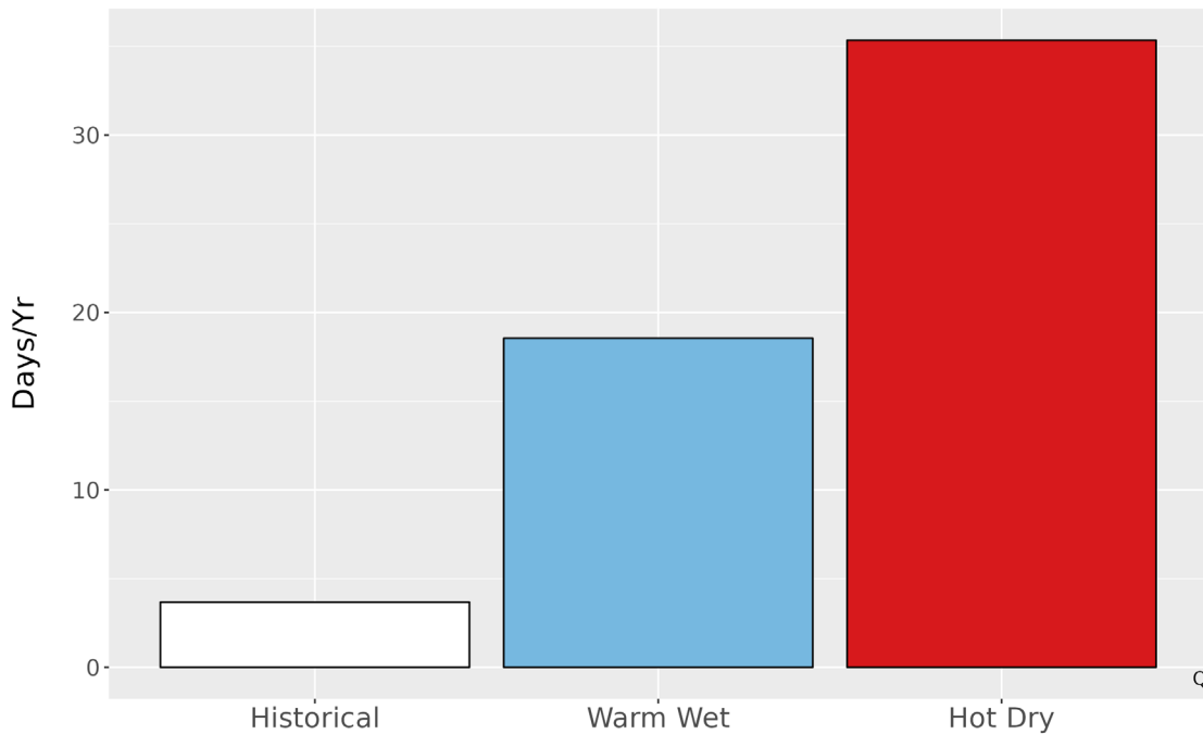
Figure 5. Metrics of extreme temperature at SAGU. The bar graph represents the average number of days annually with temperatures greater than the historical 99th percentile (94.2 °F) historically (1979-2012) and for the two climate futures (2050).
