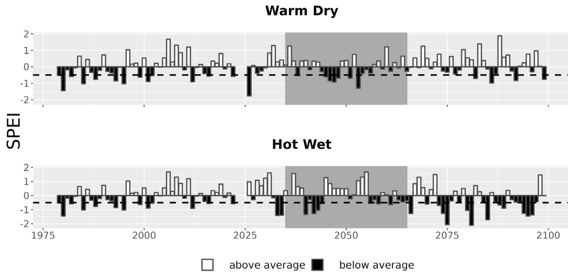
Figure 7. Drought metrics for SAGA. Drought index (SPEI; units = standard deviations from historical) timeseries for each climate future. Below-average SPEI (black bars) indicates dry conditions. The dotted line (SPEI = -0.5) indicates drought conditions.
