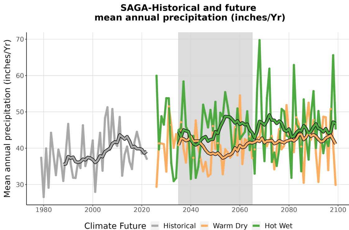
Figure 4. This graph compares observed average annual precipitation at SAGA (inches/year) (1979-2022) with projected average annual precipitation for the two climate futures over the period 2023-2099. The historically observed data is shown in gray, the Warm Dry climate future in orange, and the Hot Wet climate future in green. The smooth line running through each projection is the 10-year running average for historical observations and future projections. The gray-shaded area represents the time period that was averaged (2035-2065) to summarize future projections for the year 2050 (Appendix 1).
