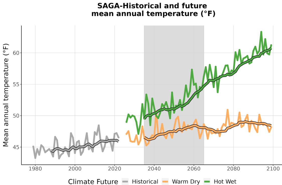
Figure 3. This graph compares observed average annual temperature at SAGA (°F) (1979-2022) with projected average annual temperature for the two climate futures over the period 2023-2099. The historically observed data is shown in gray, the Warm Dry climate future in orange, and the Hot Wet climate future in green. The smooth line
