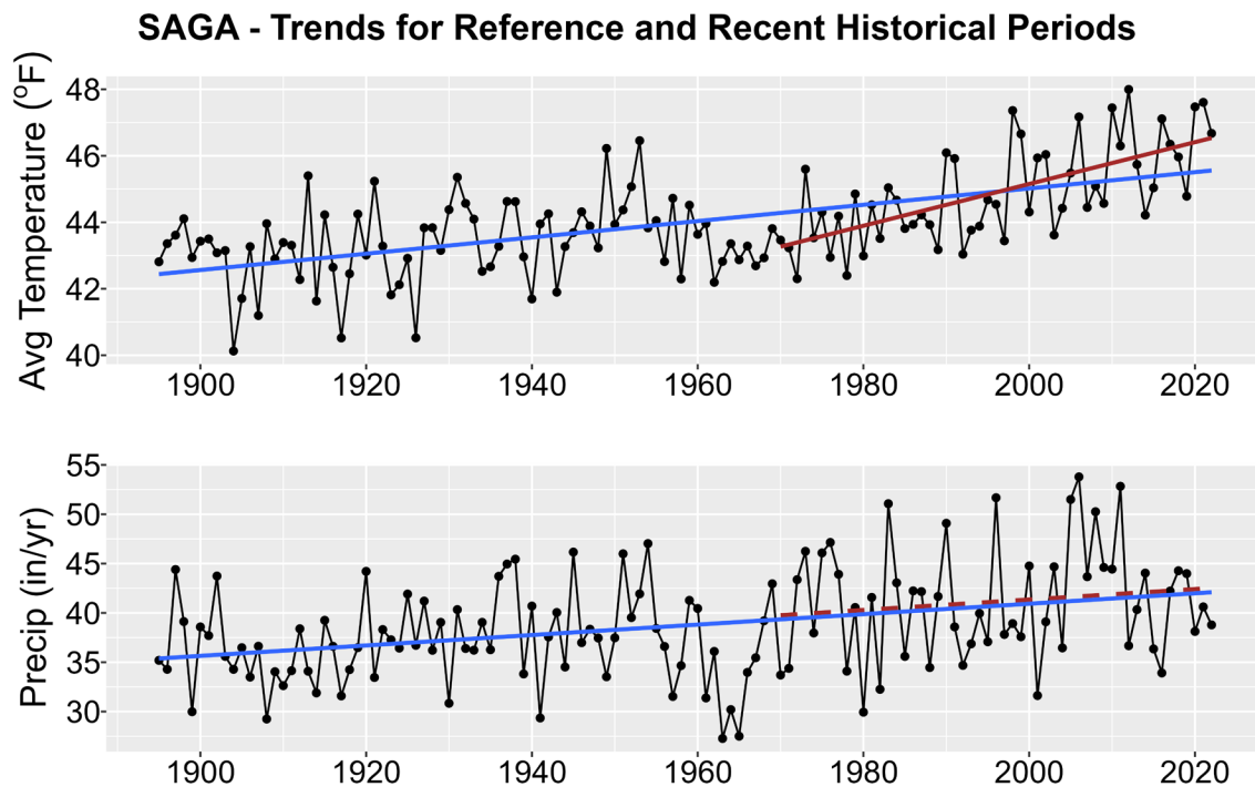
Figure 1. Historical trends in annual average temperature (upper plot) and annual total precipitation (lower plot) for SAGA from 1895-2022. Black points show yearly values while blue lines are linear regressions for the entire period record and red lines for 1970-2022 trends. Solid lines are significant trends (i.e., p < 0.05 ); dashed lines are not statistically significant.
