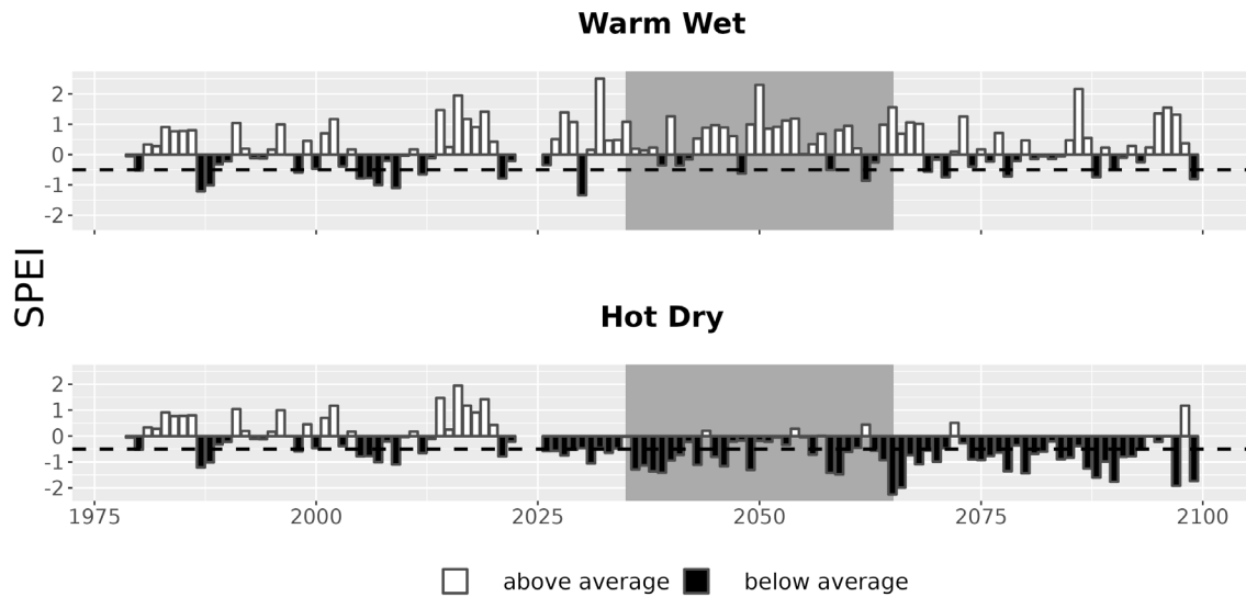
Figure 7. Drought metrics for SACN. Drought index (SPEI; units = standard deviations from historical) timeseries for each climate future. Below-average SPEI (black bars) indicates dry conditions. The dotted line (SPEI = -0.5) indicates drought conditions.
