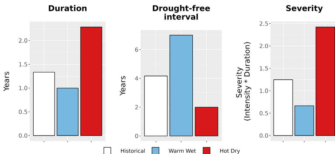
Figure 8. Drought metrics for SACN. (Left) Average drought duration (years) historically (1979-2012) and under each climate future. (Middle) Average drought return interval (years), indicating the expected amount of time between periods of drought, historically and under each climate future. (Right) Average drought severity, a measure of drought intensity multiplied by duration, historically and under each climate future.
