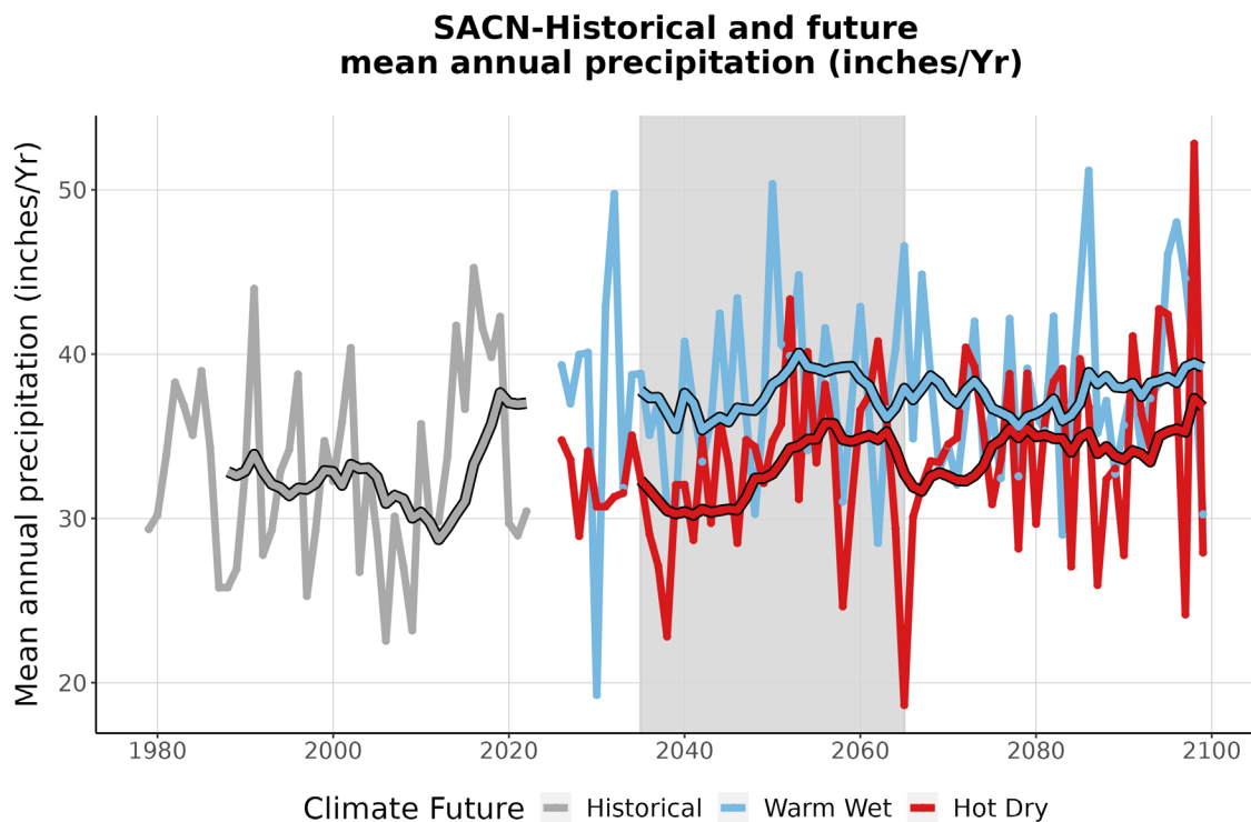
Figure 4. This graph compares observed average annual precipitation at SACN (inches/year) (1979-2022) with projected average annual precipitation for the two climate futures over the period 2023-2099. The historically observed data is shown in gray, the Warm Wet climate future in blue, and the Hot Dry climate future in red. The smooth line running through each projection is the 10-year running average for historical observations and future projections. The gray-shaded area represents the time period that was averaged (2035-2065) to summarize future projections for the year 2050 (Appendix 1).
