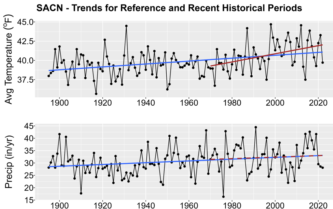
Figure 1. Historical trends in annual average temperature (upper plot) and annual total precipitation (lower plot) for SACN from 1895-2022. Black points show yearly values while blue lines are linear regressions for the entire period record and red lines for 1970-2022 trends. Solid lines are significant trends (i.e., p < 0.05 ); dashed lines are not statistically significant.
