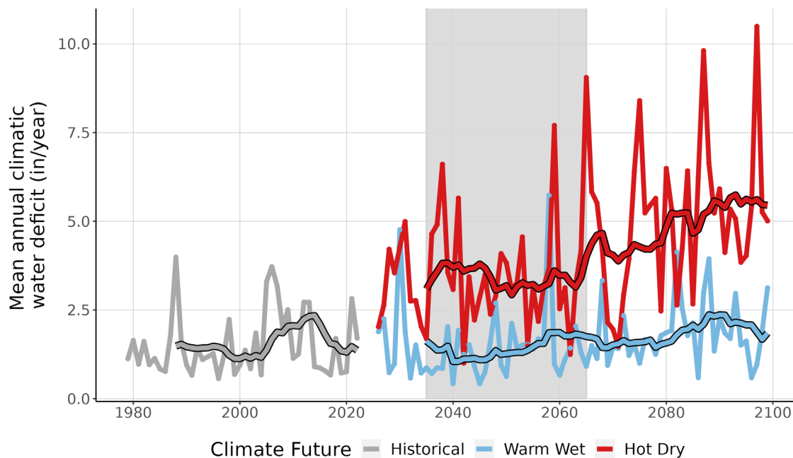
Figure 9. This line graph compares observed climatic water deficit at SACN (inches/year) (1979-2022) with projected climatic water deficit for the two climate futures over the period 2023-2099. The historical observation data is shown in gray, the Warm Wet climate future in blue, and the Hot Dry climate future in red. The smooth line running through each projection is the 10-year running average for historical observations and future projections. Gray-shaded area represents the time period that was averaged (2035-2065) to summarize future projections for the year 2050.
