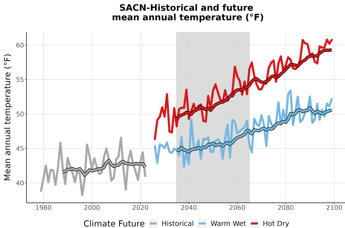
Figure 3. This graph compares observed average annual temperature at SACN (°F) (1979-2022) with projected average annual temperature for the two climate futures over the period 2023-2099. The historically observed data
