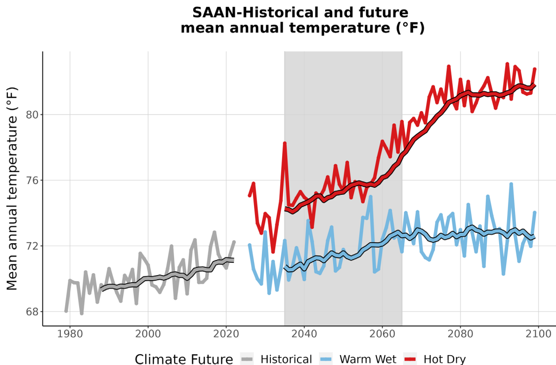
Figure 3. This graph compares observed average annual temperature at SAAN (°F) (1979-2022) with projected average annual temperature for the two climate futures over the period 2023-2099. The historically observed data
