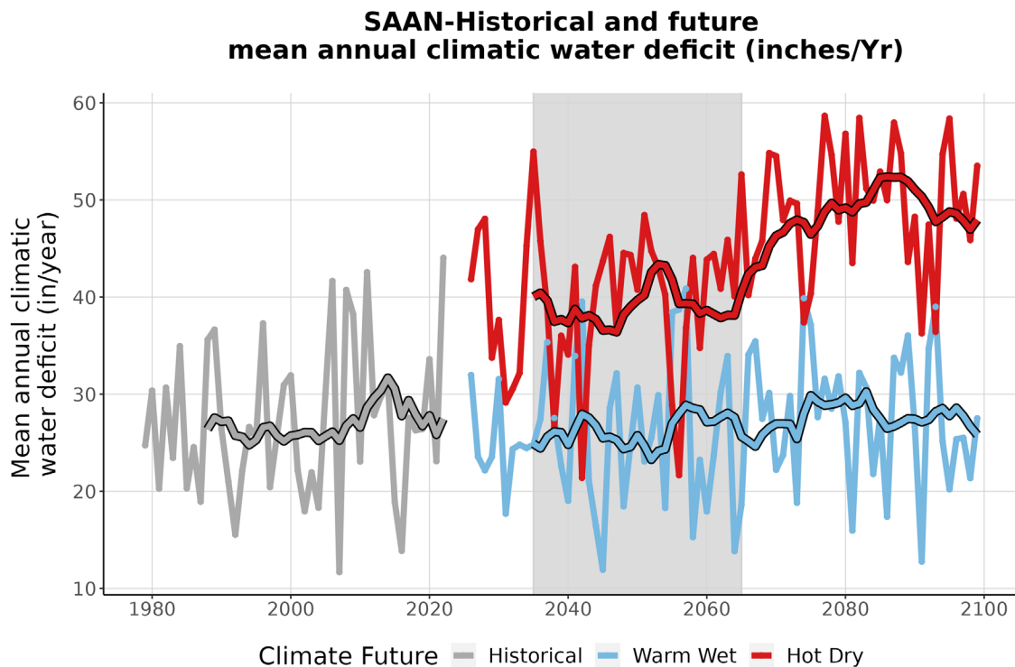
Figure 9. This line graph compares observed climatic water deficit at SAAN (inches/year) (1979-2022) with projected climatic water deficit for the two climate futures over the period 2023-2099. The historical observation data is shown in gray, the Warm Wet climate future in blue, and the Hot Dry climate future in red. The smooth line running through each projection is the 10-year running average for historical observations and future projections. Gray-shaded area represents the time period that was averaged (2035-2065) to summarize future projections for the year 2050.
