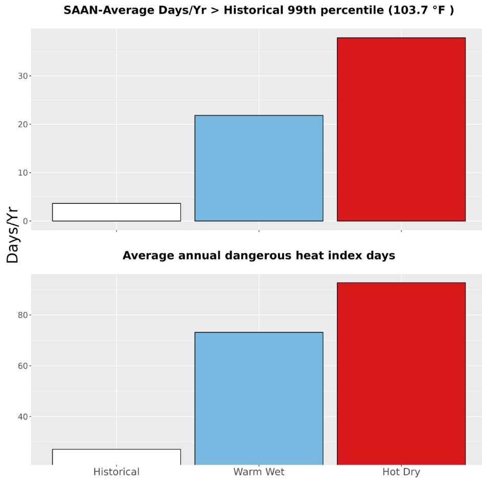
Figure 5. The upper bar graph represents the average number of days annually with temperatures greater than the historical 99th percentile (103.7 °F) historically (1979-2012) and for the two climate futures (2050). The bottom bar graph represents the average annual number of dangerous heat index days historically and for the two climate futures. Dangerous heat index days are days that exceed 105 °F.
