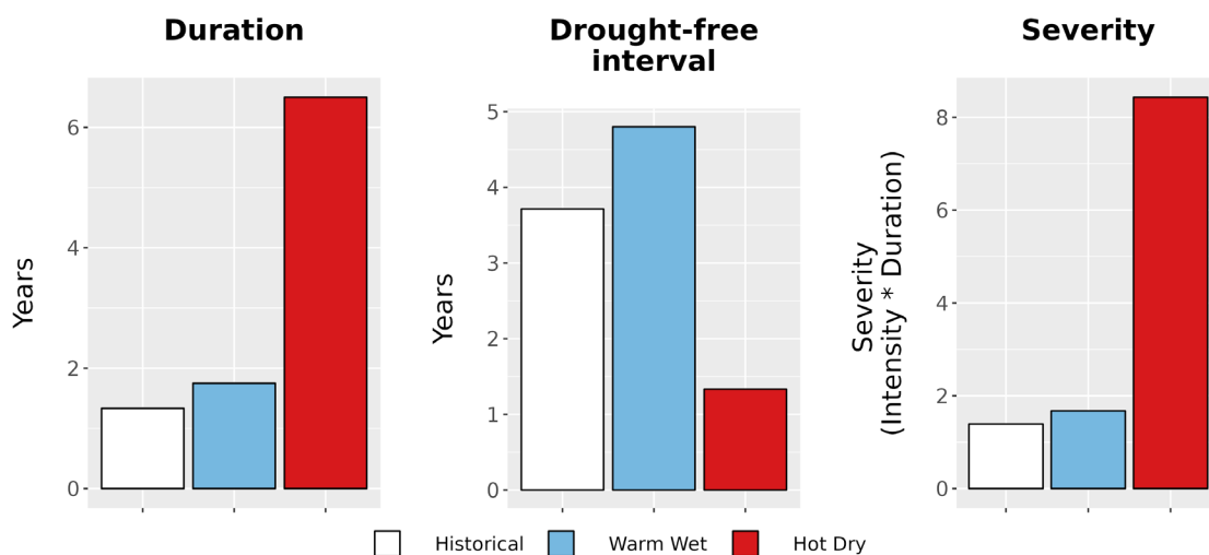
Figure 8. Drought metrics for SAAN. (Left) Average drought duration (years) historically (1979-2012) and under each climate future. (Middle) Average drought return interval (years), indicating the expected amount of time between periods of drought, historically and under each climate future. (Right) Average drought severity, a measure of drought intensity multiplied by duration, historically and under each climate future.
