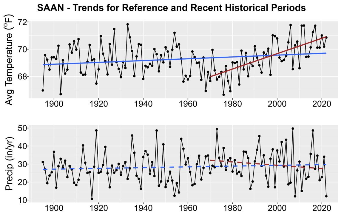
Figure 1. Historical trends in annual average temperature (upper plot) and annual total precipitation (lower plot) for SAAN from 1895-2022. Black points show yearly values while blue lines are linear regressions for the entire period record and red lines for 1970-2022 trends. Solid lines are significant trends (i.e., p < 0.05 ); dashed lines are not statistically significant.
