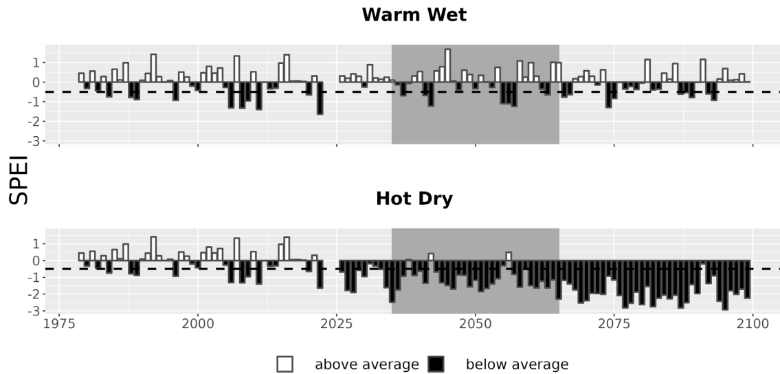
Figure 7. Drought metrics for SAAN. Drought index (SPEI; units = standard deviations from historical) timeseries for each climate future. Below-average SPEI (black bars) indicates dry conditions. The dotted line (SPEI = -0.5) indicates drought conditions.
