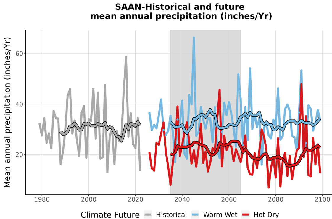
Figure 4. This graph compares observed average annual precipitation at SAAN (inches/year) (1979-2022) with projected average annual precipitation for the two climate futures over the period 2023-2099. The historically observed data is shown in gray, the Warm Wet climate future in blue, and the Hot Dry climate future in red. The smooth line running through each projection is the 10-year running average for historical observations and future projections. The gray-shaded area represents the time period that was averaged (2035-2065) to summarize future projections for the year 2050 (Appendix 1).
