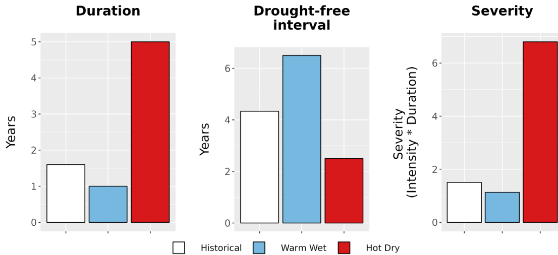
Figure 8. Drought metrics for RUCA. (Left) Average drought duration (years) historically (1979-2012) and under each climate future. (Middle) Average drought return interval (years), indicating the expected amount of time between periods of drought, historically and under each climate future. (Right) Average drought severity, a measure of drought intensity multiplied by duration, historically and under each climate future.
