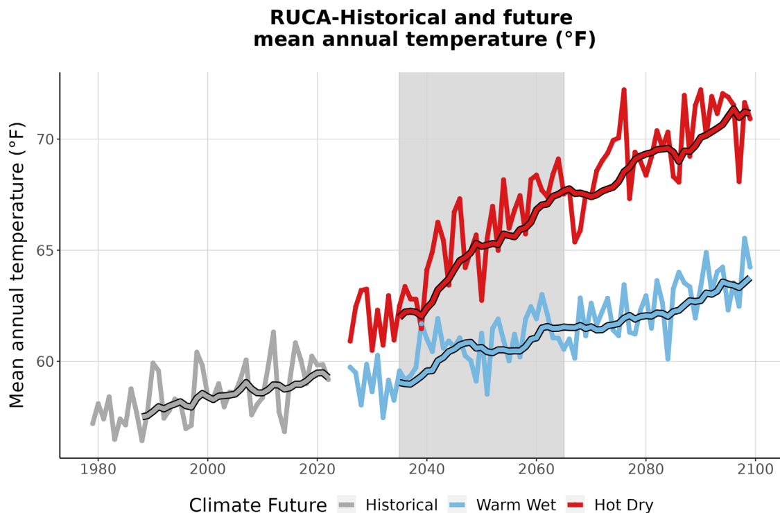
Figure 3. This graph compares observed average annual temperature at RUCA (°F) (1979-2022) with projected average annual temperature for the two climate futures over the period 2023-2099. The historically observed data
