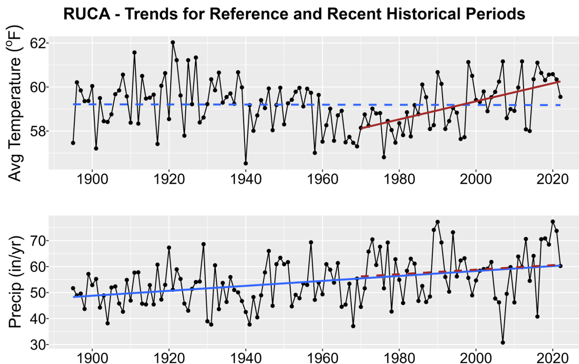
Figure 1. Historical trends in annual average temperature (upper plot) and annual total precipitation (lower plot) for RUCA from 1895-2022. Black points show yearly values while blue lines are linear regressions for the entire period record and red lines for 1970-2022 trends. Solid lines are significant trends (i.e., p < 0.05 ); dashed lines are not statistically significant.
