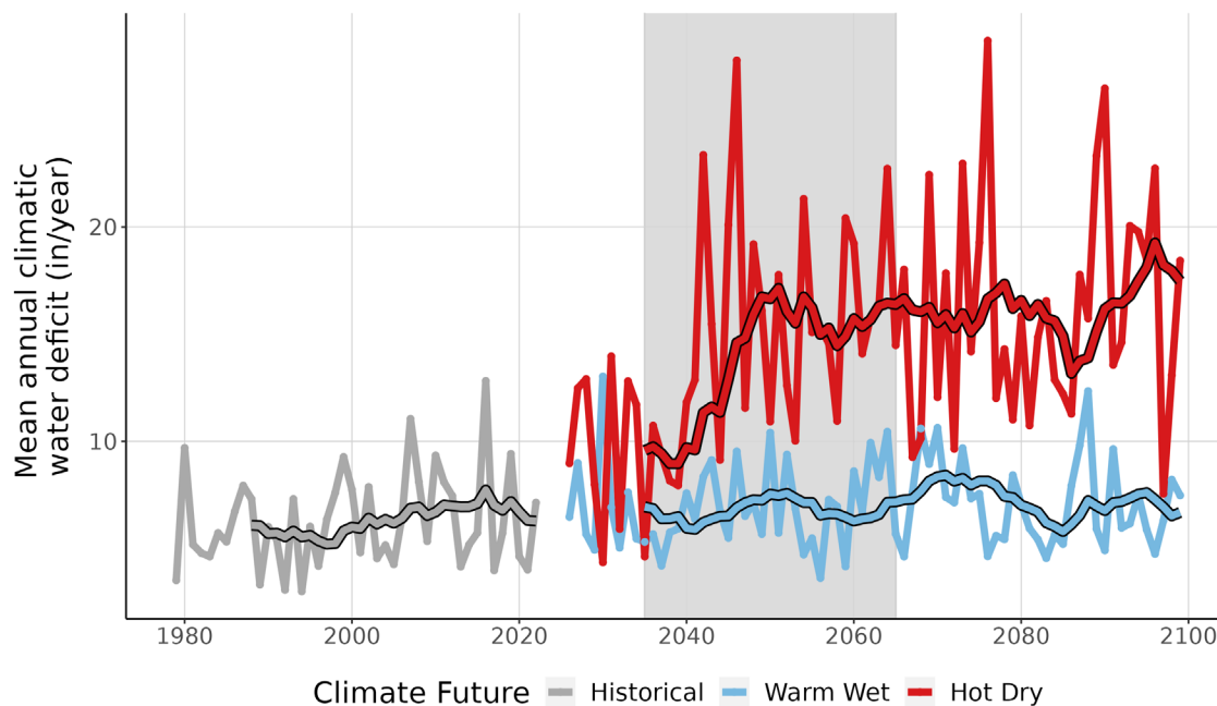
Figure 9. This line graph compares observed climatic water deficit at RUCA (inches/year) (1979-2022) with projected climatic water deficit for the two climate futures over the period 2023-2099. The historical observation data is shown in gray, the Warm Wet climate future in blue, and the Hot Dry climate future in red. The smooth line running through each projection is the 10-year running average for historical observations and future projections. Gray-shaded area represents the time period that was averaged (2035-2065) to summarize future projections for the year 2050.
