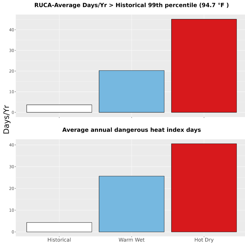
Figure 5. The upper bar graph represents the average number of days annually with temperatures greater than the historical 99th percentile (94.7 °F) historically (1979-2012) and for the two climate futures (2050). The bottom bar graph represents the average annual number of dangerous heat index days historically and for the two climate futures. Dangerous heat index days are days that exceed 105 °F.
