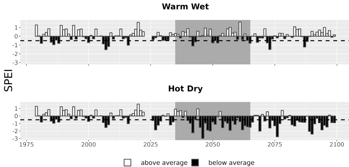
Figure 7. Drought metrics for RUCA. Drought index (SPEI; units = standard deviations from historical) timeseries for each climate future. Below-average SPEI (black bars) indicates dry conditions. The dotted line (SPEI = -0.5) indicates drought conditions.
