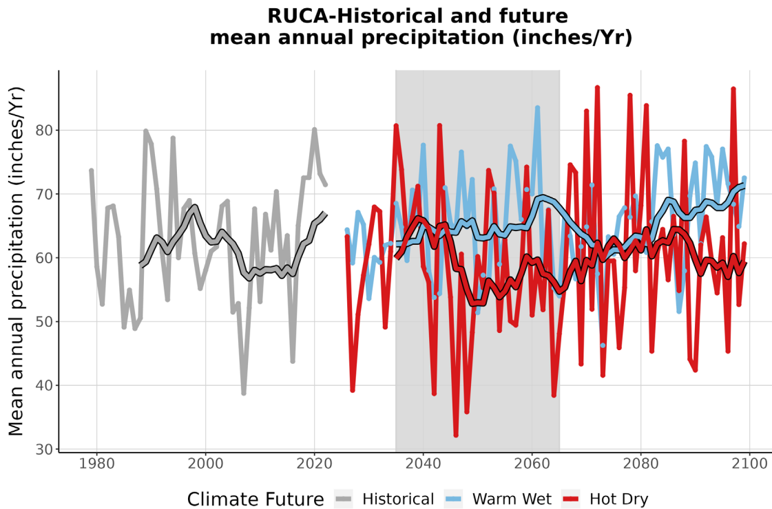
Figure 4. This graph compares observed average annual precipitation at RUCA (inches/year) (1979-2022) with projected average annual precipitation for the two climate futures over the period 2023-2099. The historically observed data is shown in gray, the Warm Wet climate future in blue, and the Hot Dry climate future in red. The smooth line running through each projection is the 10-year running average for historical observations and future projections. The gray-shaded area represents the time period that was averaged (2035-2065) to summarize future projections for the year 2050 (Appendix 1).
