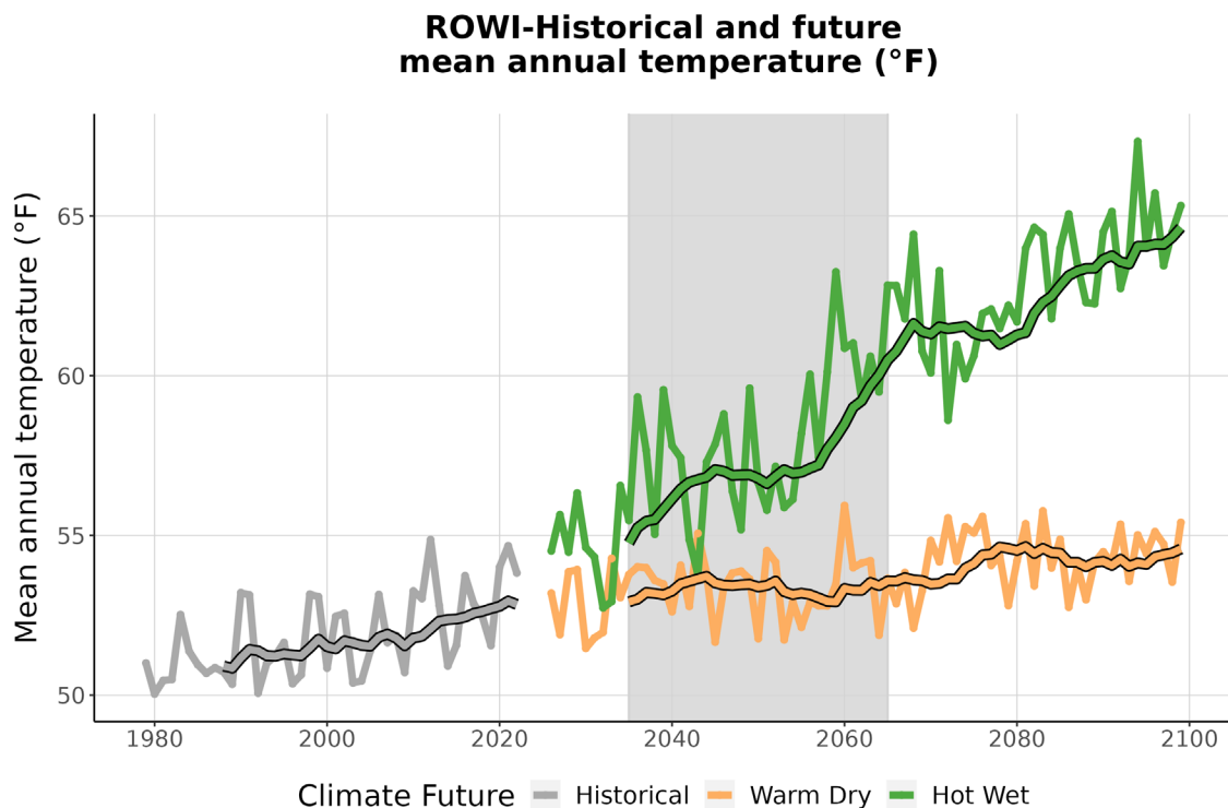
Figure 3. This graph compares observed average annual temperature at ROWI (°F) (1979-2022) with projected average annual temperature for the two climate futures over the period 2023-2099. The historically observed data
