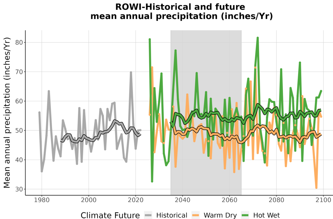
Figure 4. This graph compares observed average annual precipitation at ROWI (inches/year) (1979-2022) with projected average annual precipitation for the two climate futures over the period 2023-2099. The historically observed data is shown in gray, the Warm Dry climate future in orange, and the Hot Wet climate future in green. The smooth line running through each projection is the 10-year running average for historical observations and future projections. The gray-shaded area represents the time period that was averaged (2035-2065) to summarize future projections for the year 2050 (Appendix 1).
