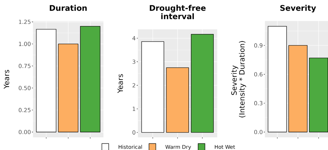
Figure 8. Drought metrics for ROWI. (Left) Average drought duration (years) historically (1979-2012) and under each climate future. (Middle) Average drought return interval (years), indicating the expected amount of time between periods of drought, historically and under each climate future. (Right) Average drought severity, a measure of drought intensity multiplied by duration, historically and under each climate future.
