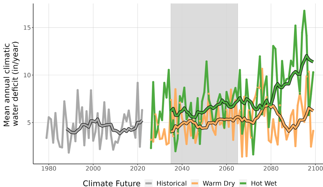
Figure 9. This line graph compares observed climatic water deficit at ROWI (inches/year) (1979-2022) with projected climatic water deficit for the two climate futures over the period 2023-2099. The historical observation data is shown in gray, the Warm Dry climate future in orange, and the Hot Wet climate future in green. The smooth line running through each projection is the 10-year running average for historical observations and future projections. Gray-shaded area represents the time period that was averaged (2035-2065) to summarize future projections for the year 2050.
