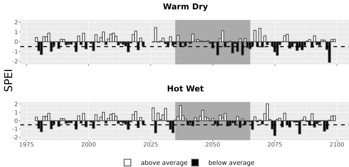
Figure 7. Drought metrics for ROWI. Drought index (SPEI; units = standard deviations from historical) timeseries for each climate future. Below-average SPEI (black bars) indicates dry conditions. The dotted line (SPEI = -0.5) indicates drought conditions.
