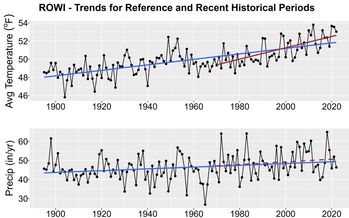
Figure 1. Historical trends in annual average temperature (upper plot) and annual total precipitation (lower plot) for ROWI from 1895-2022. Black points show yearly values while blue lines are linear regressions for the entire period record and red lines for 1970-2022 trends. Solid lines are significant trends (i.e., p < 0.05 ); dashed lines are not statistically significant.
